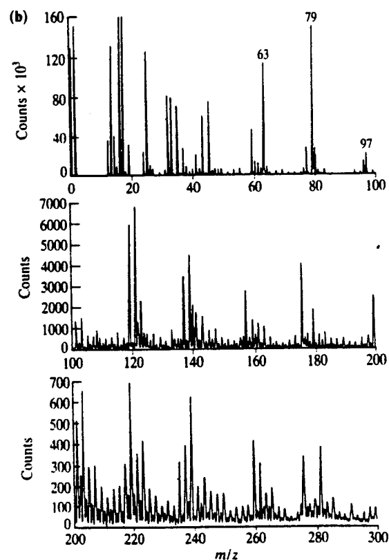
Figure (continued) (b) Negative ion spectrum; annotated peaks are due to PO 2 - (63), PO 3 - (79), H 2 PO 4 - (97); all other peaks are molecular fragments from organic species.
