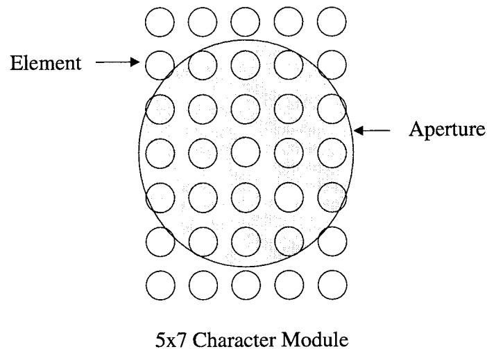
Figure 1. PCMS Character Module and Photometer Aperture.
