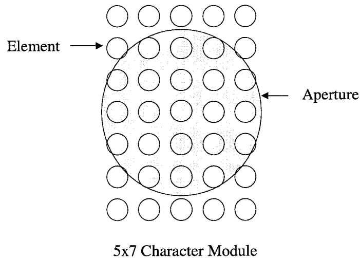
Figure 5. Luminance Meter Aperture Relative to Character Module.
