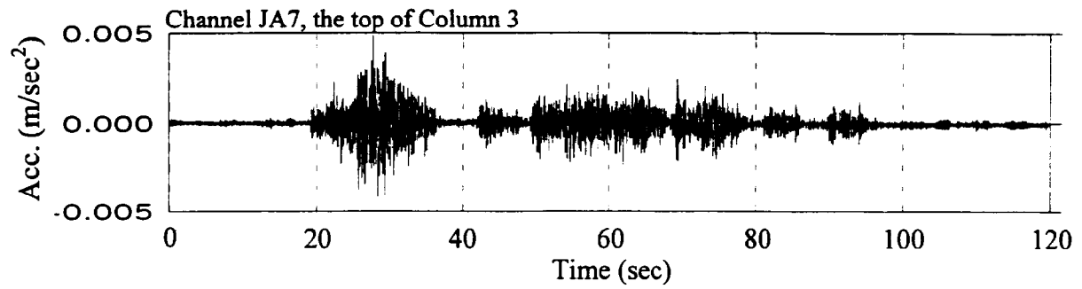
Figure 5.3: Typical Longitudinal Acceleration Time History of Super-Structure at Jamboree Road Overcrossing
