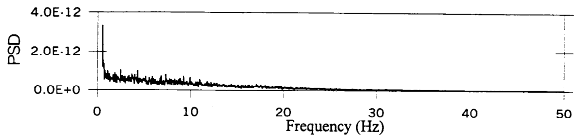
Figure 5.17: Power Spectral Density Function of Averaged Displacement
