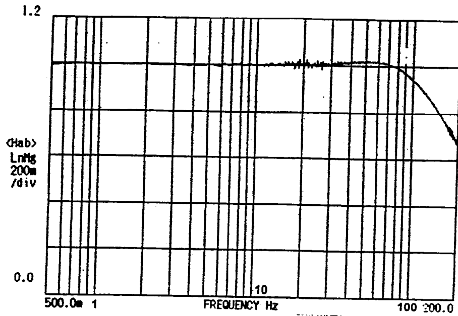
Figure 3.2: Frequency Response Function of a Force-Balance Servo Accelerometer; Amplitude
