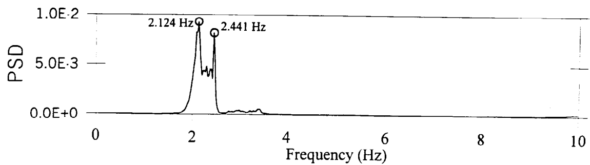
Figure 6.23: Power Spectral Density Function of Transverse Accelerations During Bumping Tests
