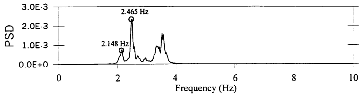
Figure 6.20: Power Spectral Density Function of Vertical Accelerations During Braking Vibration Tests
