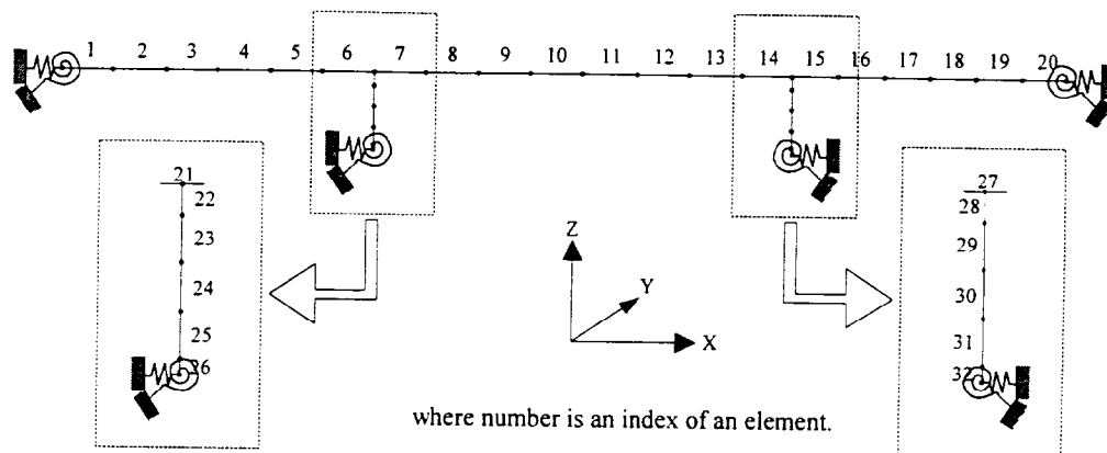
Figure 2.9: Finite Element Model of Jamboree Road Overcrossing
