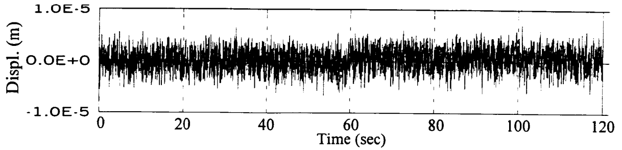
Figure 5.5: Typical Longitudinal Displacement Time History of Super-Structure at Abutment 4 at Jamboree Road Overcrossing
