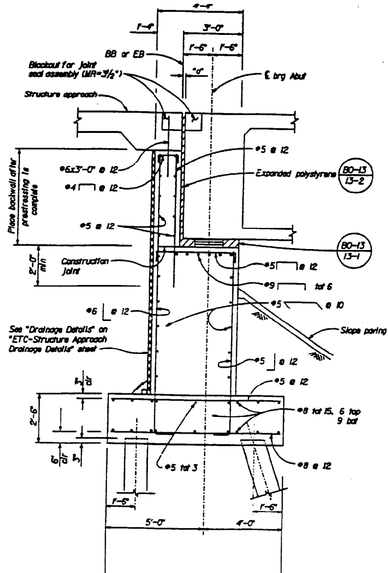
Figure 2.4: Typical Abutment Section at Jamboree Road Overcrossing
