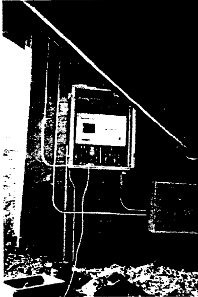
Figure 3.26: Data Recorder Installed on the Abutment Wall at Jamboree Road Overcrossing
