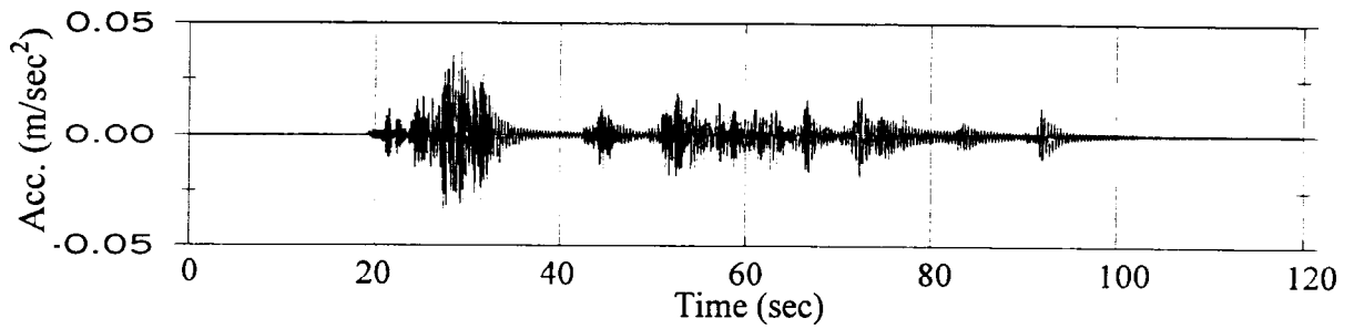
Figure 5.6: Typical Vertical Acceleration Time History in the Middle of Span 2 at Jamboree Road Overcrossing
