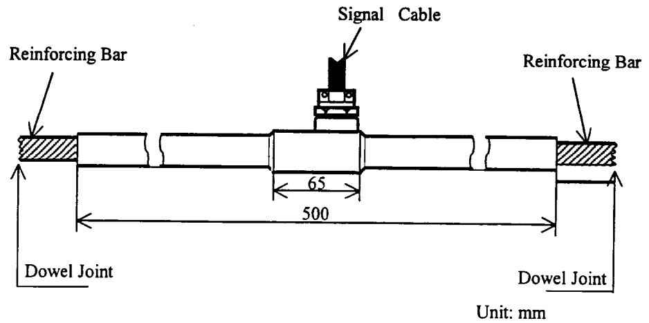
Figure 3.9: Rebar Strain Gauge; Outside View
