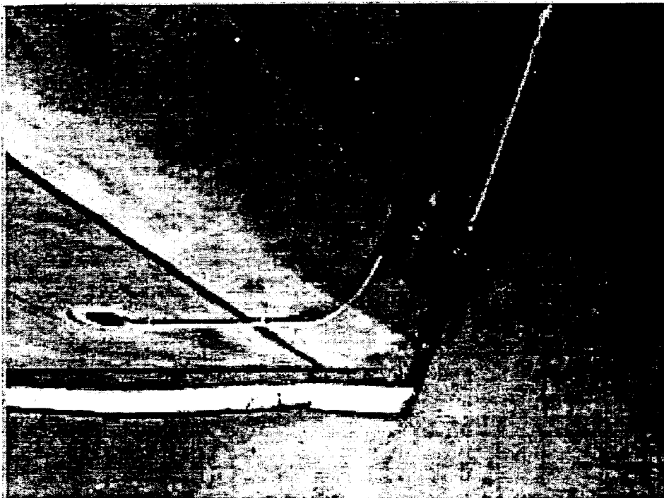
Figure 3.20: Displacement Sensor at West Street On-Ramp
