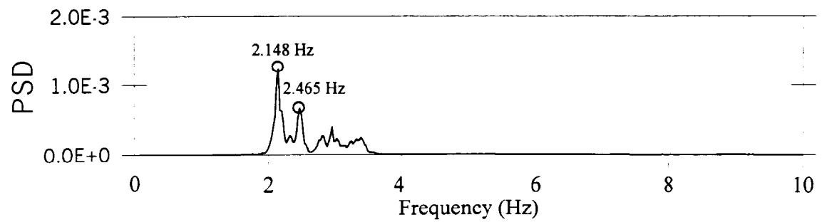
Figure 6.21: Power Spectral Density Function of Transverse Accelerations During Braking Vibration Tests
