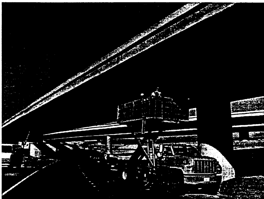
Figure 3.36: Installation of Accelerometers Using a Cherry Picker
