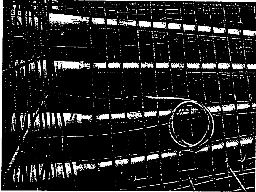
Figure 3.13: Strain Gauge Embedded in Super-Structure of West Street On-Ramp
