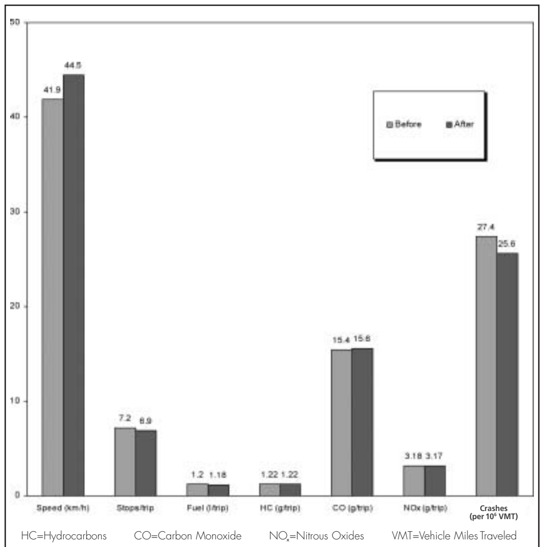
Figure 6. Average Measure of Efficiency Comparison
