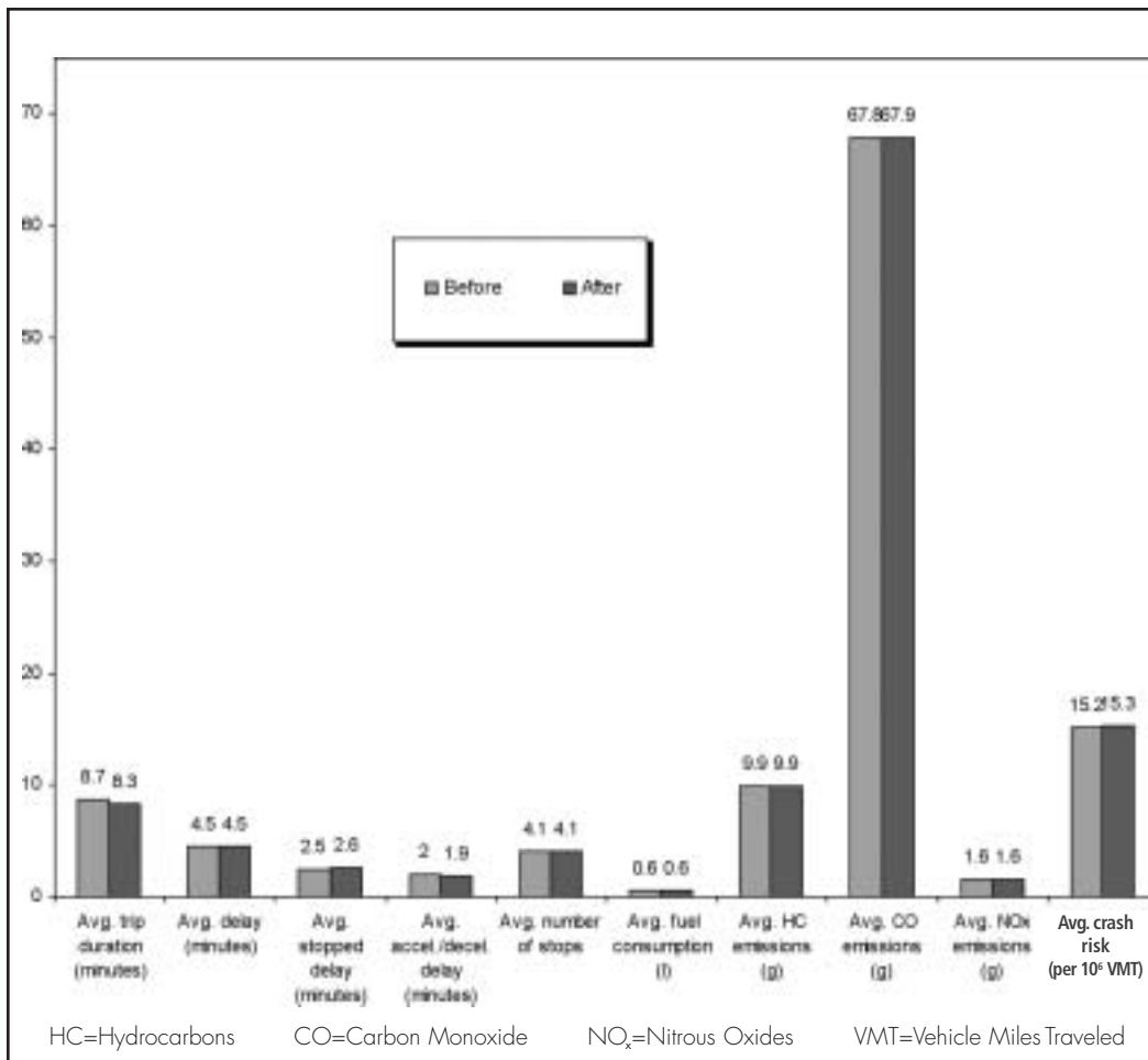
Figure 7. Comparison of Means
