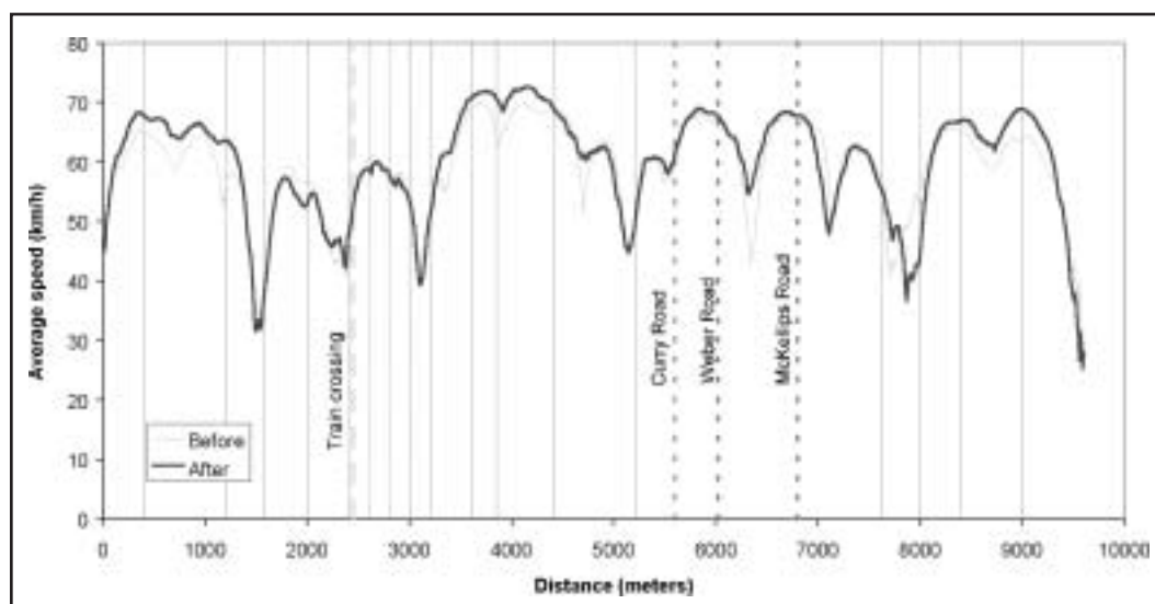
Figure 4. Northbound Speed Profile Comparison
