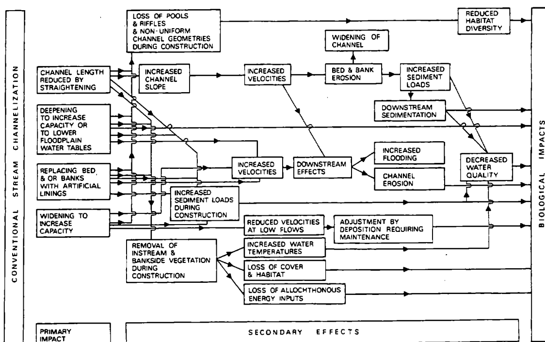
Figure 1. Principal effects of major types of channelization (taken from Brookes 1988)
