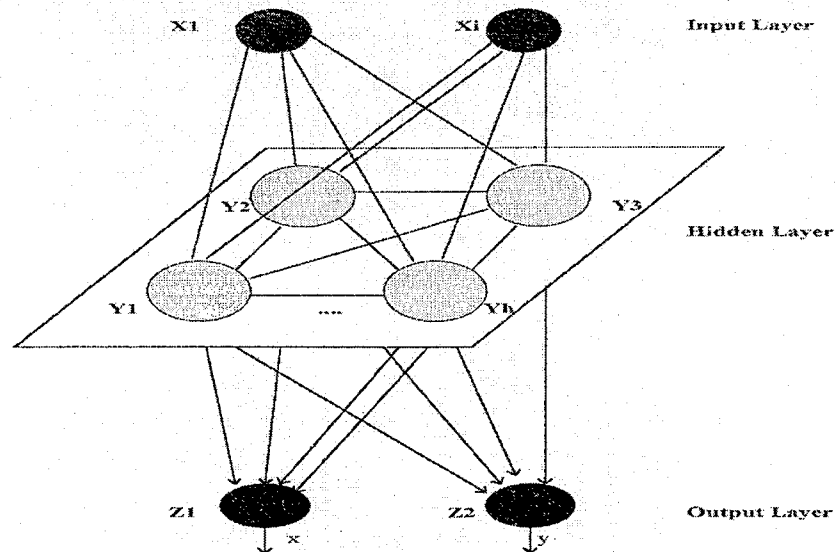
FIGURE 5. SELF-ORGANIZING MAP ARCHITECTURE
