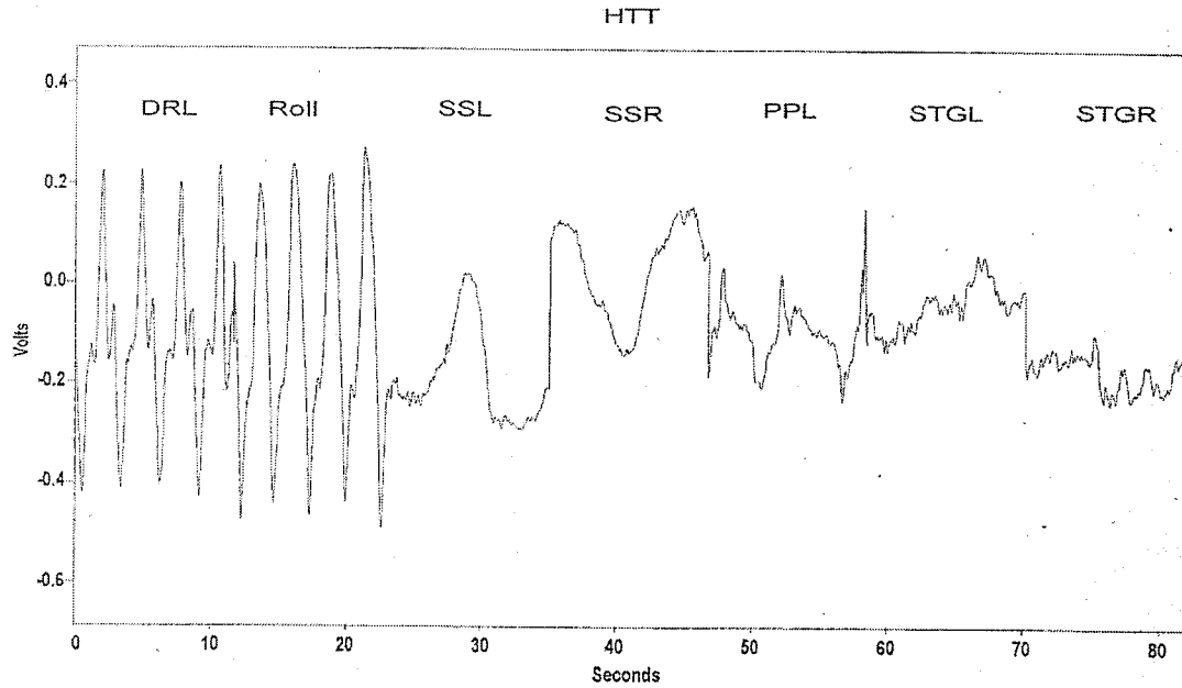
FIGURE 10. HORIZONTAL TAIL LOAD DURING MANEUVERS
