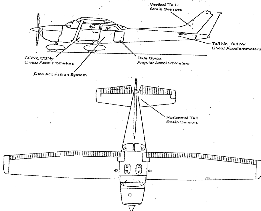
FIGURE 8. INSTRUMENTATION SETUP
