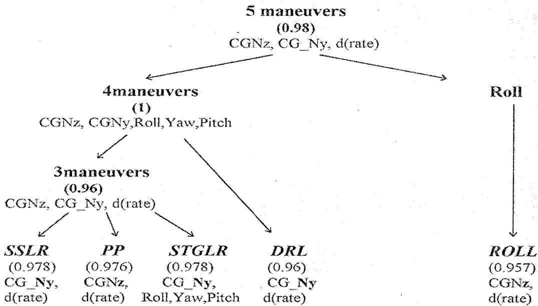
FIGURE 13. CLASSIFICATION ALGORITHM
