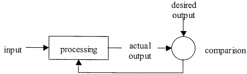
FIGURE 2. SUPERVISED TRAINING
