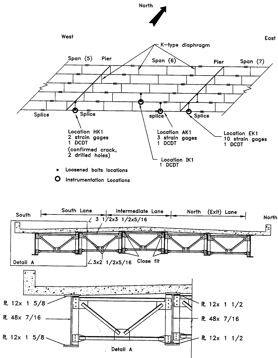
Figure 11. Schematic plan and cross sections of Mosquito Creek Bridge (Bridge K1) showing instrumentation and loosened bolts locations
