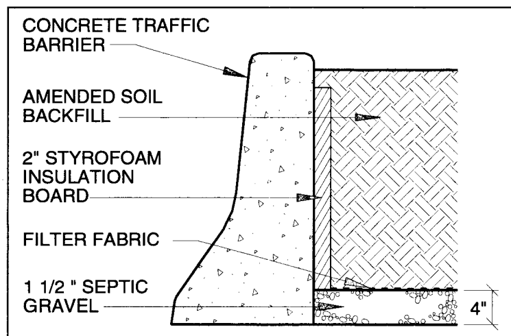
Figure 6. Median planter detail.
