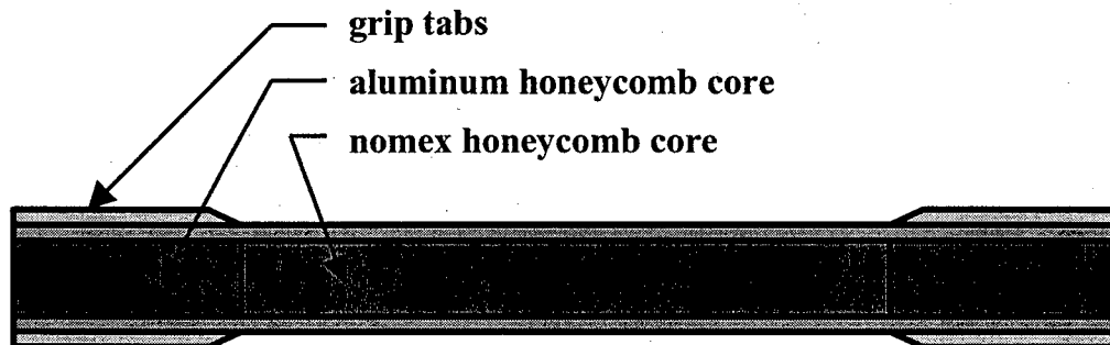
FIGURE 22. GRIPPED SPECIMEN
