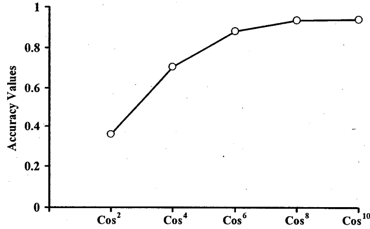
FIGURE 13. EQUATION ACCURACY
