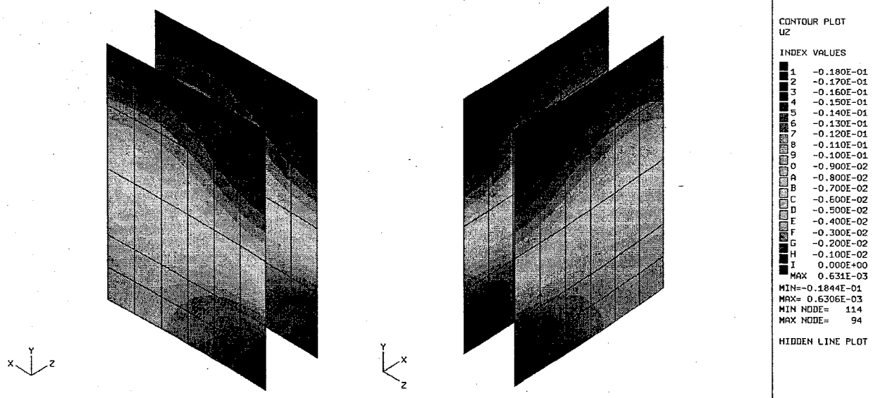
FIGURE 35. OUT-OF-PLANE DISPLACEMENTS OF FRONT AND BACK FACESHEETS (Curved-152, \beta = 10\% )
