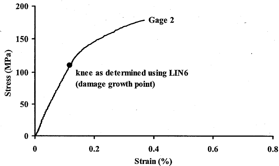
FIGURE 27. DAMAGE GROWTH—TYPICAL GAGE-2 DATA
