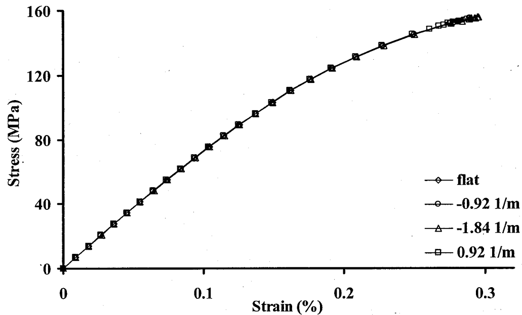
FIGURE 46. MODEL CURVATURE EFFECTS ON DAMAGE GROWTH
