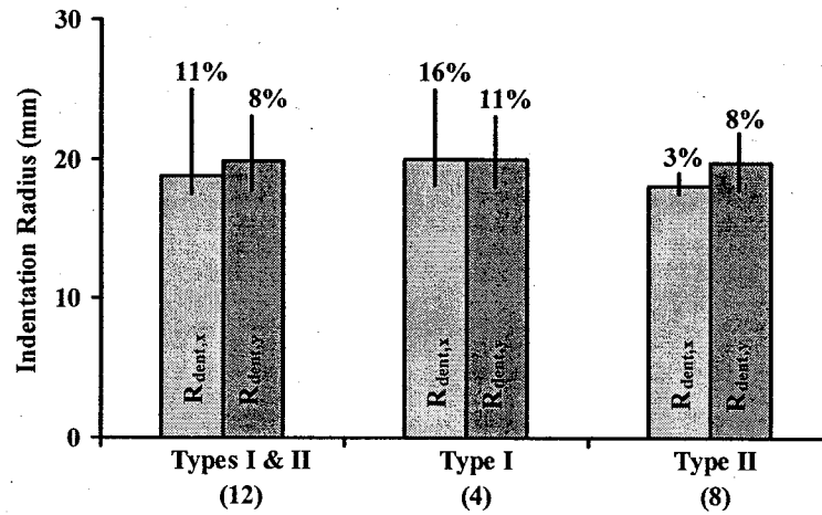
FIGURE 14. SIZE OF INDENTATION REGION
