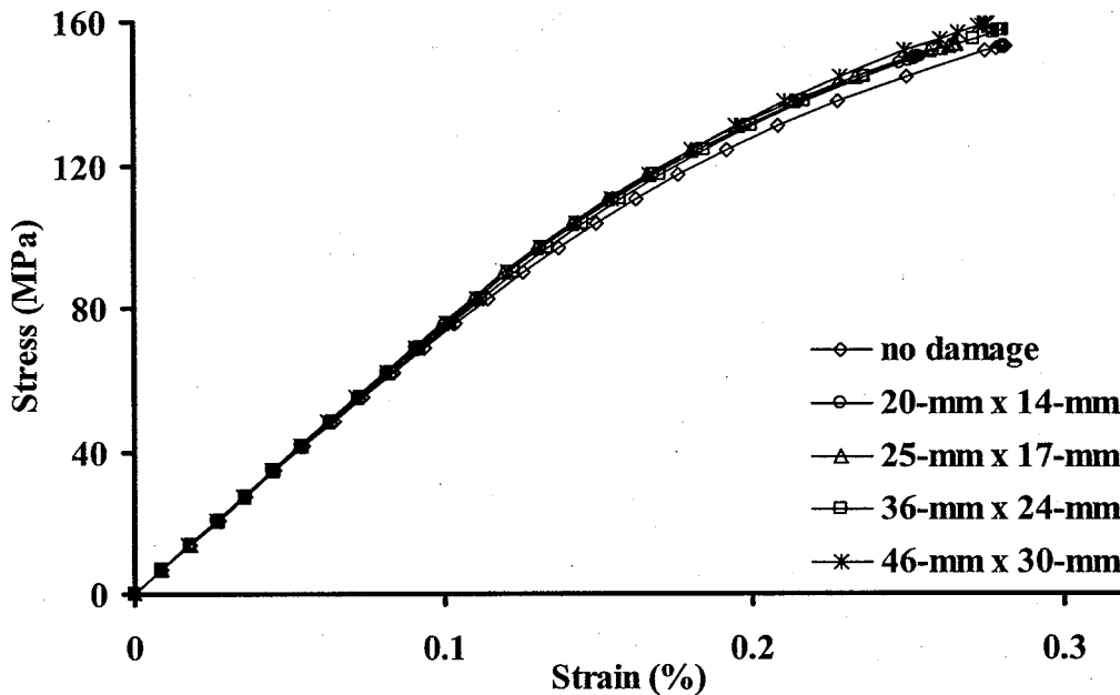
FIGURE 47. MODEL MEMBRANE DAMAGE SIZE EFFECTS ON DAMAGE GROWTH
