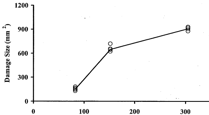
FIGURE 6. DAMAGE SIZE VS PANEL WIDTH
