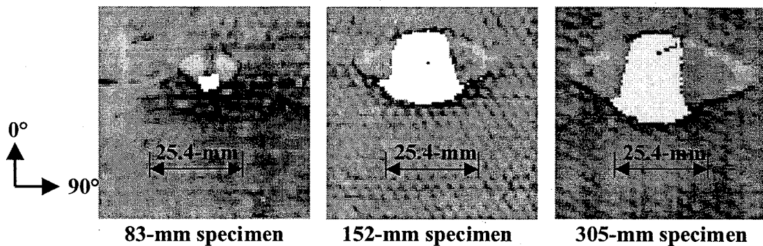
FIGURE 5. ULTRASONIC SCAN OF IMPACT DAMAGE (3 widths)
