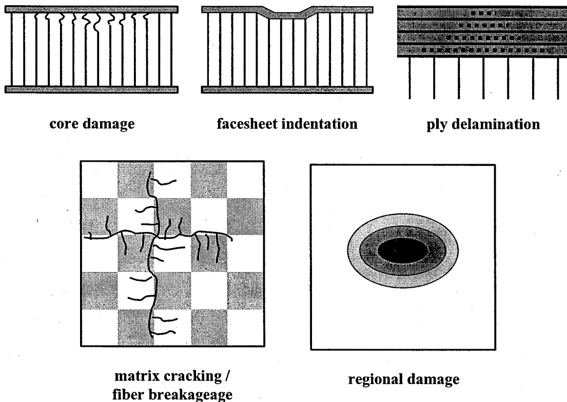
FIGURE 4. FORMS OF IMPACT DAMAGE
