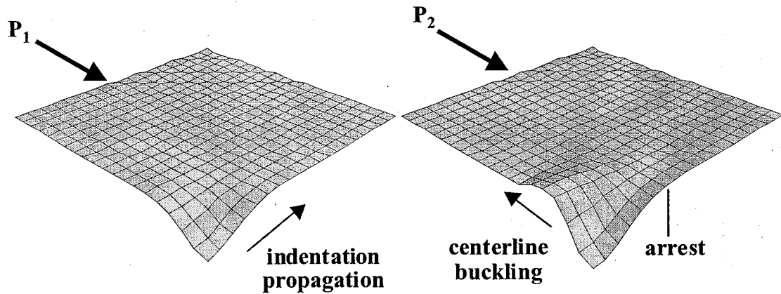
FIGURE 49. DAMAGE ARREST MECHANISM ( P_1 < P_2 )
