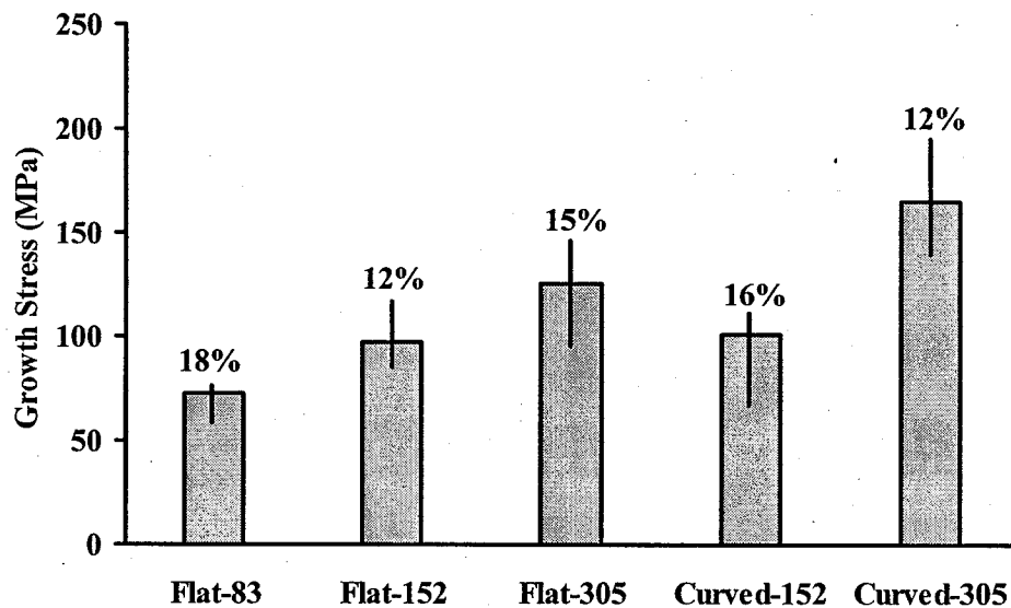
FIGURE 28. DAMAGE GROWTH STRESS
