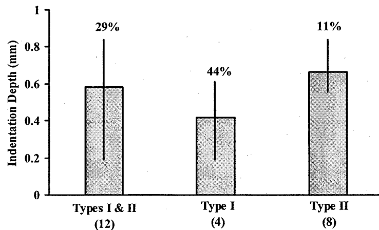
FIGURE 9. MAXIMUM RESIDUAL INDENTATION DEPTH
