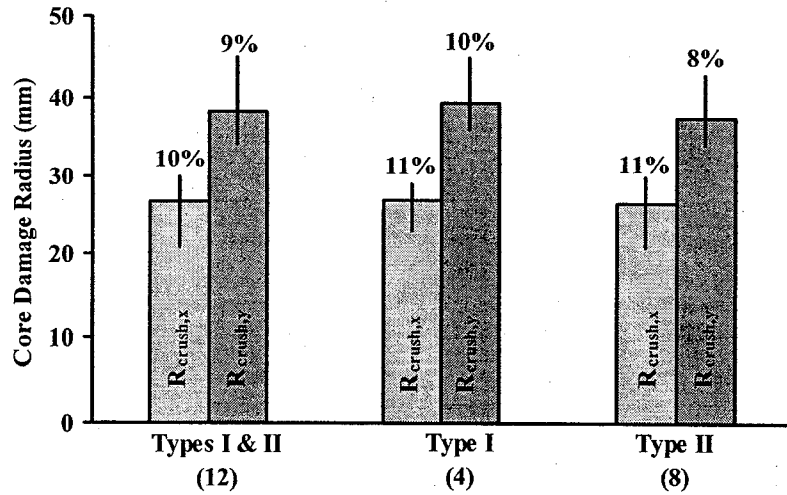
FIGURE 16. SIZE OF CORE DAMAGE REGION
