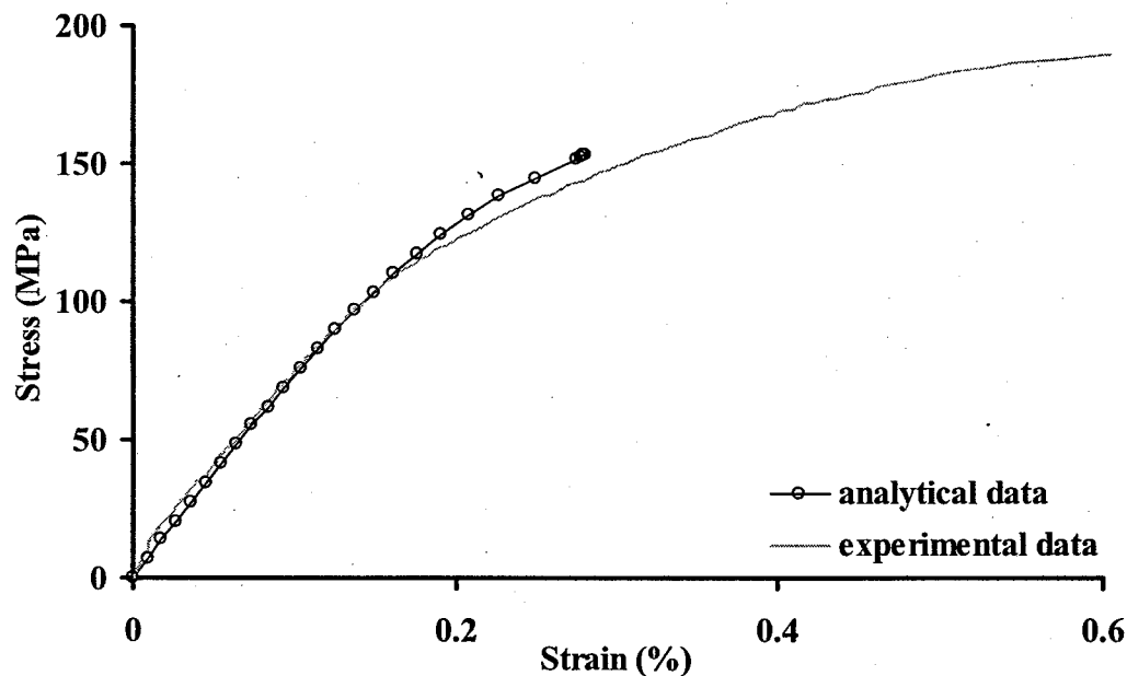
FIGURE 44. ANALYTICAL VS EXPERIMENTAL RESULTS
