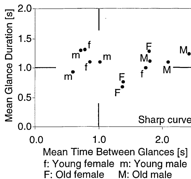
Figure 14. Glance allocation for sharp curve
