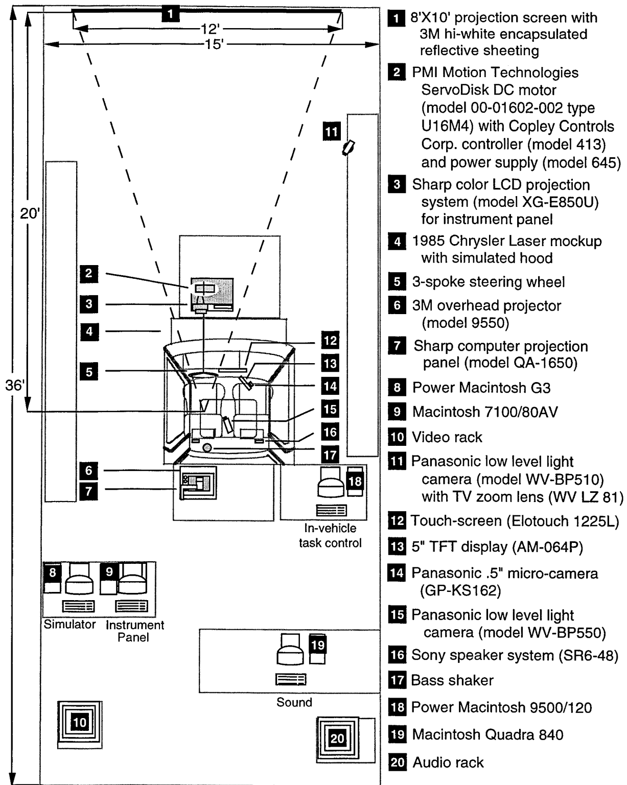
Figure 2. Plan view of UMTRI's Driver Interface Research Simulator
