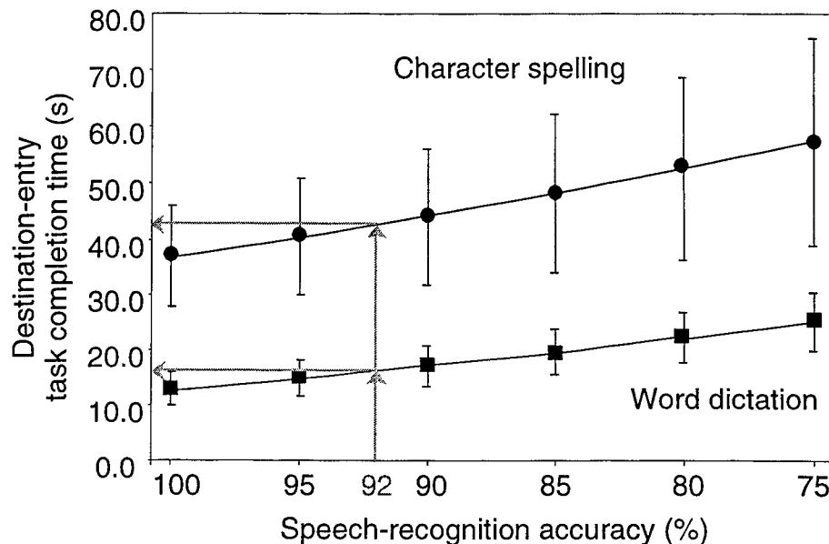
Figure 49. Task completion time as a function of speech-recognition accuracy
