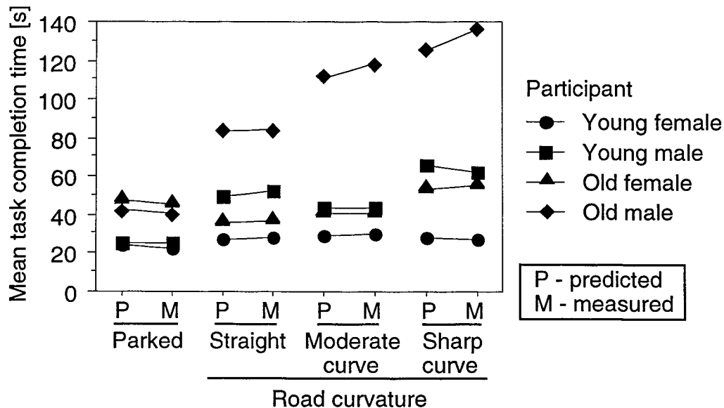
Figure 46. The effect of driving conditions on keyboard-entry task completion time
