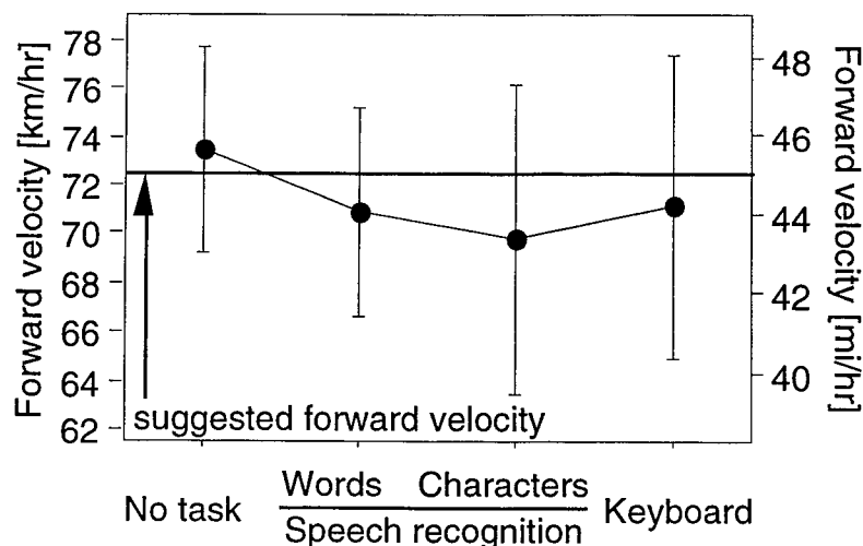
Figure 24. The effect of entry method on mean forward velocity
