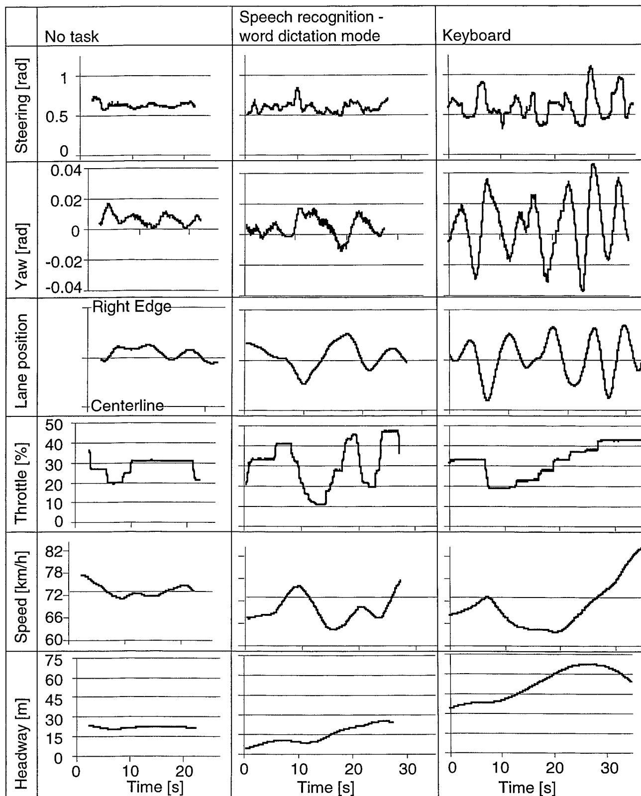
Figure 18. Typical driving performance for a destination entry trial
