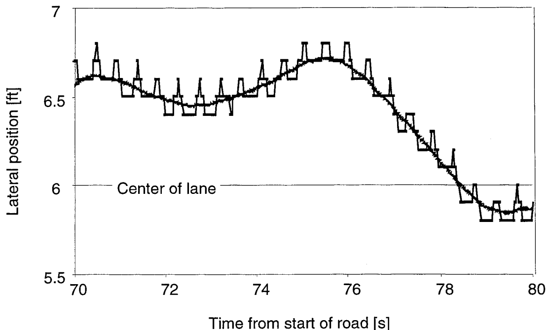
Figure 54. Recorded lateral position for a sample of a curve
