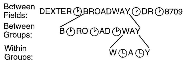
Figure 16. Breakdown of character entry measures
