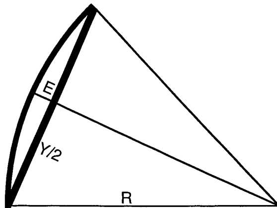
Figure 55. A lateral error ( E ) is caused by the segmentation of the curve
