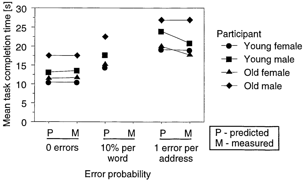
Figure 44. The effect of number of errors on task completion time
