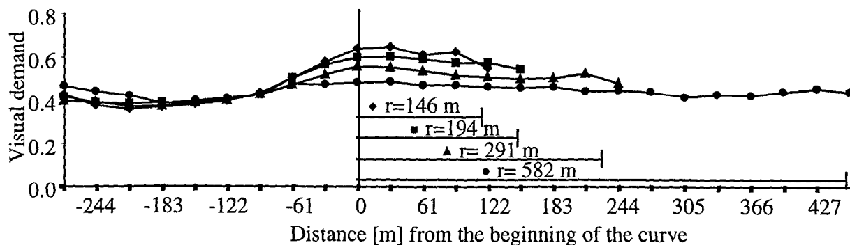
Figure 33. Visual demand for curves of different radii
