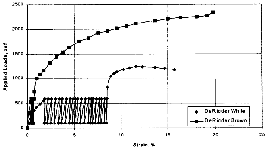
Stress-Strain for Cyclic Triaxial Tests with DeRidder Soils
