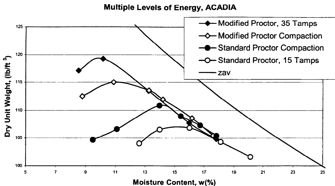
Figure 9 Acadia's family of curves for different compaction efforts
