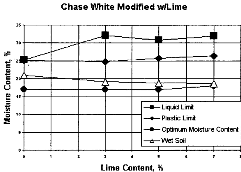
Figure 26 Variation of plasticity, OMC, and moisture with lime content
