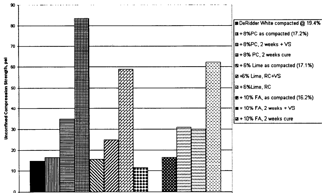
DeRidder White Modification/Stabilization Performance
