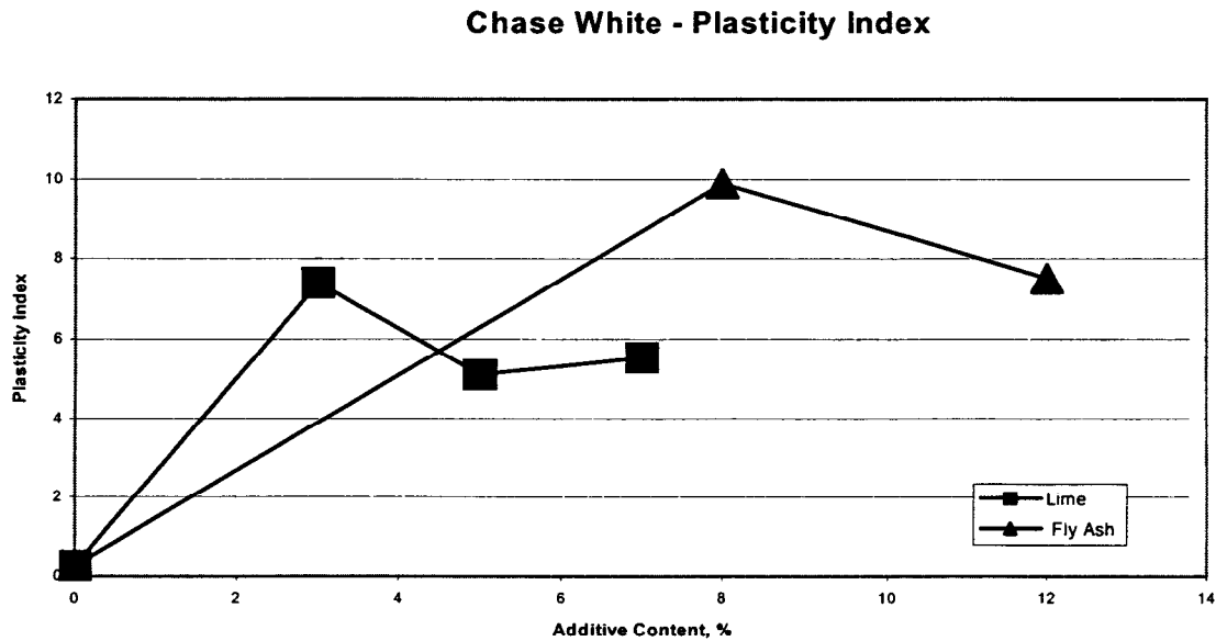
Figure 28 Plasticity Index vs Percent Additive
