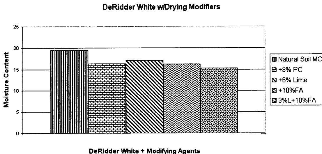
Figure 25 Additives drying ability with DeRidder White Soil
