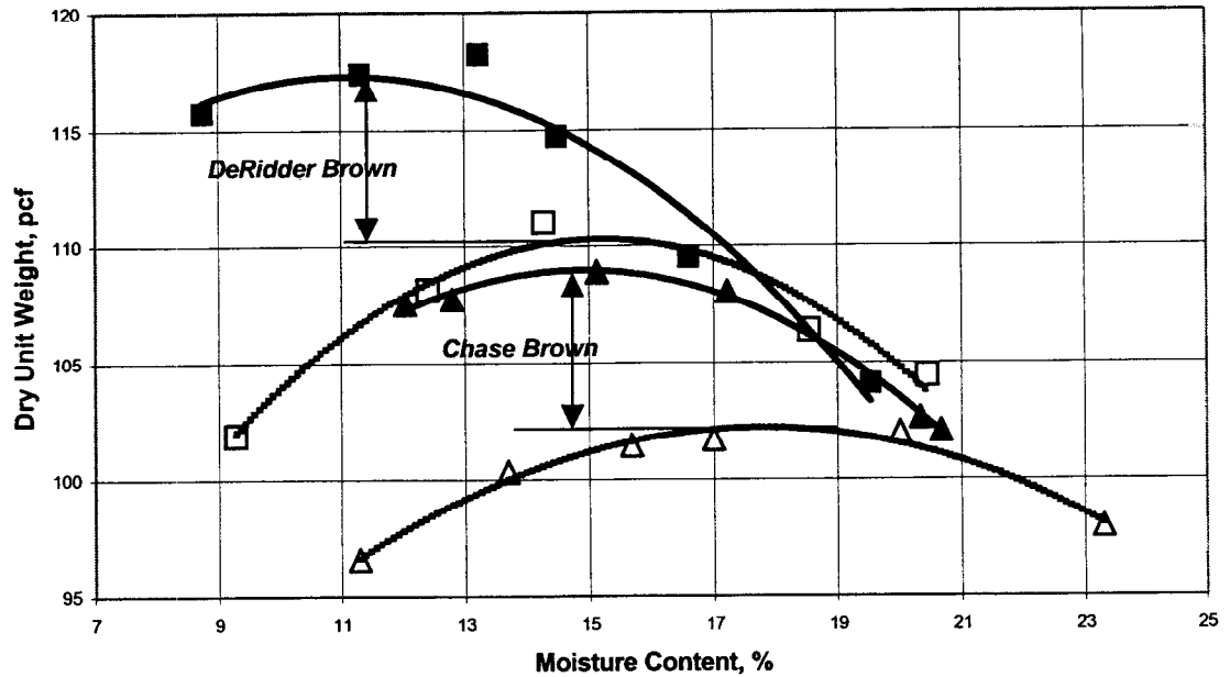
Figure 8 Influence of the compaction effort for soils with higher plasticity
