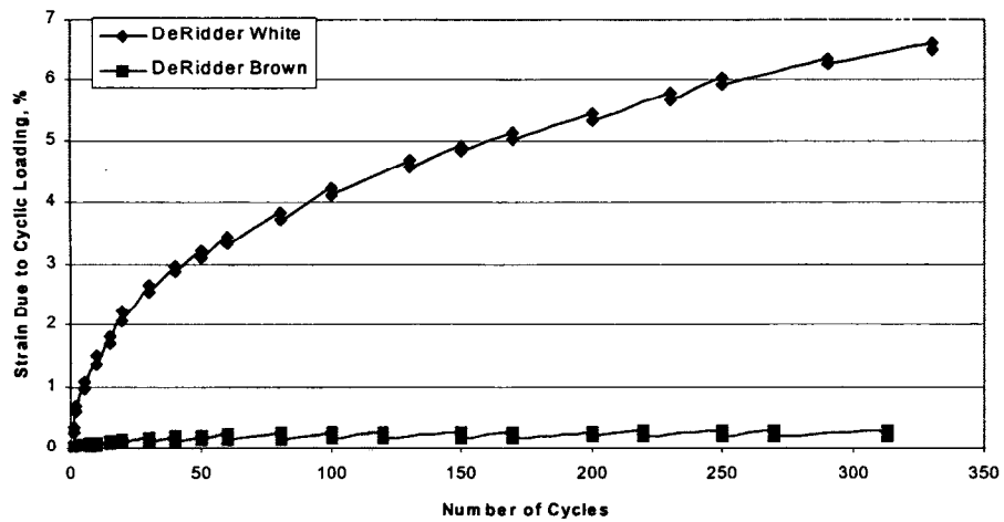
Cyclic Triaxial Tests for DeRidder Soil Samples
