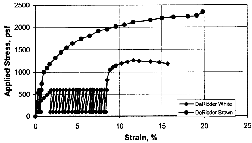
Stress-Strain for CycLic Triaxial Tests with DeRidder Soils
