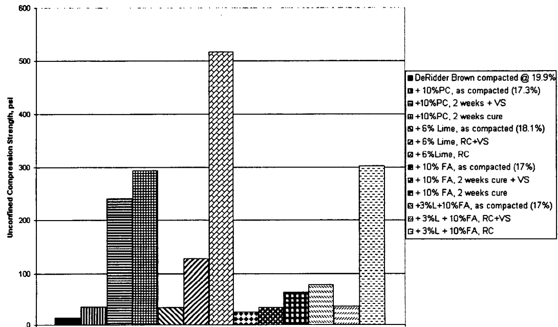
DeRidder Brown: Modification/Stabilization Performance
