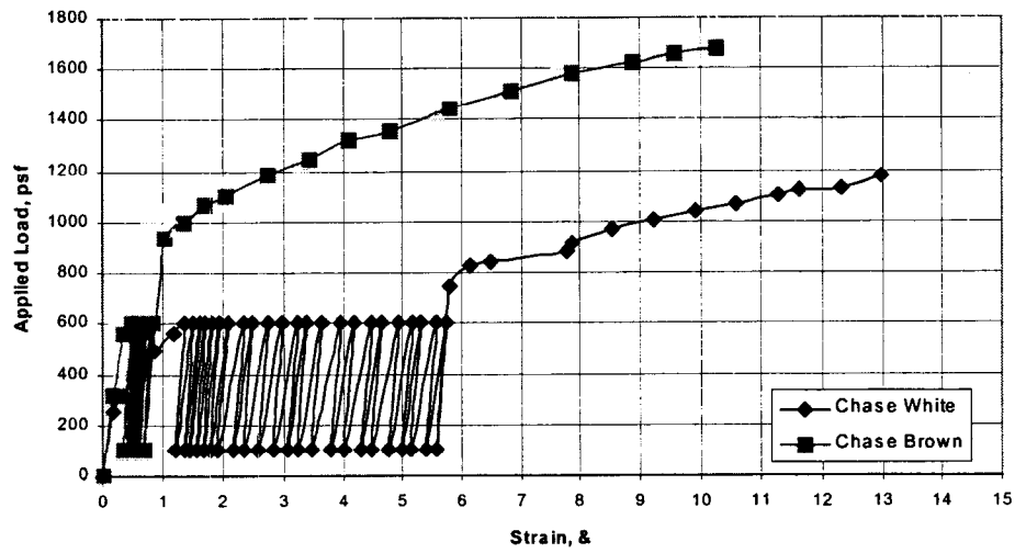
Chase Brown and White Cyclic Triaxial Tests
