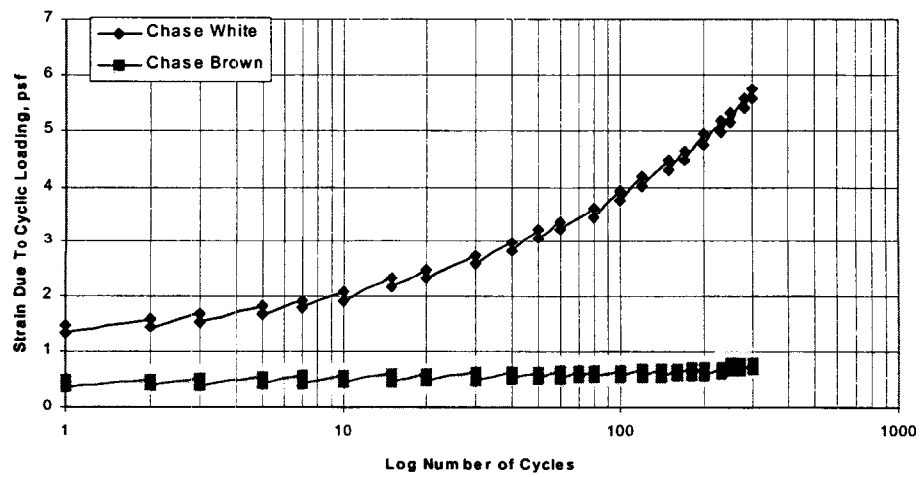
Chase Brown & White Cyclic Triaxial Tests
