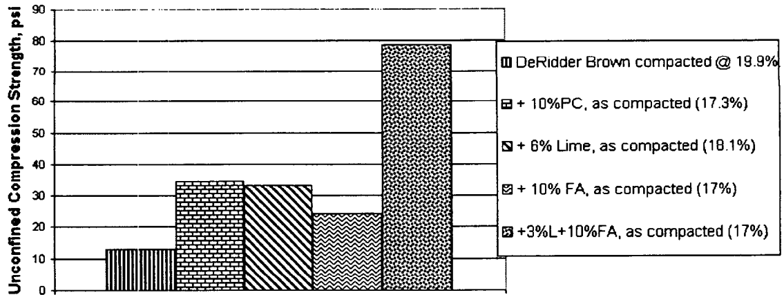
DeRidder Brown: Modification/Stabilization Performance
