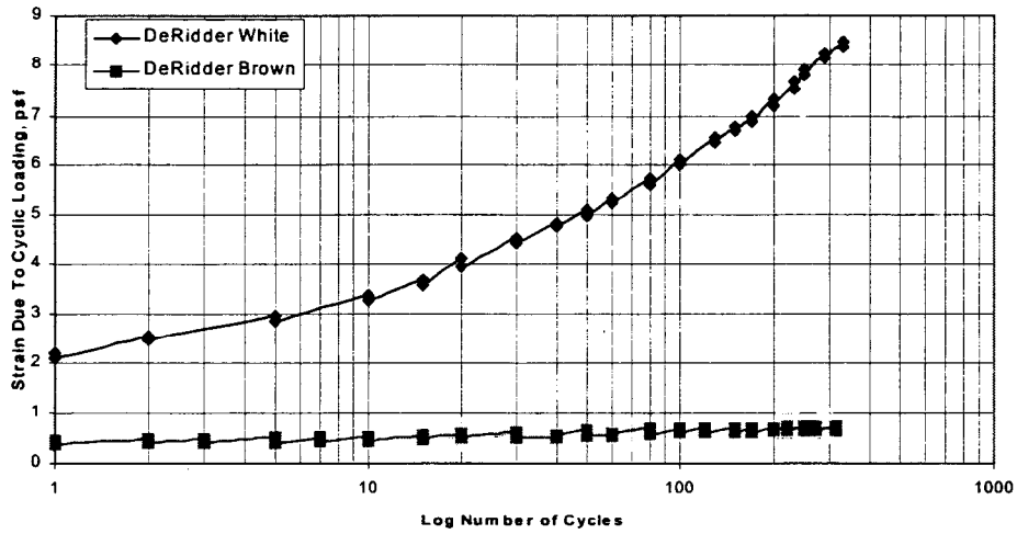
DeRidder White/Brown Cyclic Triaxial Tests
