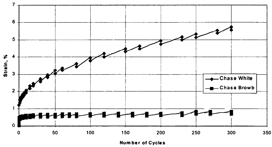
Chase White Triaxial Tests
