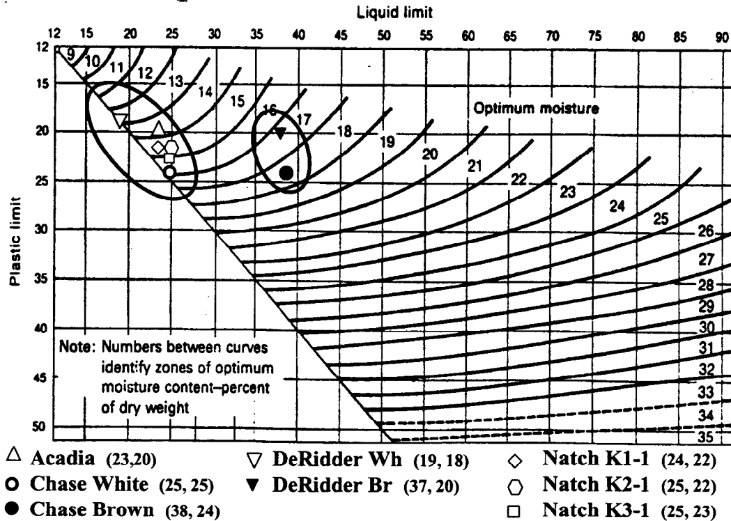
Figure 11 Optimum moisture content estimates by Johnson and Sallberg (1962)
