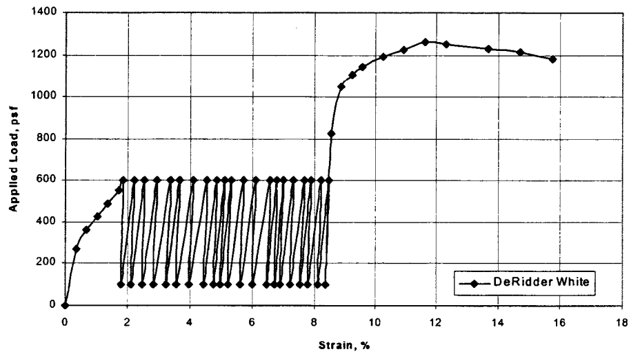
DeRidder White Cyclic Triaxial Test
