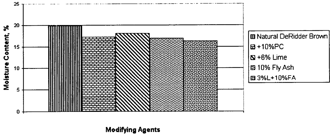
DeRidder Brown Drying Modifiers
