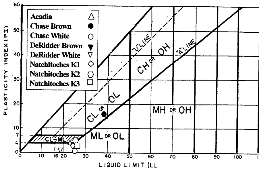
Figure 3 Plasticity Chart w/ Unified Classification of Soil Samples
