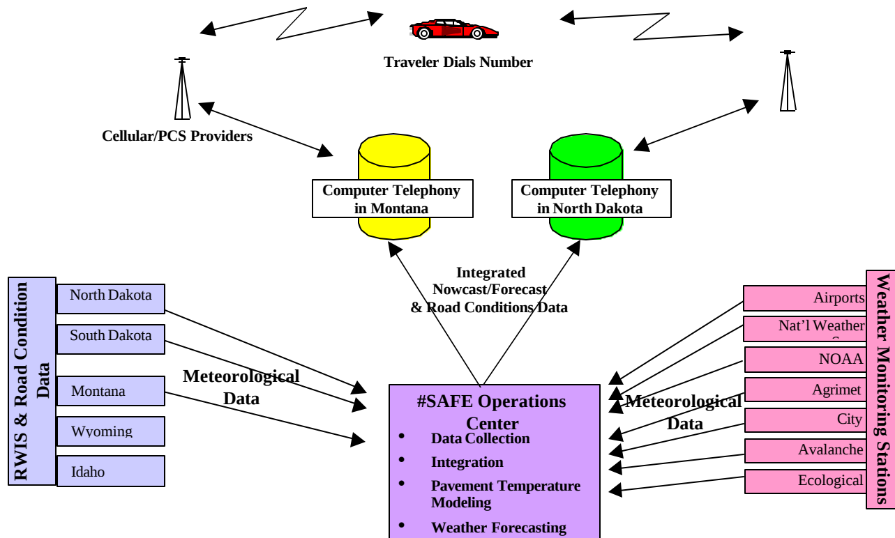
Figure 2. #SAFE System
