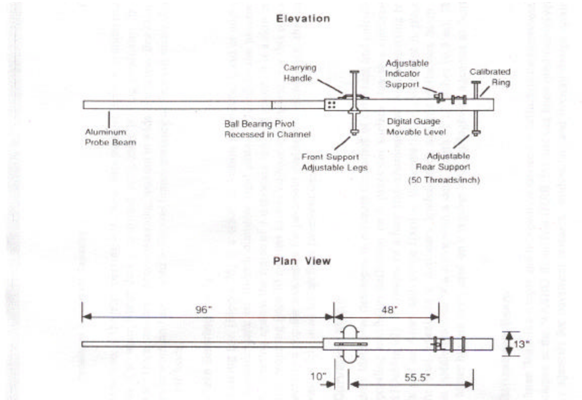
Fig. 21. Benkelman beam apparatus (Haas, Hudson, and Zaneiwski, 1994)
