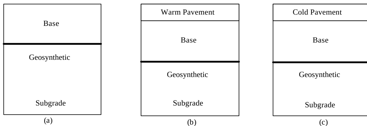
Fig. 9. Typical road cross-sections (a) Unsurfaced, (b) Warm pavement, (c) Cold pavement
