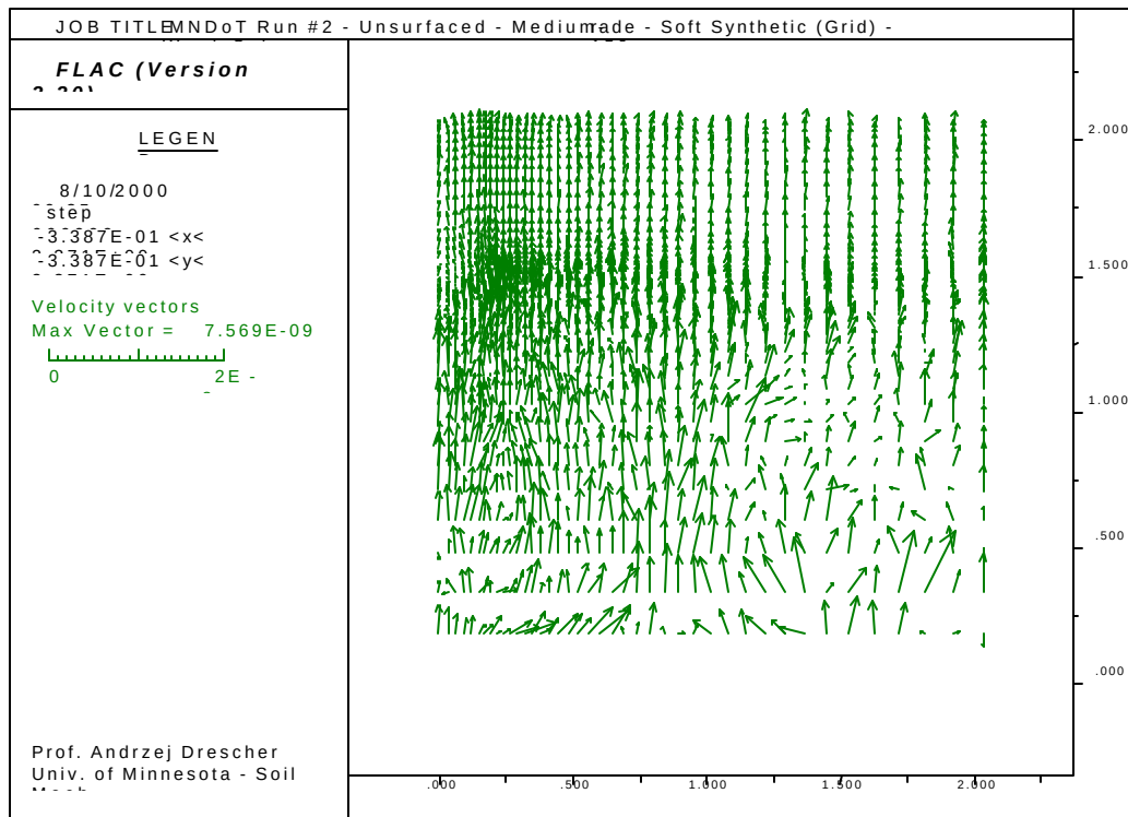
Fig. 17. Velocity profile for gravitational stress field with large interface shear stiffness
