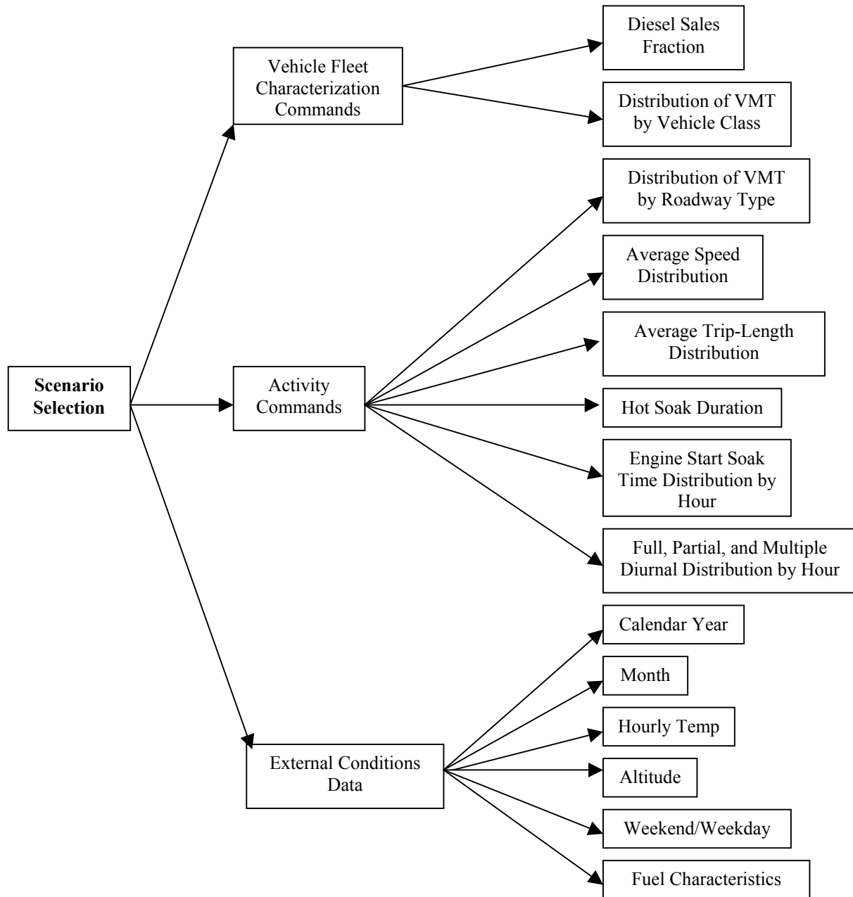
Figure 2. Scenario Selection
