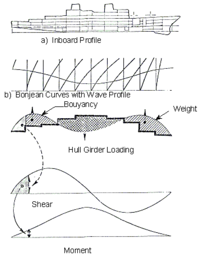
Figure 21: A representation of Buoyancy, Bending Moment and Shear.
