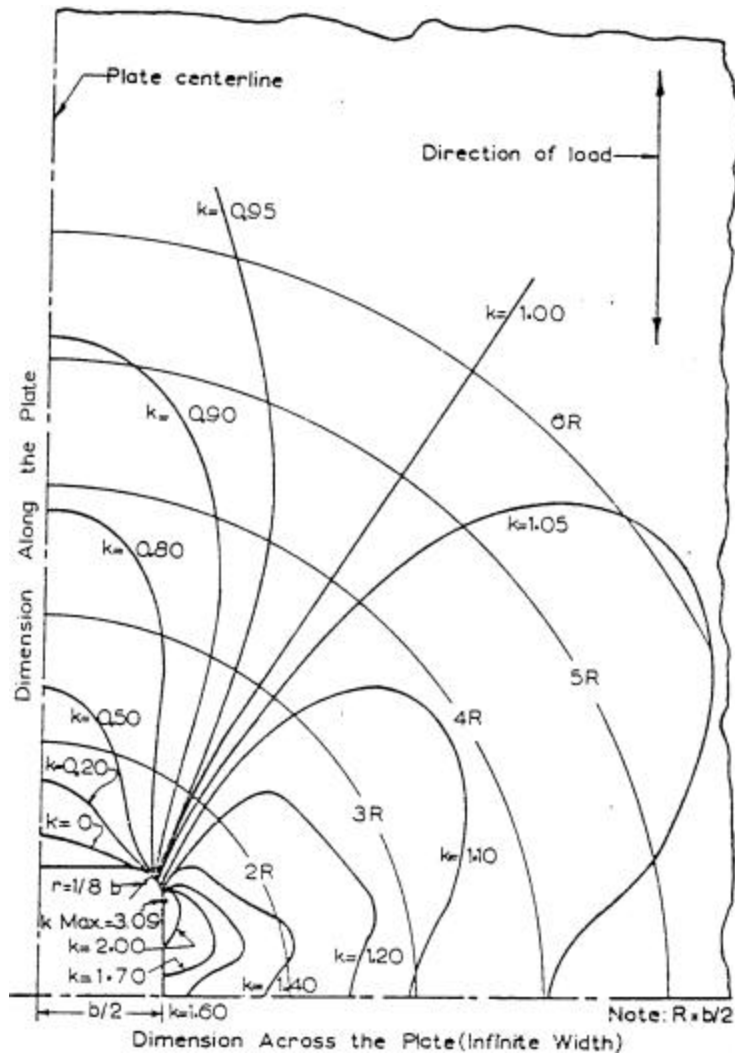
Figure 12: Stress Concentration Factor for a Square Hole in an Infinite Plate.
