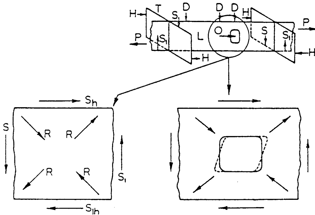
Figure 20: Shear Force Distribution in a Penetrated Longitudinal Bulkhead.
