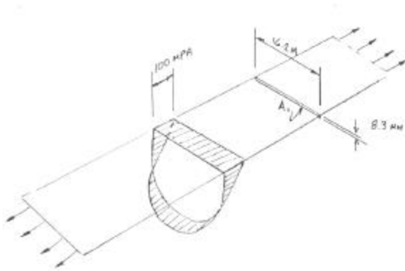
Figure 24: Bending Moment and Stress Distributions.
