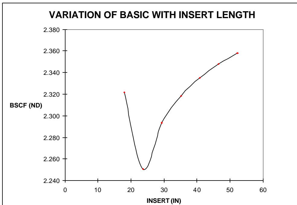
Figure 40: Variation of SCF with Corner Insert Length.
