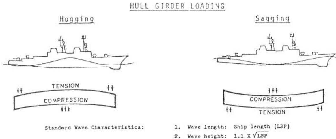
Figure 1: Vessel in Hogging and Sagging Conditions.
