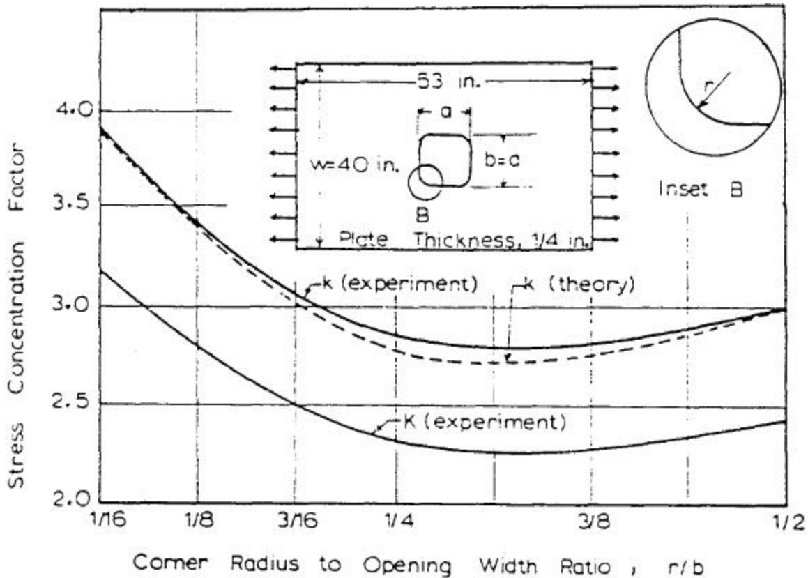
Figure 13: Variation of Stress Concentration Factor with Corner Radius Size.
