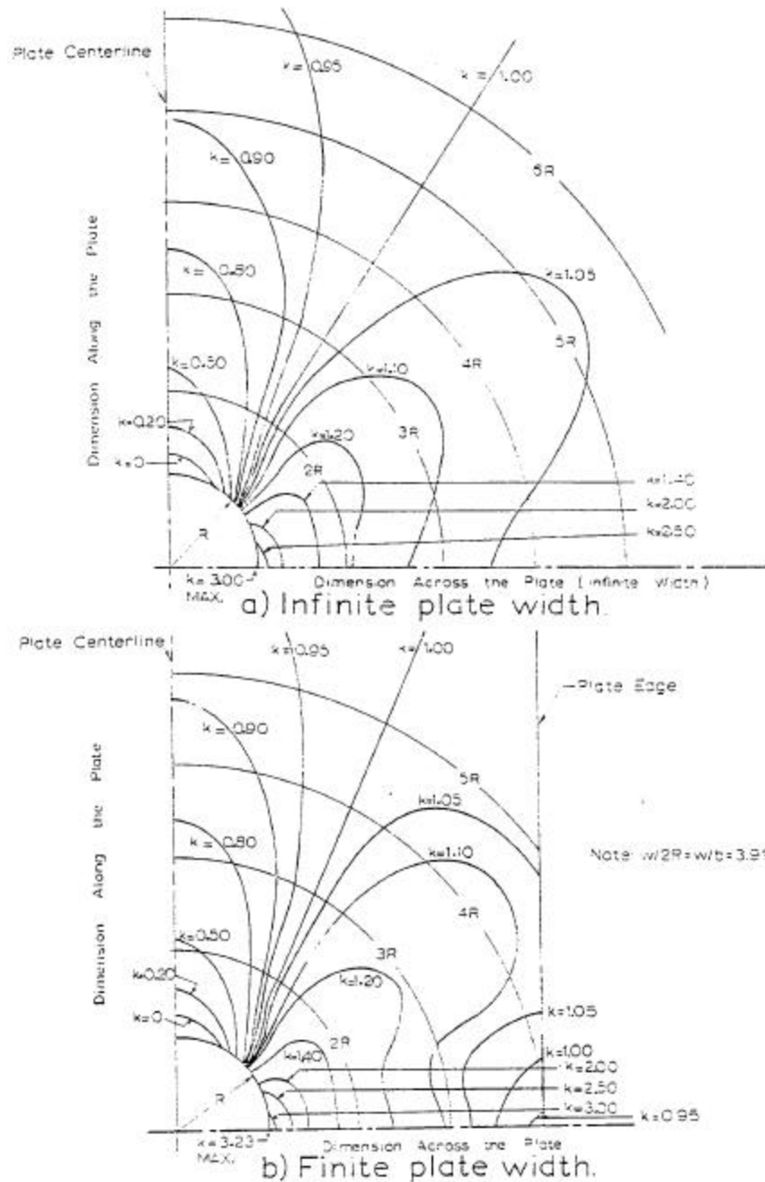
Figure 9: Local Stress Concentration around a Circular Hole in Plates.
