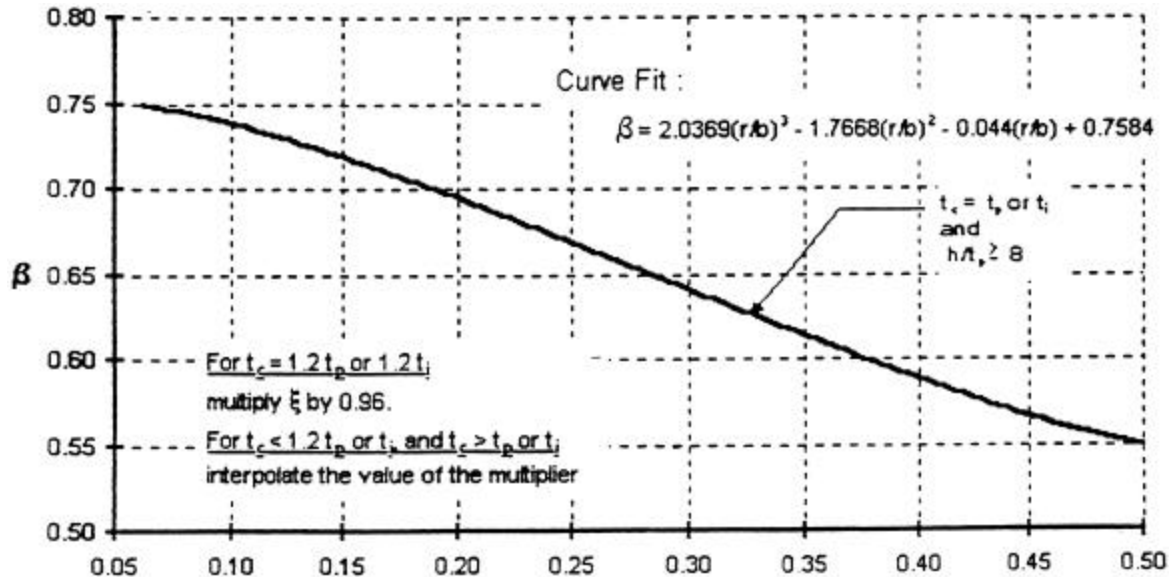
Figure 34: Coaming Factor to Help Determine Reduction in K.
