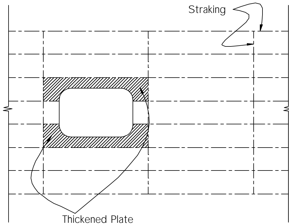
Figure 29: Compensation Plate Thickening and Plate Straking.
