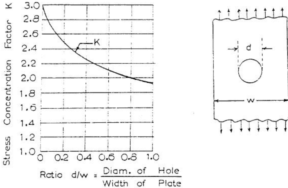
Figure 11: Stress Concentration Factor for Holes of Significant Size.
