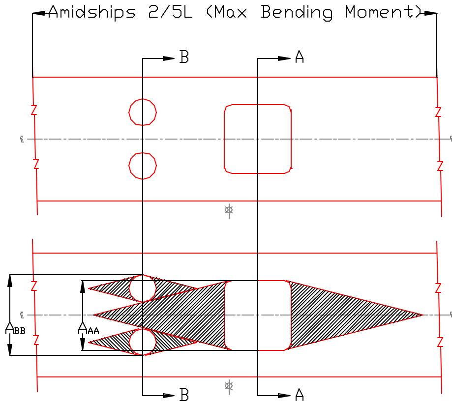
Figure 17: Ineffective Areas from Openings in Strength Deck.
