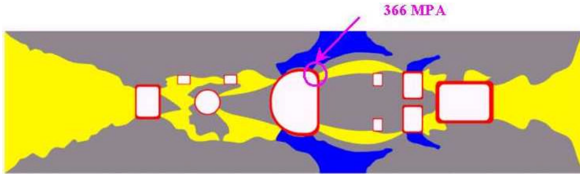
Figure 22: A Representation of Stress Fields.
