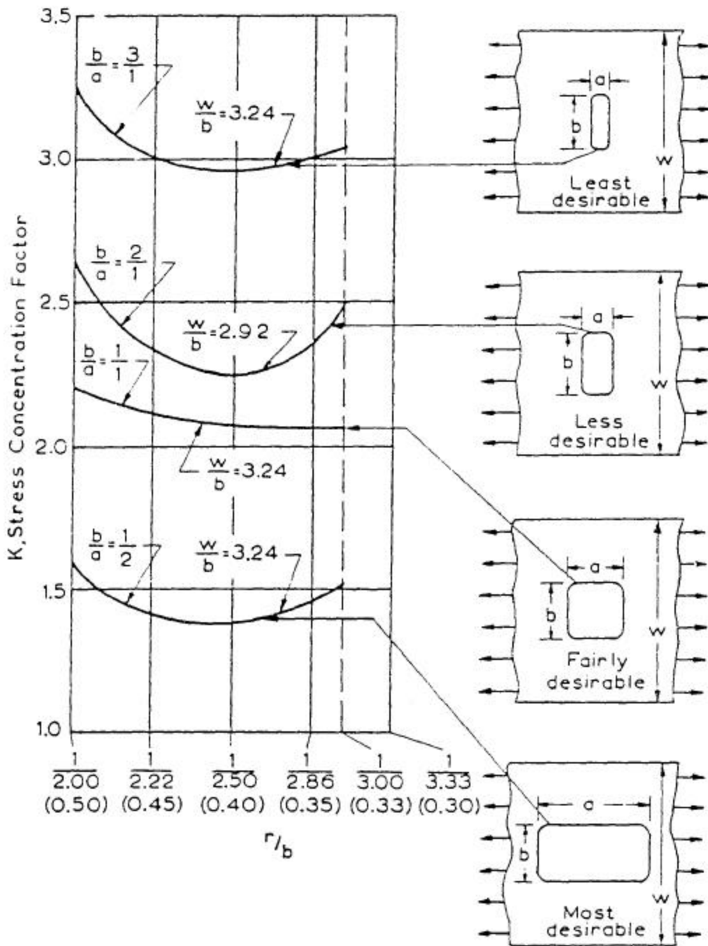
Figure 14: Effect of b/a Ratio on Stress Concentration Factor (K).
