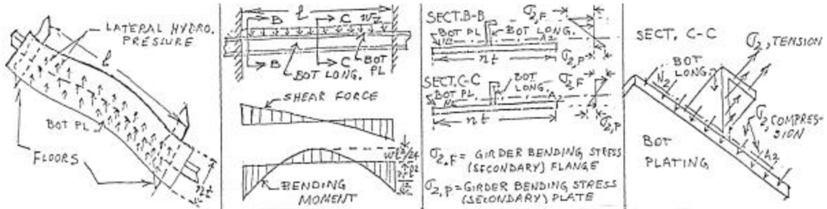
Figure 4: Secondary Stresses Induced by Local Pressure.
