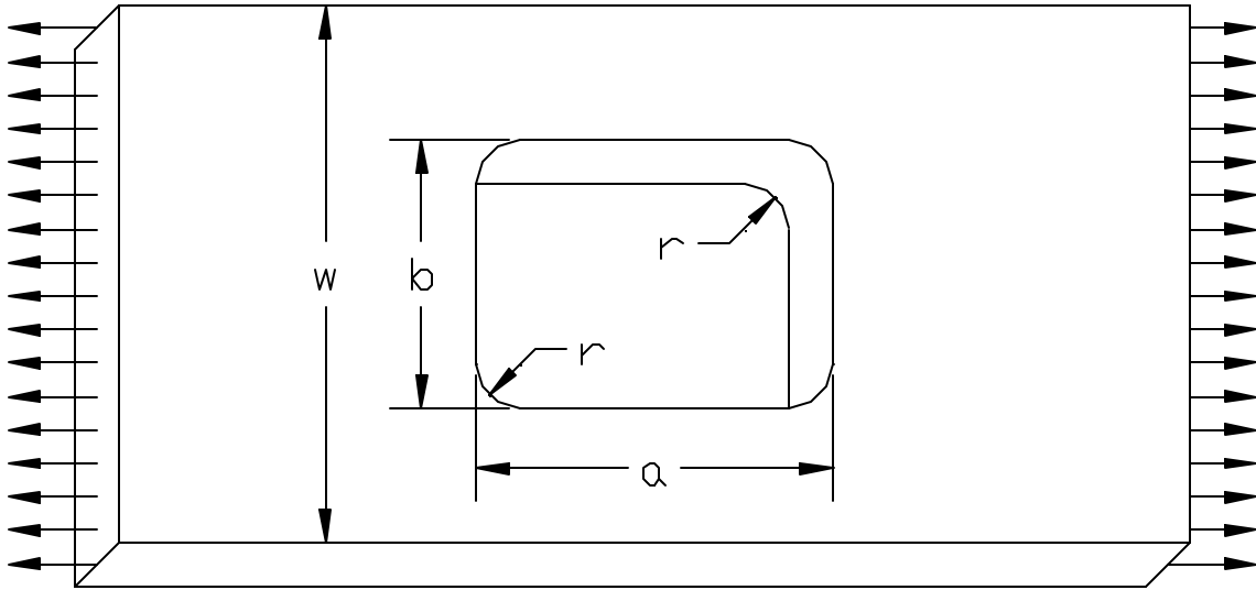
Figure 8: Parameterized opening in a uniformly loaded plate in tension.
