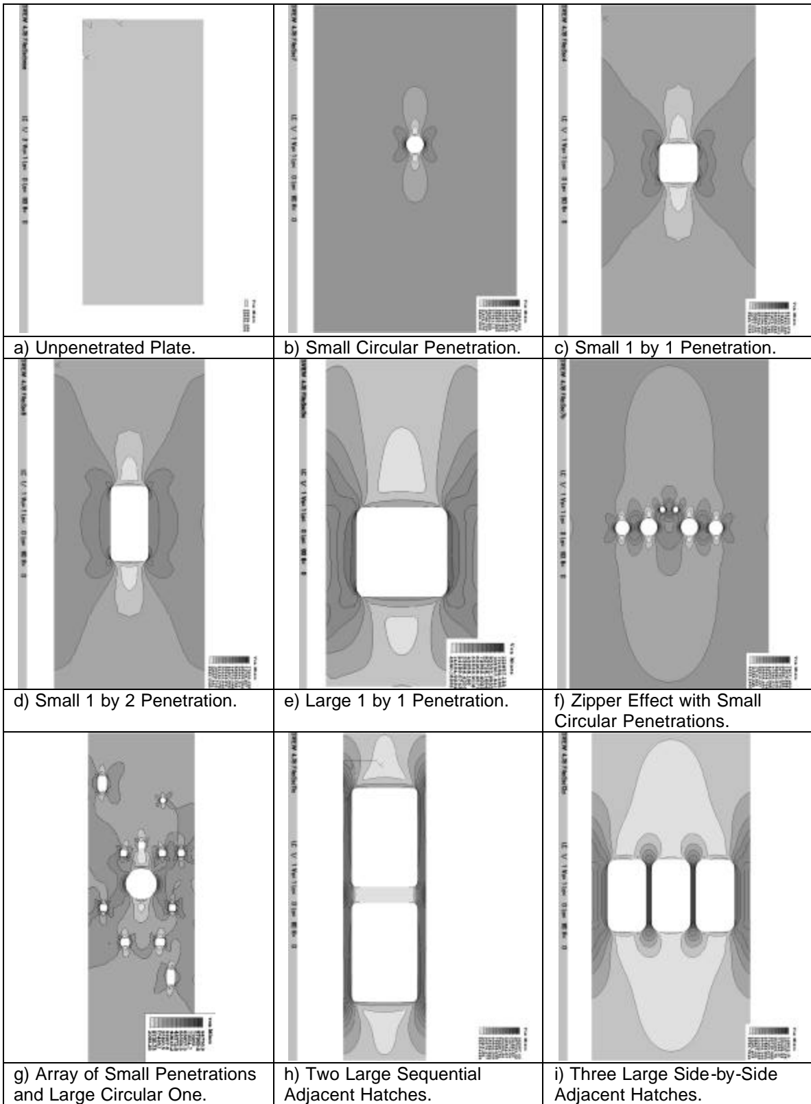
Figure 27: Some representative Finite Element Models.
