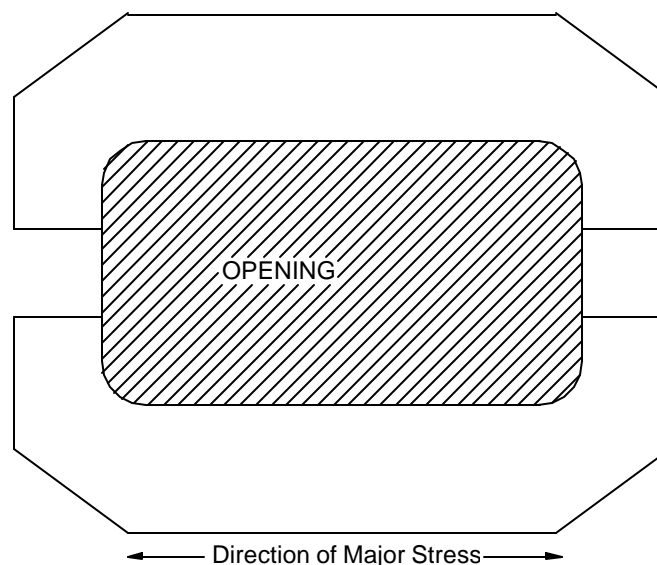
Figure 28: Typical Compensating Insert of a Larger Hole.
