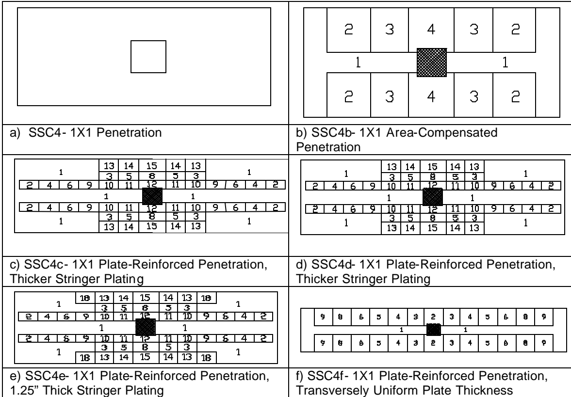
Figure 36: Illustrations of Compensation for a 1 by 1 Deck Penetration.
