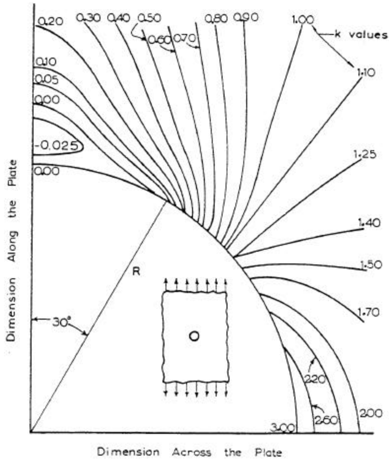
Figure 10: Local Stress Concentration for a Circular Hole in an Infinite Plate.
