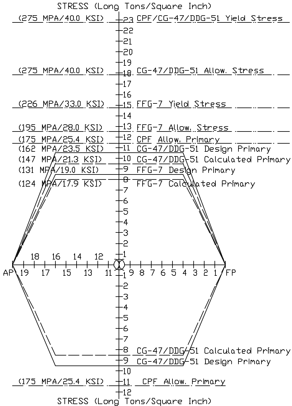
Figure 6: Ship Primary Hull Structural Envelope and Strength Criterion.
