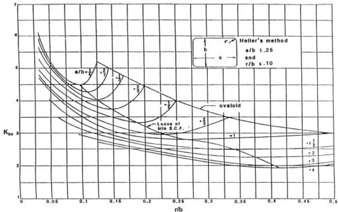
Figure 15: Far-Field SCF for Rectangular Openings.
