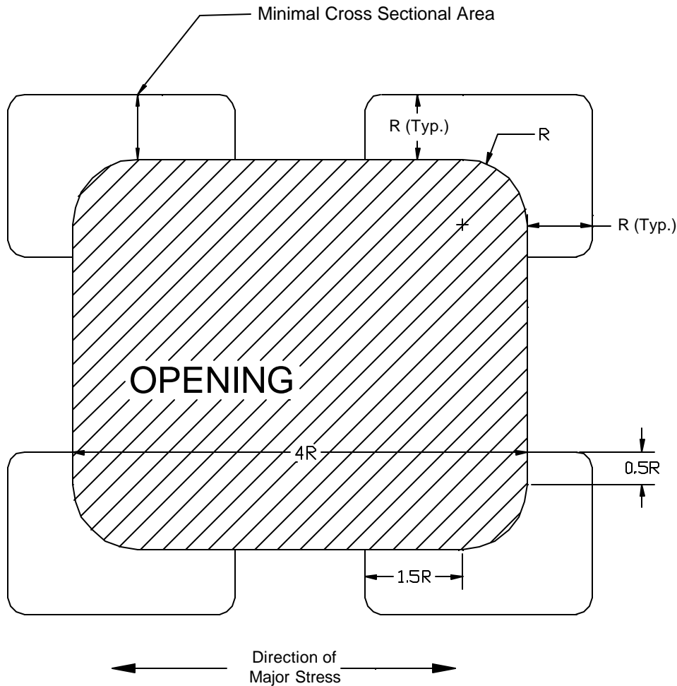
Figure 30: A Large Opening that has been Reinforced at the Corners.
