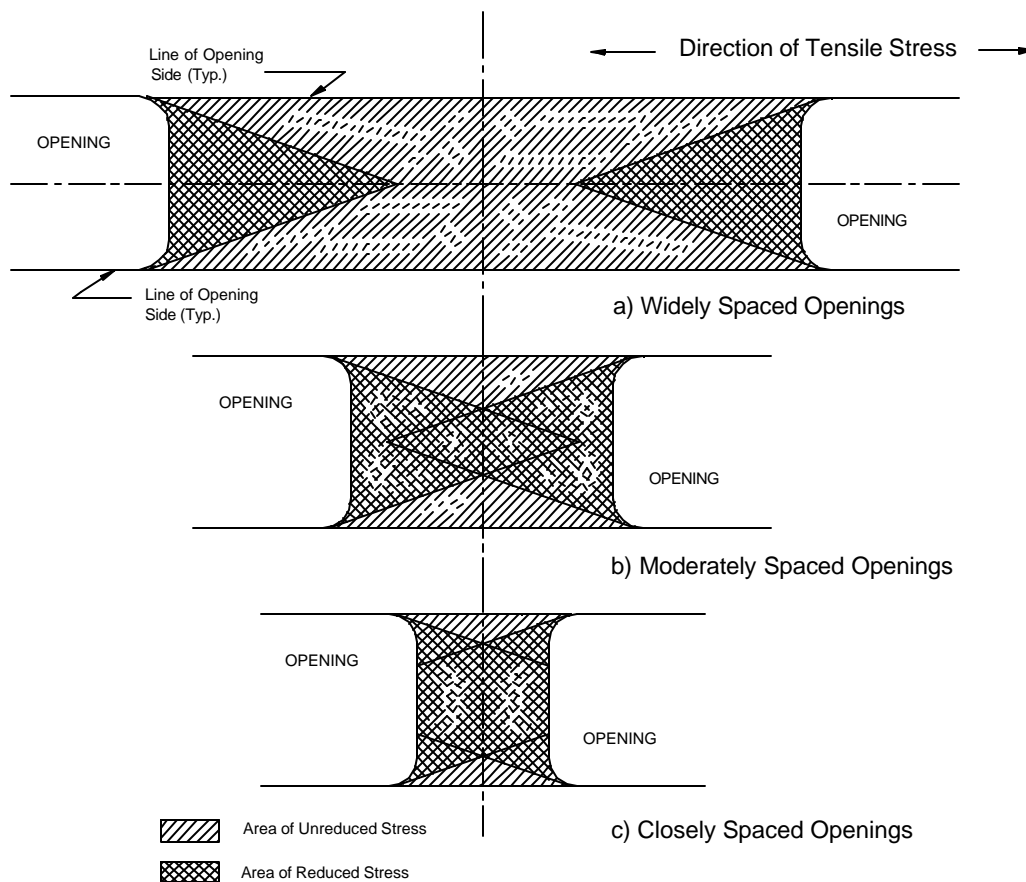
Figure 18: Multiple Rectangular Openings in Primary Structure.
