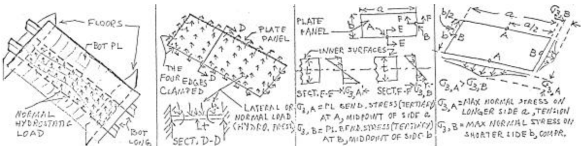
Figure 5: Tertiary Stress Induced by Local Pressure on Plate.
