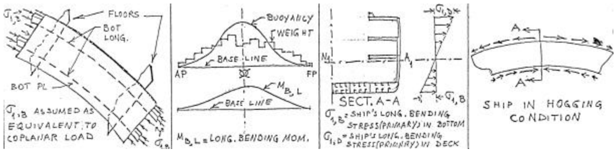
Figure 2: Primary Stresses Induced by Global Bending Moments.
