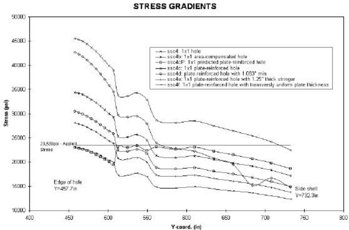
Figure 38: Stress Levels Outboard for Compensation Variations of a 1 by 1.
