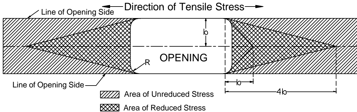
Figure 16: Rectangular Opening in Primary Structure.
