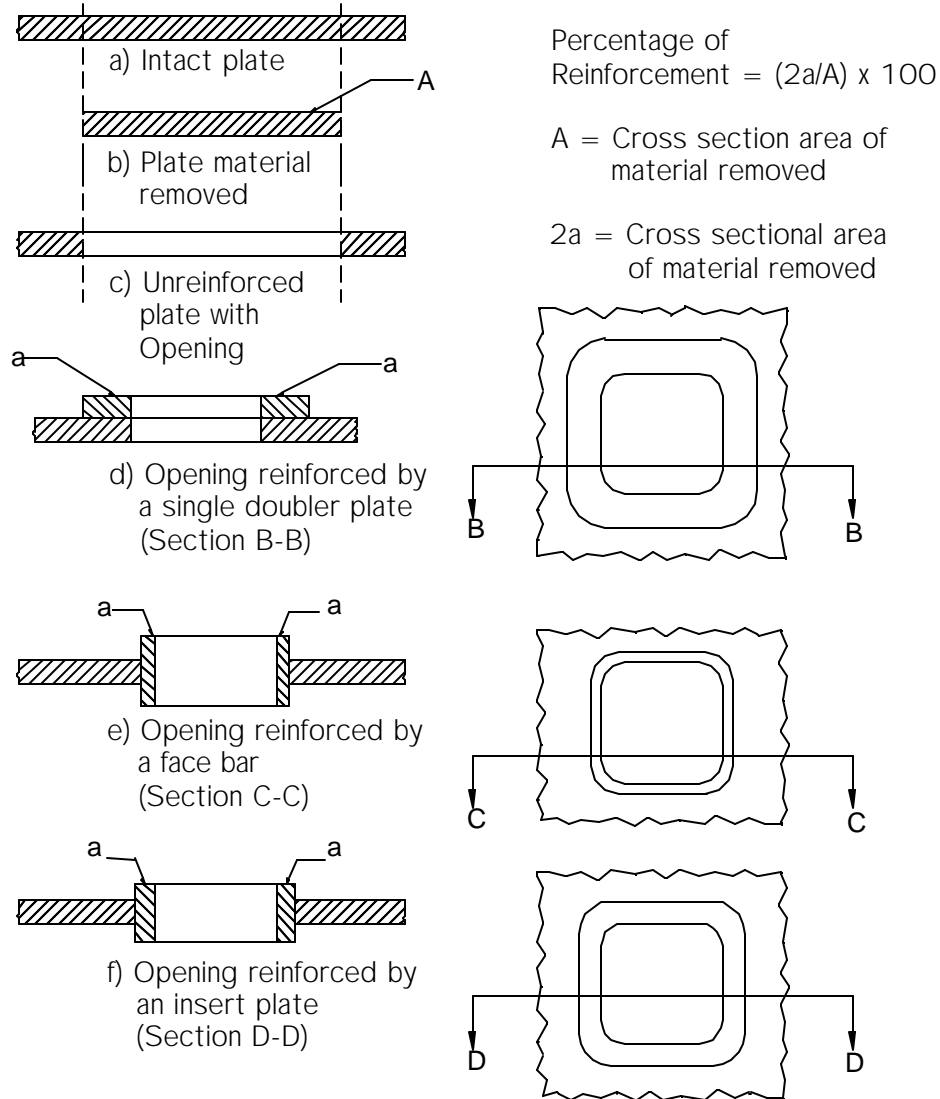
Figure 31: Typical Types of Reinforcements.
