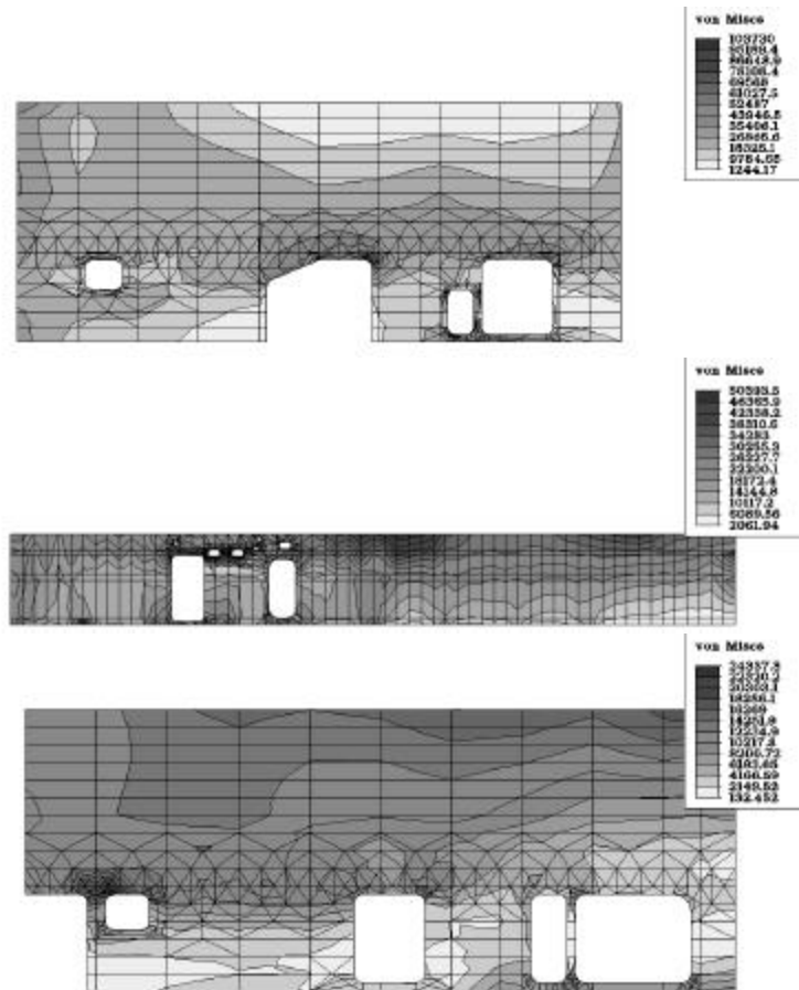
Figure 26: Stress Fields in Deck 1, Longitudinal Bulkhead, and Deck 2.
