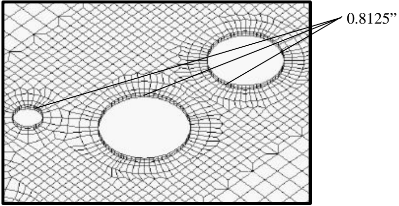
CASE 5: Small Round Central Hole and Zipper Effect
