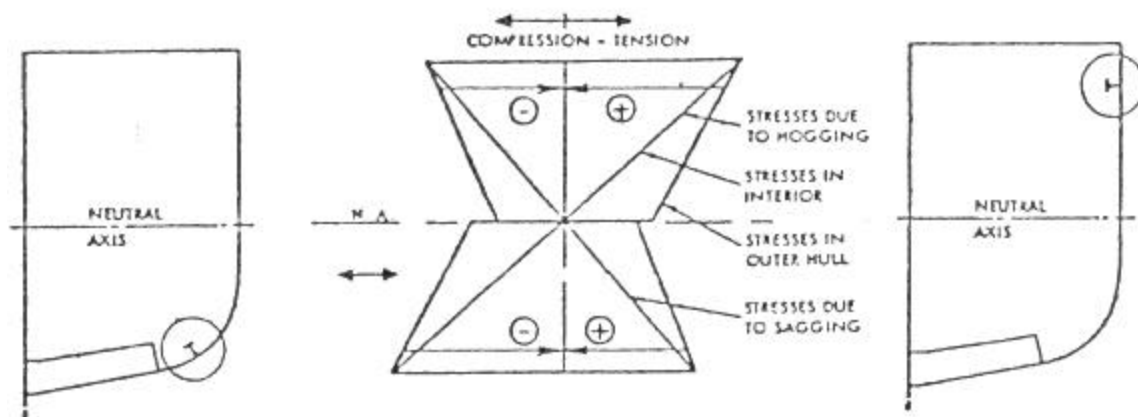
Figure 3: Design Stress Distribution through the Hull cross-section.
