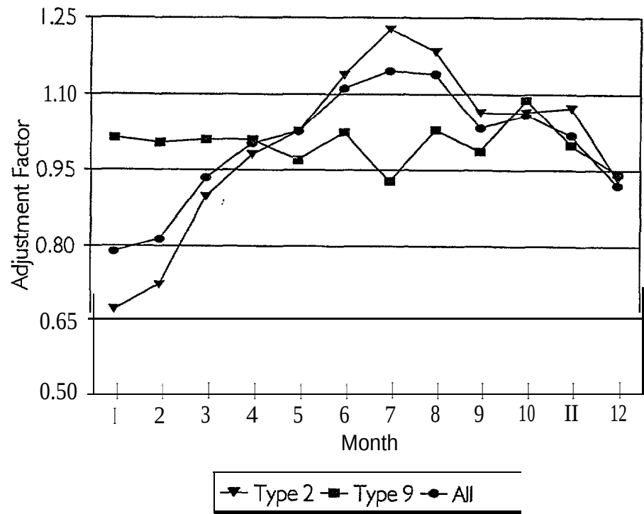
Figure 1. Monthly variation for rural interstate and parkways
