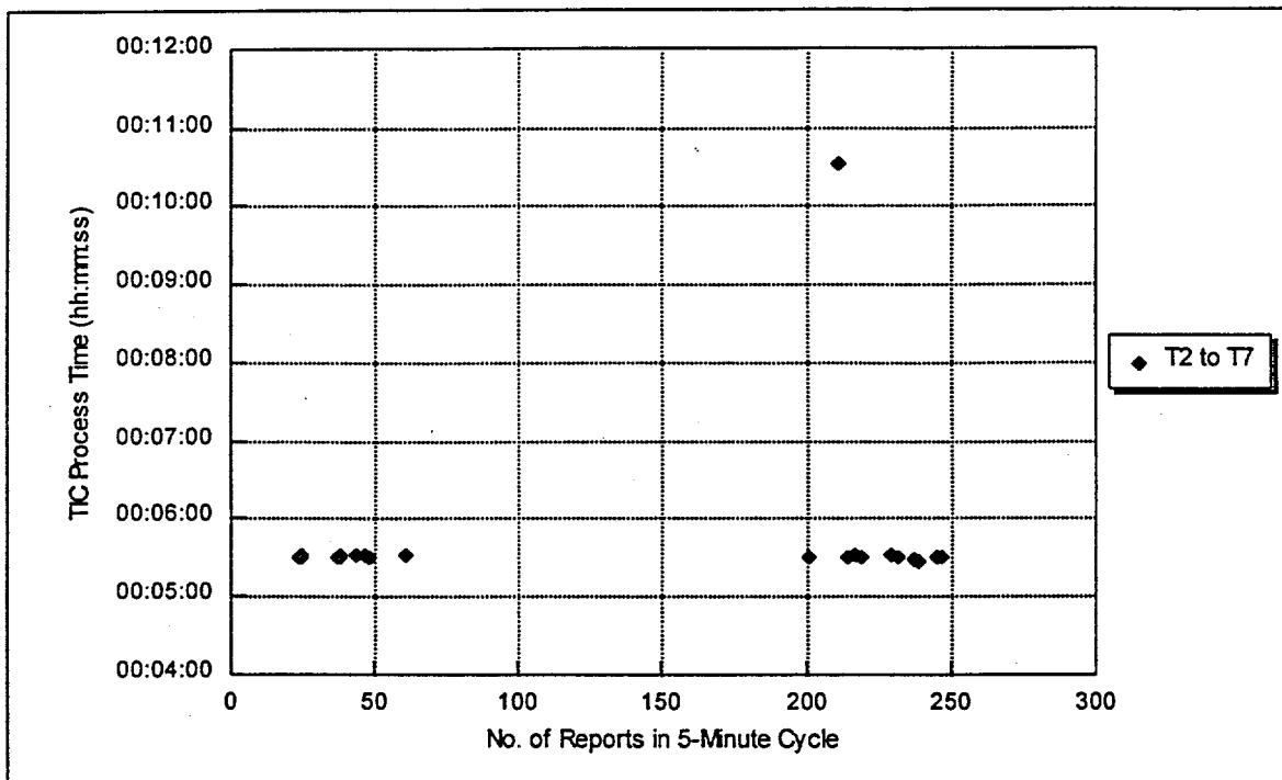
Figure 5.12 TIC Processing Time and Number of Reports Processed Using Live Data
