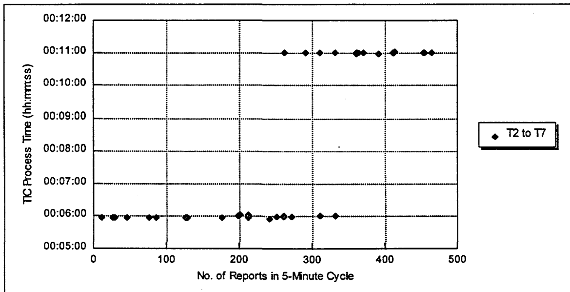
Figure 5.14 TIC Processing Time and Simulated Probe / Loop Detector Reports
