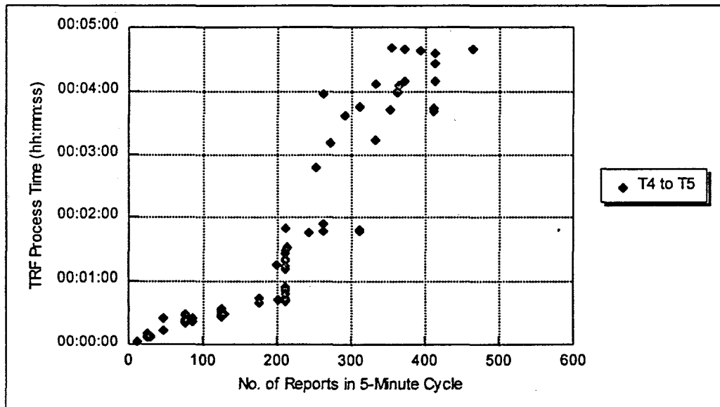
Figure 5.13 TRF Processing Time and Simulated Probe / Loop Detector Reports
