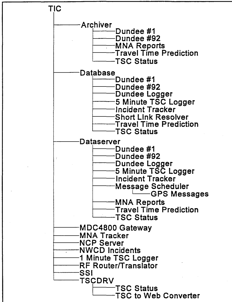
Figure 5.2 TIC Process Failure Hierarchy
