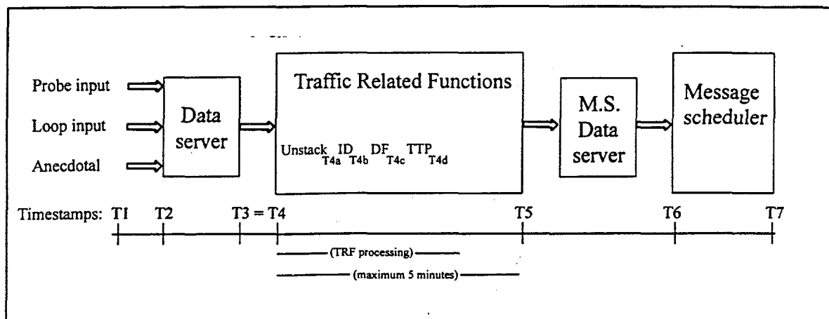
Figure 5.10 Timestamps Logged by the TIC
