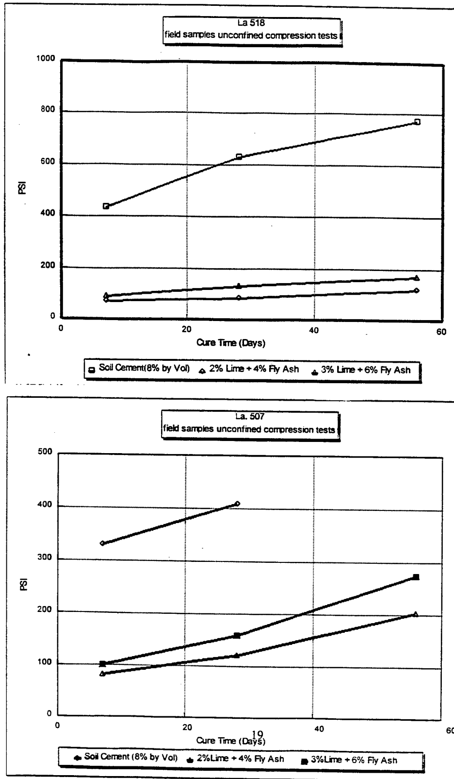
Figure 3 Field and Laboratory unconfined compression results
