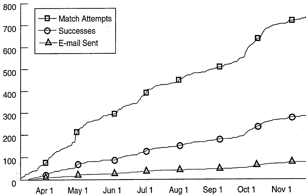
Figure 5: Usage as a function of time
