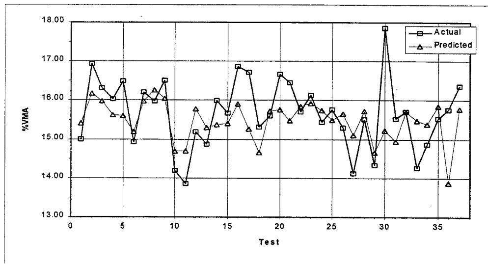
Figure 7.3 MDT Data: Corrected Estimation of the %VMA
