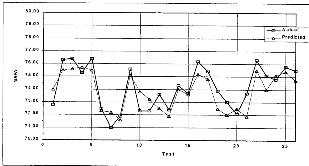
Figure 7.11 GDOT Data: Estimation of the %VFA
