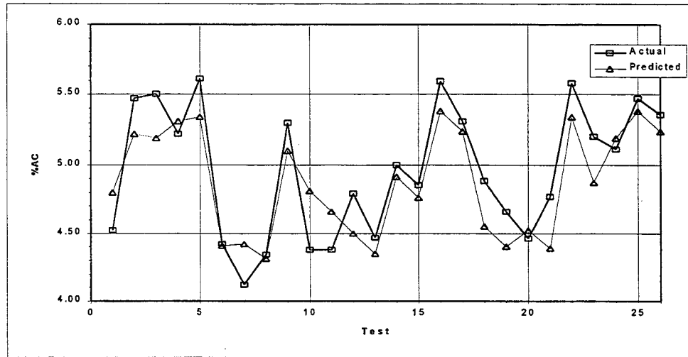
Figure 7.8 GDOT Data: Estimation of the %AC
