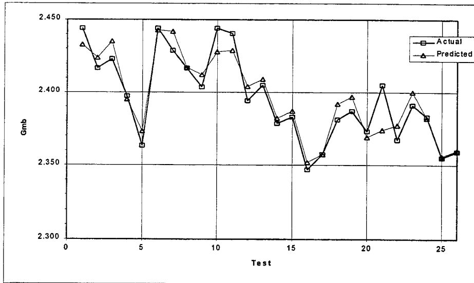
Figure 7.6 GDOT Data: Estimation of G_{mb}
