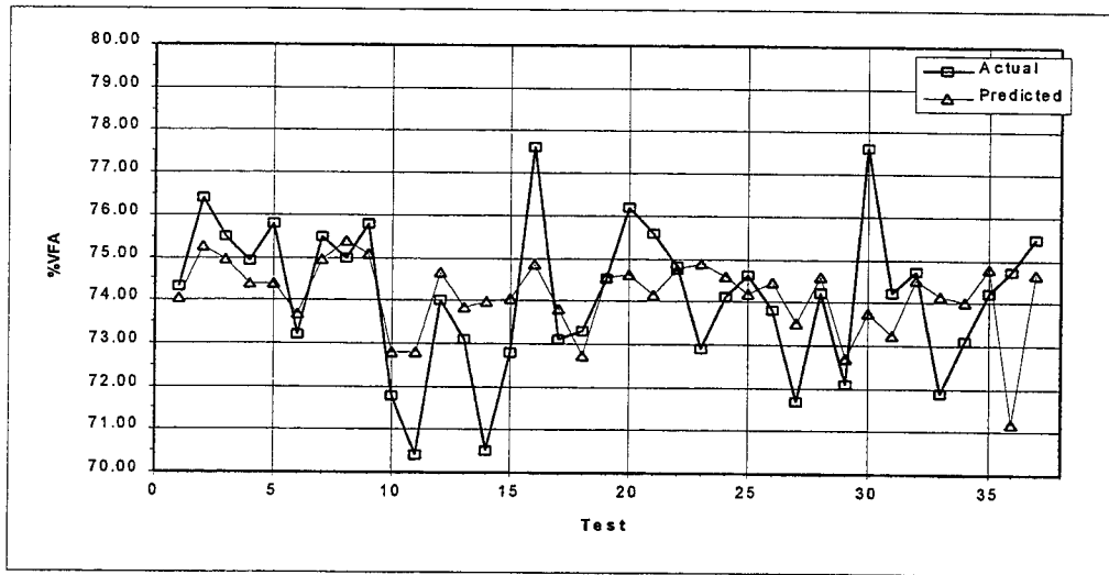
Figure 7.10 MDT Data: Corrected Estimation of the %VFA
