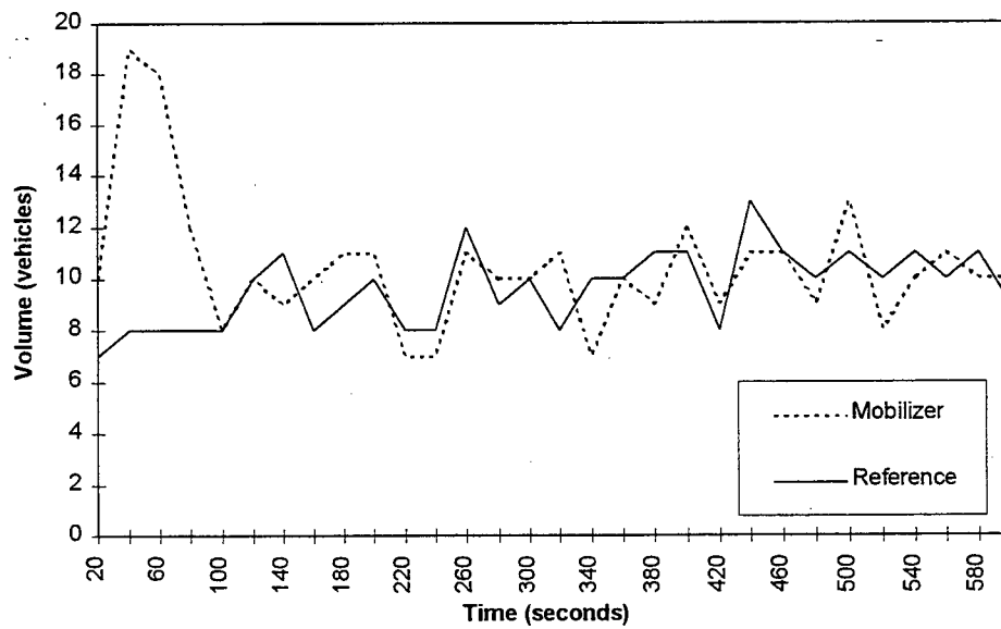
Figure 15. Volume Comparison - Lane 4
