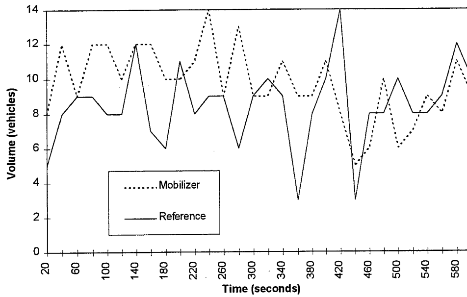
Figure 13. Volume Comparison - Lane 4
