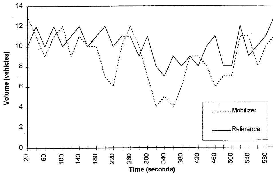
Figure 12. Volume Comparison - Lane 1
