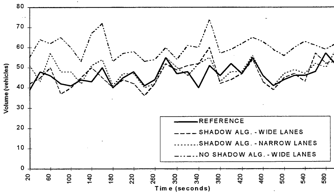
Figure 7. Lane Geometry Comparison
