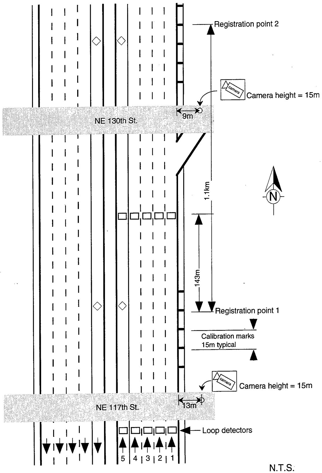
Figure 5. Test Section Layout
