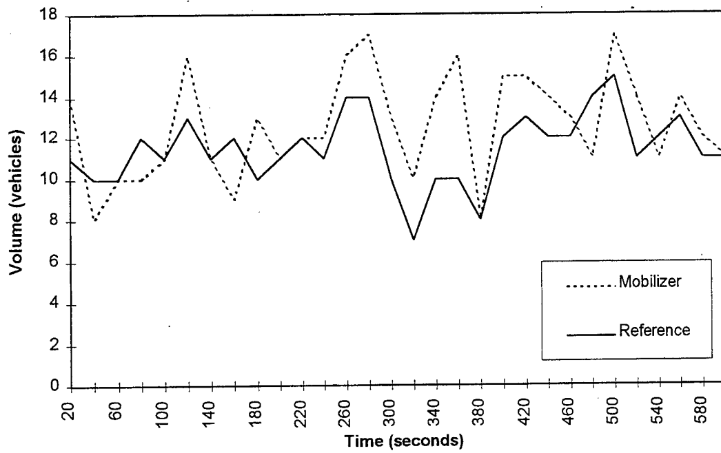
Figure 11. Volume Comparison - Lane 4
