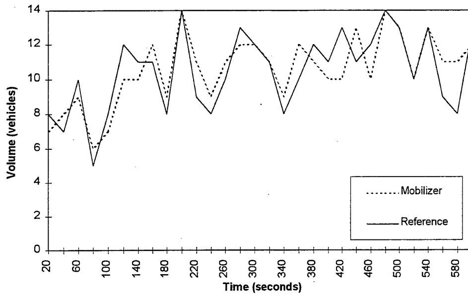
Figure 9. Volume Comparison - Lane 1
