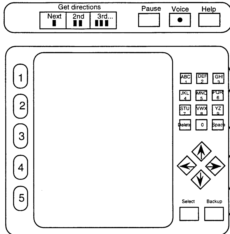
Figure 3. Design A - Soft Keys and Dedicated Keys (12 dedicated keys (including arrow cursor keys), 12-key alphanumeric pad, 5 soft keys, and a menu hierarchy with many layers)
