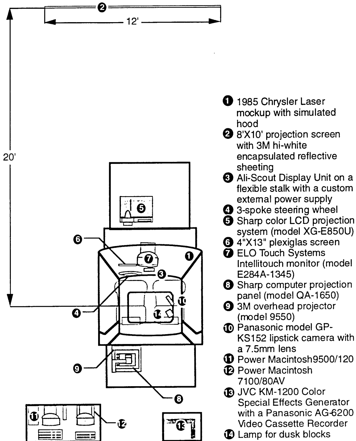
Figure 17. Simulator Layout
