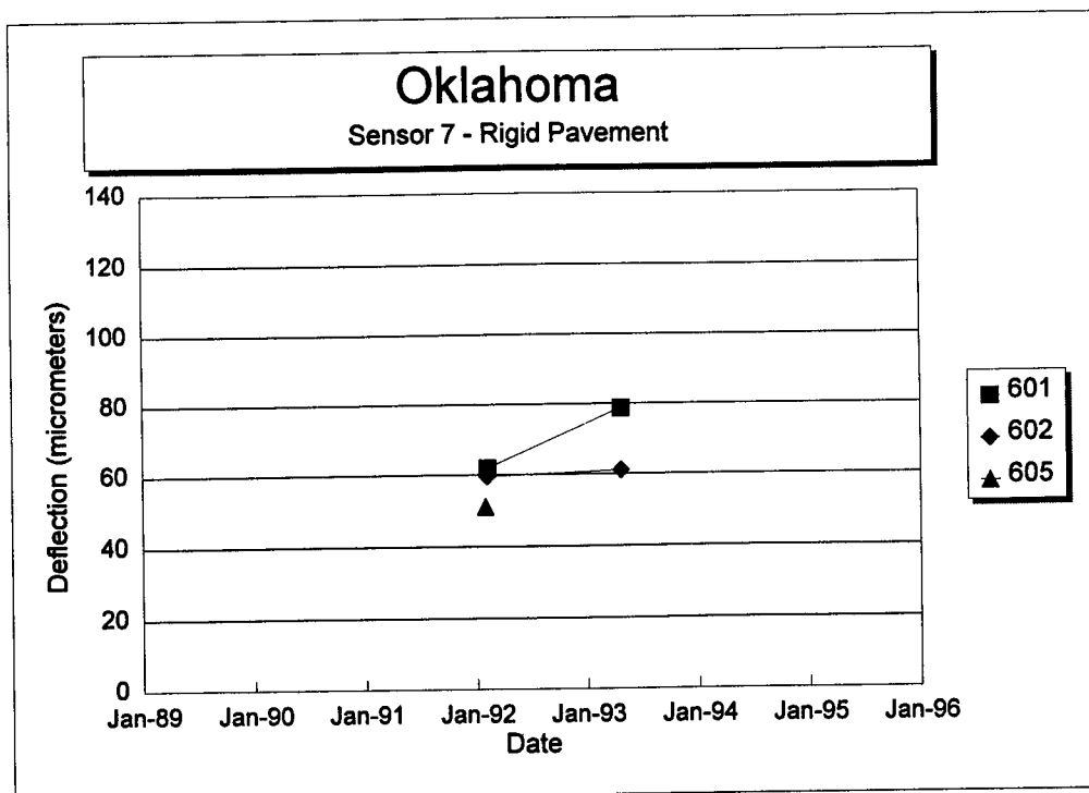
Figure 150. Sensor 7 deflection versus time for each section of the Oklahoma SPS-6 project.
