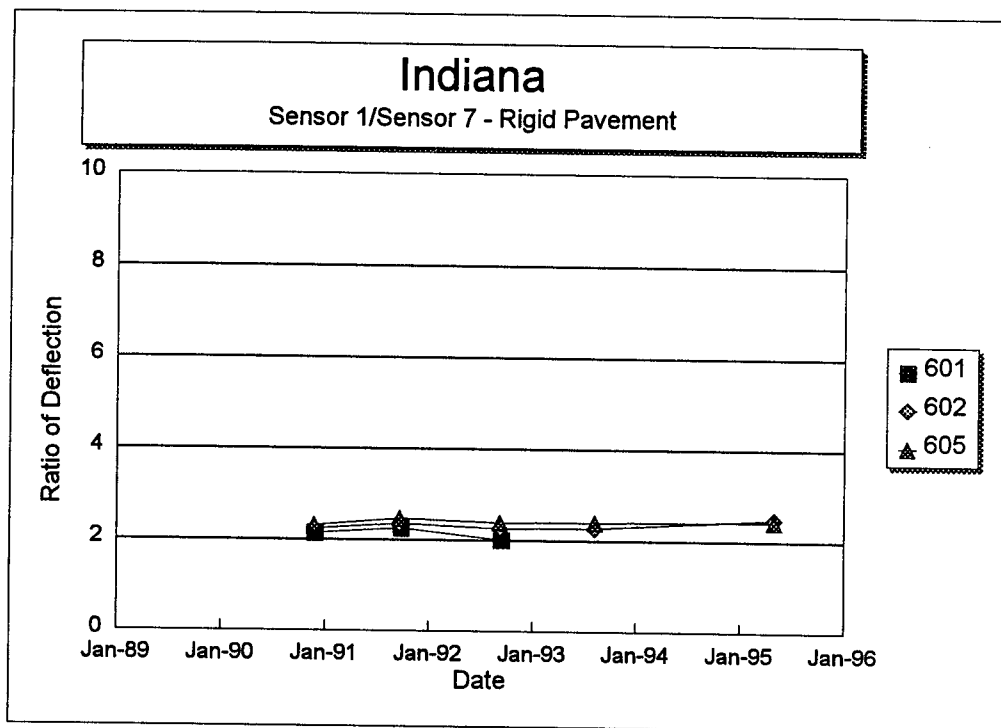
Figure 139. Sensor 1 deflection divided by Sensor 7 deflection versus time for each section of the Indiana SPS-6 project.
