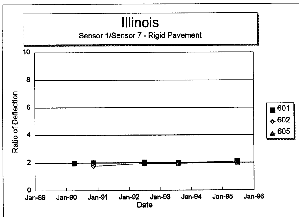
Figure 136. Sensor 1 deflection divided by Sensor 7 deflection versus time for each section of the Illinois SPS-6 project.
