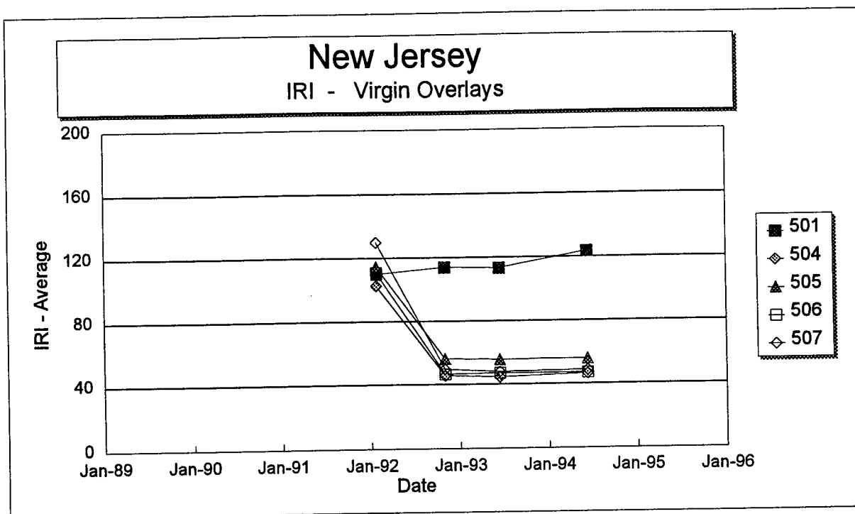
Figure 48. International Roughness Index versus time on each section of the New Jersey SPS-5 project.
