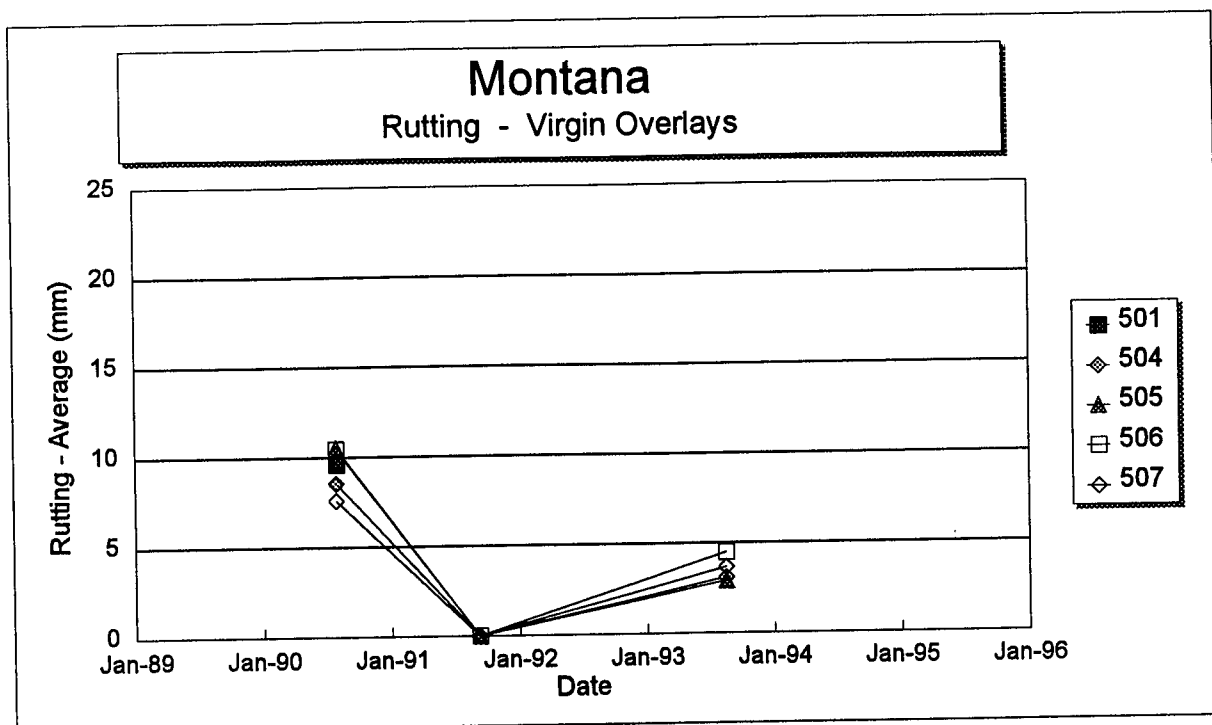
Figure 60. Rut depth versus time on each section of the Montana SPS-5 project.
