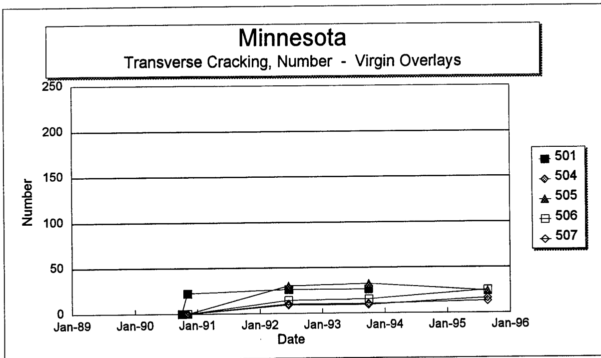
Figure 26. Total number of transverse cracks versus time on each section of the Minnesota SPS-5 project.
