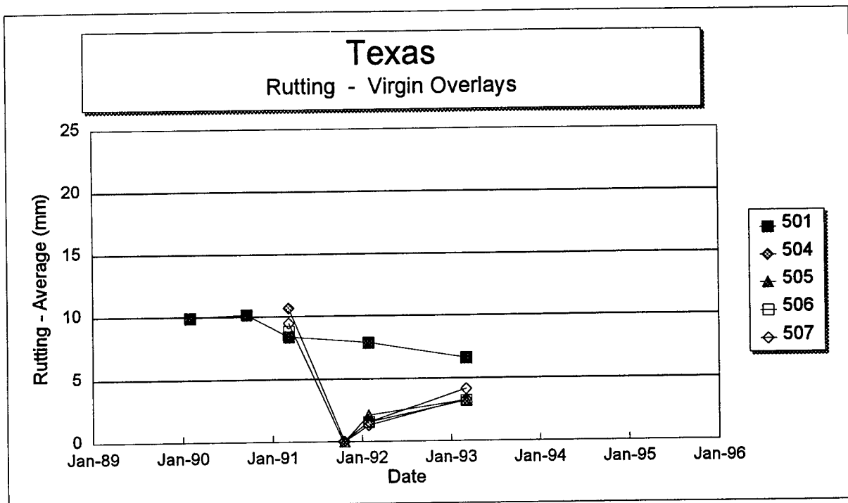
Figure 62. Rut depth versus time on each section of the Texas SPS-5 project.
