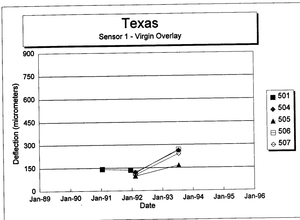
Figure 98. Sensor 1 deflection versus time for each section of the Texas SPS-5 project.
