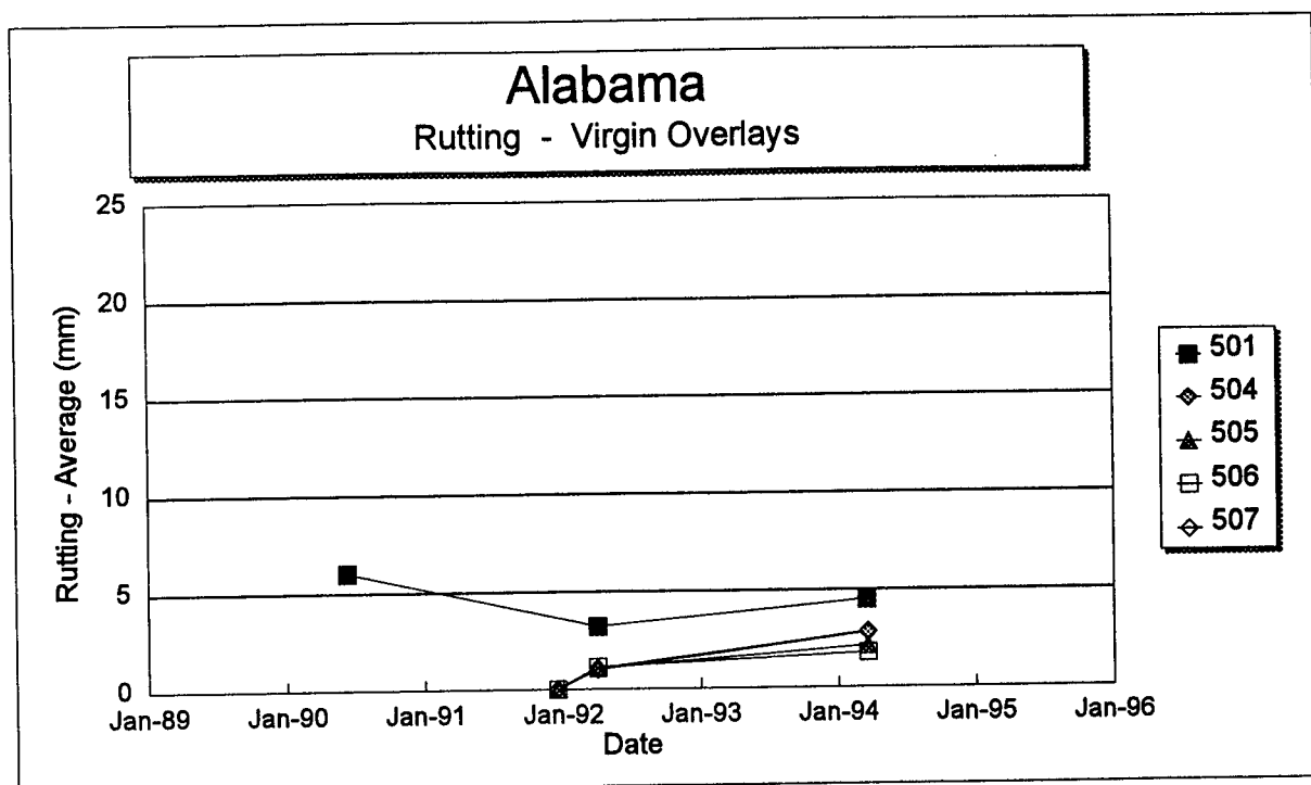
Figure 52. Rut depth versus time on each section of the Alabama SPS-5 project.
