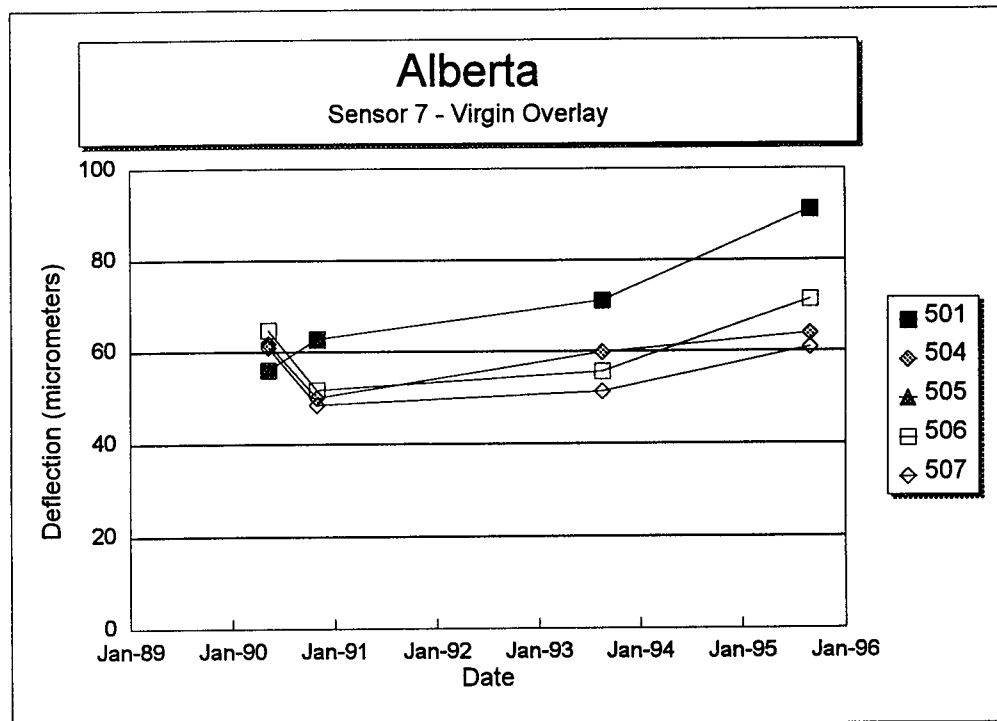
Figure 102. Sensor 7 deflection versus time for each section of the Alberta SPS-5 project.
