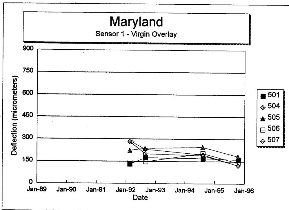
Figure 83. Sensor 1 deflection versus time for each section of the Maryland SPS-5 project.
