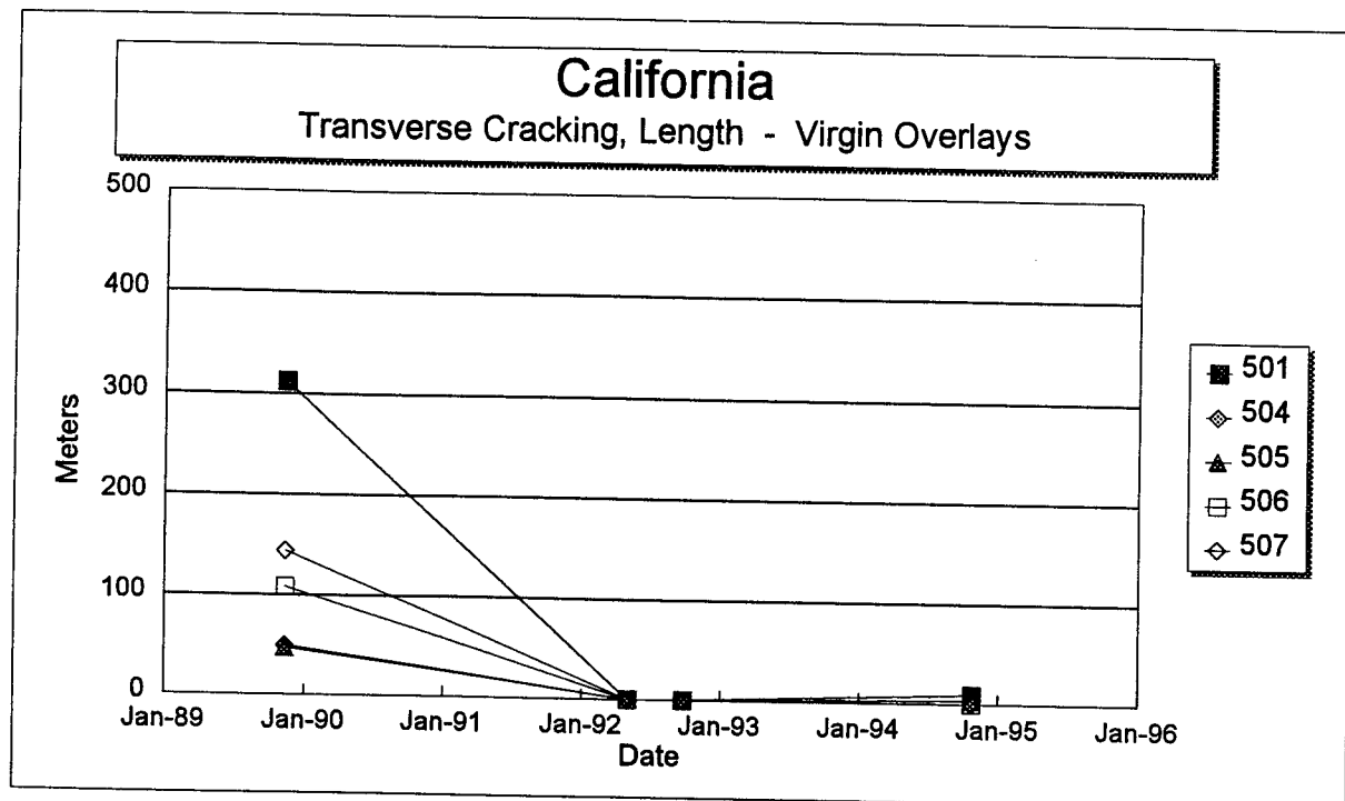
Figure 31. Total length of transverse cracks versus time on each section of the California SPS-5 project.
