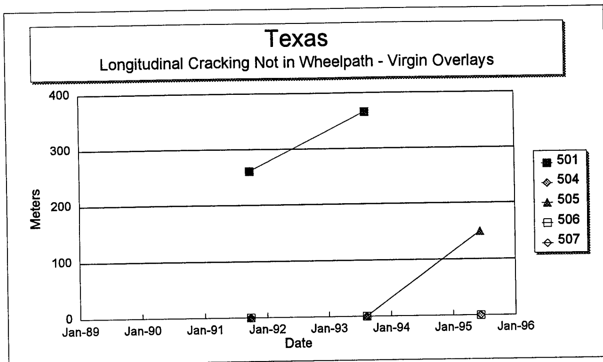
Figure 20. Total length of longitudinal cracking not in the wheelpath versus time on each section of the Texas SPS-5 project.
