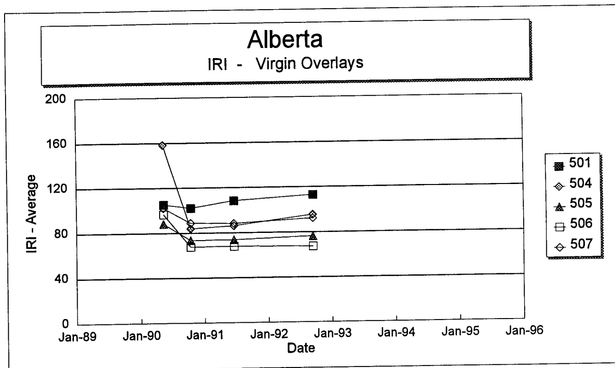
Figure 50. International Roughness Index versus time on each section of the Alberta SPS-5 project.
