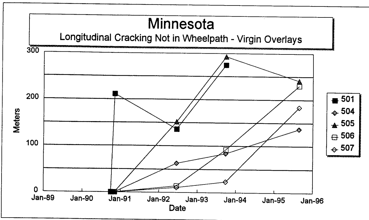
Figure 19. Total length of longitudinal cracking not in the wheelpath versus time on each section of the Minnesota SPS-5 project.
