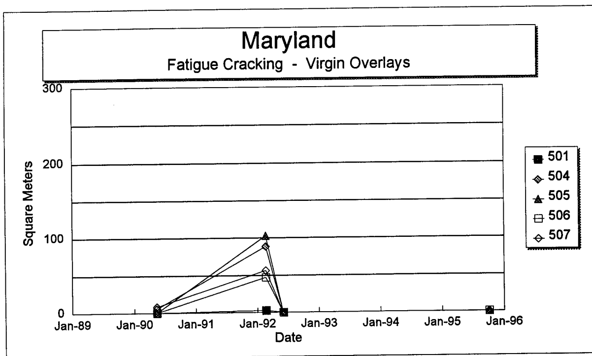
Figure 10. Total area of fatigue cracking versus time on each section of the Maryland SPS-5 project.
