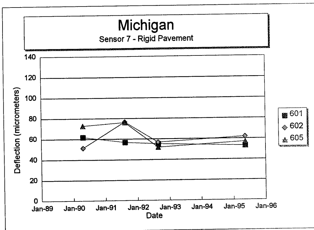
Figure 144. Sensor 7 deflection versus time for each section of the Michigan SPS-6 project.
