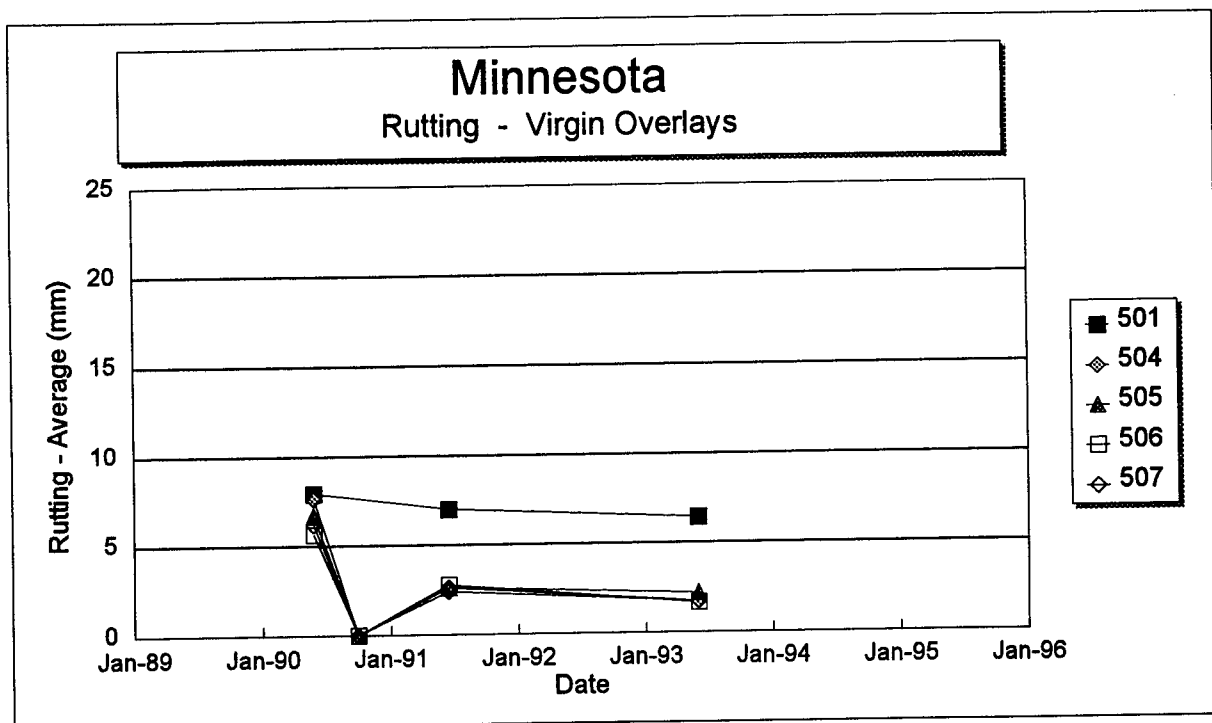
Figure 58. Rut depth versus time on each section of the Minnesota SPS-5 project.
