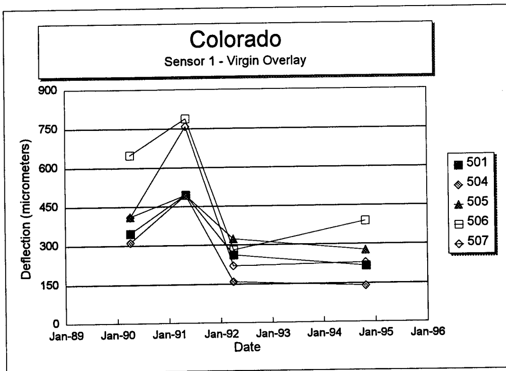
Figure 74. Sensor 1 deflection versus time for each section of the Colorado SPS-5 project.
