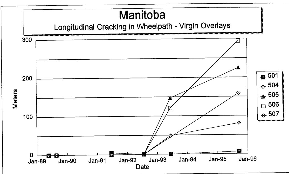
Figure 16. Total length of longitudinal cracking in the wheelpath versus time on each section of the Manitoba SPS-5 project.
