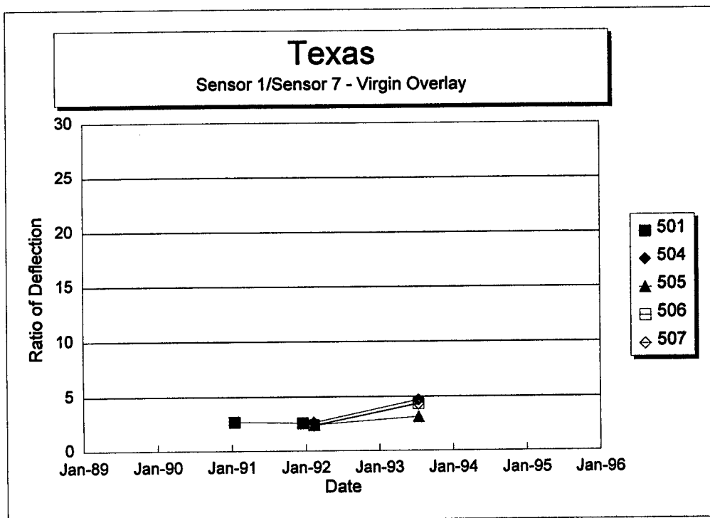
Figure 100. Sensor 1 deflection divided by Sensor 7 deflection versus time for each section of the Texas SPS-5 project.
