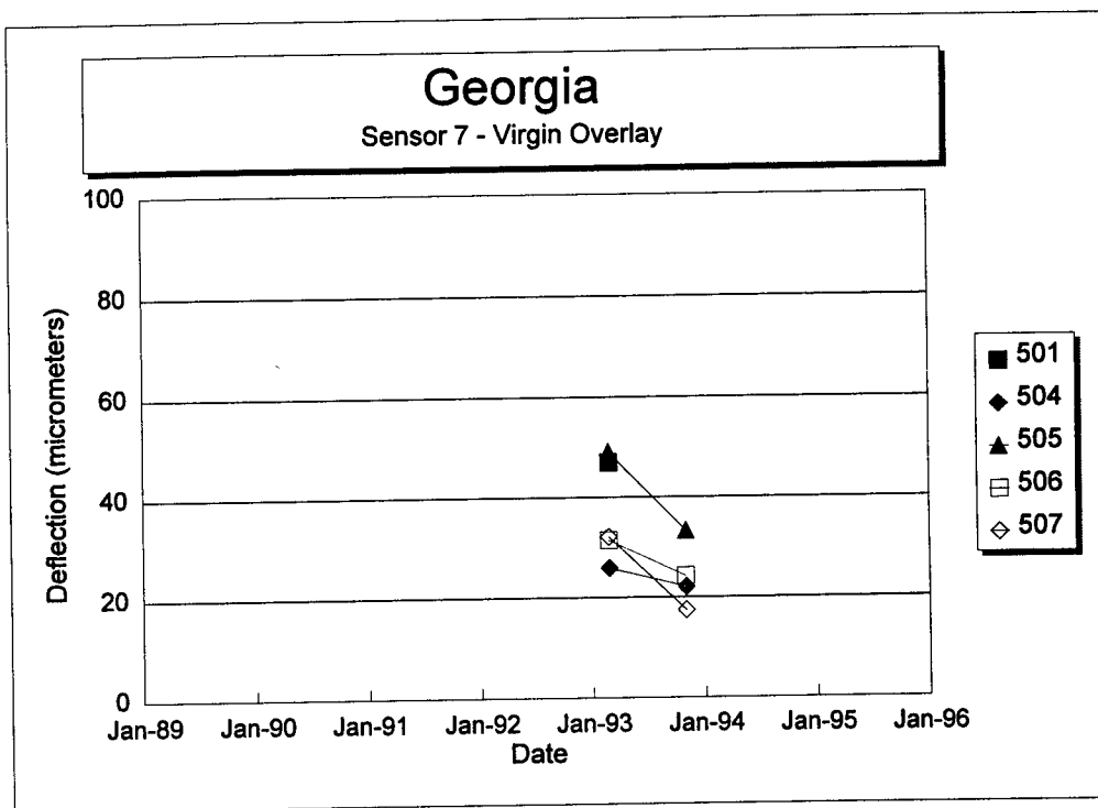
Figure 78. Sensor 7 deflection versus time for each section of the Georgia SPS-5 project.
