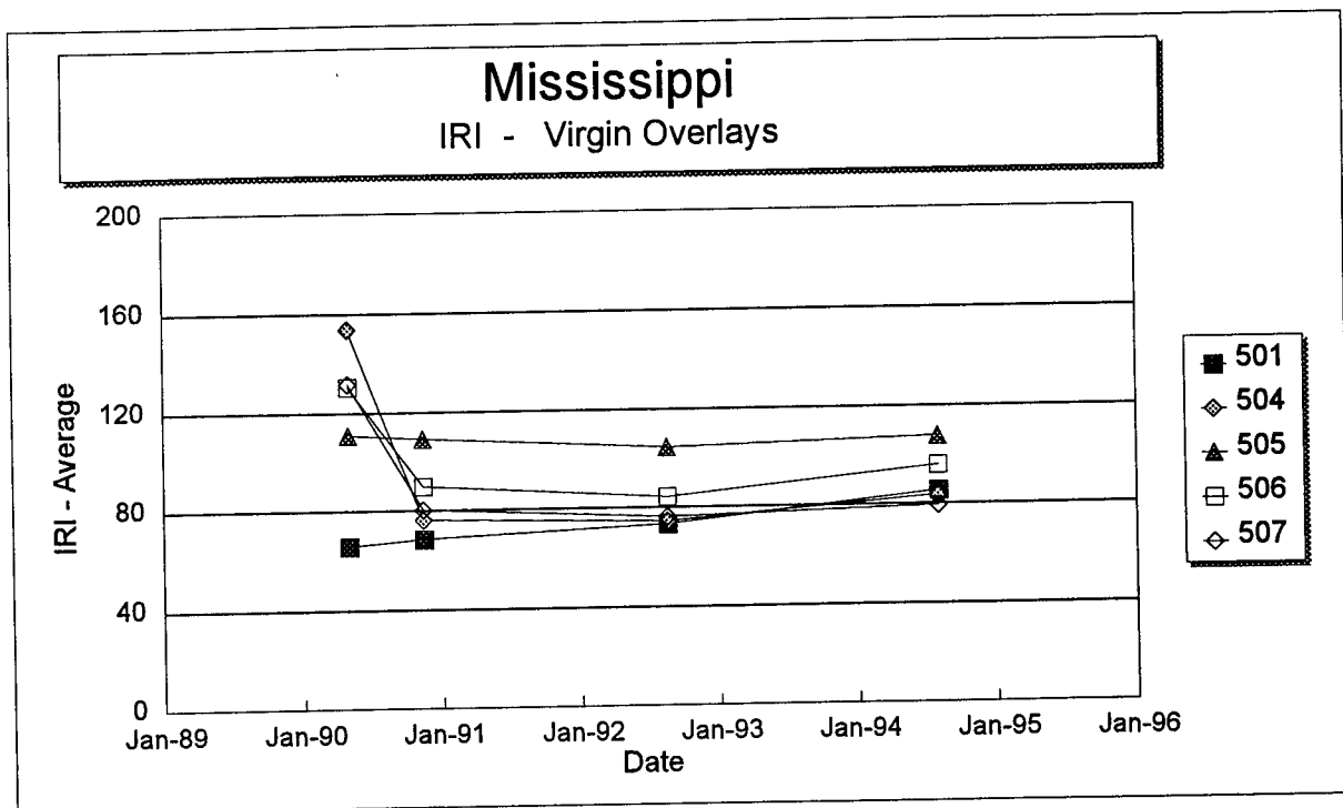
Figure 46. International Roughness Index versus time on each section of the Mississippi SPS-5 project.
