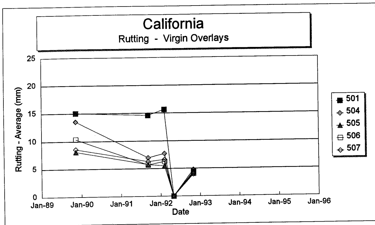
Figure 54. Rut depth versus time on each section of the California SPS-5 project.
