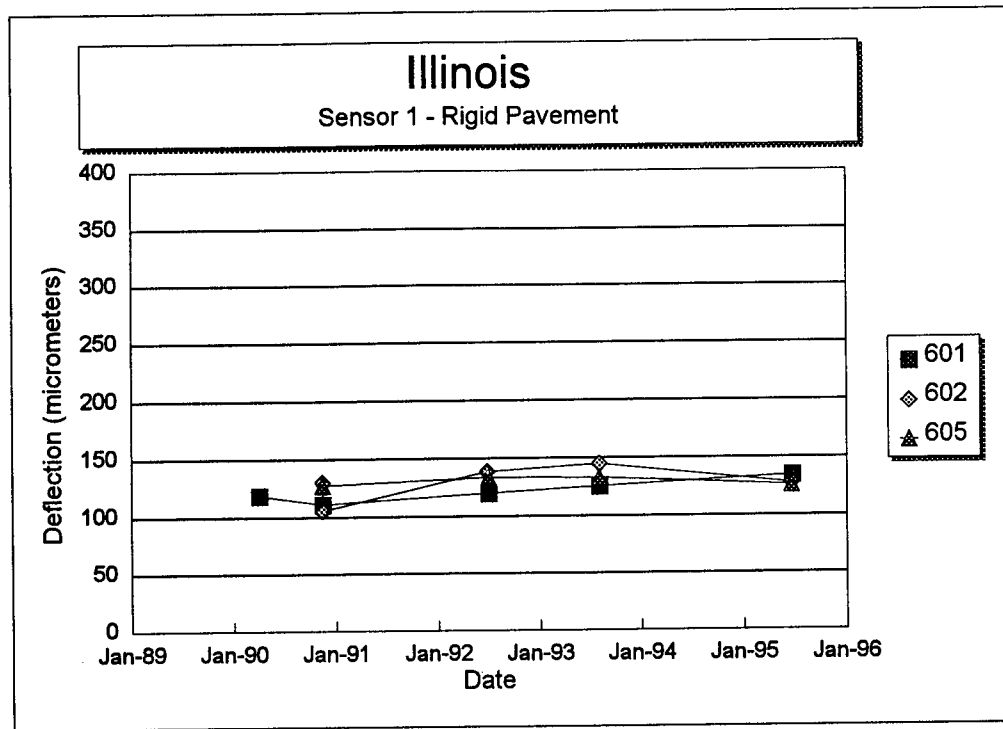
Figure 134. Sensor 1 deflection versus time for each section of the Illinois SPS-6 project.
