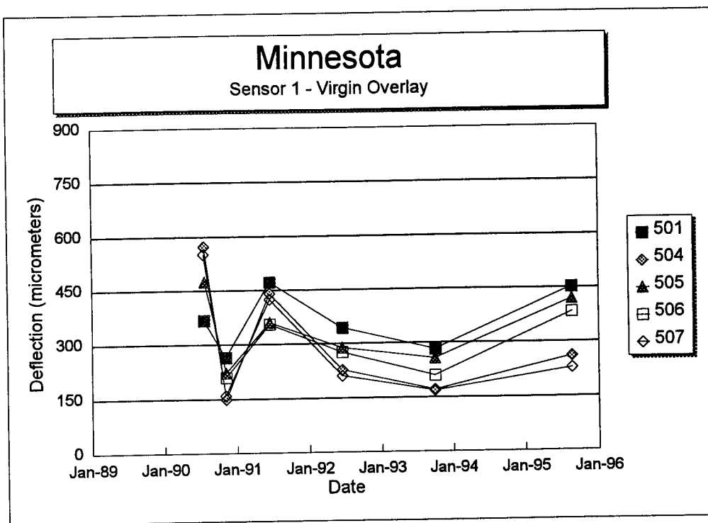
Figure 86. Sensor 1 deflection versus time for each section of the Minnesota SPS-5 project.
