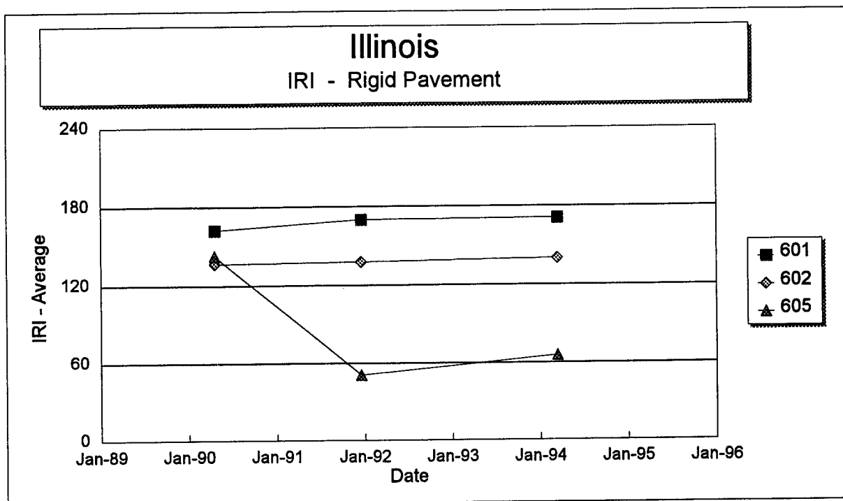
Figure 118. International Roughness Index versus time on each section of the Illinois SPS-6 project.
