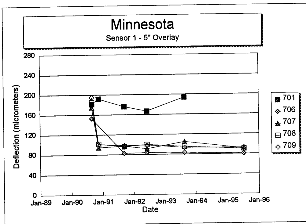
Figure 174. Sensor 1 deflection versus time for each section of the Minnesota SPS-7 project.
