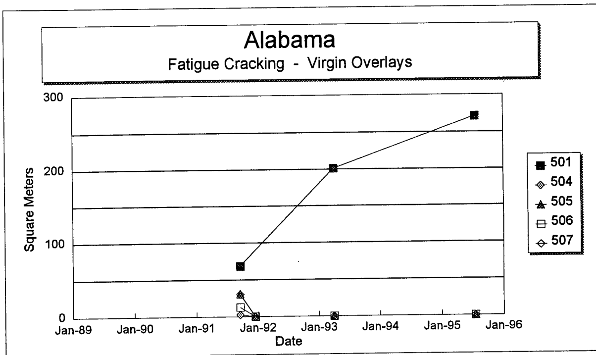
Figure 6. Total area of fatigue cracking versus time on each section of the Alabama SPS-5 project.
