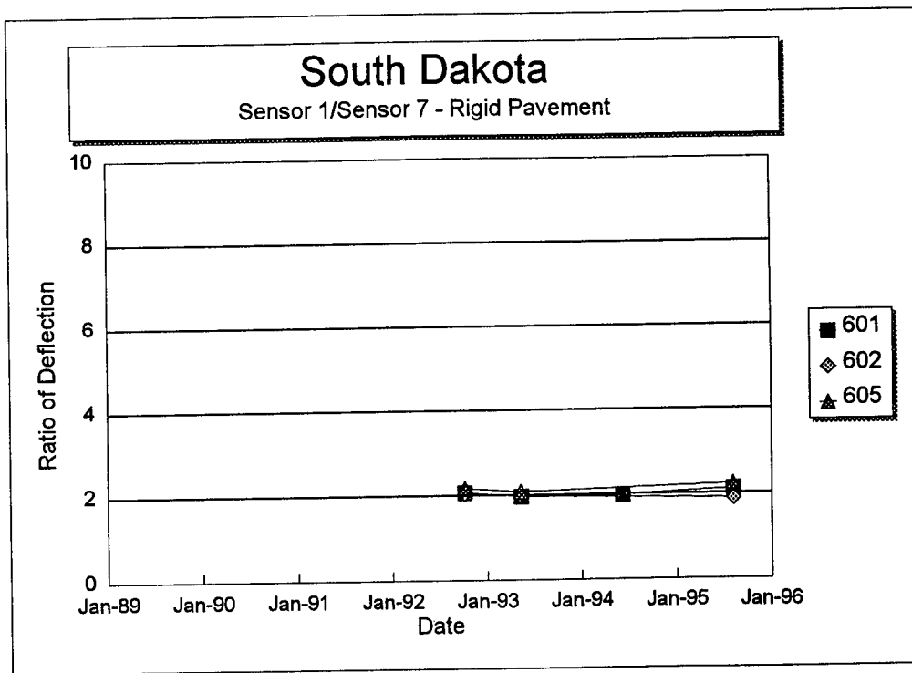
Figure 154. Sensor 1 deflection divided by Sensor 7 deflection versus time for each section of the South Dakota SPS-6 project.
