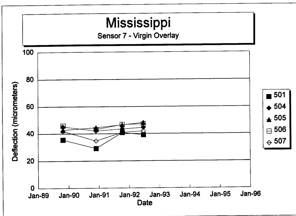
Figure 90. Sensor 7 deflection versus time for each section of the Mississippi SPS-5 project.
