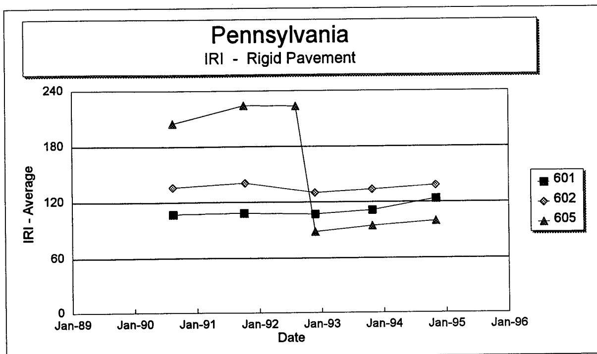
Figure 124. International Roughness Index versus time on each section of the Pennsylvania SPS-6 project.
