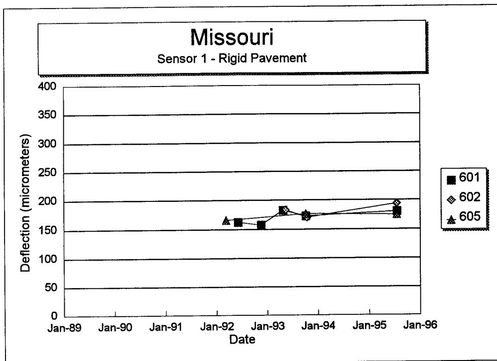
Figure 146. Sensor 1 deflection versus time for each section of the Missouri SPS-6 project.
