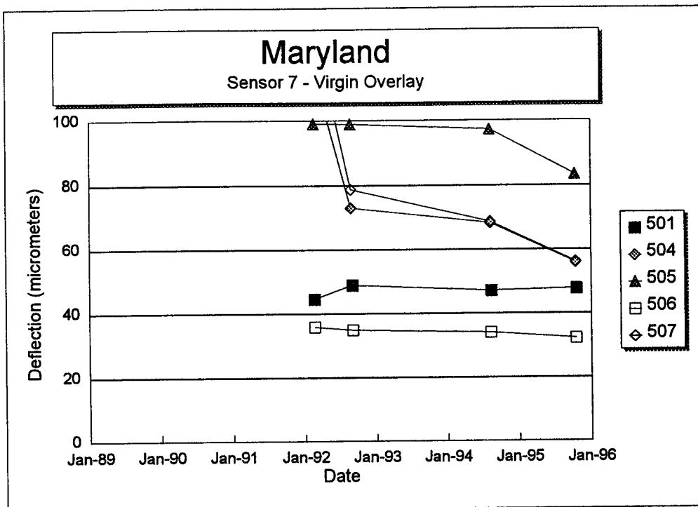
Figure 84. Sensor 7 deflection versus time for each section of the Maryland SPS-5 project.
