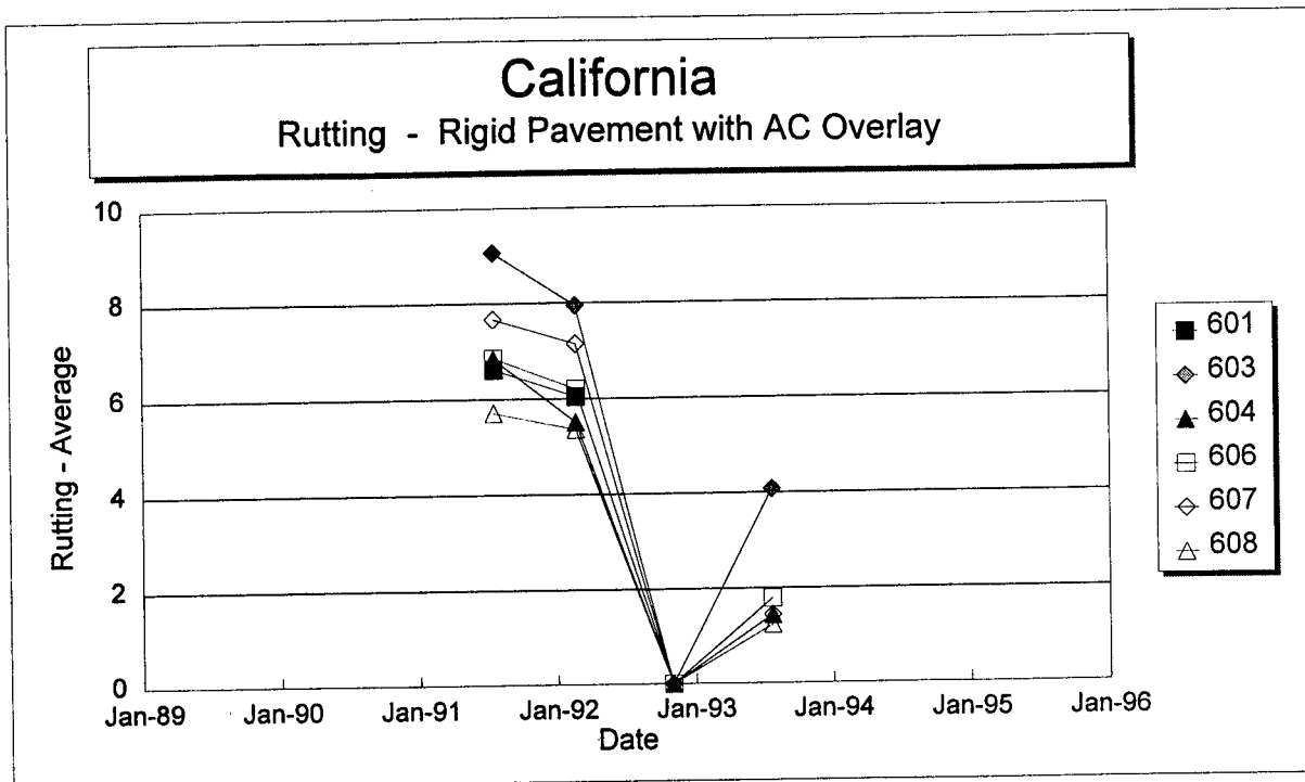
Figure 126. Rut depth versus time on each HMAC section of the Arizona and California SPS-6 projects.
