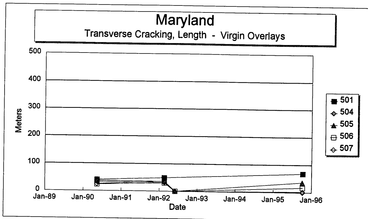
Figure 33. Total length of transverse cracks versus time on each section of the Maryland SPS-5 project.
