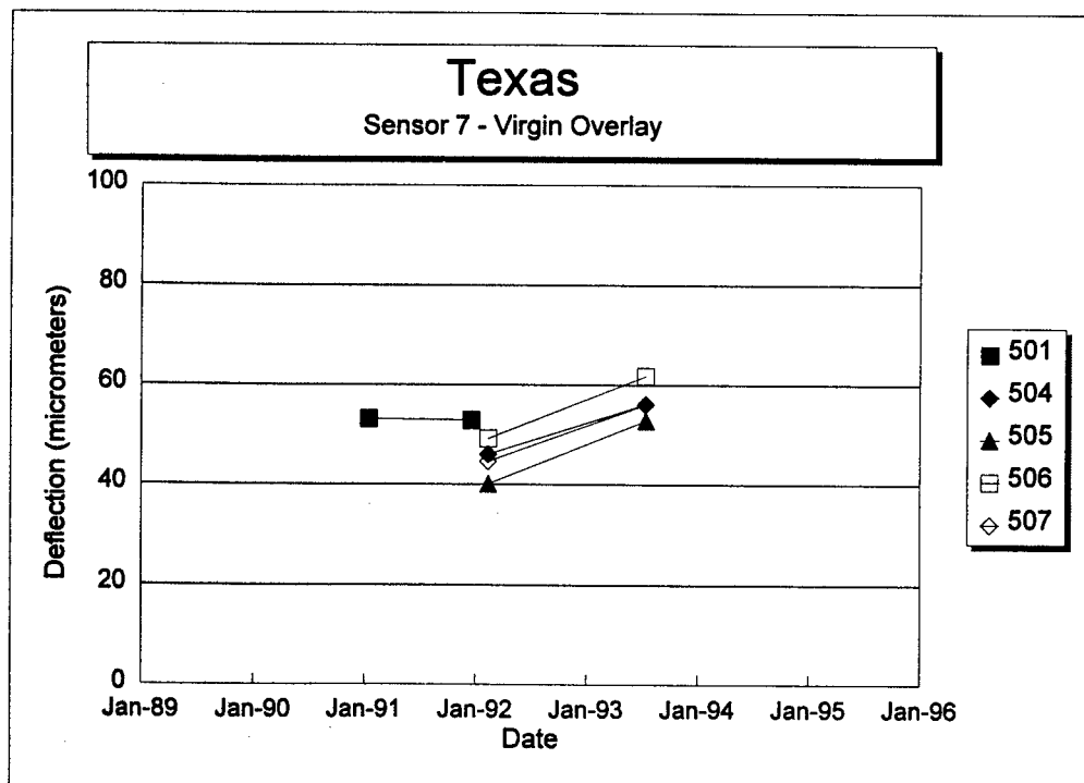
Figure 99. Sensor 7 deflection versus time for each section of the Texas SPS-5 project.
