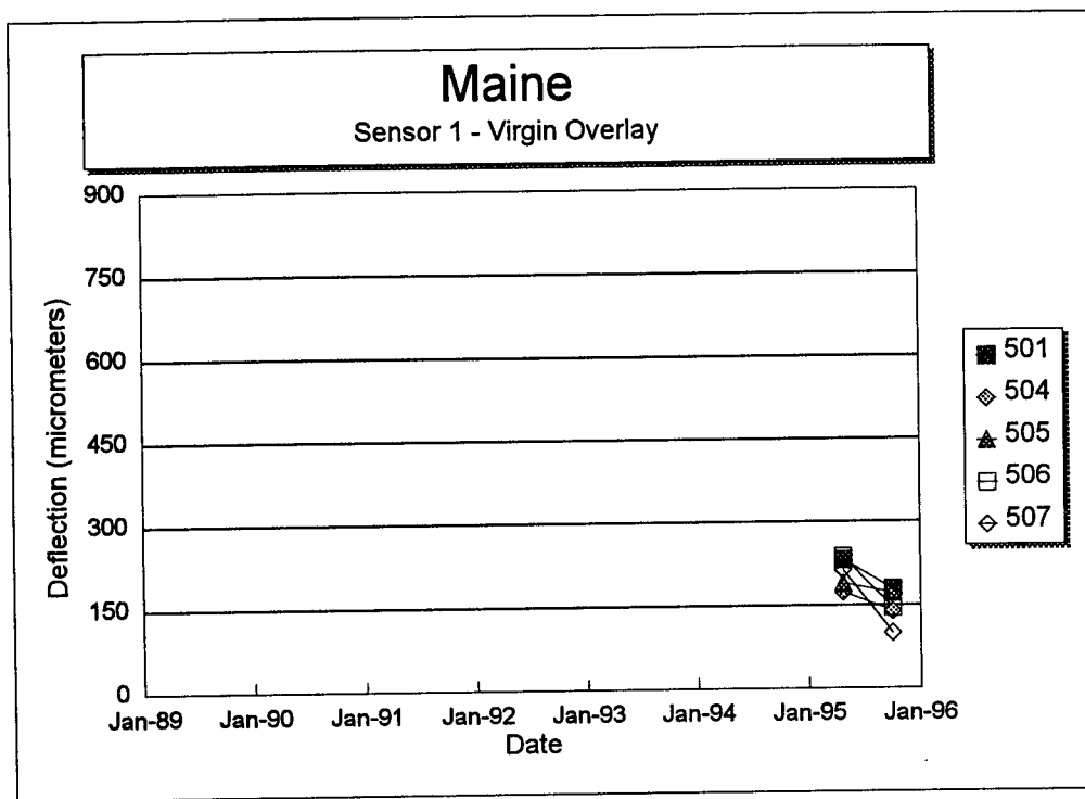
Figure 80. Sensor 1 deflection versus time for each section of the Maine SPS-5 project.
