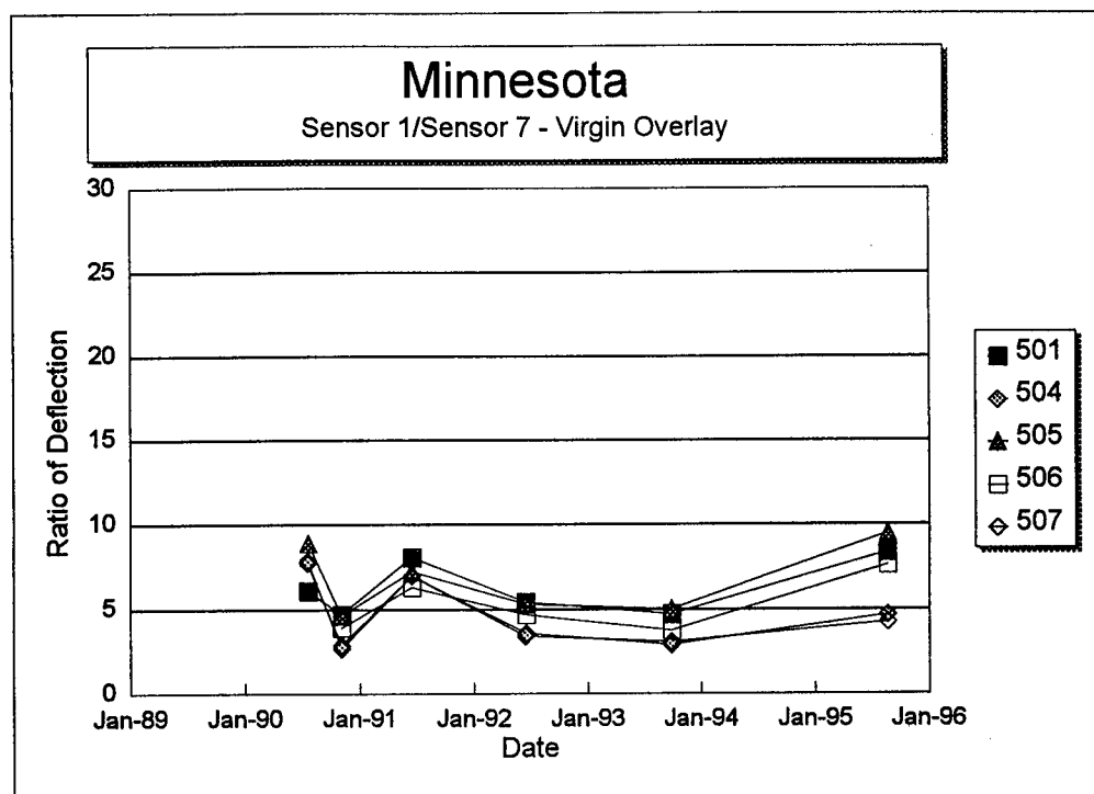
Figure 88. Sensor 1 deflection divided by Sensor 7 deflection versus time for each section of the Minnesota SPS-5 project.
