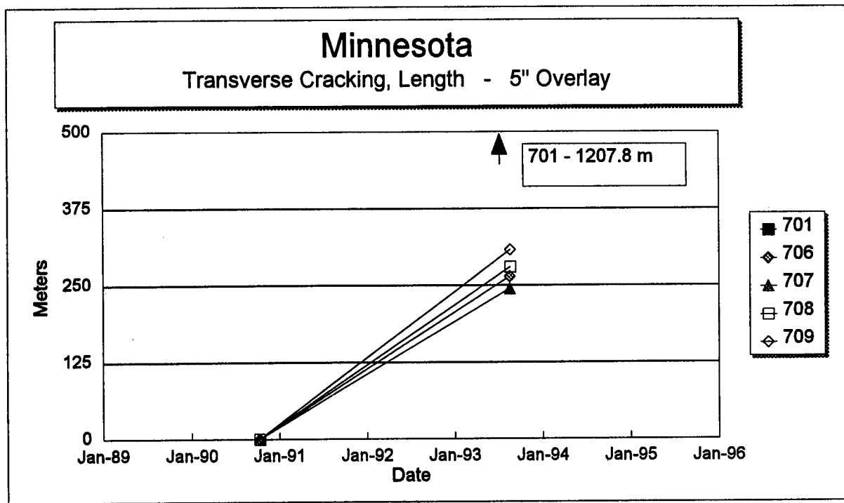
Figure 160. Total length of transverse cracks versus time on each section of the Minnesota SPS-7 project.
