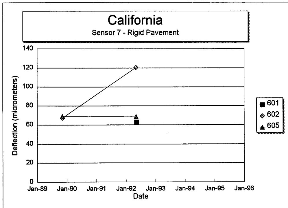
Figure 132. Sensor 7 deflection versus time for each section of the California SPS-6 project.
