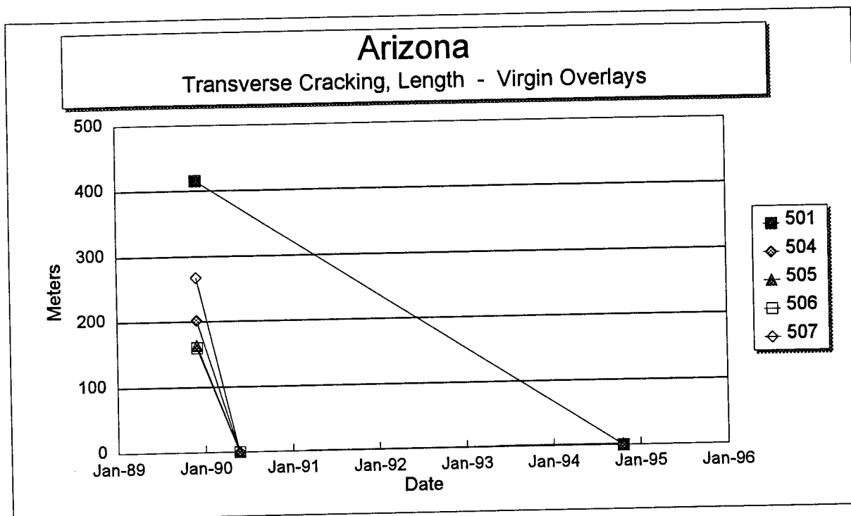
Figure 30. Total length of transverse cracks versus time on each section of the Arizona SPS-5 project.
