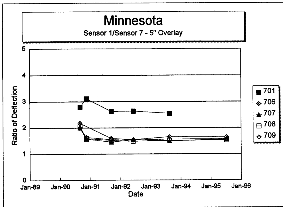
Figure 176. Sensor 1 deflection divided by Sensor 7 deflection versus time for each section of the Minnesota SPS-7 project.
