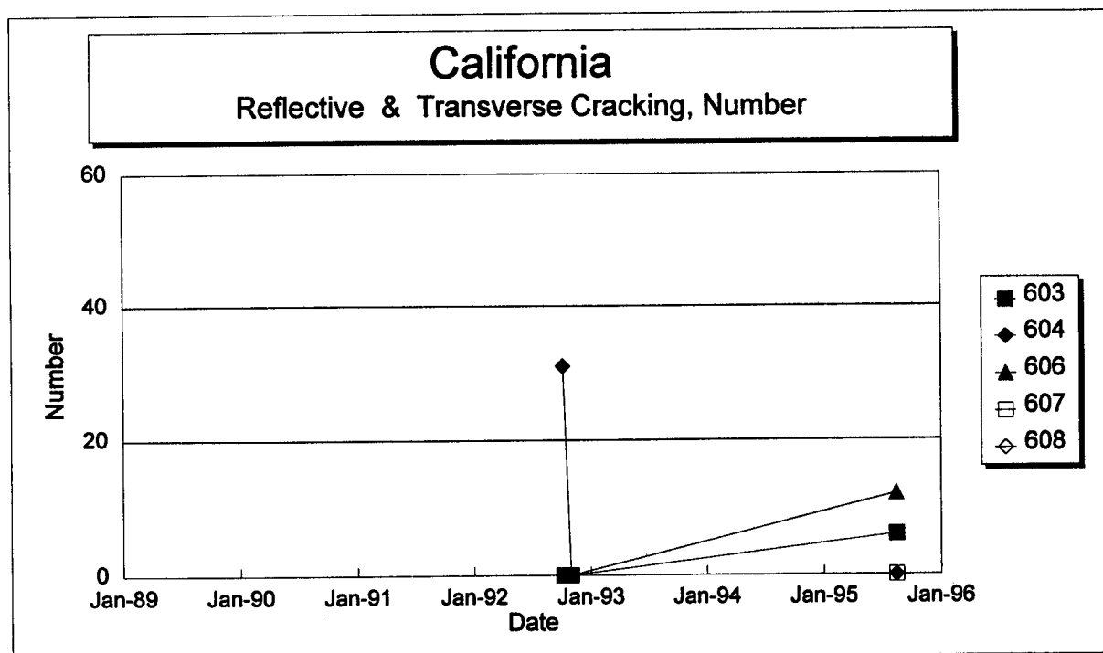
Figure 108. Total number of reflective and transverse cracks versus time on each HMAC section of the California SPS-6 project.
