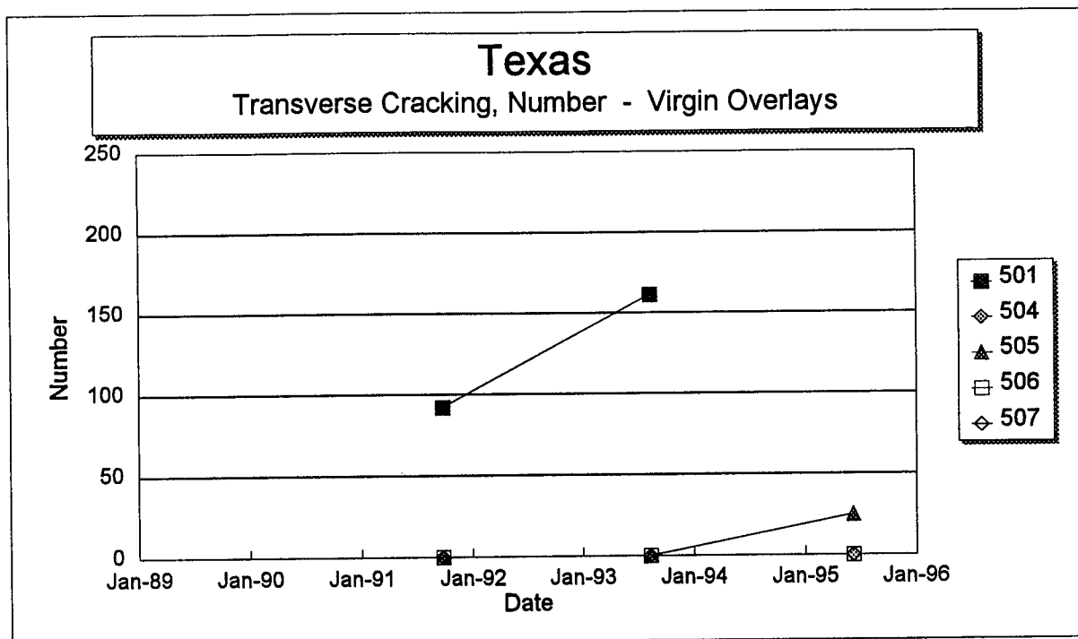
Figure 28. Total number of transverse cracks versus time on each section of the Texas SPS-5 project.
