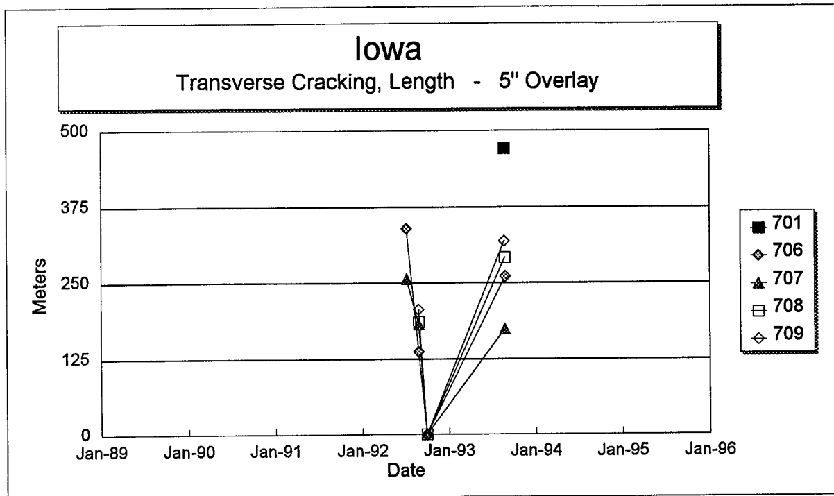
Figure 156. Total length of transverse cracks versus time on each section of the Iowa SPS-7 project.
