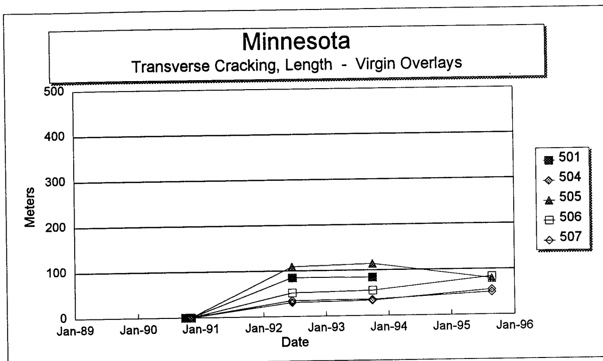
Figure 34. Total length of transverse cracks versus time on each section of the Minnesota SPS-5 project.
