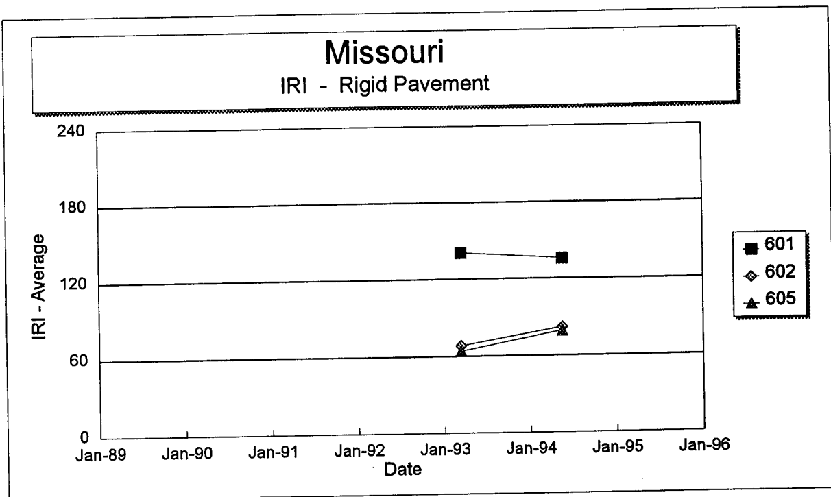
Figure 122. International Roughness Index versus time on each section of the Missouri SPS-6 project.
