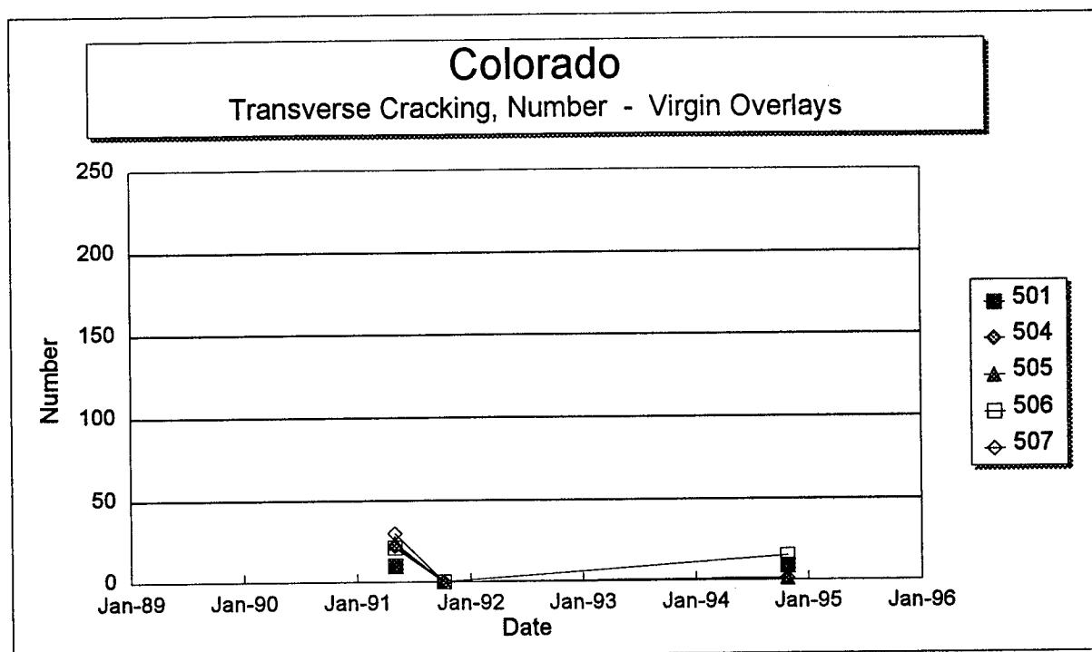
Figure 24. Total number of transverse cracks versus time on each section of the Colorado SPS-5 project.
