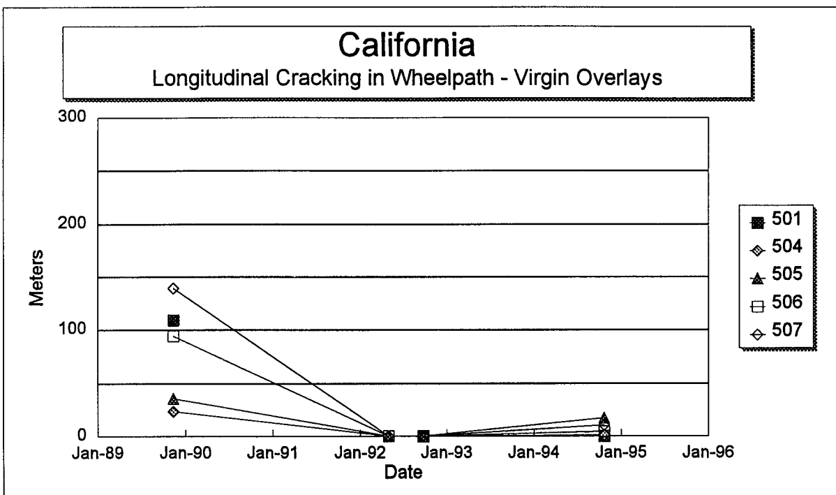
Figure 12. Total length of longitudinal cracking in the wheelpath versus time on each section of the California SPS-5 project.
