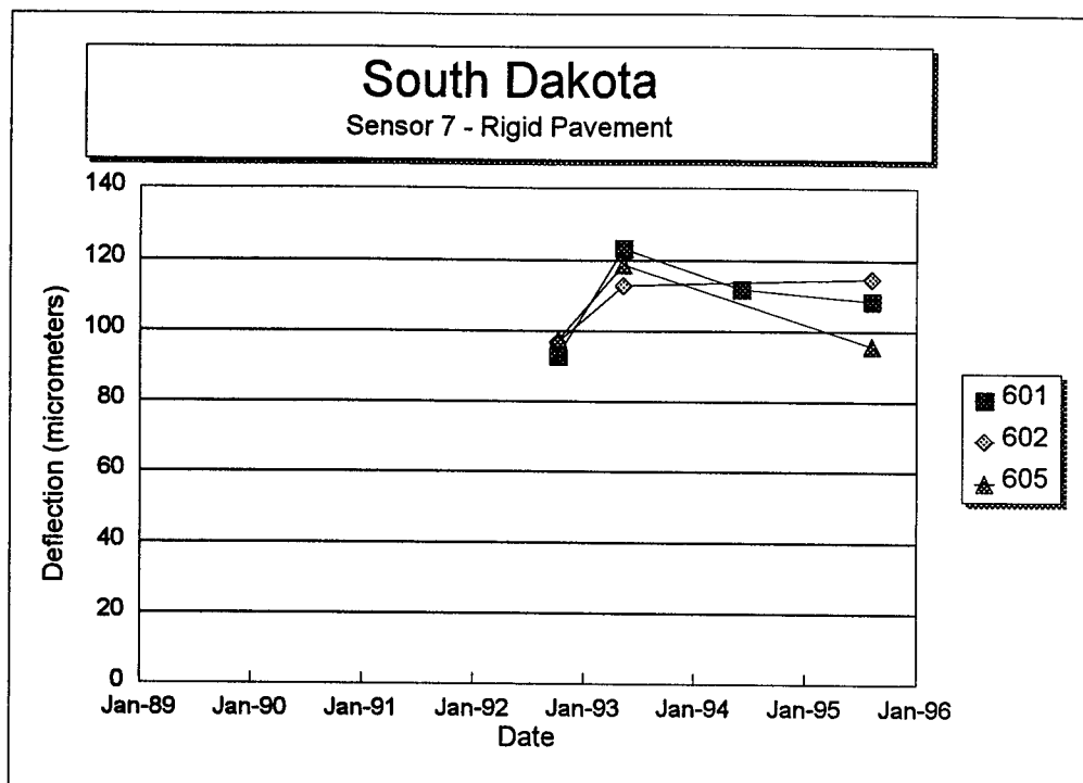
Figure 153. Sensor 7 deflection versus time for each section of the South Dakota SPS-6 project.
