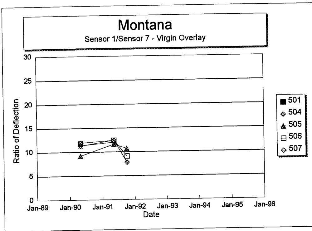
Figure 94. Sensor 1 deflection divided by Sensor 7 deflection versus time for each section of the Montana SPS-5 project.
