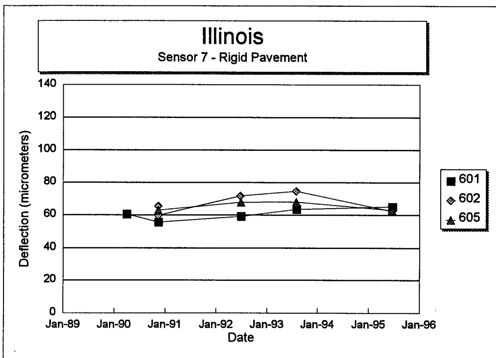
Figure 135. Sensor 7 deflection versus time for each section of the Illinois SPS-6 project.
