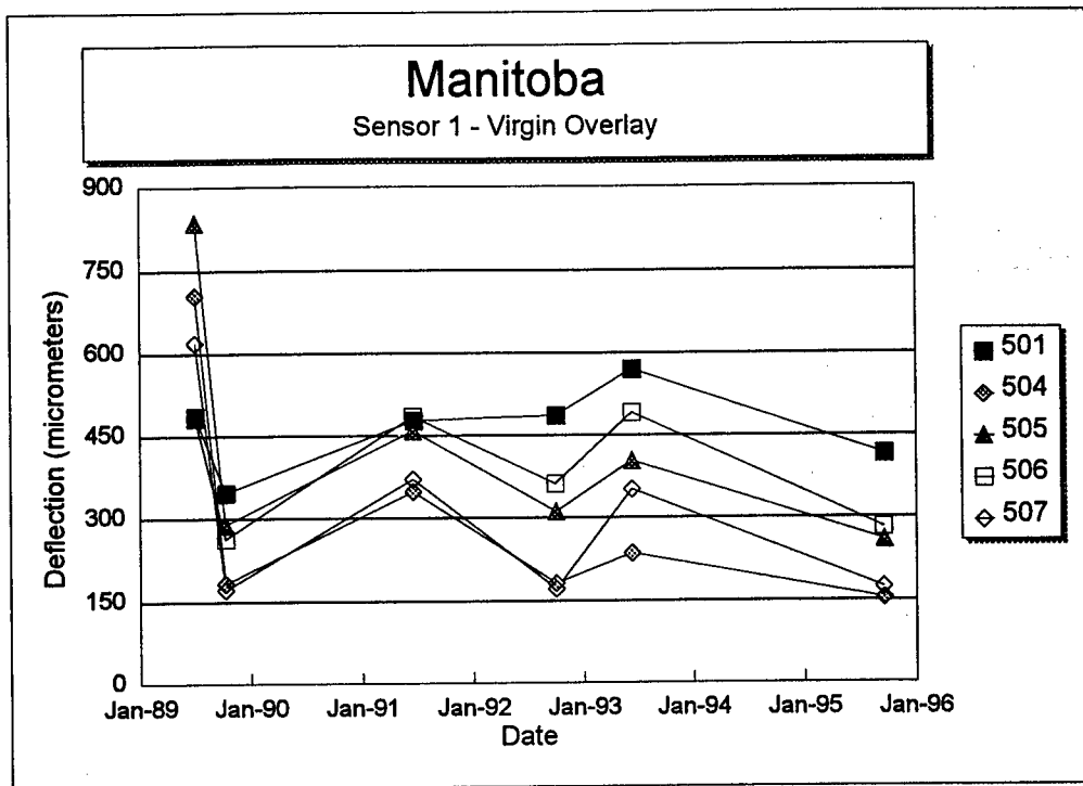
Figure 104. Sensor 1 deflection versus time for each section of the Manitoba SPS-5 project.
