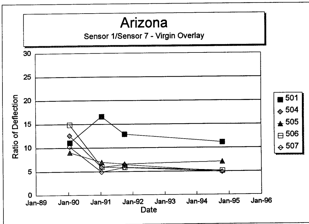
Figure 70. Sensor 1 deflection divided by Sensor 7 deflection versus time for each section of the Arizona SPS-5 project.
