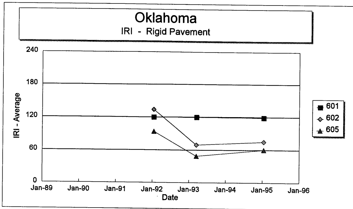
Figure 123. International Roughness Index versus time on each section of the Oklahoma SPS-6 project.
