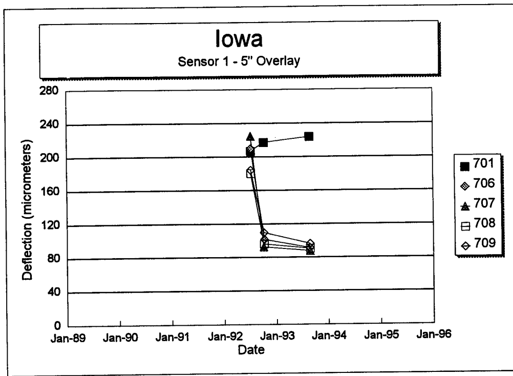
Figure 168. Sensor 1 deflection versus time for each section of the Iowa SPS-7 project.
