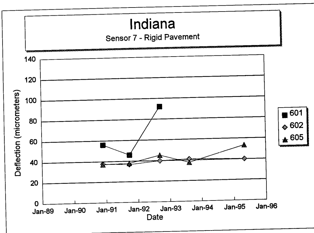
Figure 138. Sensor 7 deflection versus time for each section of the Indiana SPS-6 project.
