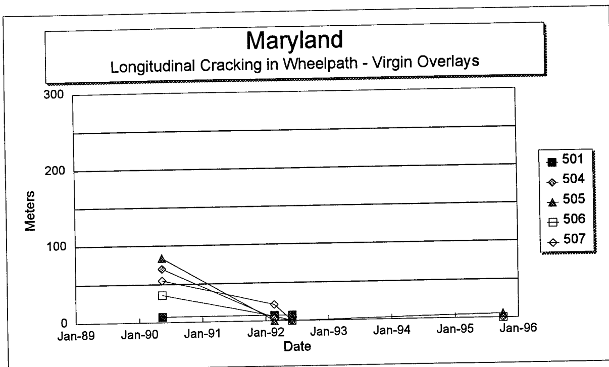
Figure 14. Total length of longitudinal cracking in the wheelpath versus time on each section of the Maryland SPS-5 project.
