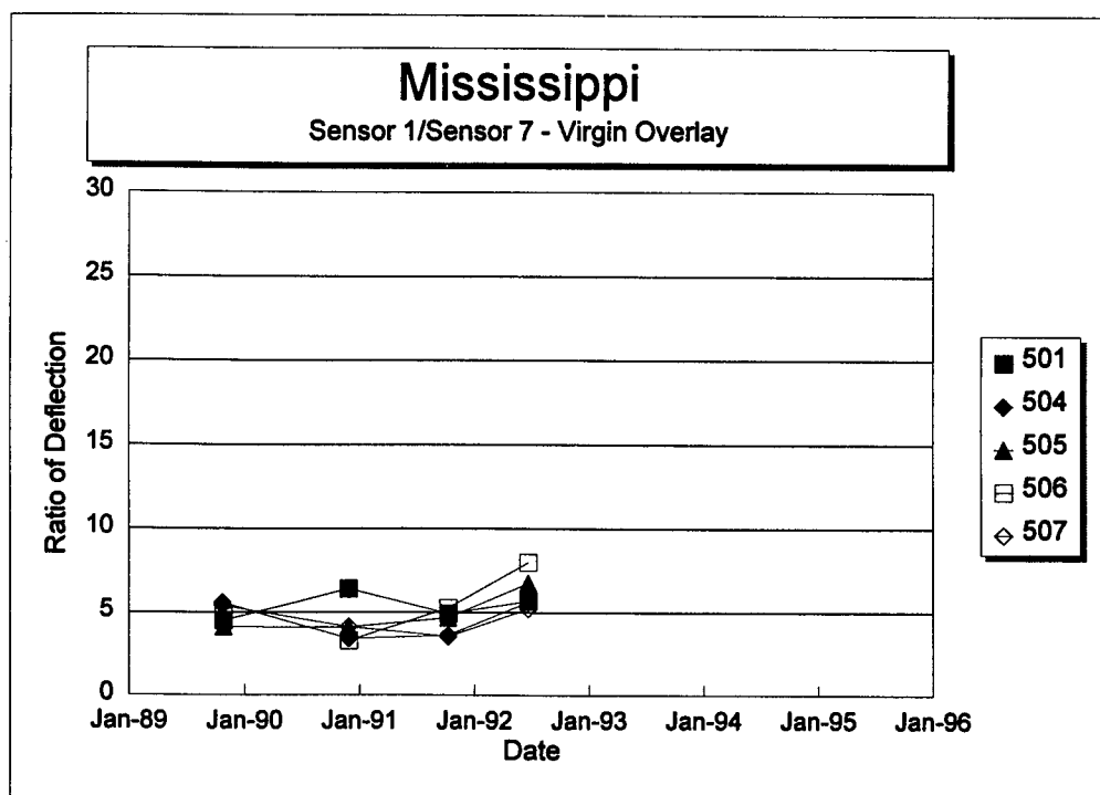
Figure 91. Sensor 1 deflection divided by Sensor 7 deflection versus time for each section of the Mississippi SPS-5 project.
