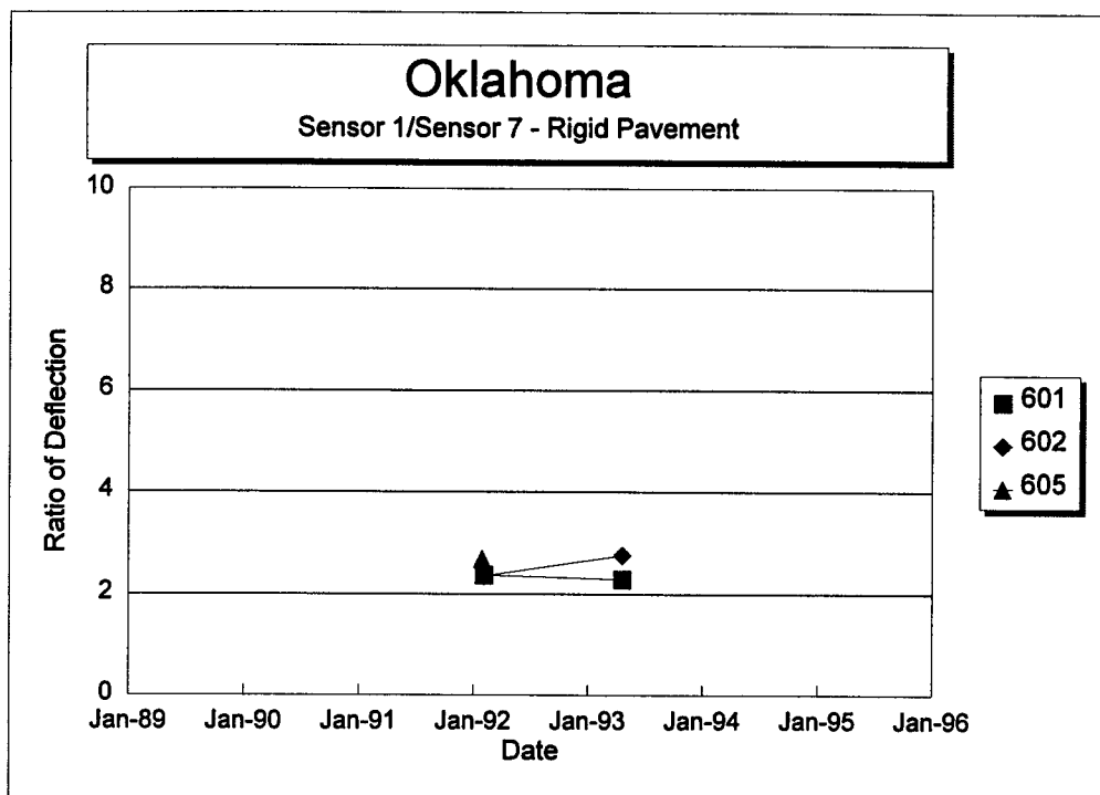
Figure 151. Sensor 1 deflection divided by Sensor 7 deflection versus time for each section of the Oklahoma SPS-6 project.
