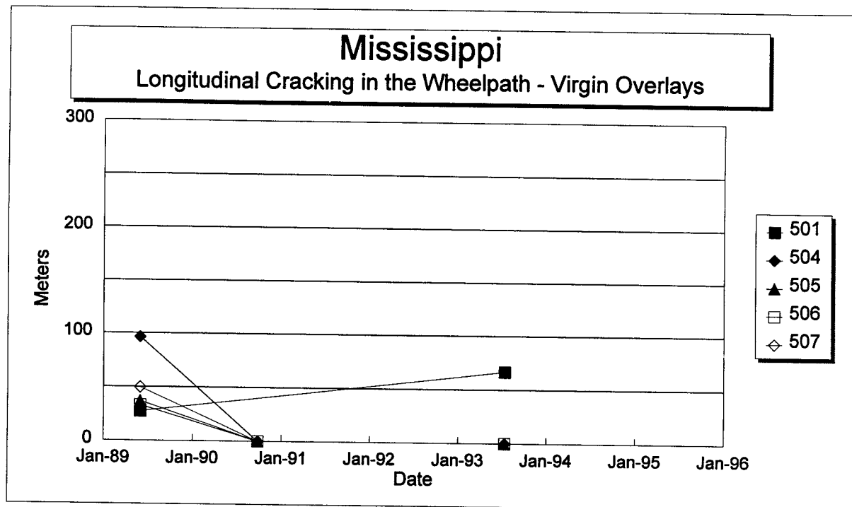
Figure 15. Total length of longitudinal cracking in the wheelpath versus time on each section of the Mississippi SPS-5 project.
