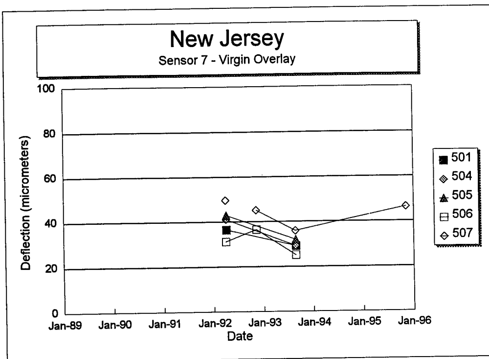
Figure 96. Sensor 7 deflection versus time for each section of the New Jersey SPS-5 project.
