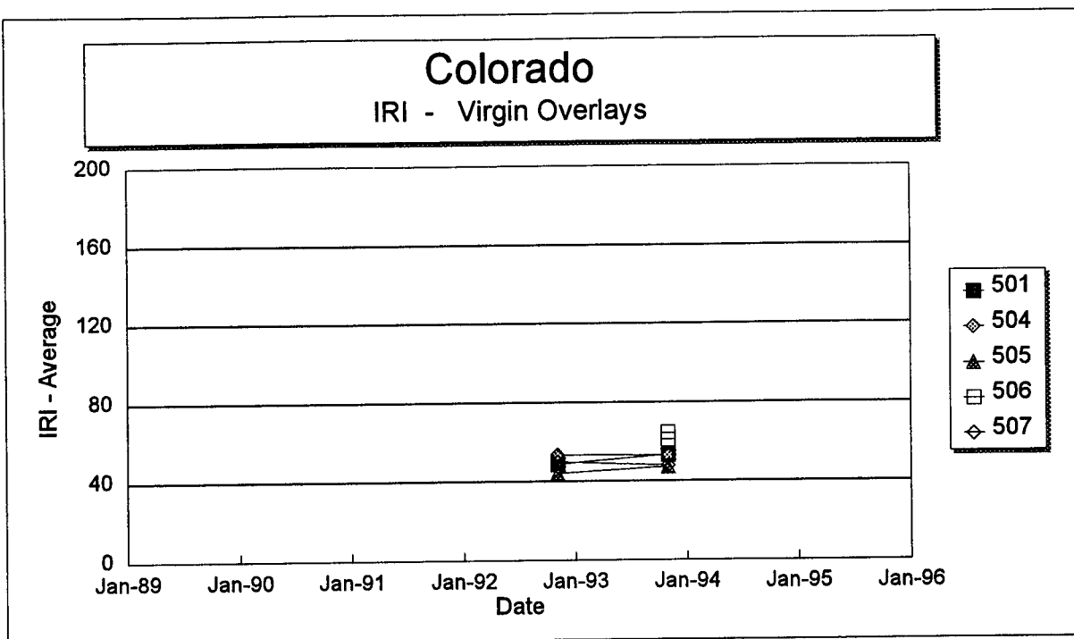
Figure 42. International Roughness Index versus time on each section of the Colorado SPS-5 project.
