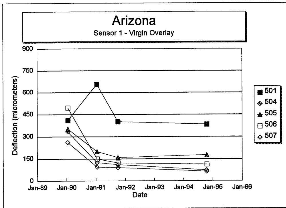
Figure 68. Sensor 1 deflection versus time for each section of the Arizona SPS-5 project.
