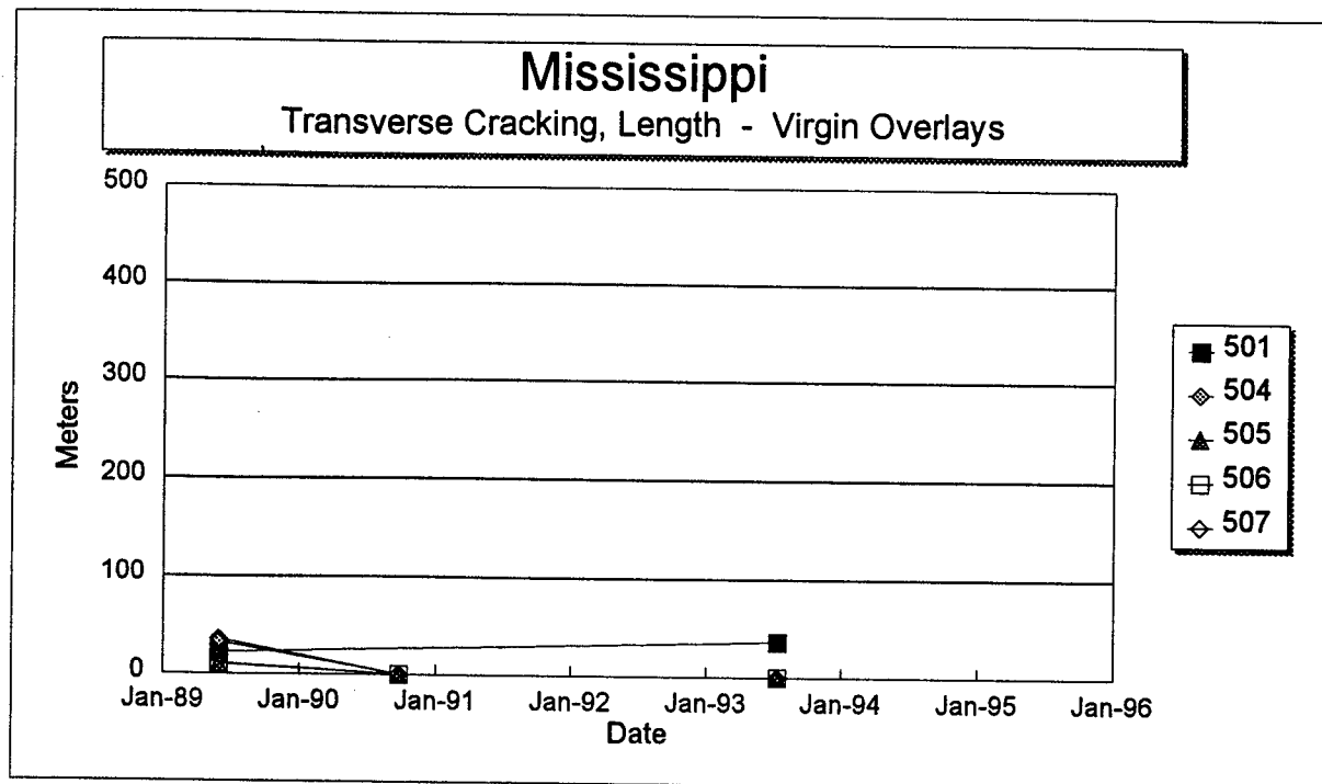
Figure 35. Total length of transverse cracks versus time on each section of the Mississippi SPS-5 project.
