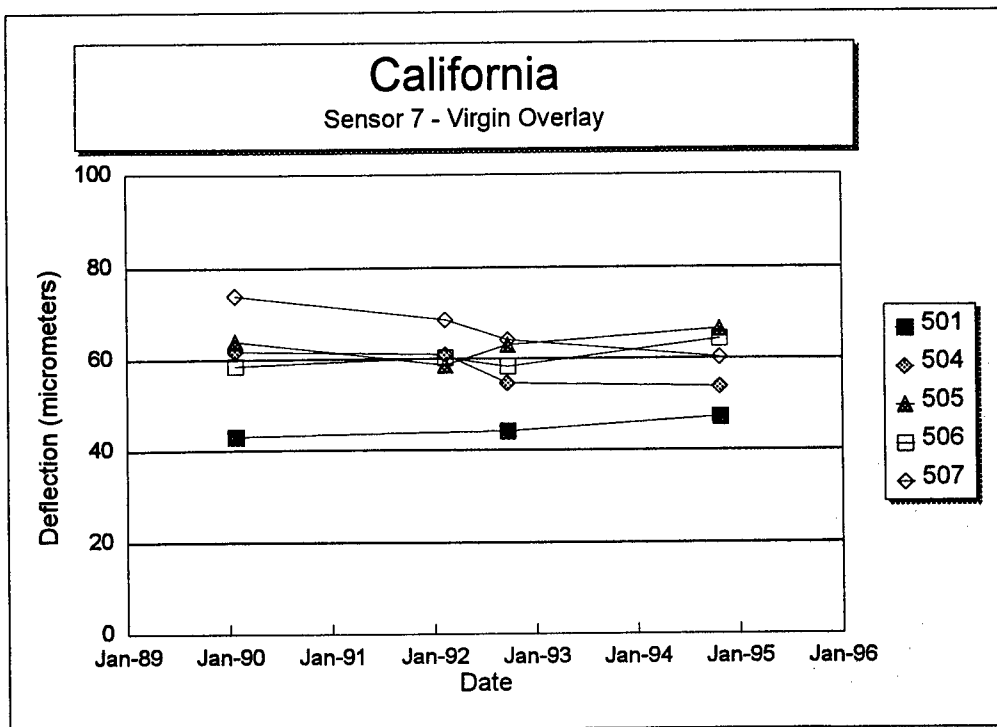
Figure 72. Sensor 7 deflection versus time for each section of the California SPS-5 project.
