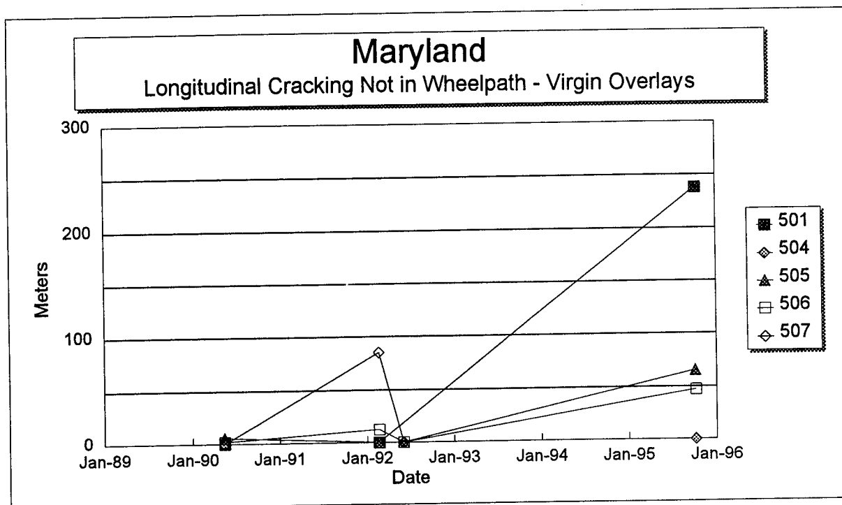
Figure 18. Total length of longitudinal cracking not in the wheelpath versus time on each section of the Maryland SPS-5 project.
