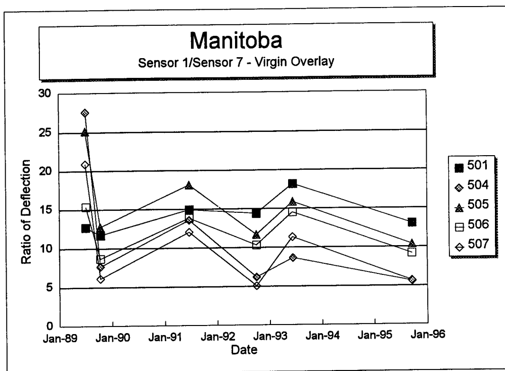
Figure 106. Sensor 1 deflection divided by Sensor 7 deflection versus time for each section of the Manitoba SPS-5 project.
