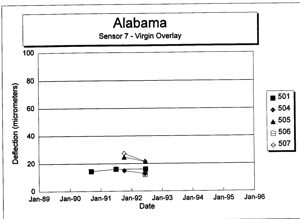
Figure 66. Sensor 7 deflection versus time for each section of the Alabama SPS-5 project.
