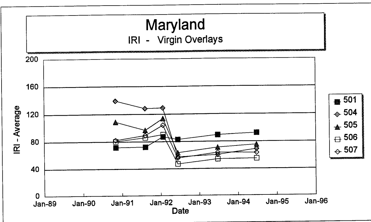
Figure 44. International Roughness Index versus time on each section of the Maryland SPS-5 project.
