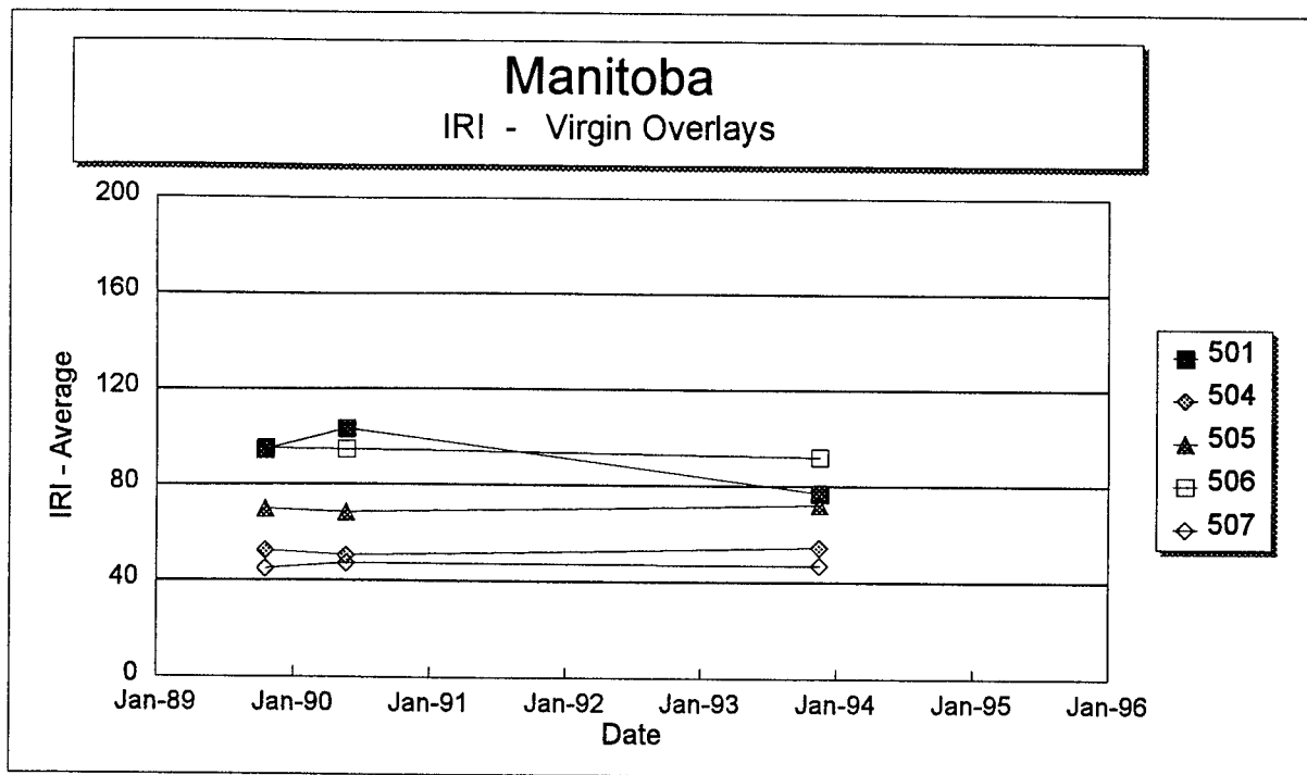
Figure 51. International Roughness Index versus time on each section of the Manitoba SPS-5 project.
