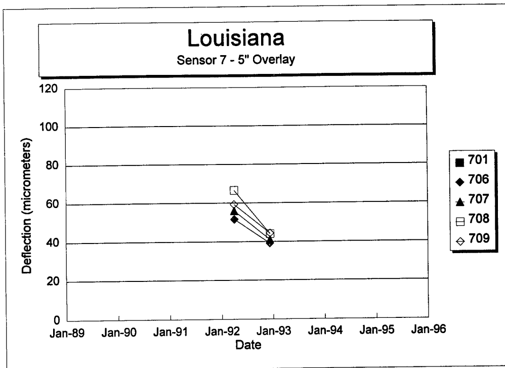
Figure 172. Sensor 7 deflection versus time for each section of the Louisiana SPS-7 project.
