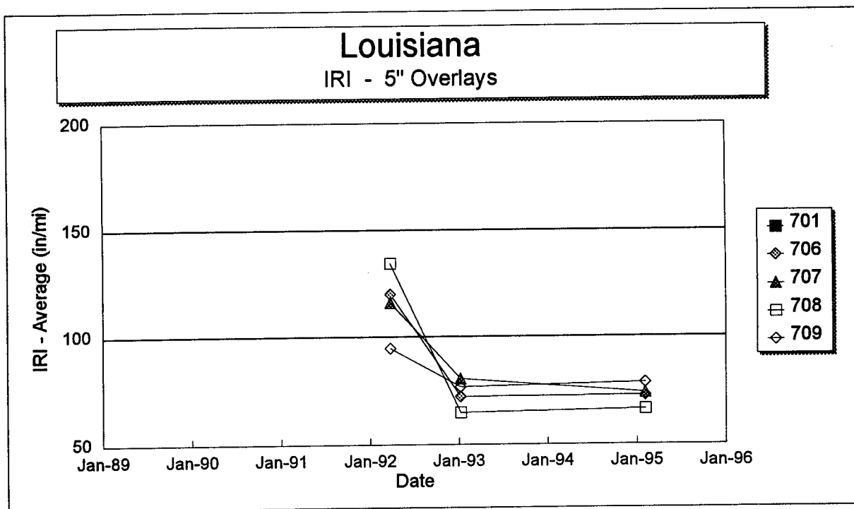
Figure 166. International Roughness Index versus time on each section of the Louisiana SPS-7 project.
