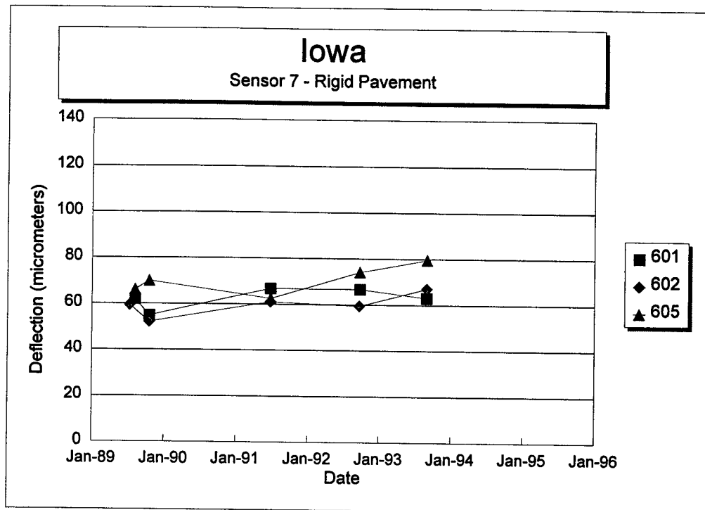
Figure 141. Sensor 7 deflection versus time for each section of the Iowa SPS-6 project.
