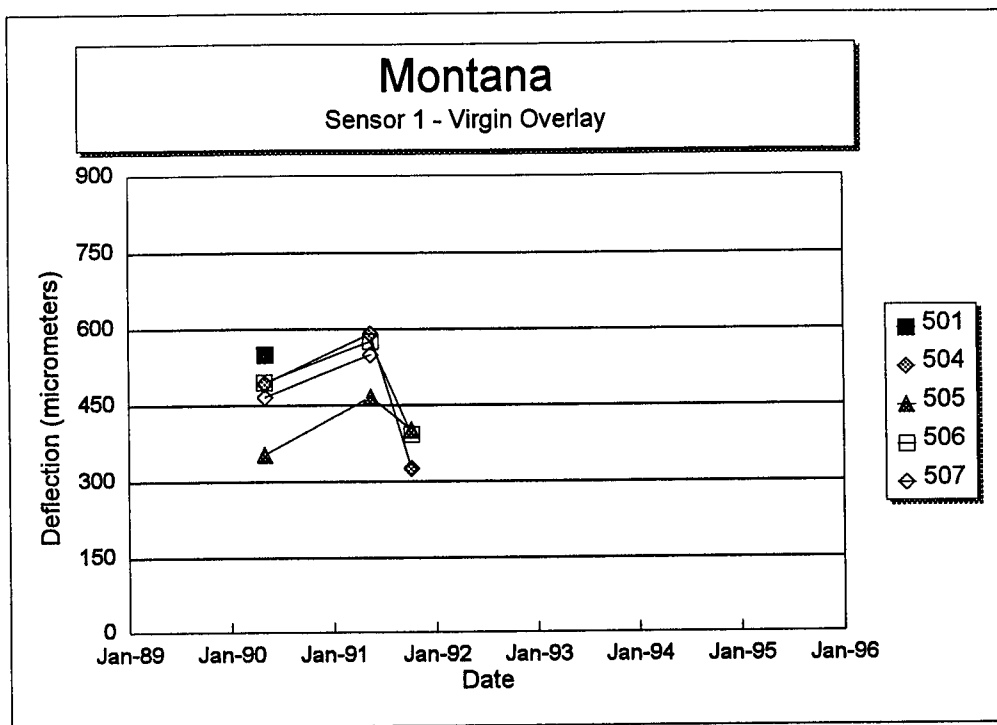
Figure 92. Sensor 1 deflection versus time for each section of the Montana SPS-5 project.
