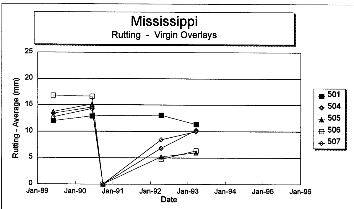
Figure 59. Rut depth versus time on each section of the Mississippi SPS-5 project.
