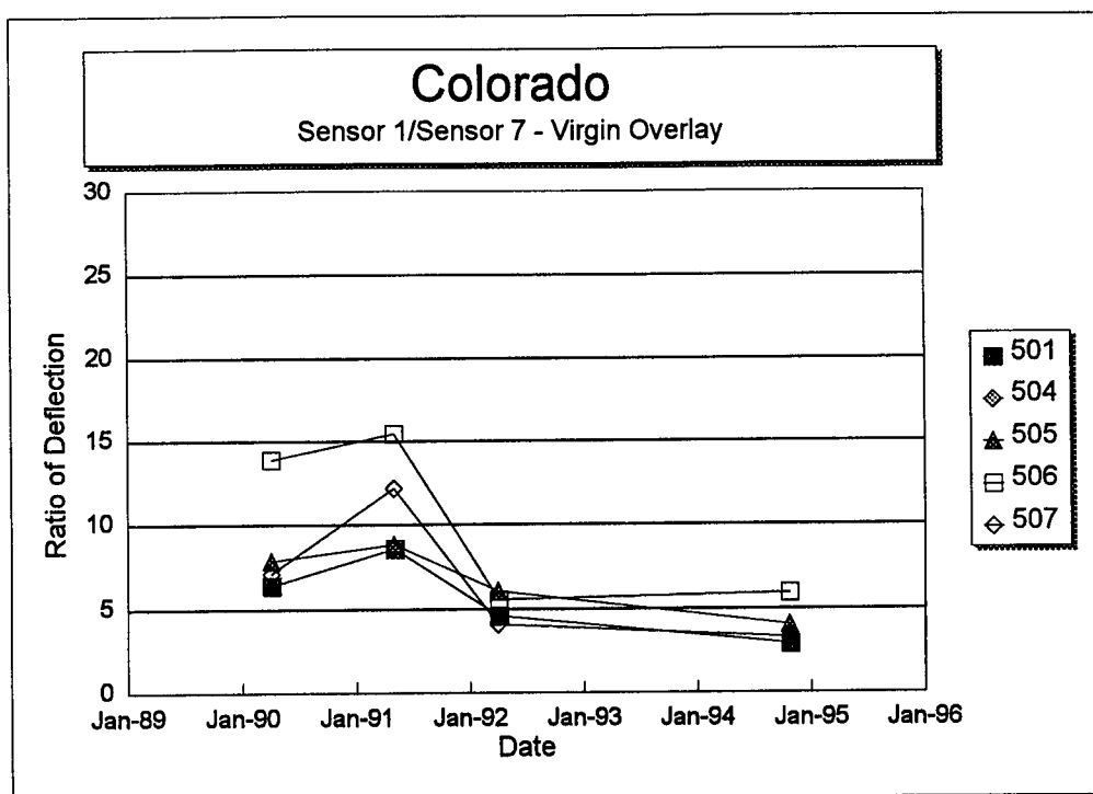
Figure 76. Sensor 1 deflection divided by Sensor 7 deflection versus time for each section of the Colorado SPS-5 project.
