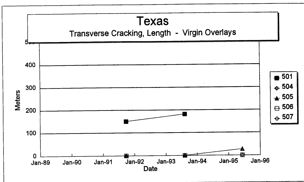
Figure 36. Total length of transverse cracks versus time on each section of the Texas SPS-5 project.
