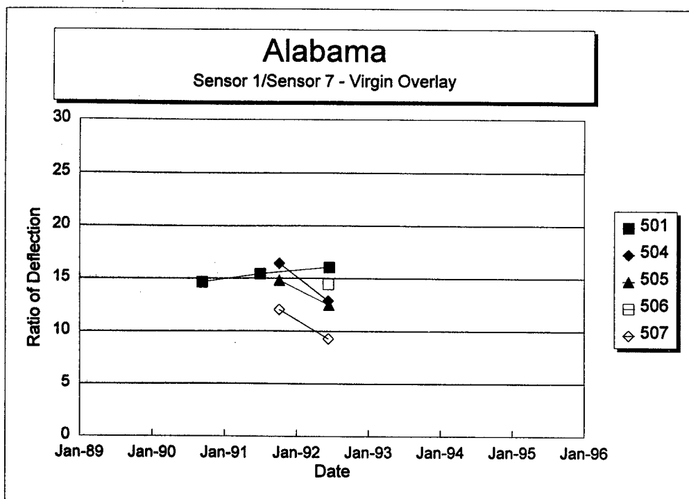
Figure 67. Sensor 1 deflection divided by Sensor 7 deflection versus time for each section of the Alabama SPS-5 project.
