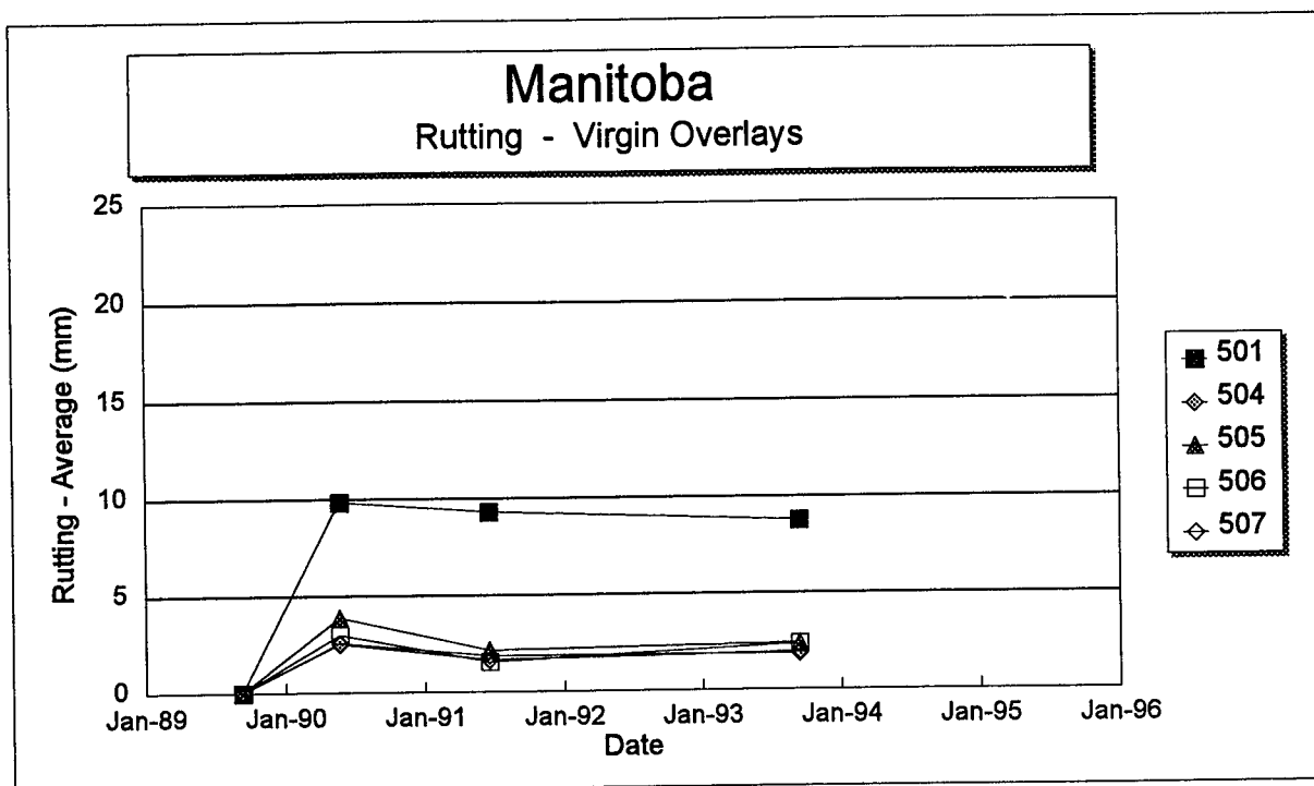
Figure 64. Rut depth versus time on each section of the Manitoba SPS-5 project.
