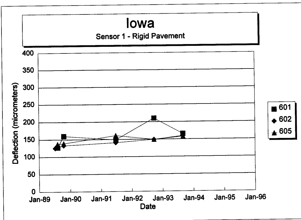
Figure 140. Sensor 1 deflection versus time for each section of the Iowa SPS-6 project.
