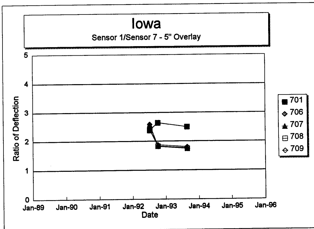
Figure 170. Sensor 1 deflection divided by Sensor 7 deflection versus time for each section of the Iowa SPS-7 project.
