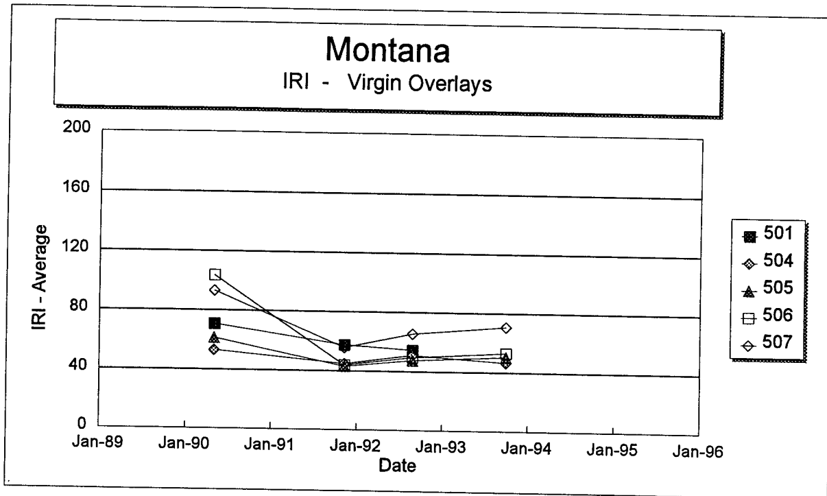
Figure 47. International Roughness Index versus time on each section of the Montana SPS-5 project.
