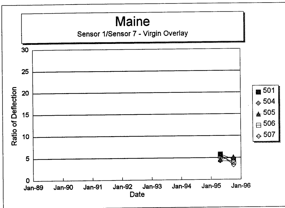
Figure 82. Sensor 1 deflection divided by Sensor 7 deflection versus time for each section of the Maine SPS-5 project.
