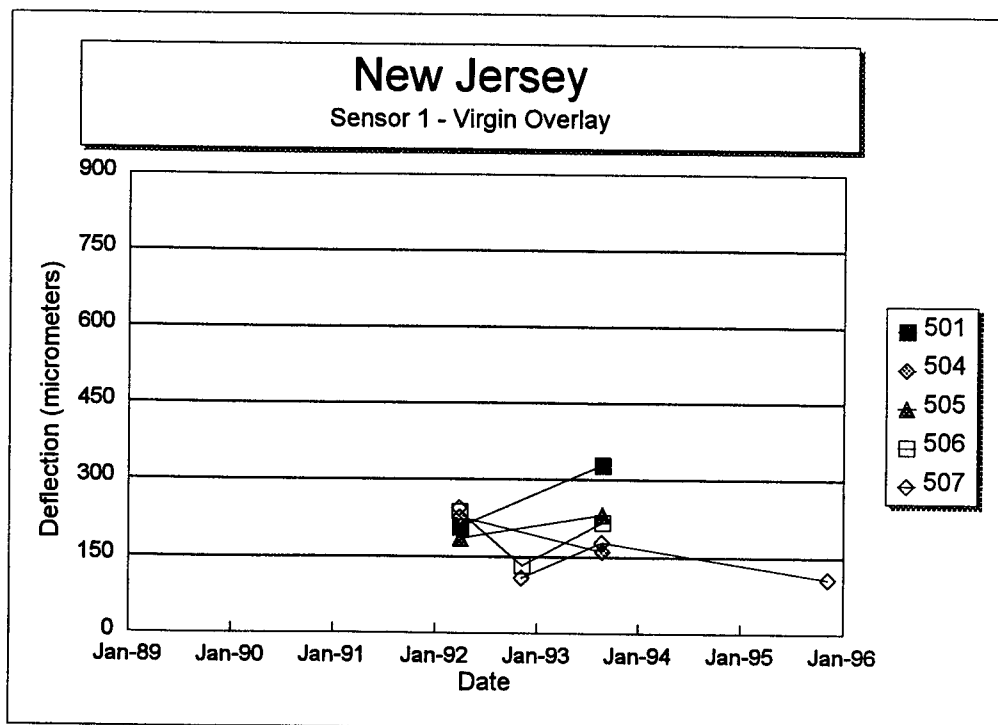
Figure 95. Sensor 1 deflection versus time for each section of the New Jersey SPS-5 project.
