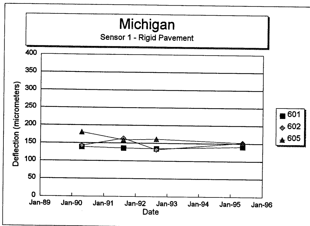
Figure 143. Sensor 1 deflection versus time for each section of the Michigan SPS-6 project.
