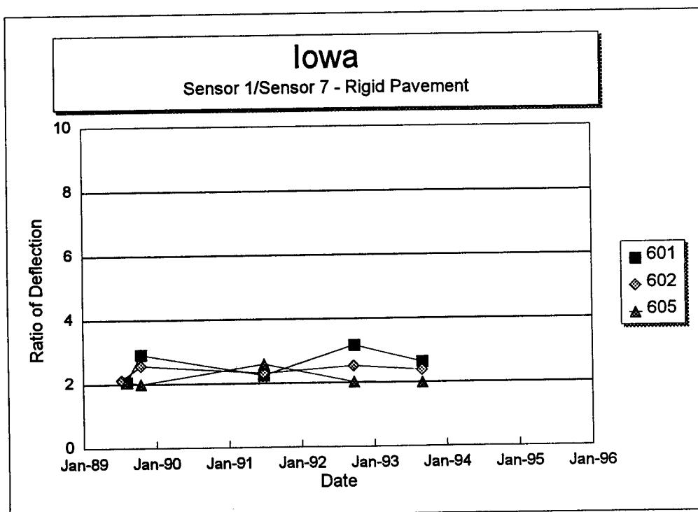
Figure 142. Sensor 1 deflection divided by Sensor 7 deflection versus time for each section of the Iowa SPS-6 project.
