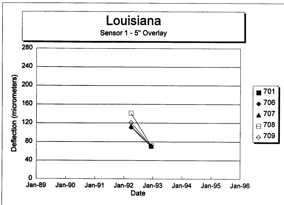
Figure 171. Sensor 1 deflection versus time for each section of the Louisiana SPS-7 project.
