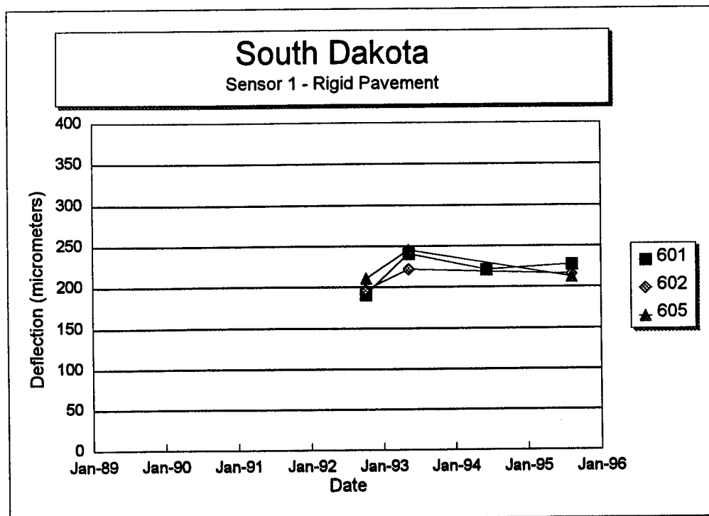
Figure 152. Sensor 1 deflection versus time for each section of the South Dakota SPS-6 project.
