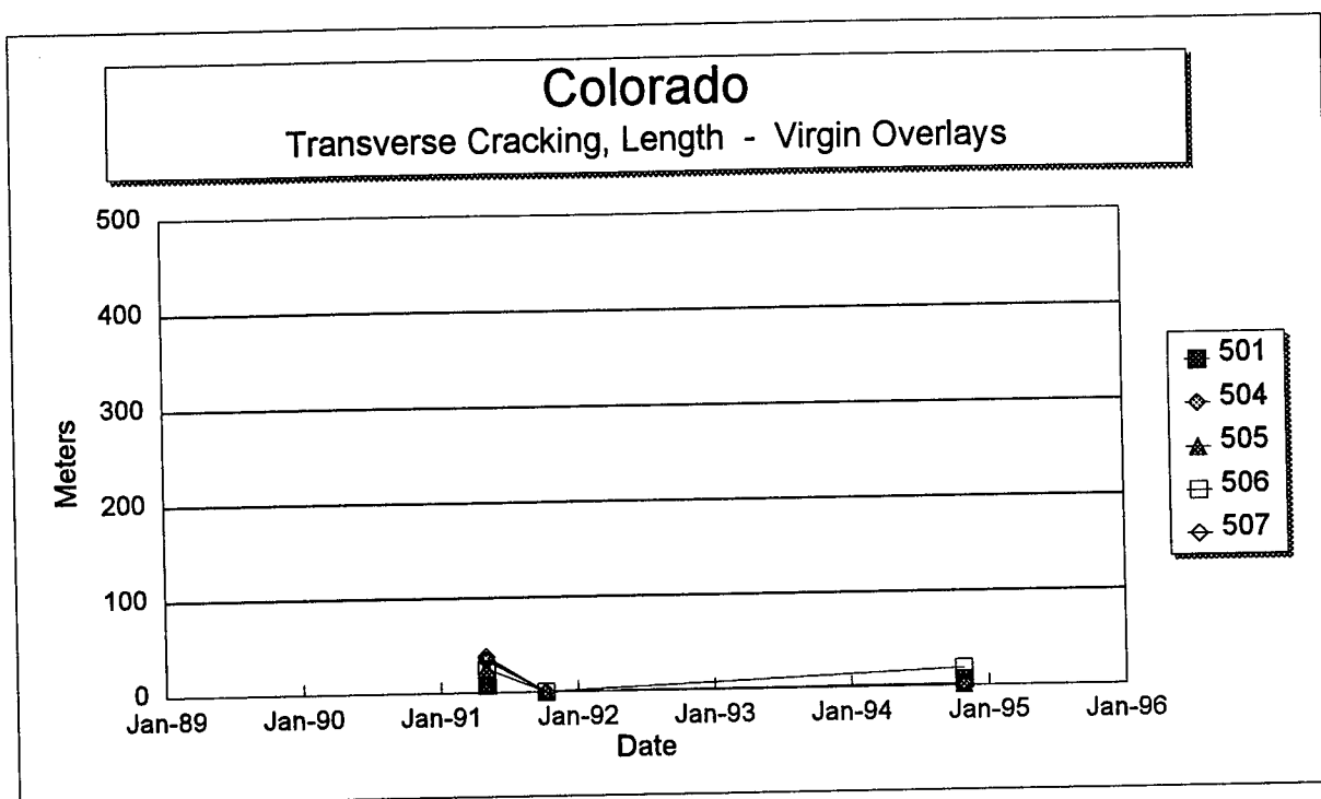
Figure 32. Total length of transverse cracks versus time on each section of the Colorado SPS-5 project.
