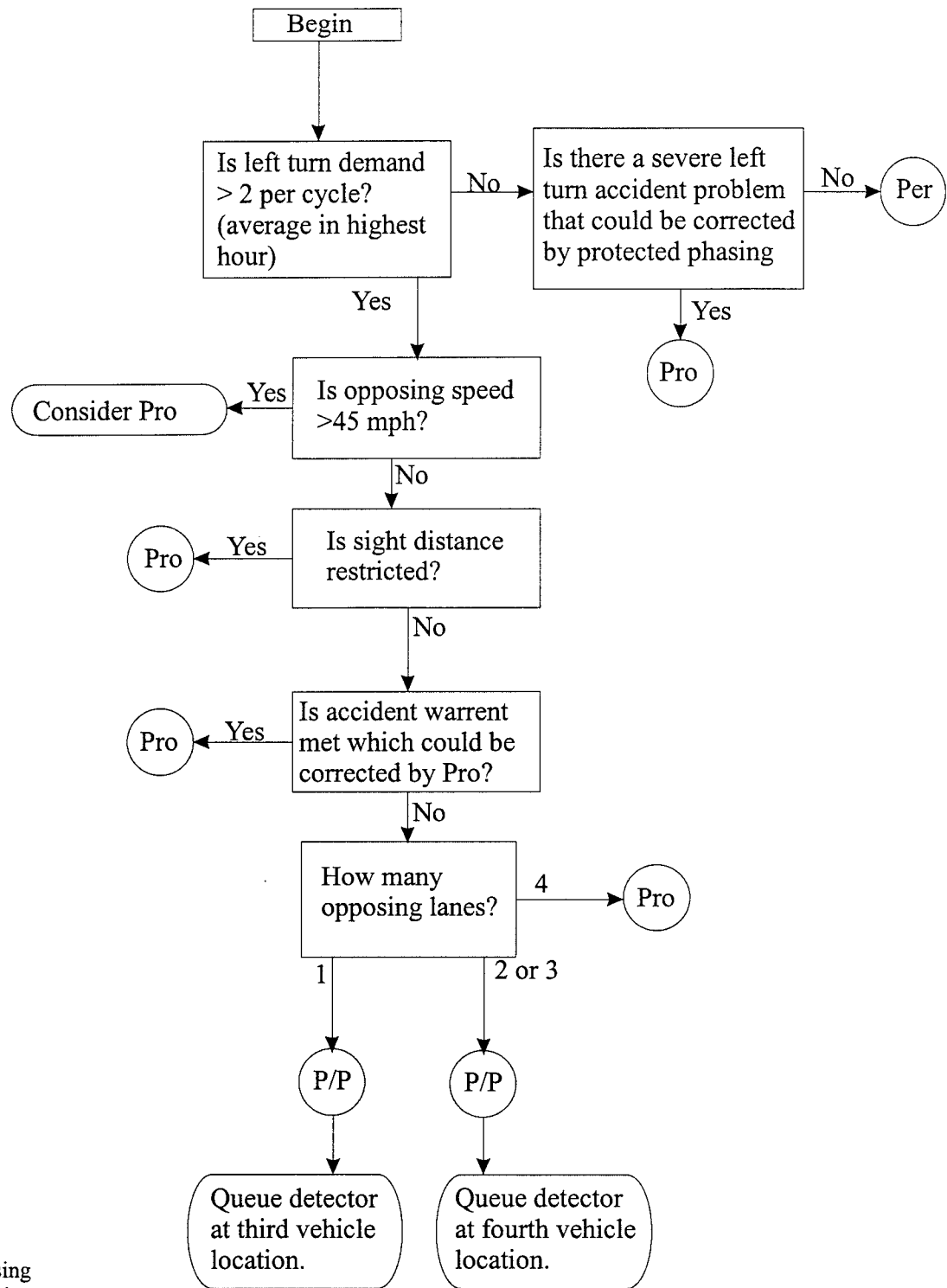
Figure 6.1 Flowchart of Left-Turn Phasing Guidelines
