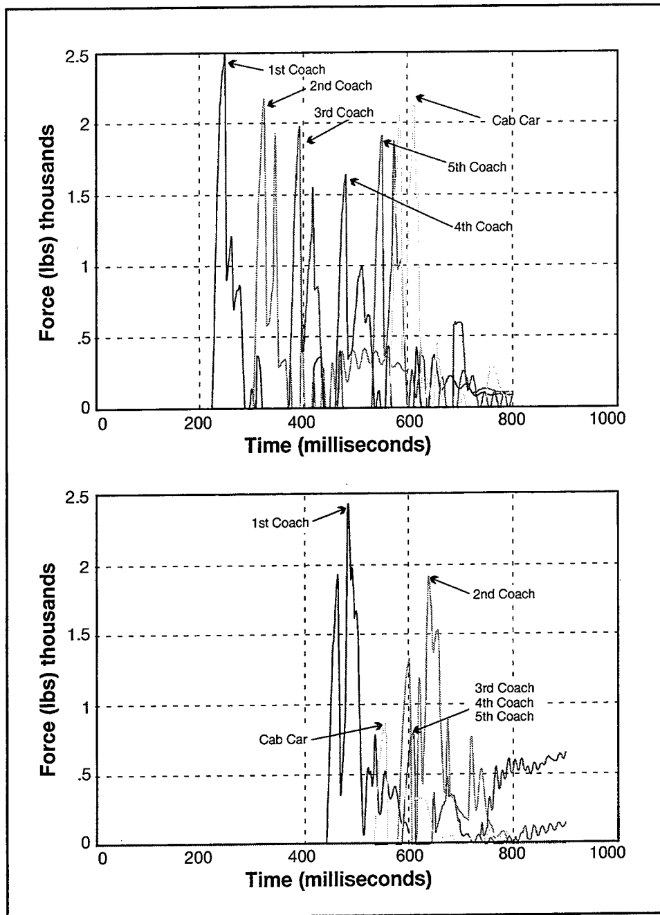
Figure 3-24. Forces on Forward Seat Back Due to Unrestrained Occupant (by Car)
