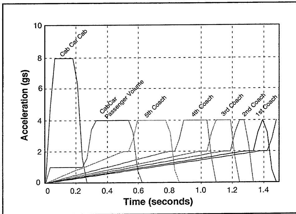
Figure A-15. Power Car, Five Coach, Cab Car Consist Deceleration Characteristic, 30 mph Brick Wall Collision, Cab Car Leading
