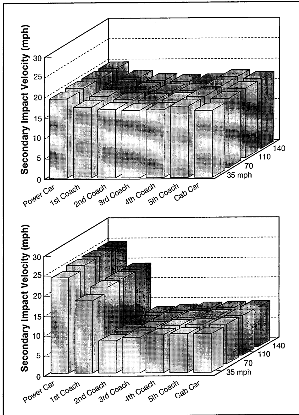
Figure 2-31. Bar Chart of Occupant Secondary Impact Velocity, Power Car to Commuter MU, Intercity Passenger Train
