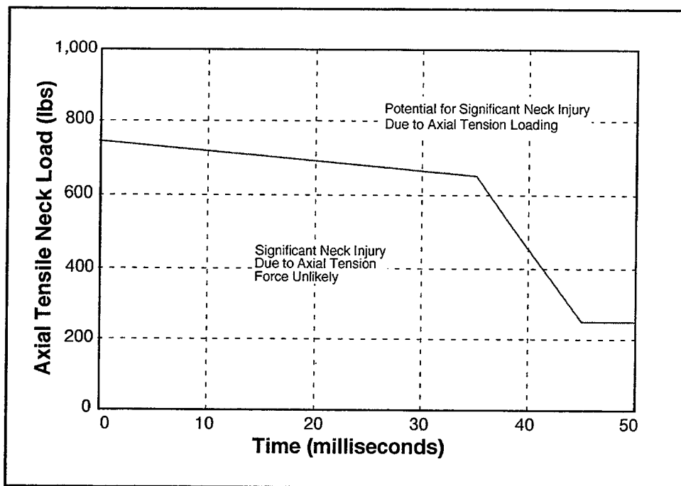
Figure 3-11. Injury Criteria for Tensile Neck Loads
