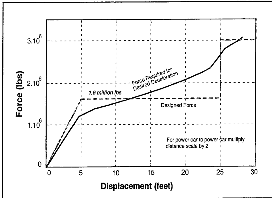
Figure A-11. Power Car to Brick Wall Crush Zones Force/Crush Characteristic Required to Ensure Occupant Survival in 140 mph Train-to-Train Collision
