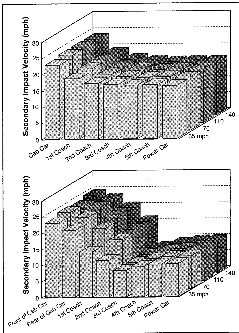
Figure 2-37. Bar Chart of Occupant Secondary Impact Velocity, Cab Car to Commuter MU, Intercity Passenger Train
