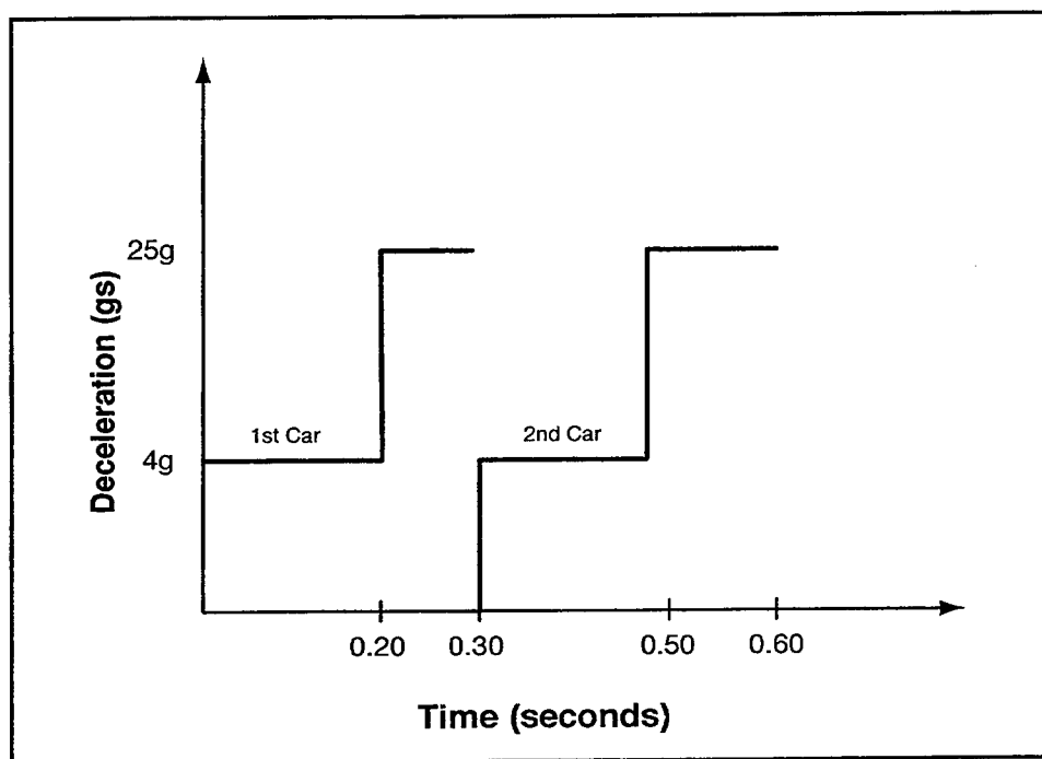
Figure A-4. Ideal Deceleration Characteristic
