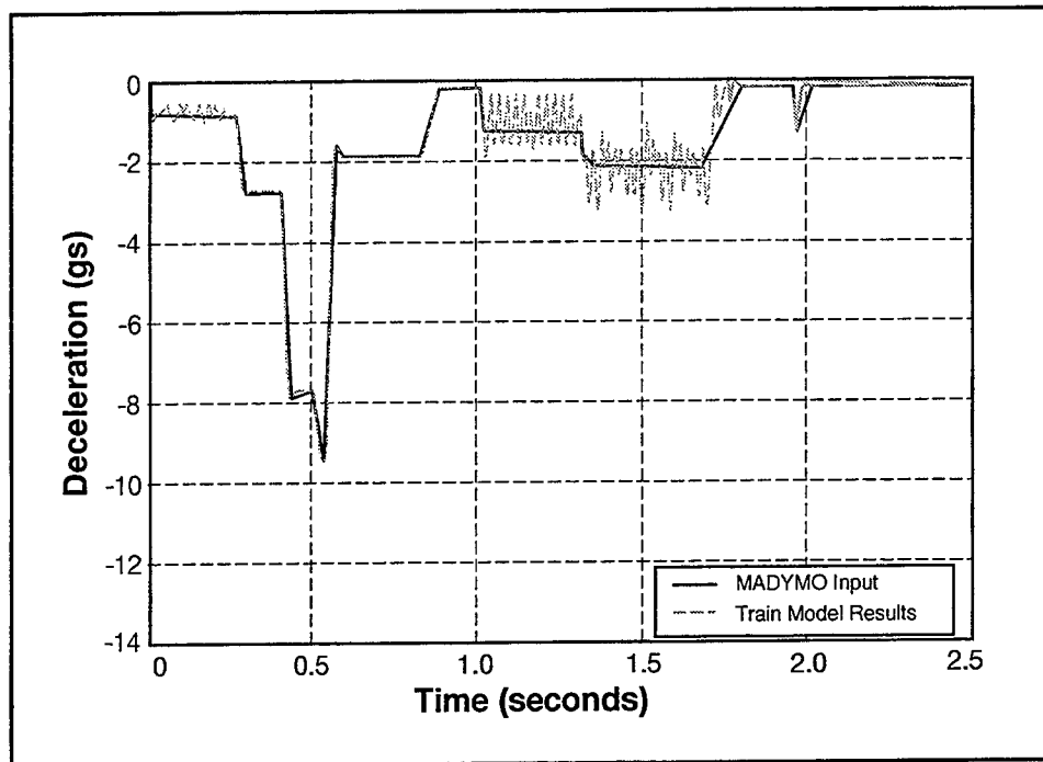
Figure 3-9. Crash Pulse, First Coach, 140 mph Power Car-to-Power Car Collision, Crash-Energy Management Design, MADYMO Input and Train Model Results
