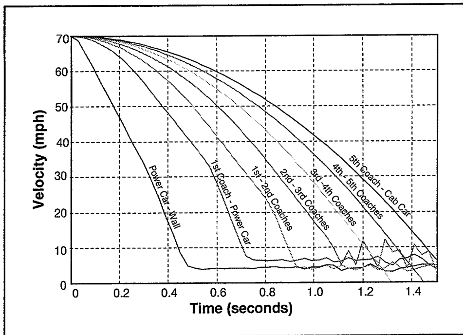
Figure A-9. Velocity Versus Time for All Cars
