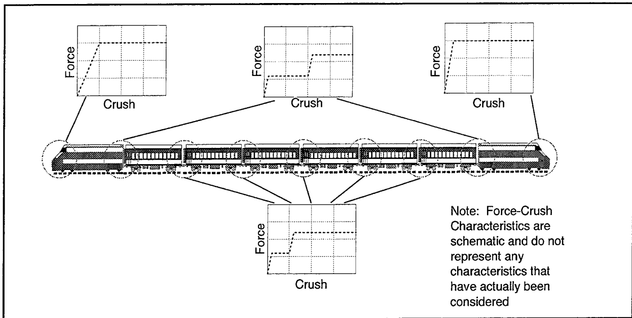
Figure 2-1. Structural Crashworthiness Analysis Model
