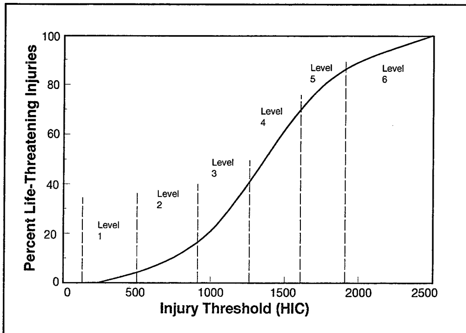
Figure 3-10. Probability of Fatality Versus Head Injury Criteria [21]
