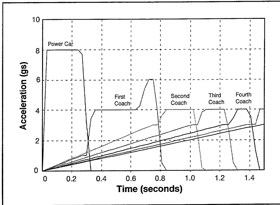
Figure A-14. Power Car, Five Coach, Cab Car Consist Deceleration Characteristic, 45 mph Brick Wall Collision, Power Car Leading
