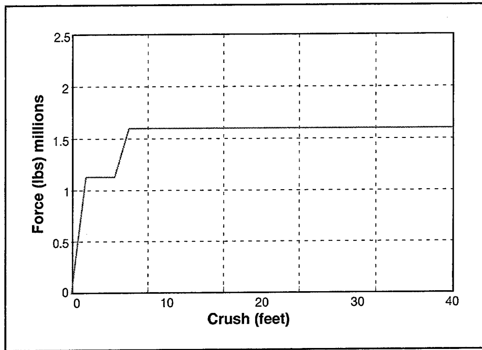
Figure 2-10. Commuter MU Train Car-to-Car Crush Characteristic
