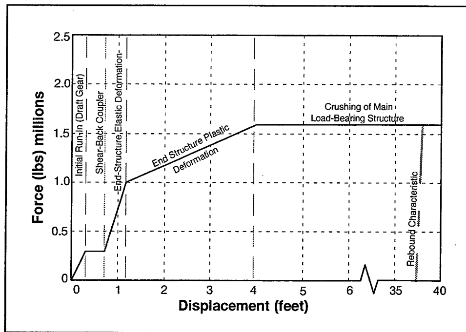
Figure 2-6. Conventional Design Car-to-Car Crush Characteristics
