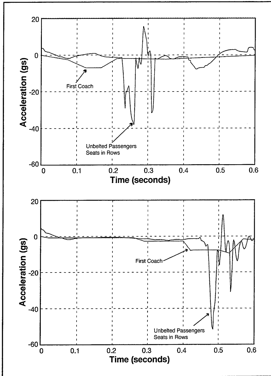
Figure 3-17. Unrestrained Passenger and Vehicle Decelerations, 140 mph Power Car-to-Power Car Collision
