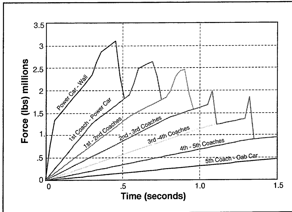
Figure A-8. Force Versus Time for All Cars
