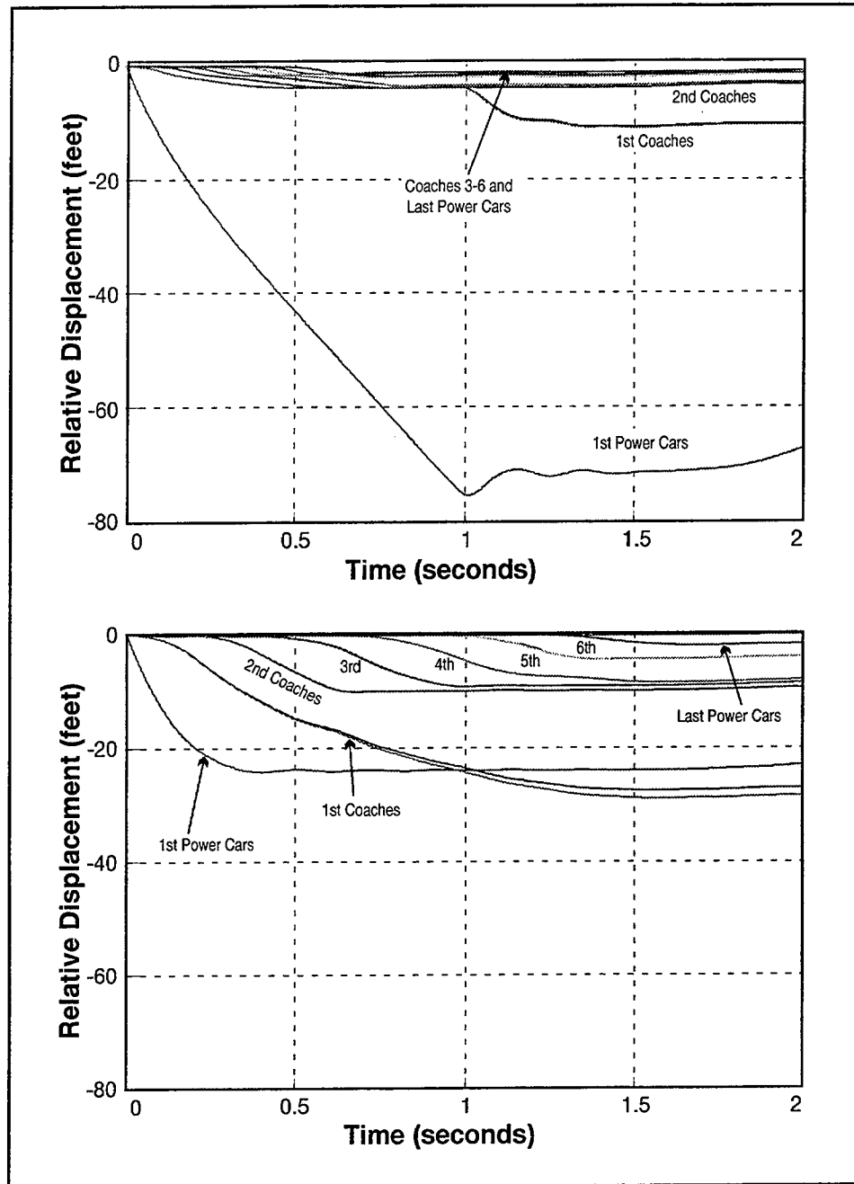
Figure 2-13. Relative Displacement Time Histories, Each Car in the Consist, 100 mph Closing Speed
