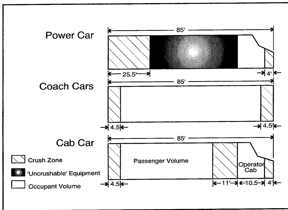
Figure A-1. Crash-Energy Management Design Crush-Zone Locations
