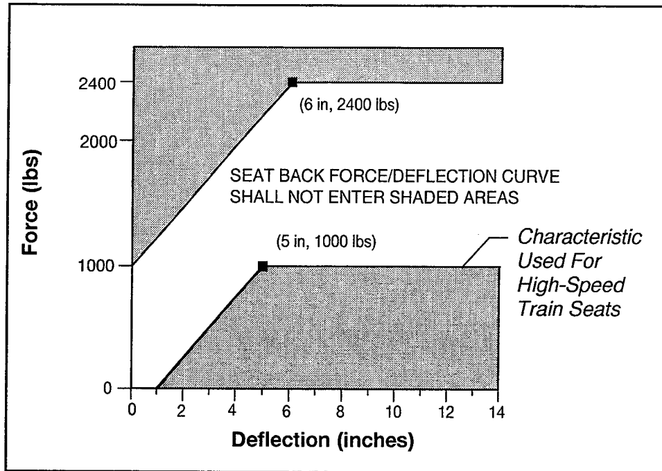
Figure 3-4. Force/Deflection Characteristic of Seat Back
