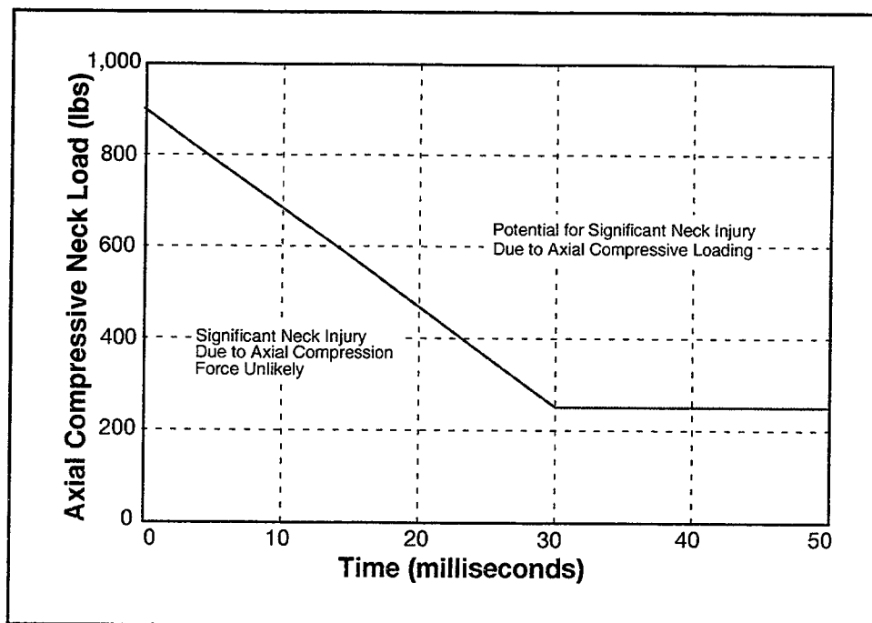
Figure 3-12. Injury Criteria for Compressive Neck Loads
