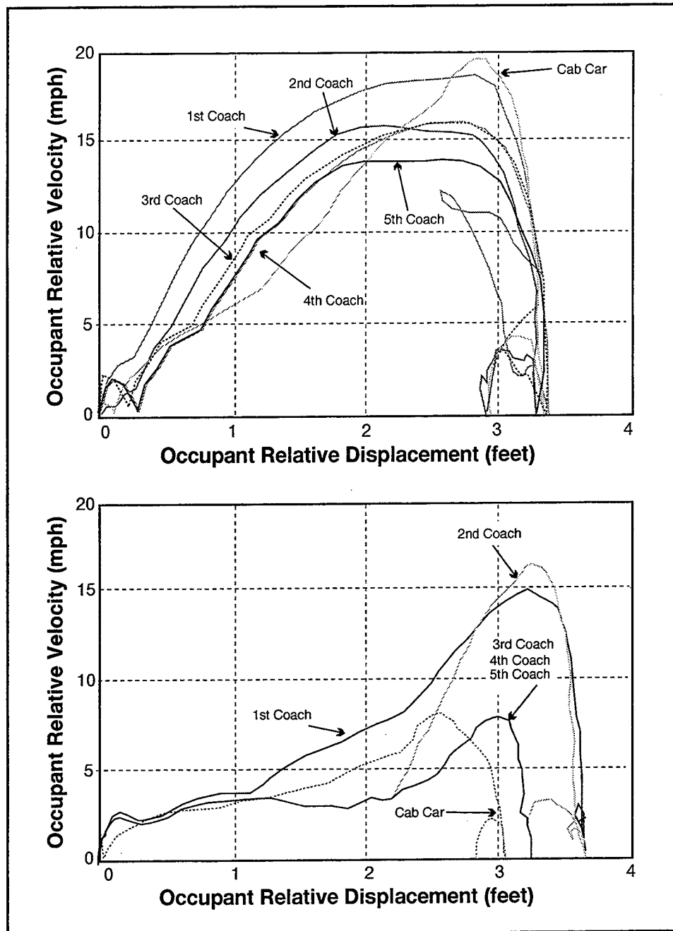
Figure 3-19. Secondary Impact Velocities for Occupants by Passenger Car
