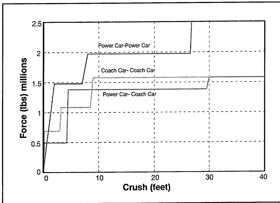
Figure 2-7. Car-to-Car Crush Characteristics, Power Car, Six Coach, Power Car Consist
