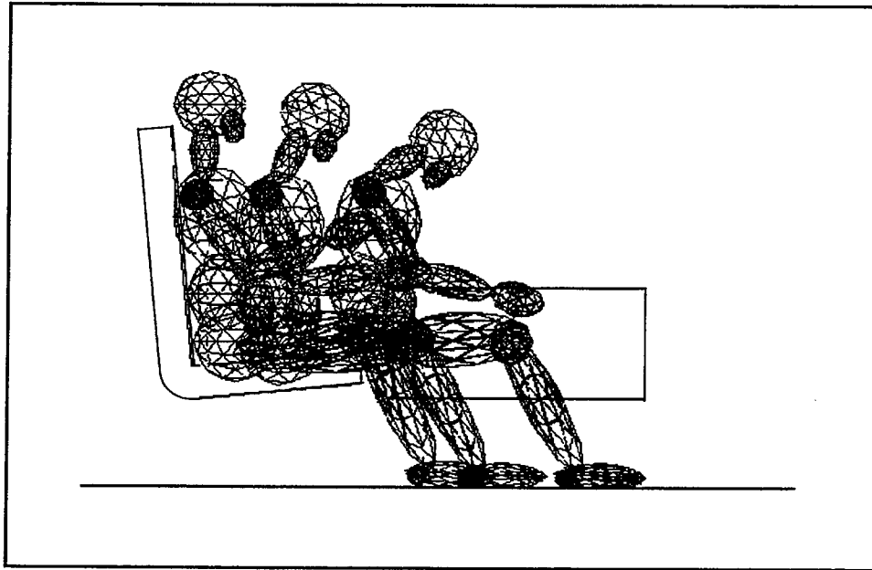
Figure 3-29. Motions for Occupants in Seats and Table Interior
