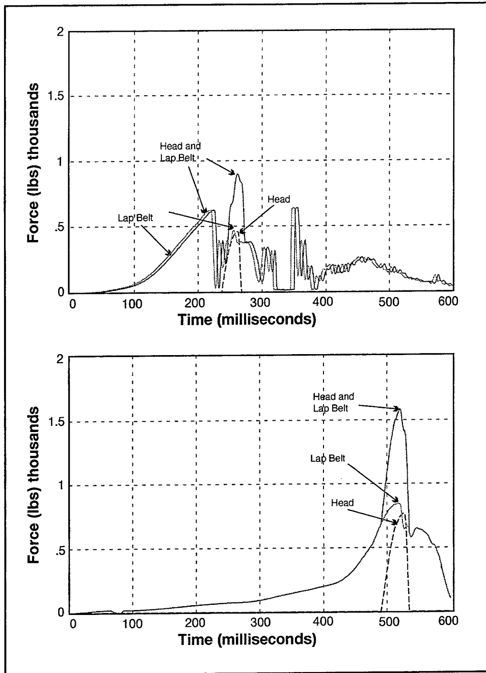
Figure 3-26. Forces on Seat Due to Restrained Occupant in First Coach Car
