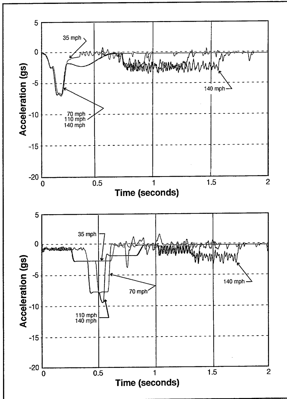
Figure 3-7. Influence of Speed on First Coach Crash Pulse, 140 mph Power Car-to-Power Car Collision
