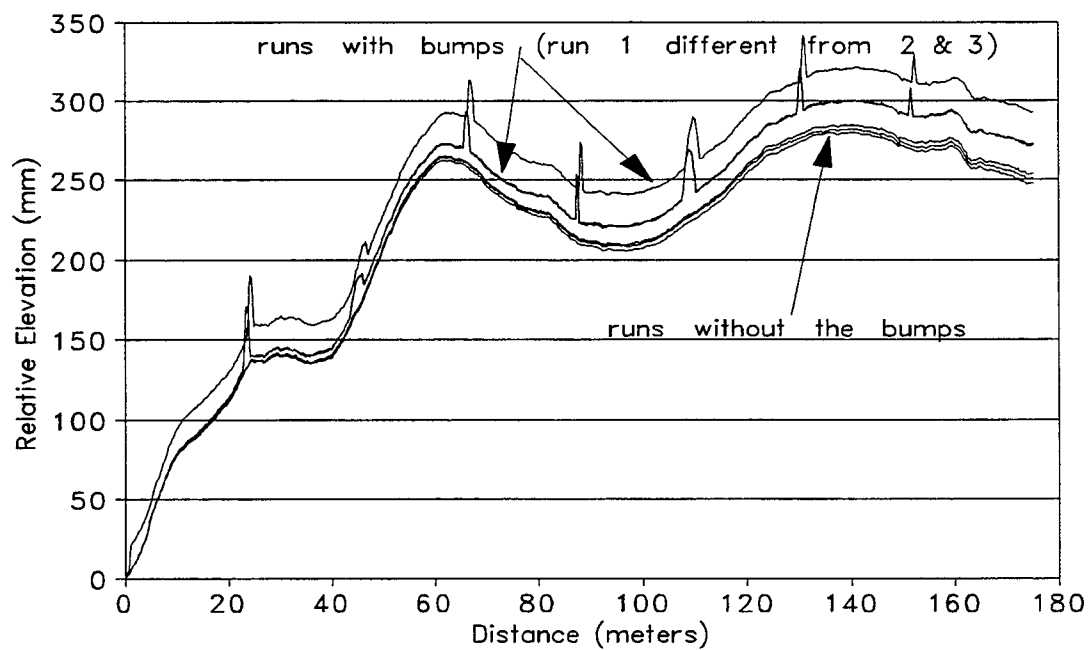
Figure 59. Profiles Measured on Annex 2 with and Without the Simulated Bumps Using the Walking Profiler.
