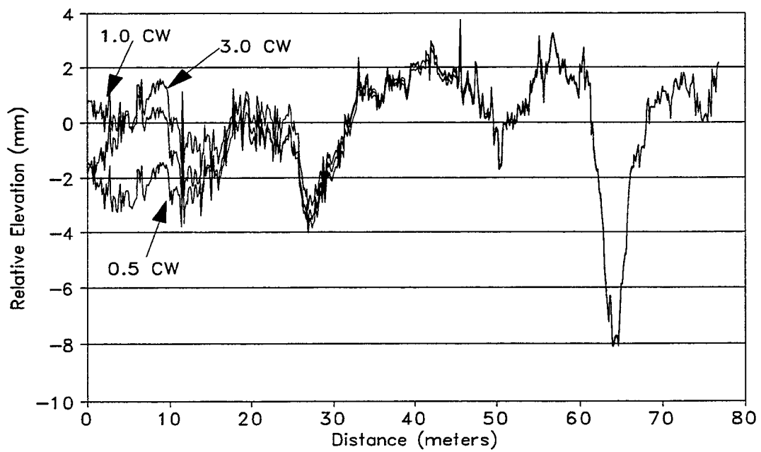
Figure B9. Comparison of Filtered Profiles Determined with Lead-ins of 0.5, 1.0, and 3.0 CW Using Rod & Level Data on Annex 2.
