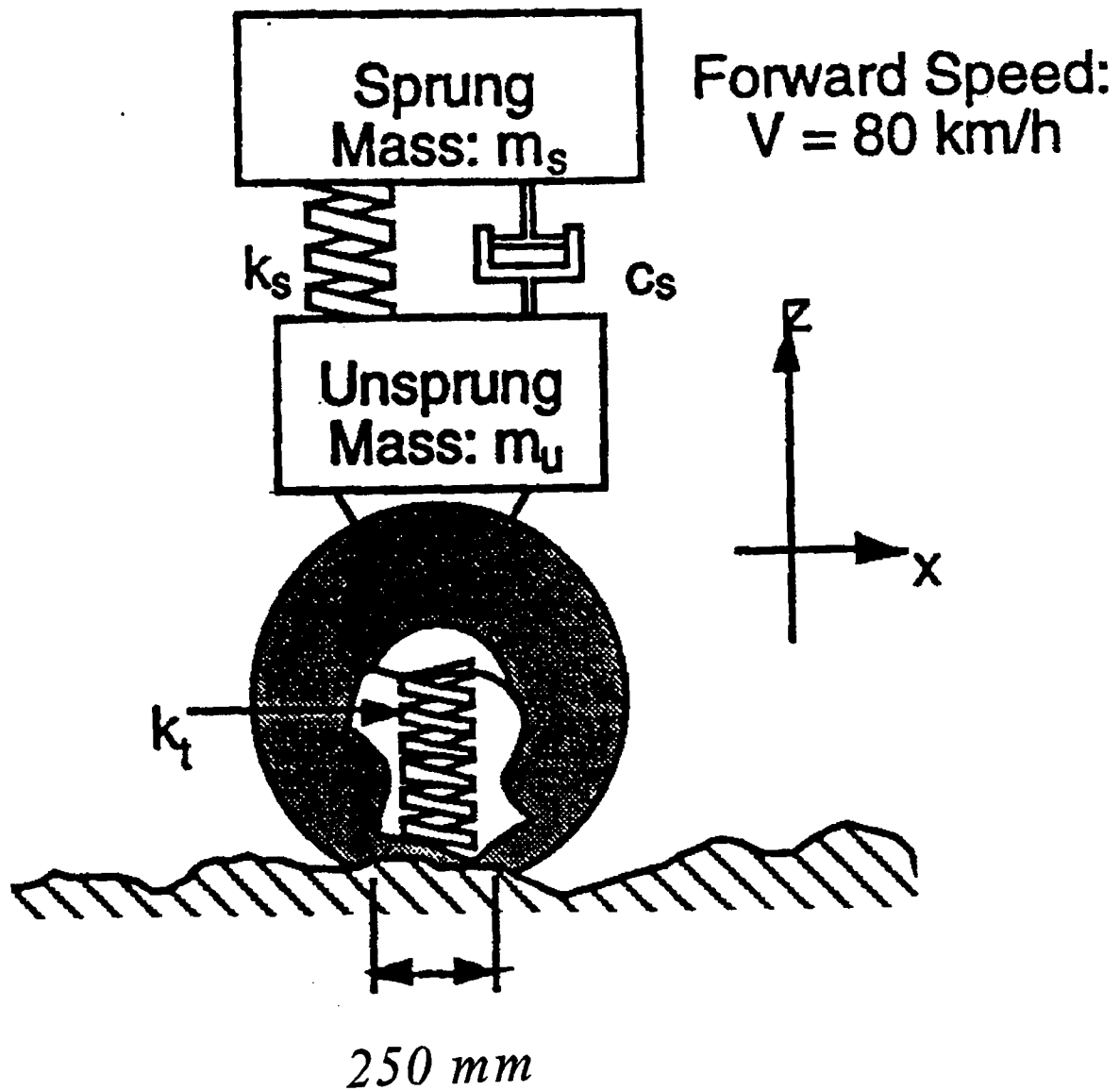
Figure 16. The Quarter Car Model (Sayers, 1995).
