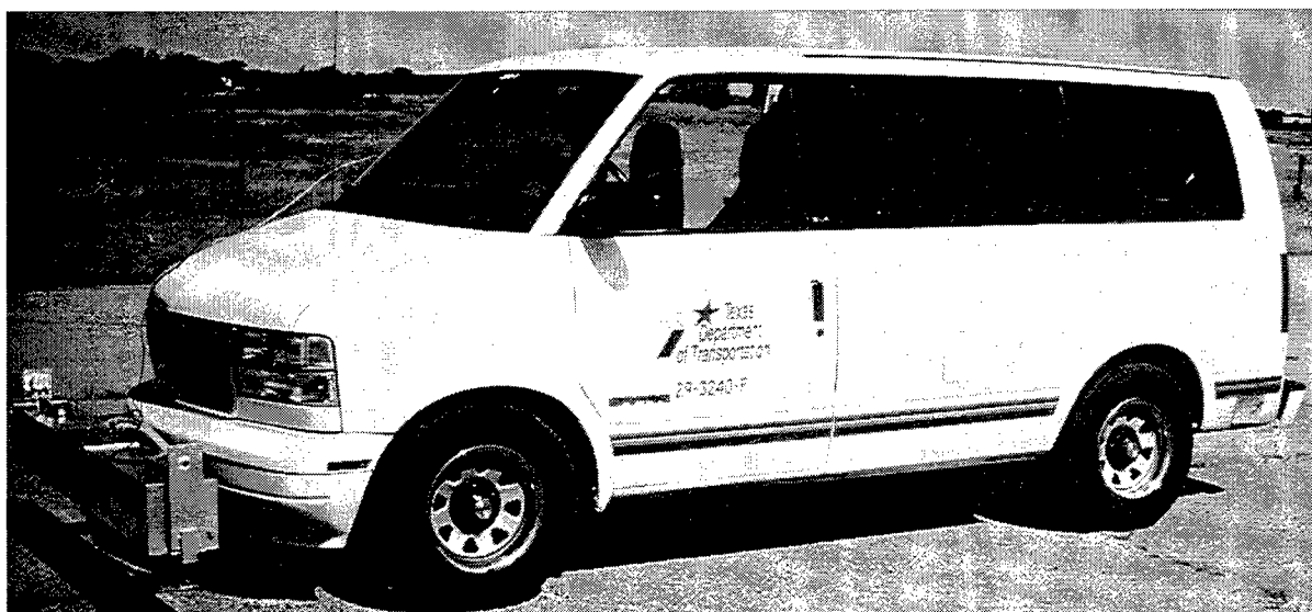
Figure 9. The Laser Rut/Profiler Developed by TxDOT.
