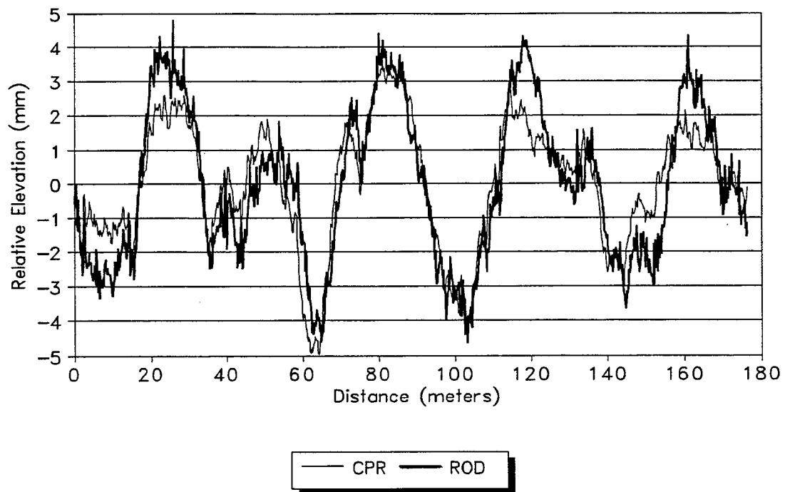
Figure 51. Average Synchronized CPR Profile vs Average Filtered Rod & Level Profile (SH47A).
