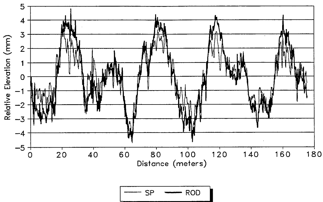
Figure 57. Average Synchronized Profile from Surface Profiler vs Average Filtered Rod & Level Profile (SH47A).
