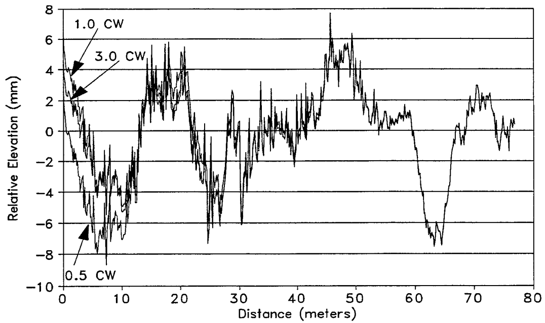
Figure B7. Comparison of Filtered Profiles Determined with Lead-ins of 0.5, 1.0, and 3.0 CW Using Rod & Level Data on Annex 1.
