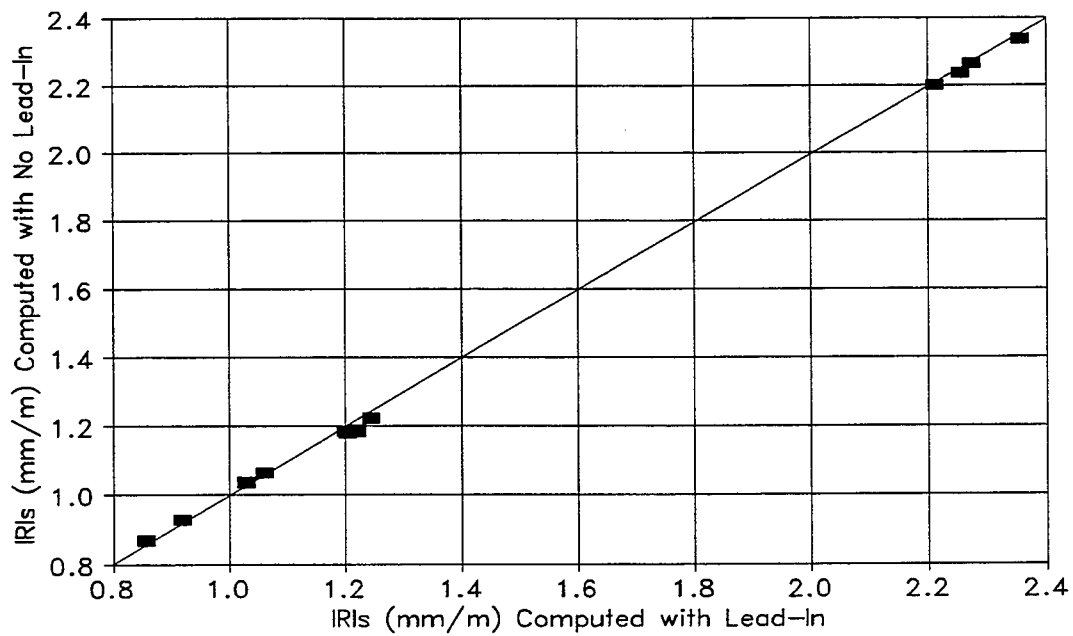
Figure B16. Comparison of IRIs Computed from Filtered Profiles Determined with and Without a Lead-in.
