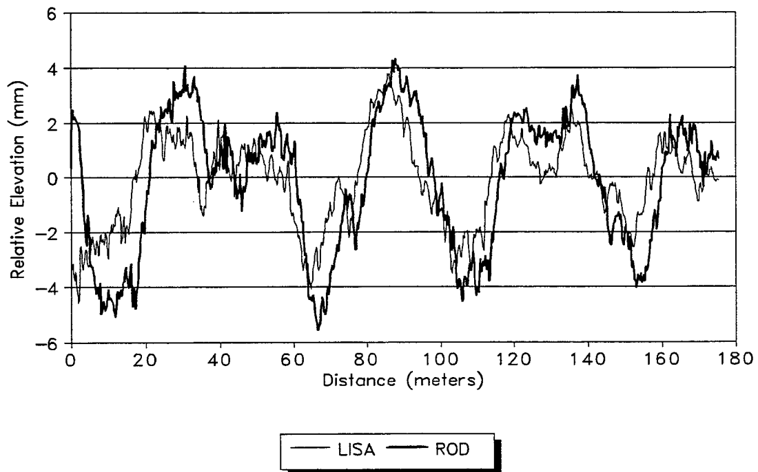
Figure 45. Average Synchronized LISA Profile vs Average Filtered Rod & Level Profile (SH47A).
