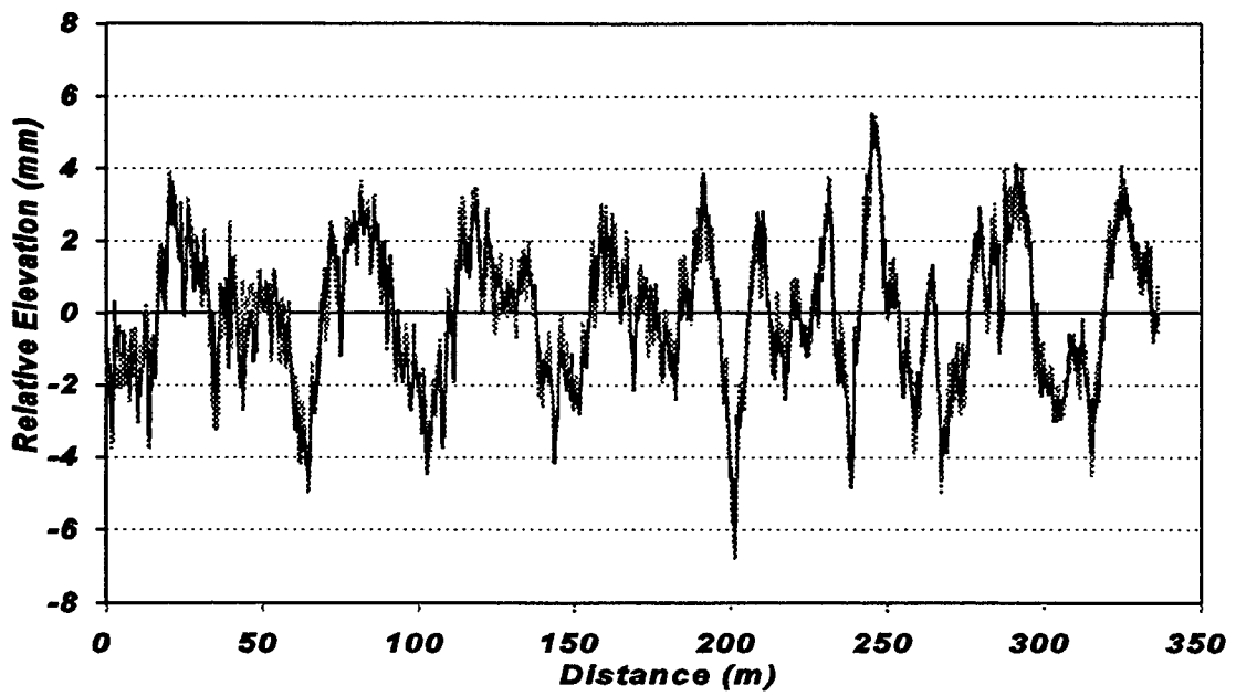
Figure A36. Original Profiles from TxDOT's Surface Profiler on SH47A, LWP.
