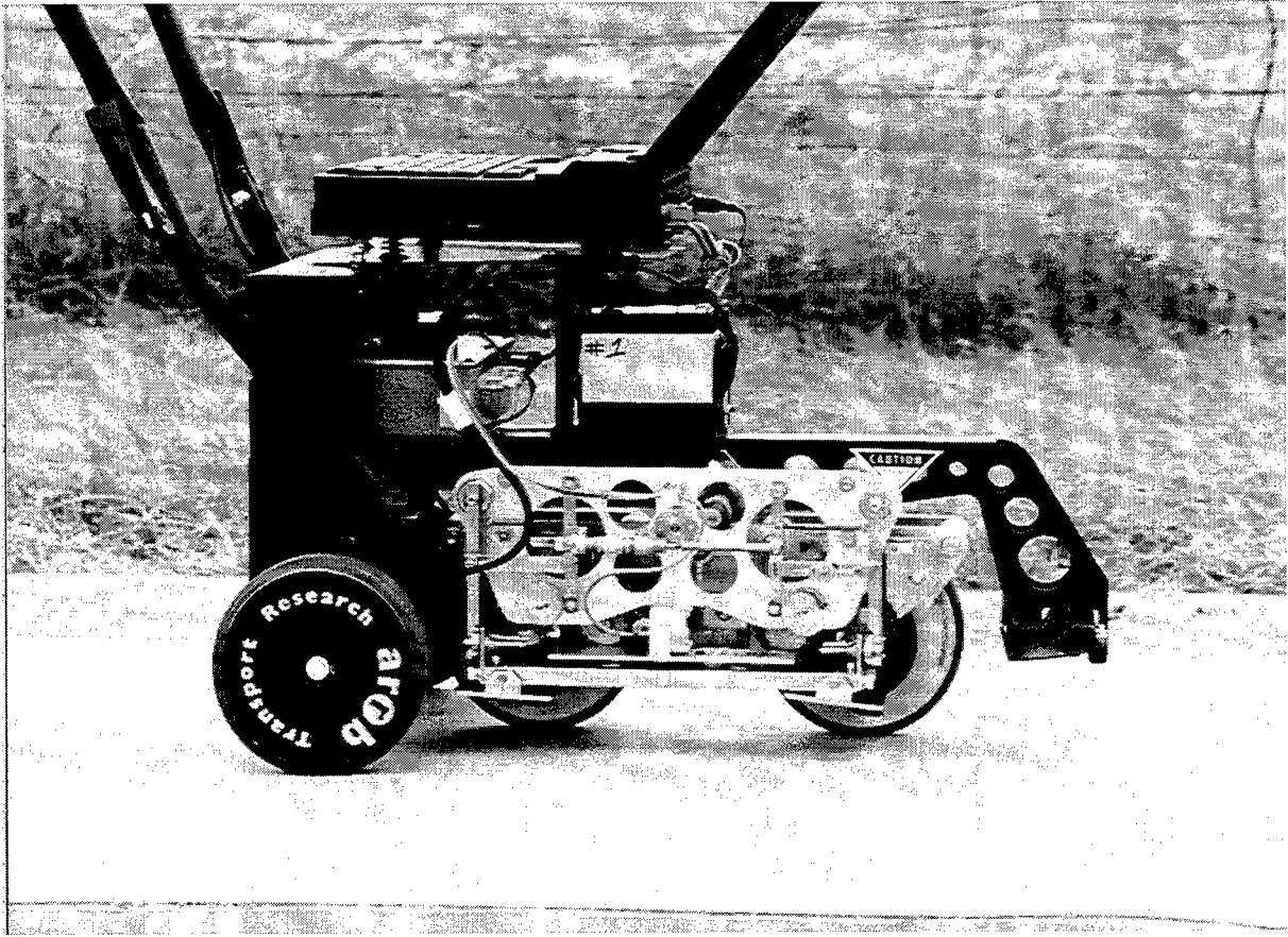
Figure 5. The Walking Profiler Developed by ARRB Transport Research Limited.
