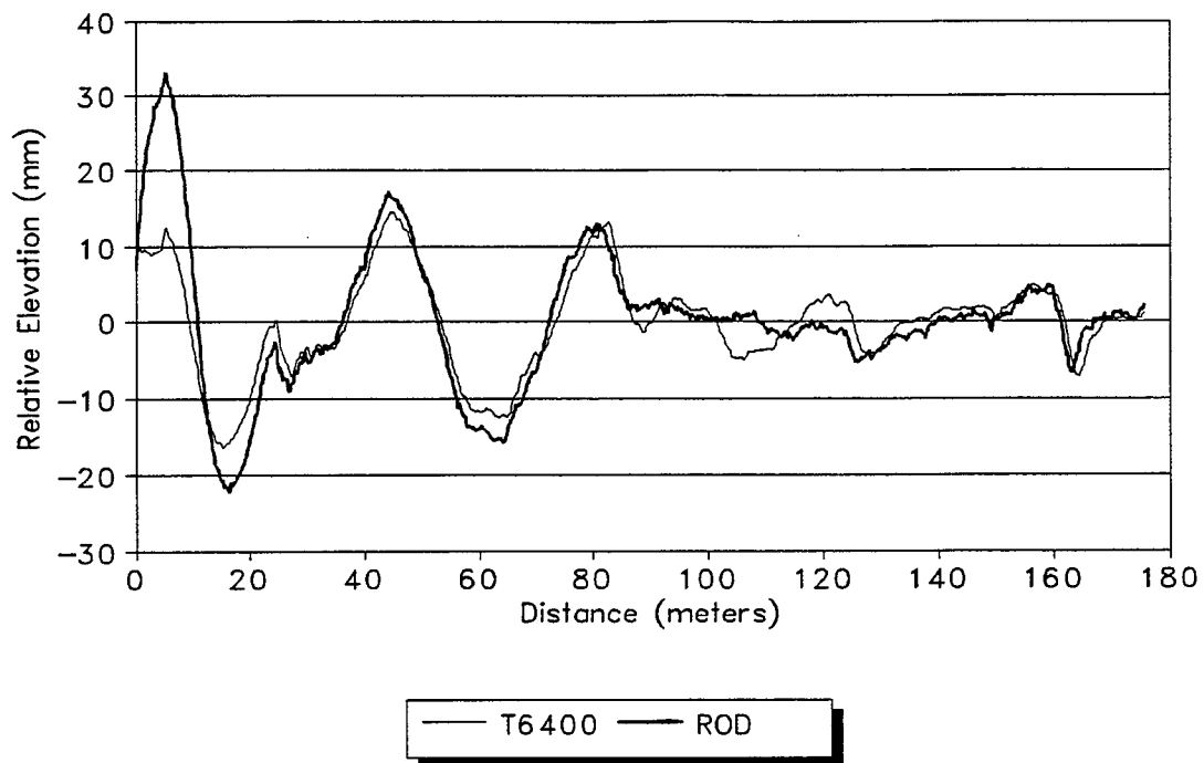
Figure 47. Average Synchronized T6400 Profile vs Average Filtered Rod & Level Profile (Annex 2).
