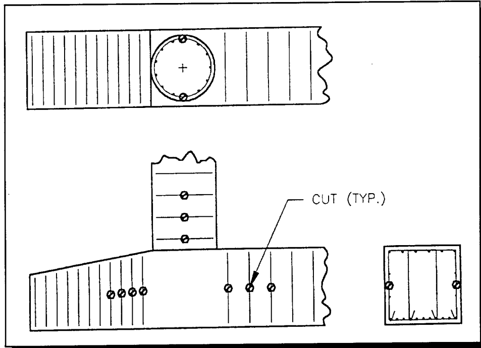
Figure 4 Exposed view of stirrups showing cut positions. (Scale 1:60).
