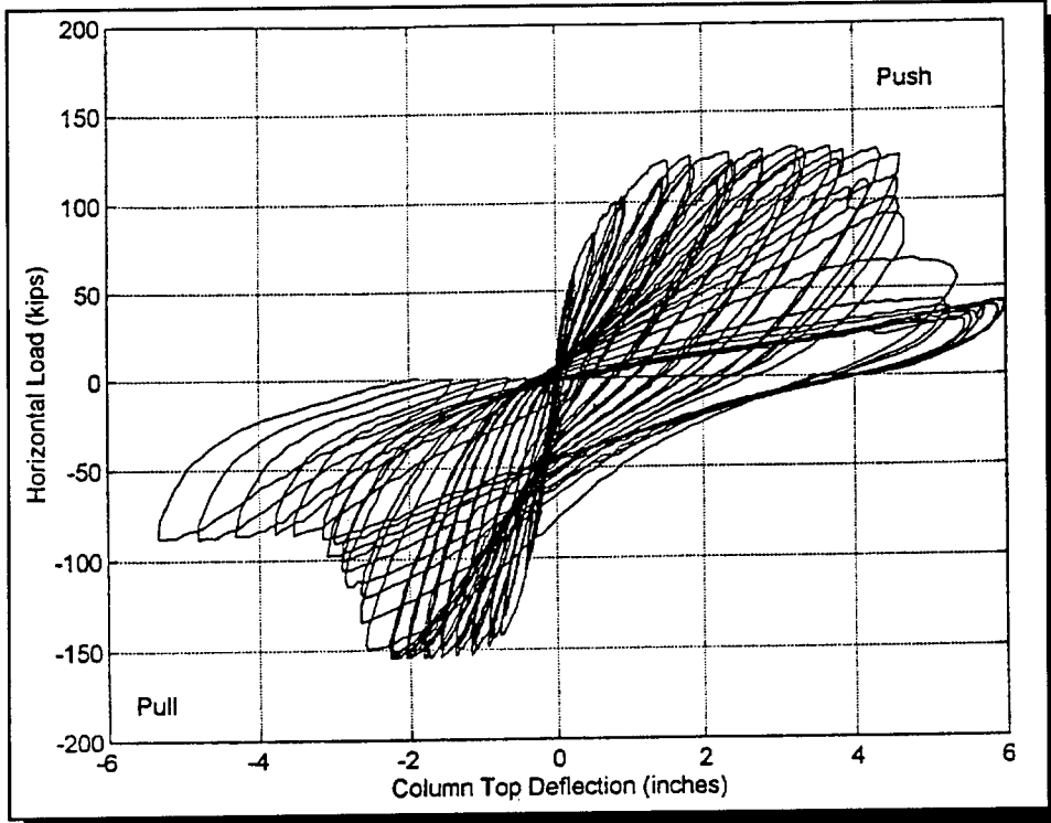
Figure 14 Test #4: 45° wrap load-deflection curve.
