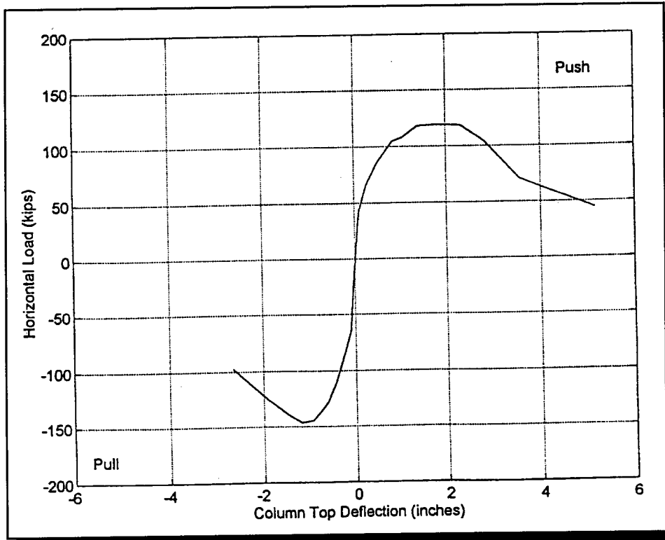
Figure 6 Test #1: Bare concrete load-deflection envelope.
