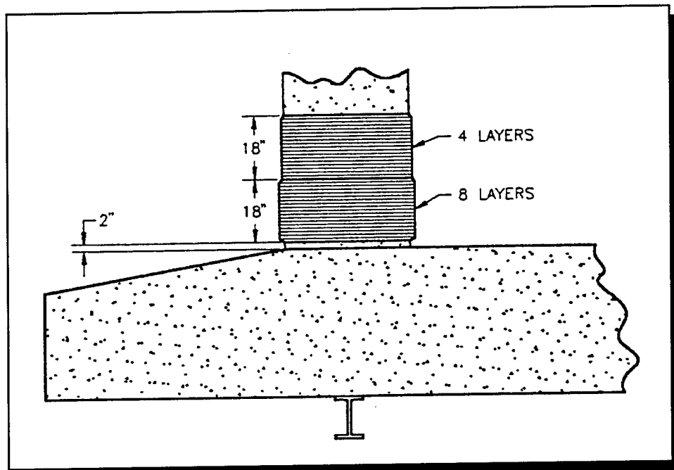
Figure 7 Test #2: Design for column composite wrap only. (Scale 1:50).
