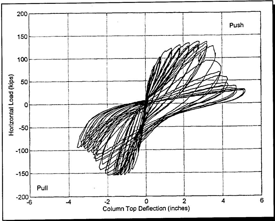
Figure 17 Test #5: 45° and 0° wrap load-deflection curve.
