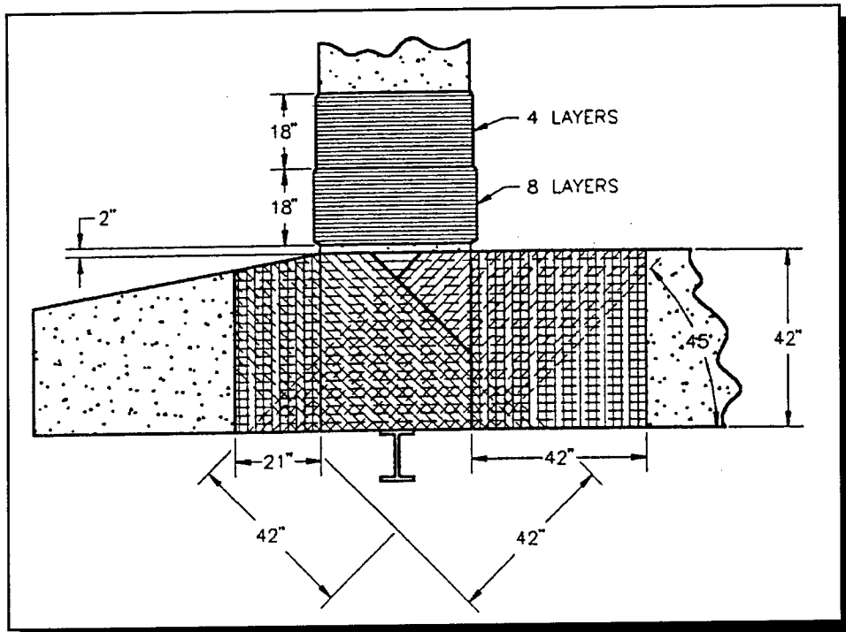
Figure 16 Test #5: Design for 0° and 45° composite wraps. (Scale 1:50).
