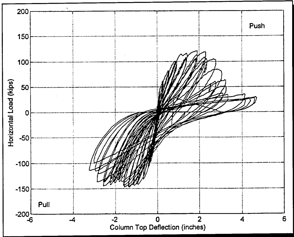
Figure 8 Test #2: Column wrap only load-deflection curve.
