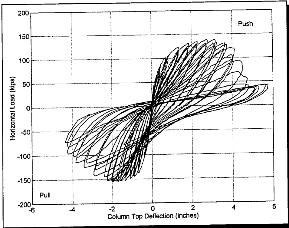
Figure 11 Test #3: 30° wrap load-deflection curve.
