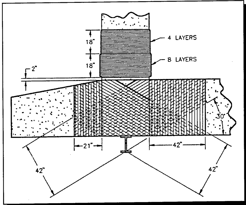
Figure 10 Test #3: Design for 30° composite wraps (Scale 1:50).
