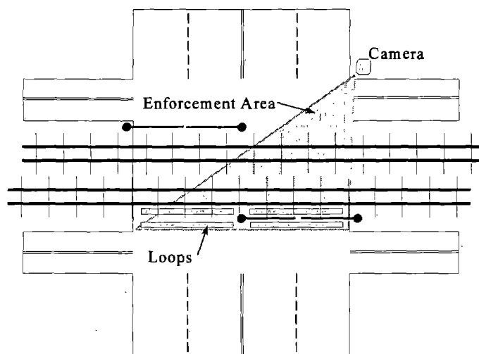
Figure 4-1. A Typical Automated Enforcement System.
