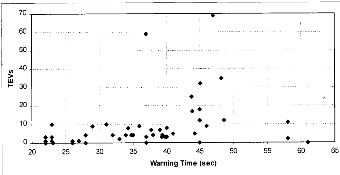
Figure 6-14. Scatter Plot of Warning Time and TEVs.
