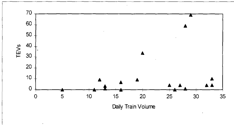
Figure 6-4. TEVs as a Function of Daily Train Volume.
