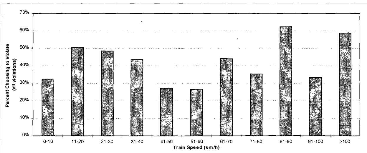
Figure 6-16. Distribution Percentage of All Violations Over Train Speed.
