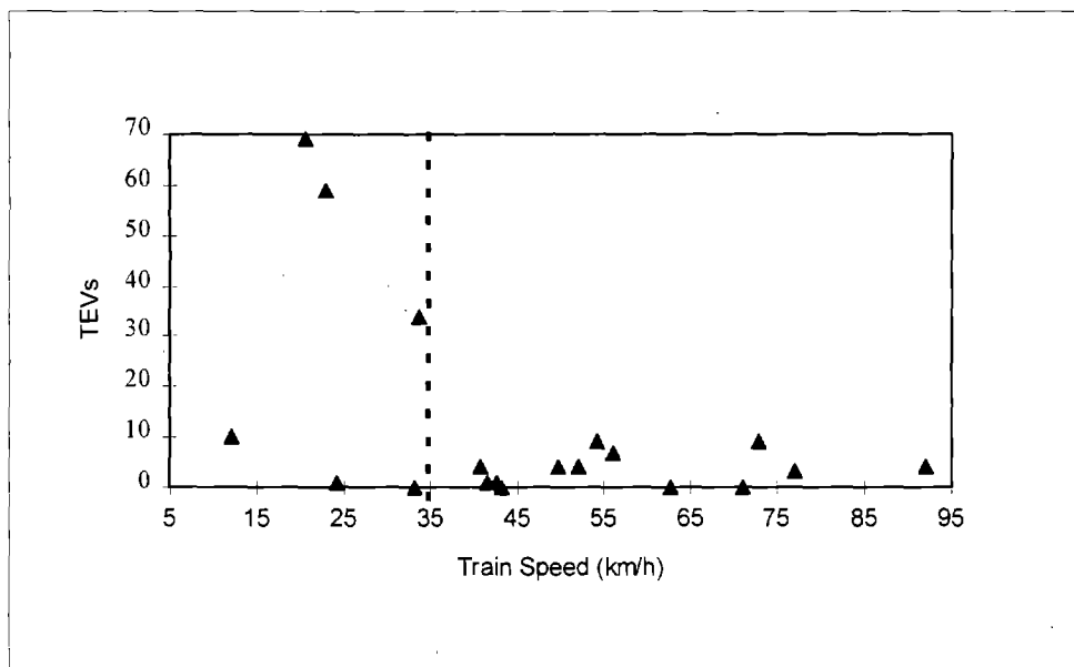
Figure 6-6. TEVs as a Function of Average Train Speed.
