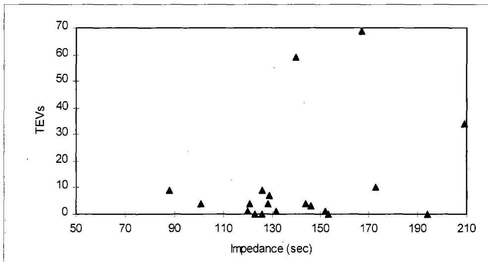
Figure 6-7. TEVs as a Function of Average Impedance.
