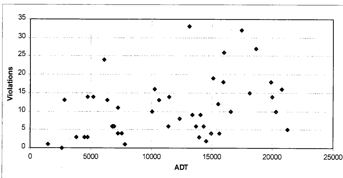
Figure 6-10. Scatter Plot of ADT and FL Violations.
