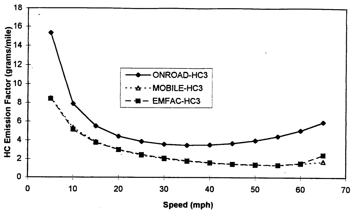
Figure 5-25: Emission factors at various instantaneous speeds for the HC emissions for vehicle type 3
