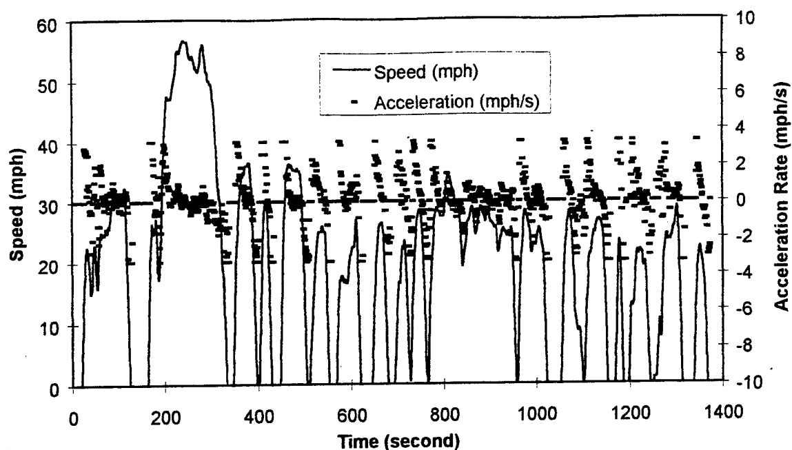
Figure 2-1: Time versus instantaneous speed and acceleration rate for FTP urban driving cycle for light-duty vehicles
