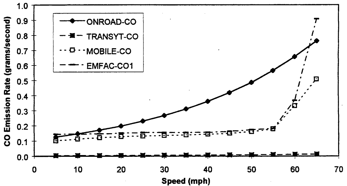
Figure 5-11: Emission factors at various instantaneous speeds for the aggregate CO emissions
