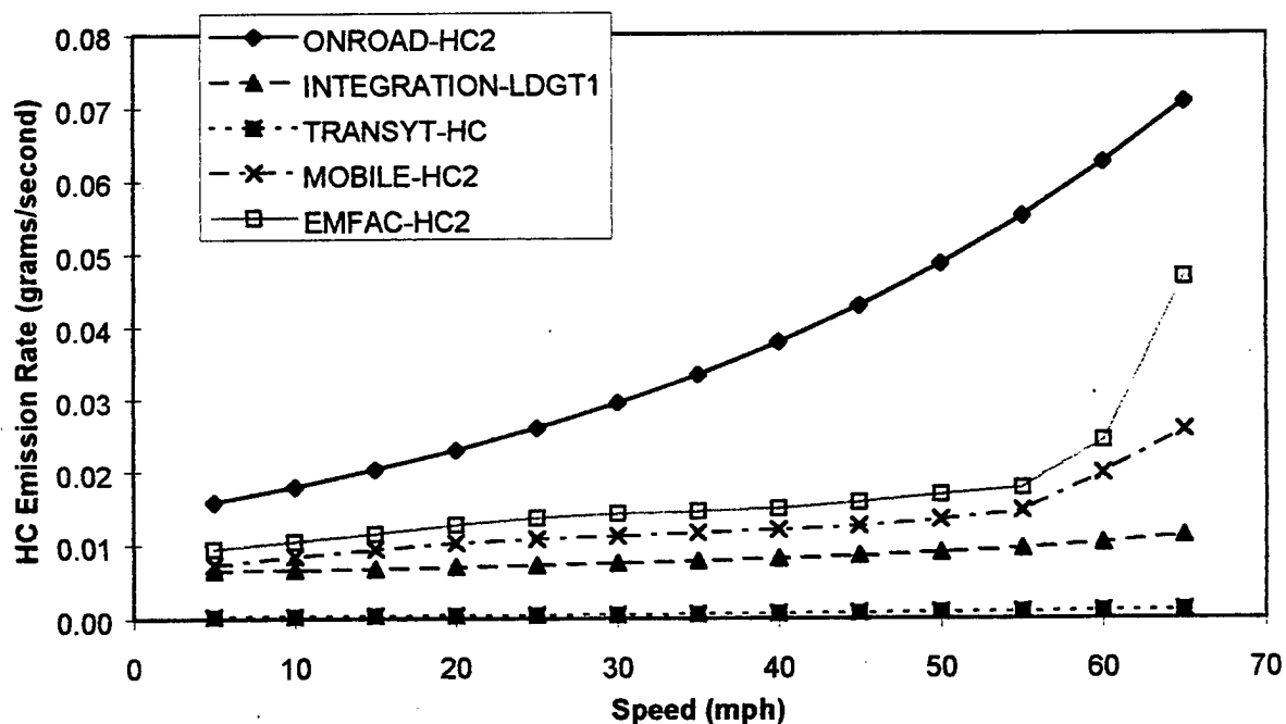
Figure 5-23: Emission factors at various instantaneous speeds for the HC emissions for vehicle type 2
