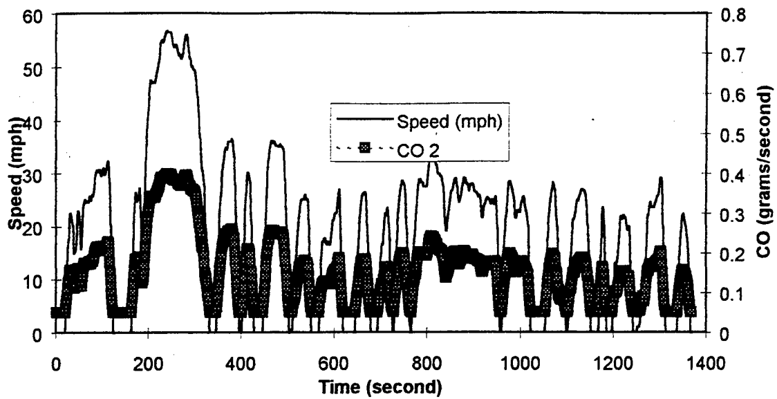
Figure 5-3: Emulated CO emission rate for vehicle type 2 for FTP urban driving cycle for light duty vehicles and light duty trucks
