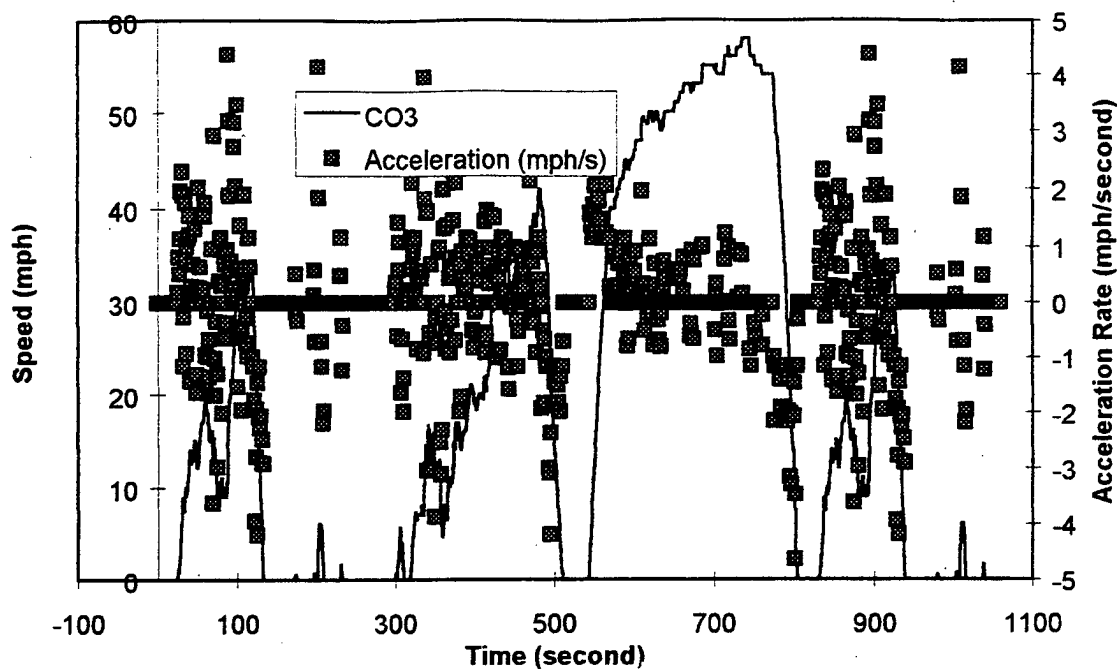
Figure 2-3: Time versus instantaneous speed and acceleration rate for FTP driving cycle for heavy-duty vehicles
