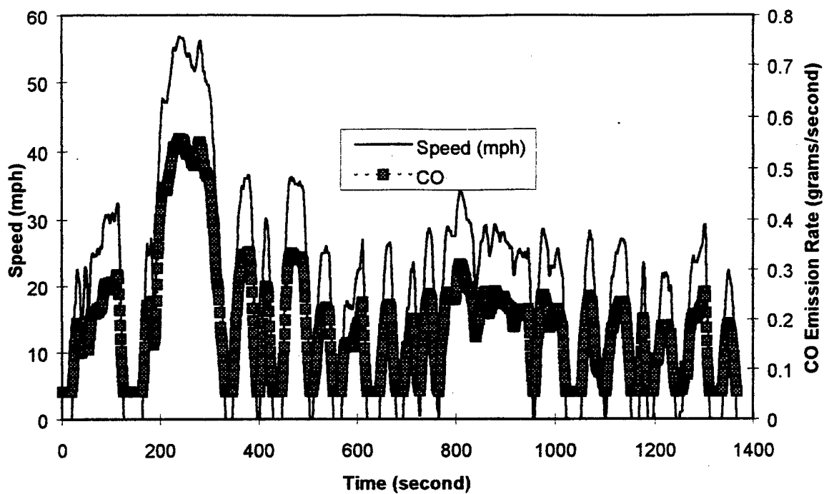
Figure 5-1: Emulated CO emission rate for FTP urban driving cycle for light duty vehicles and light duty trucks
