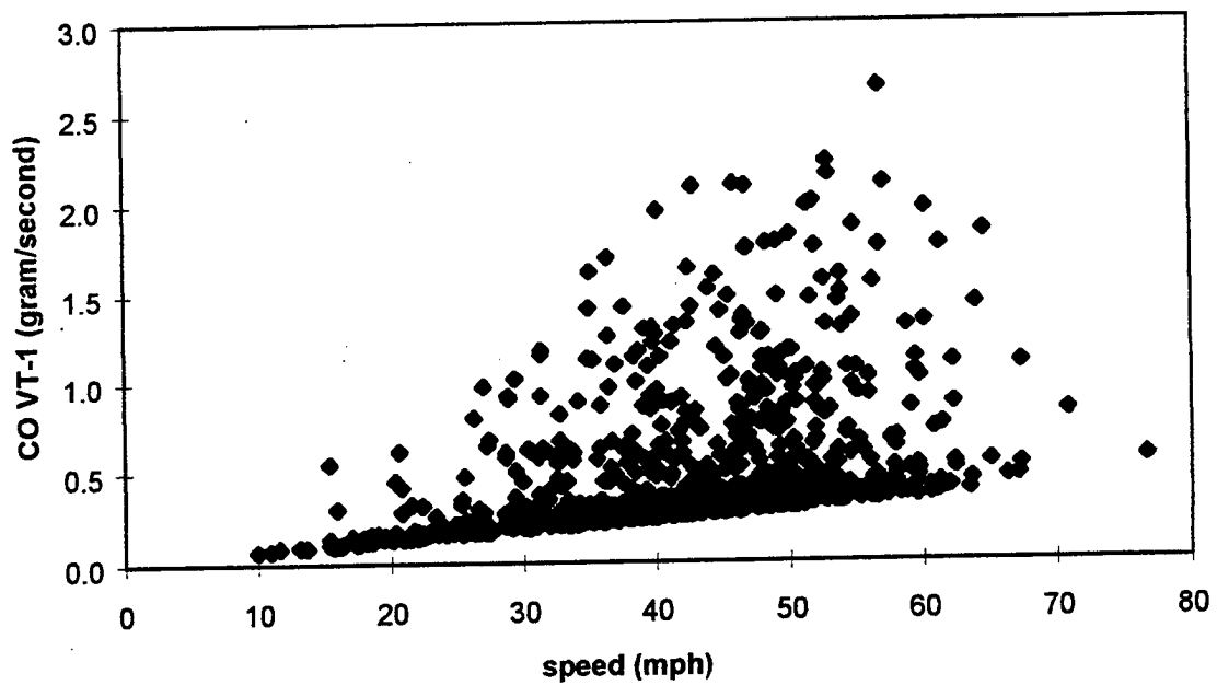
Figure 4-2: CO emissions rates versus instantaneous speed values for vehicle type 1
