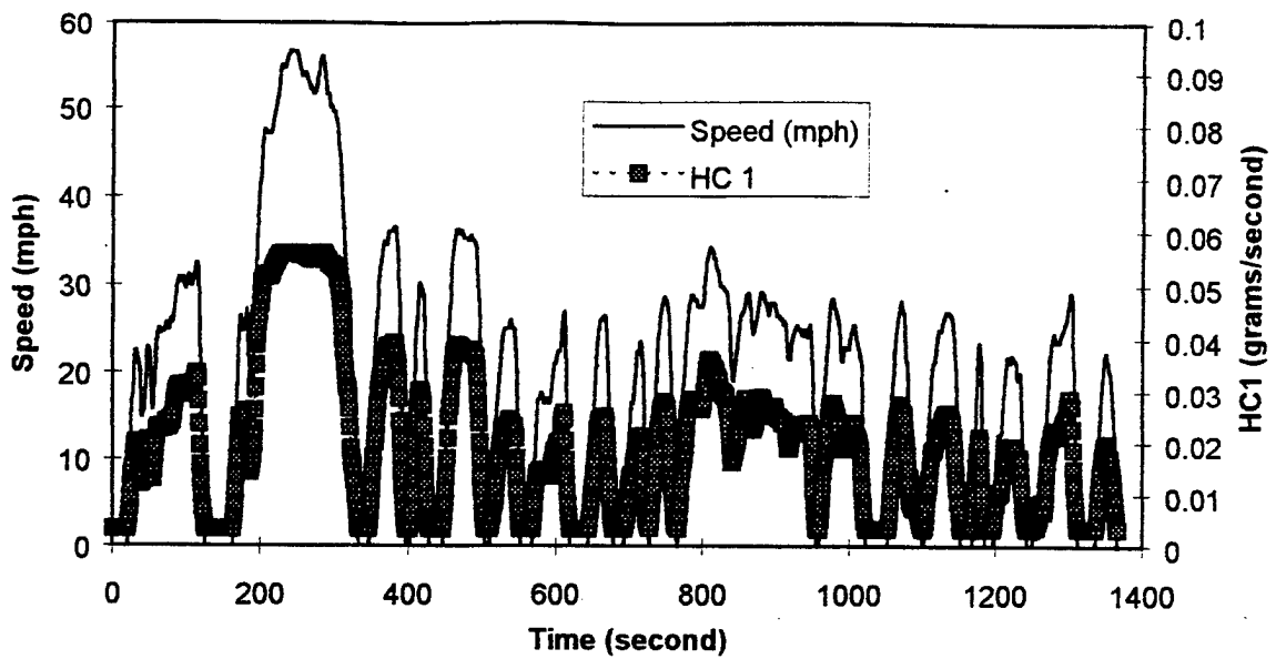
Figure 5-5: Emulated HC emission rate for vehicle type 1 for FTP urban driving cycle for light duty vehicles and light duty trucks
