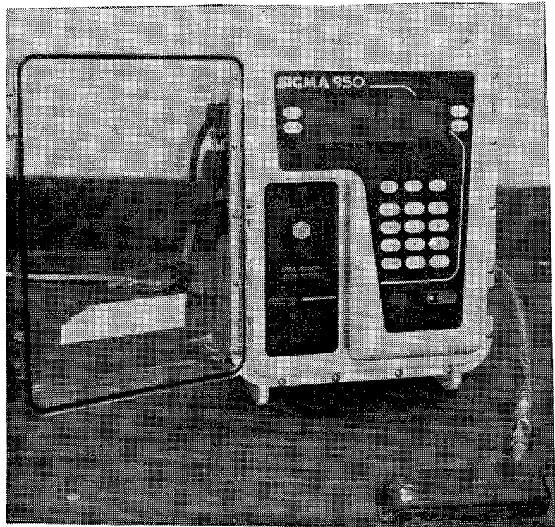
(b) American Sigma 950 flowmeter
