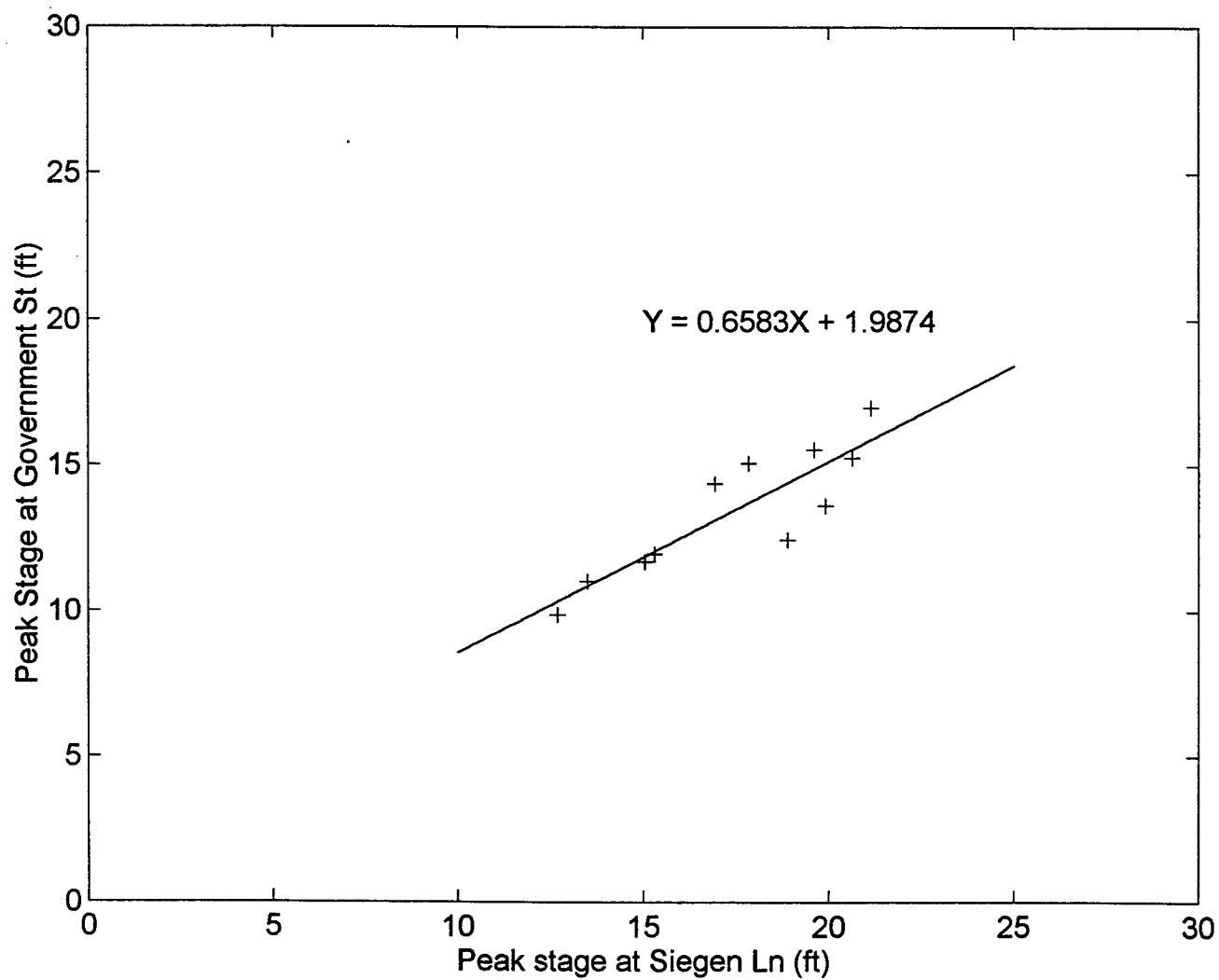
Figure 7.2 Relation between peak stages in Ward Creek at Government Street and Siegen Lane
