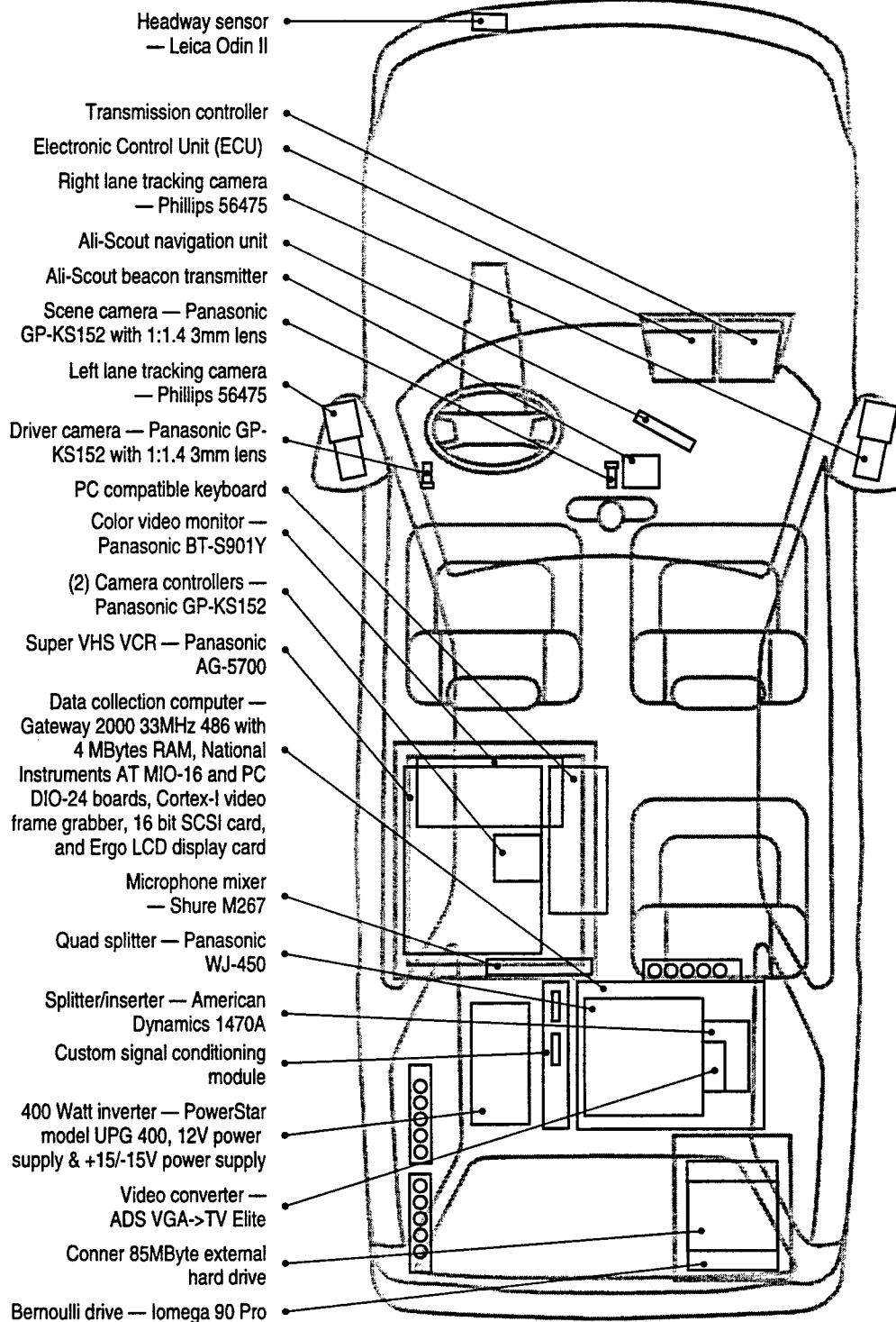
Figure 2.2.4. UMTRI instrumented vehicle
