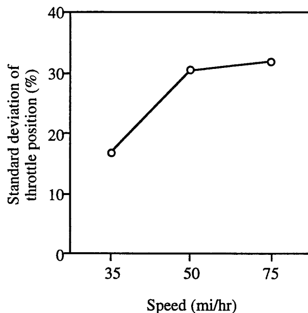
Figure 2.3.23. Effect of speed in simulator on S.D. of throttle position
