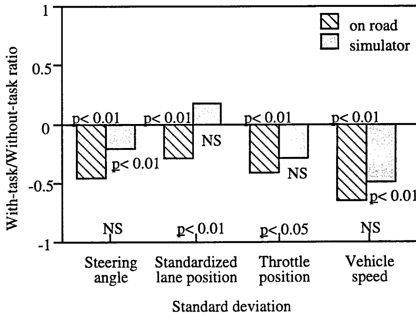
Figure 2.3.26. Summary effects of secondary task on driving performance
