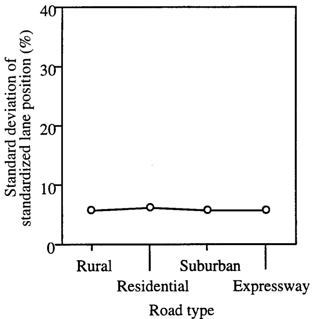
Figure 2.3.20. Effect of actual road driven on S.D. of standardized lane position
