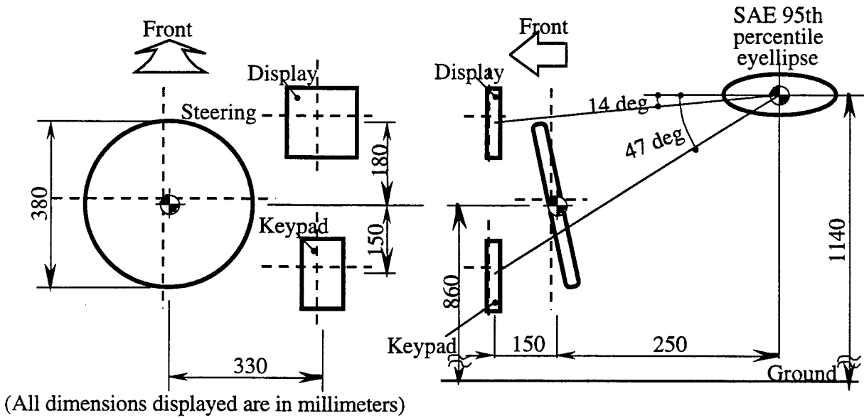
Figure 2.2.6. Locations of the LCD and the number display
