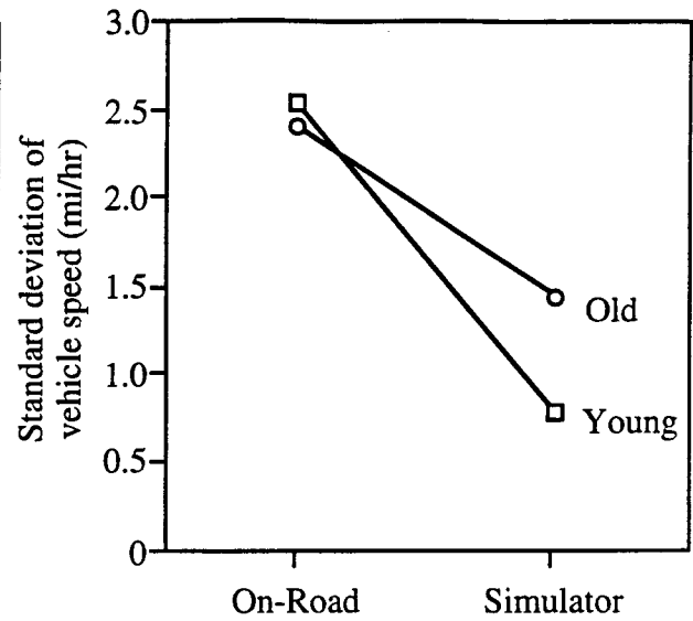
Figure 2.3.11. Age by context interaction of S.D. of vehicle speed
