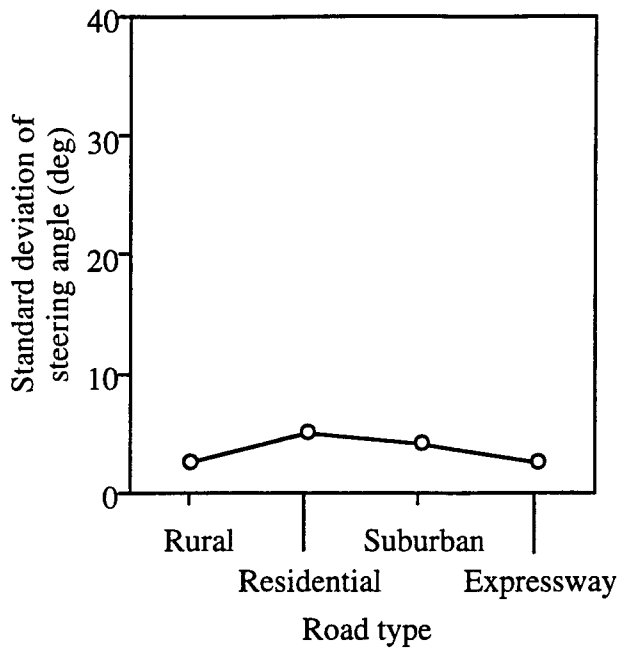
Figure 2.3.18. Effect of actual road driven on S.D. steering angle
