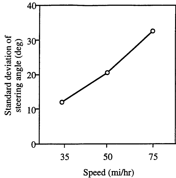
Figure 2.3.19. Effect of speed in simulator on S.D. of steering angle
