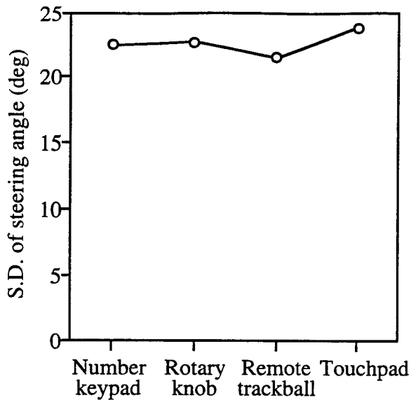
Figure 4.3.17. Effect of control on S.D. of steering angle
