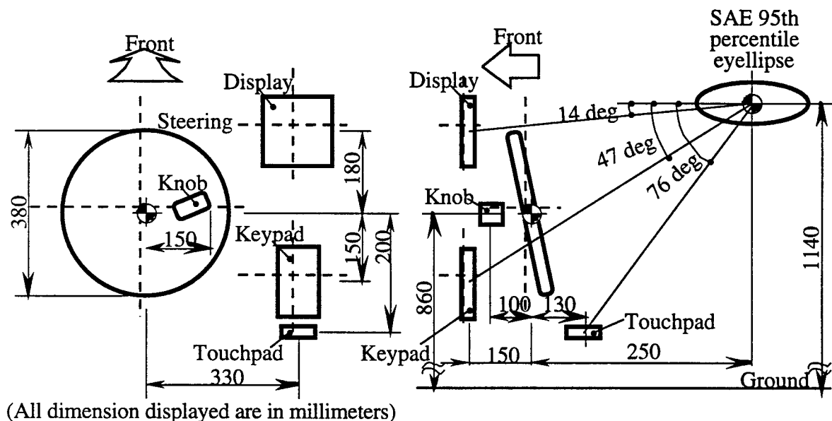
Figure 4.2.1. Location of the LCD and four multipurpose controls
