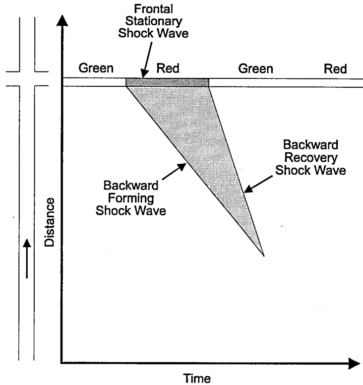
Figure 12. Shock Waves at Signalized Intersection
