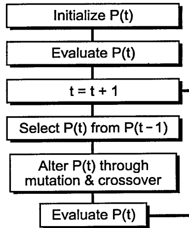
Figure 10. GA Procedure
