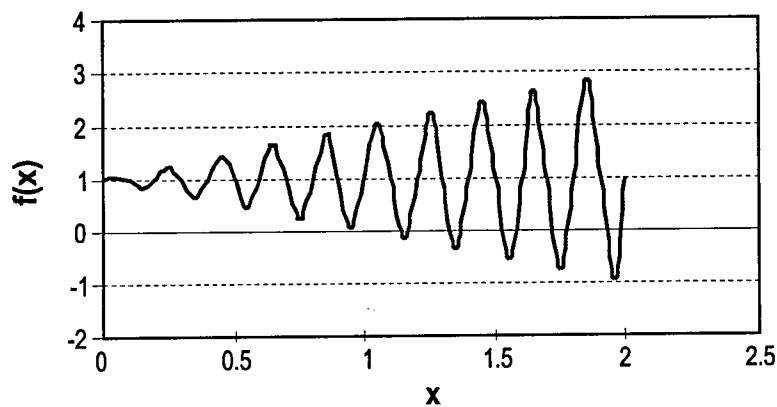
Figure 9. Function with a Number of Local Optima
