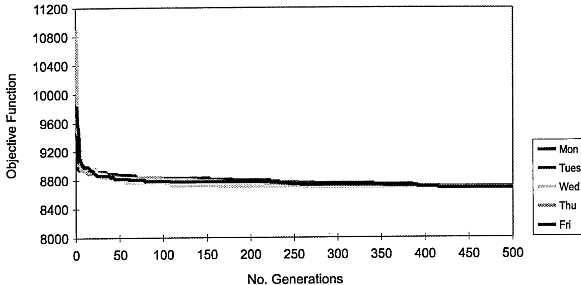
Figure 18. GA Results for Case 1
