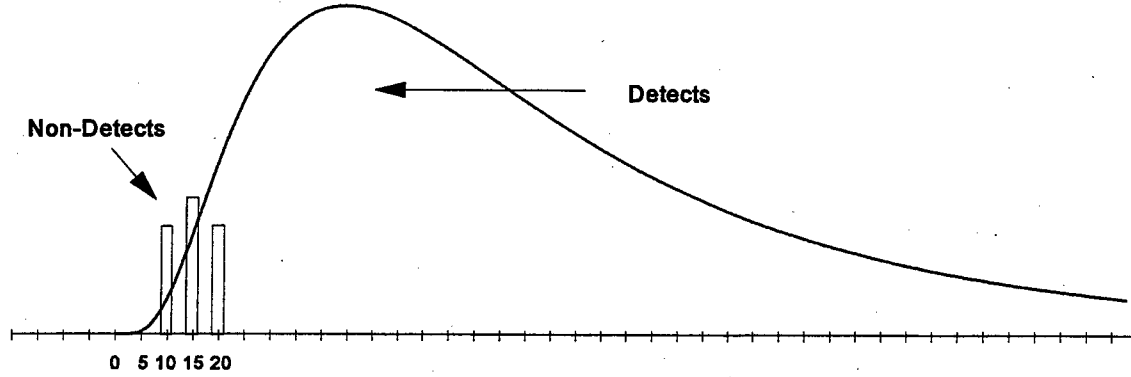
Figure 4-3. Modified Adapted Delta-lognormal Model
