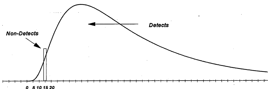
Figure 4-2. Adapted Delta-lognormal Model
