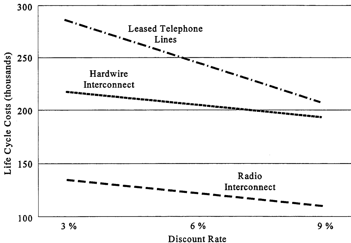
Figure I-2. Life Cycle Cost Comparison for Popular Signal Communications Media Adapted from (4)
