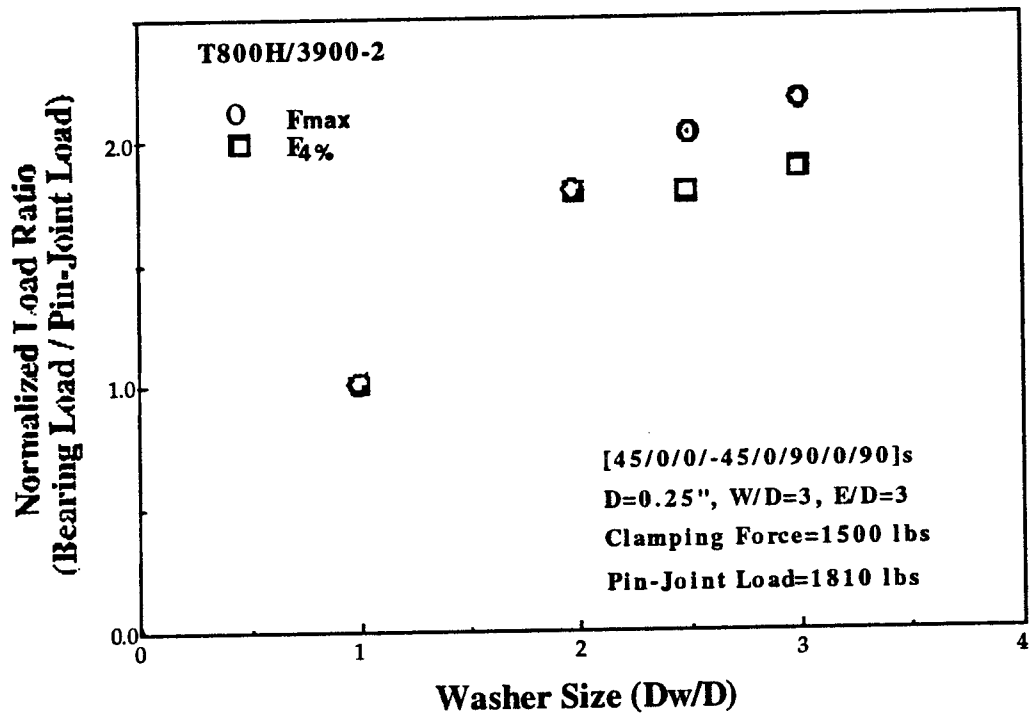
FIGURE 25. EFFECT OF WASHER SIZE ON THE FAILURE LOAD OF BOLTED COMPOSITE JOINTS
