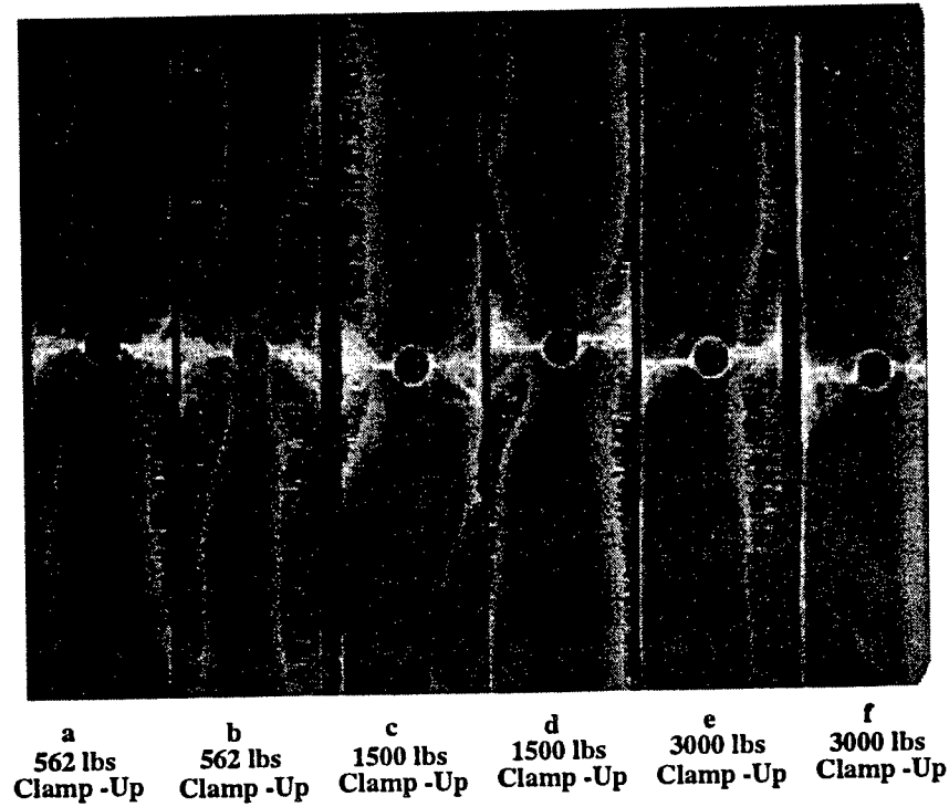
FIGURE 13. RADIOGRAPHS OF FILLED-HOLE SPECIMENS AT VARIOUS CLAMPING LOADS
