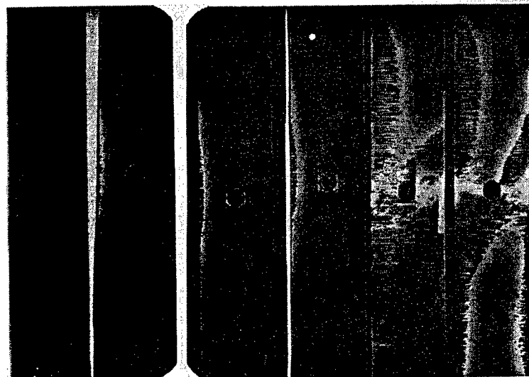
Load Level: 68% 79% 88% 95% 100% 100% Open Hole Tension
