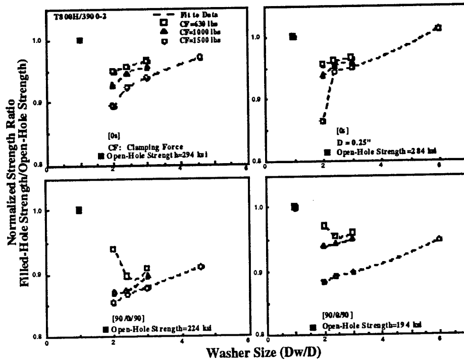
FIGURE 17. EFFECT OF WASHER SIZE ON NOTCH STRENGTH OF FILLED-HOLE LAMINATES
