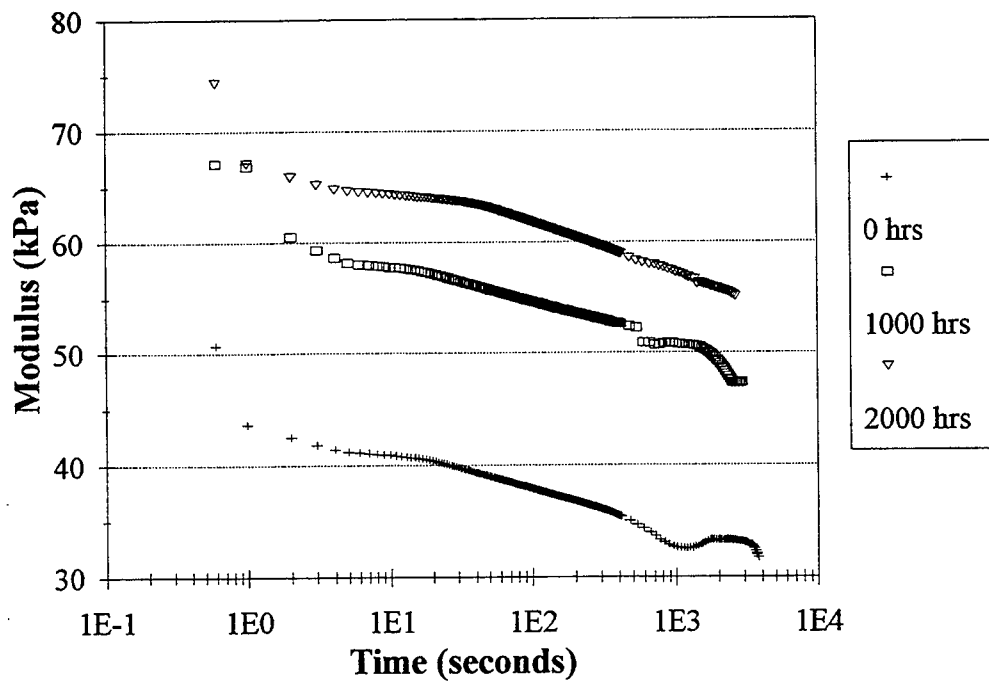
Figure 20. Relaxation Modulus for Seal V-687 at 30% Strain Level.
