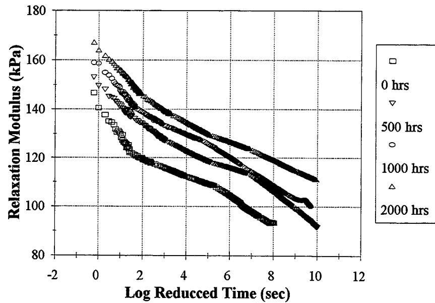
Figure 69. Relaxation Modulus Curves Normalized for Extension at 60 °C.
