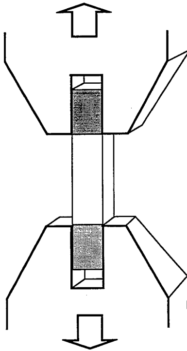
Figure 41. Test Setup for the Relaxation Test.
