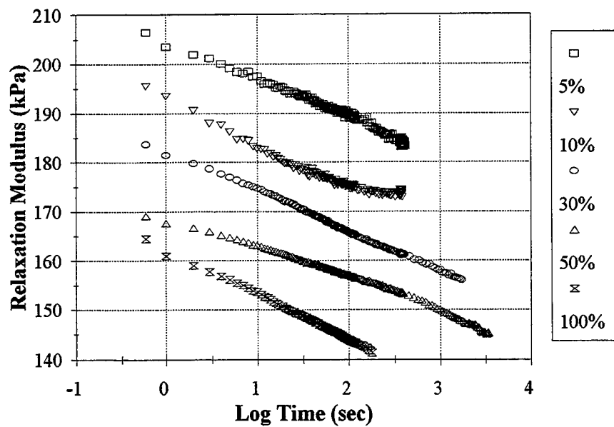
Figure 51. Relaxation Modulus of a 2000 Hours Artificially Weathered Crafc0 903 SL Specimen at 0 °C.
