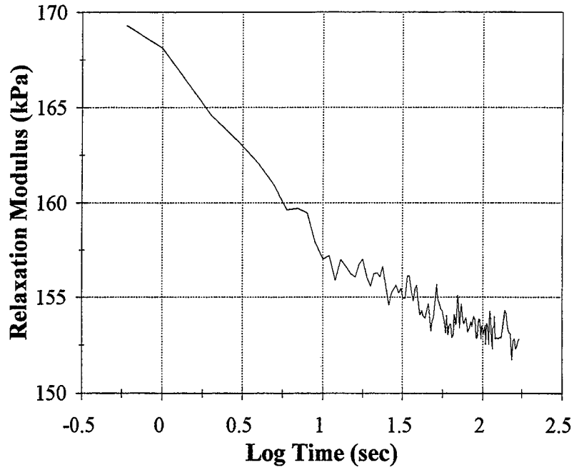
Figure 34. Relaxation Modulus of Type 3 Joint Sealants.
