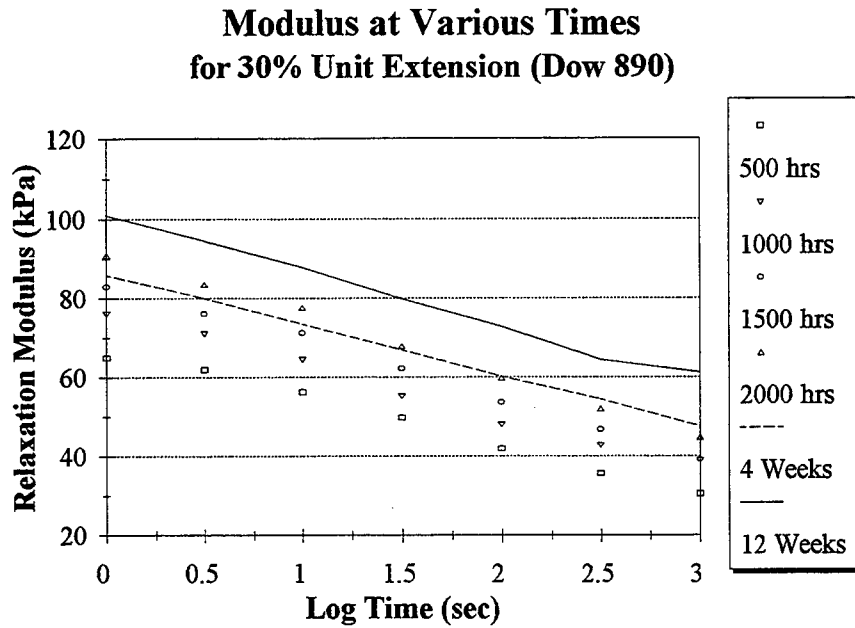
Figure 29. Relaxation Moduli of Dow Corning 890 SL After Natural and Artificial Weathering.
