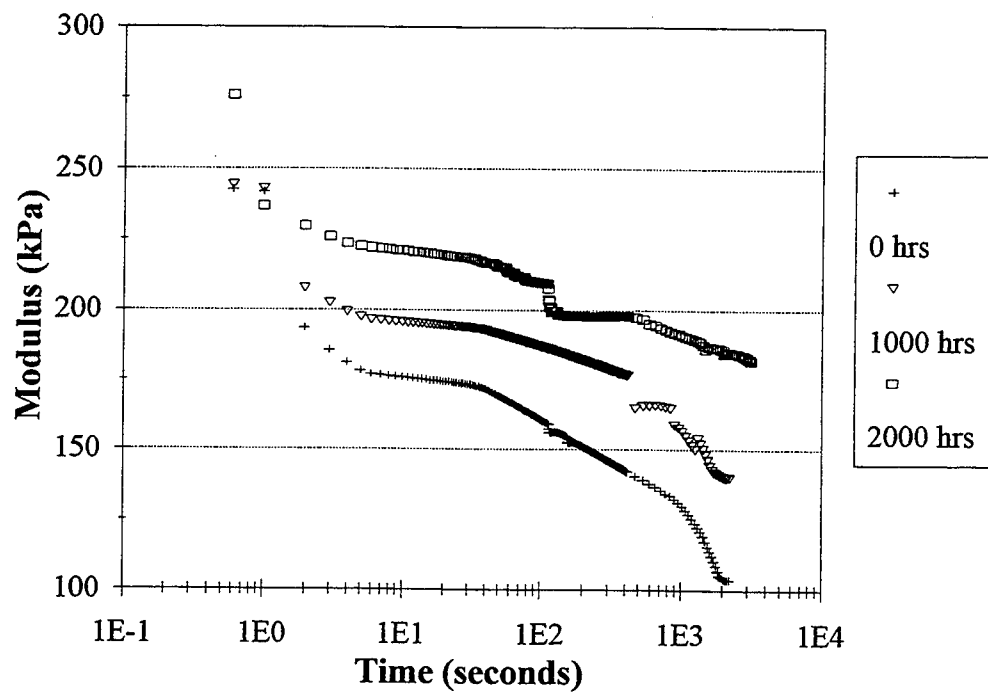
Figure 22. Relaxation Modulus for Seal V-812 at 30% Strain Level.
