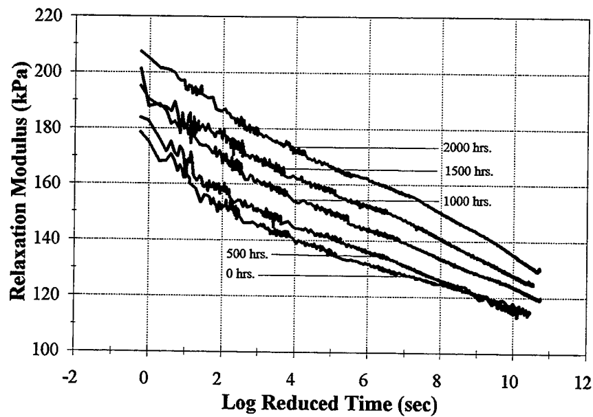
Figure 67. Relaxation Modulus Curves Normalized for Extension at 25 °C.
