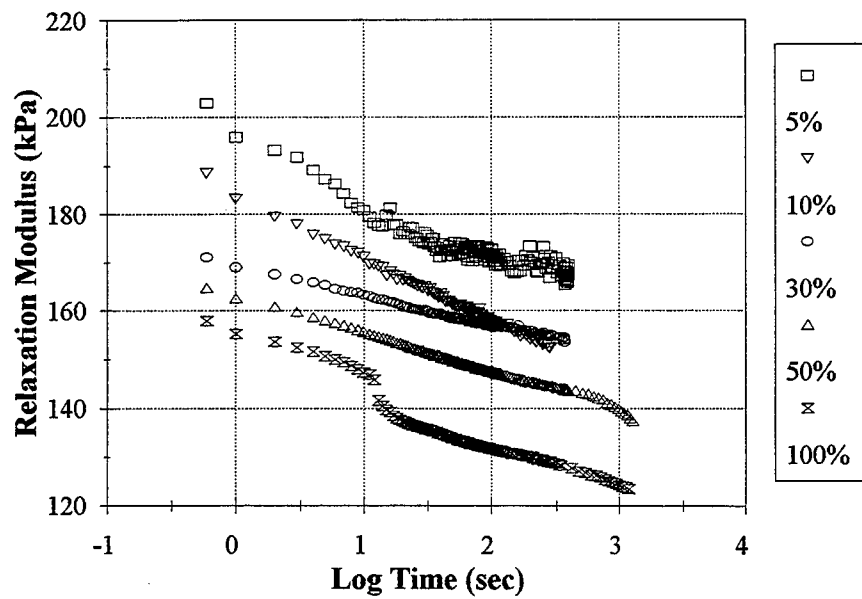
Figure 45. Relaxation Modulus of a 500 Hours Artificially Weathered Crafc0 903 SL Specimen at -25°C.
