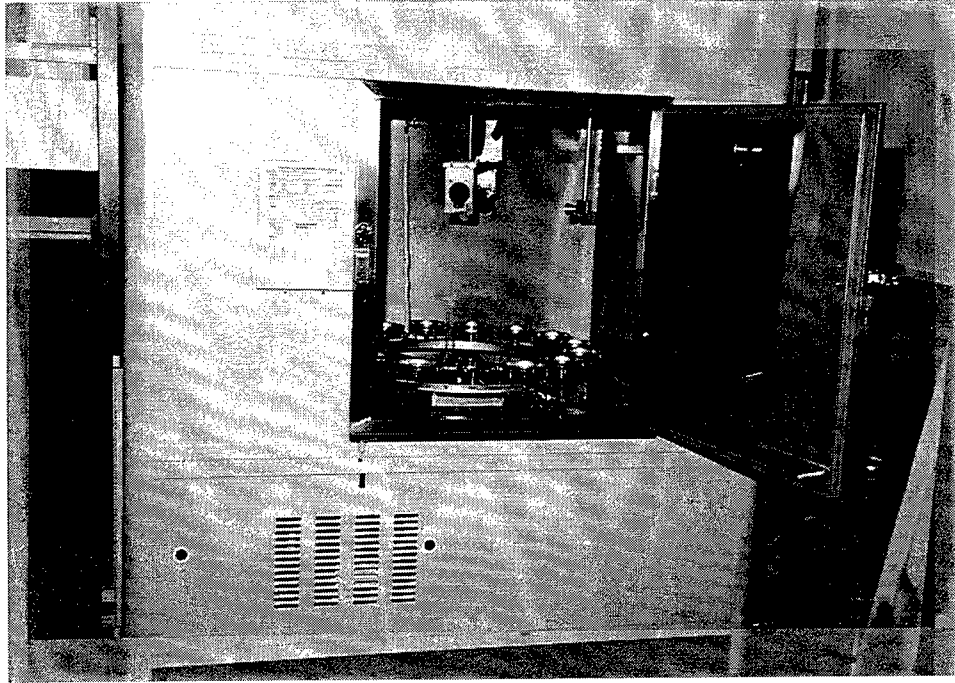
FIGURE 11. Test Samples in Atlas Ci65A Xenon Weather-Ometer®.
