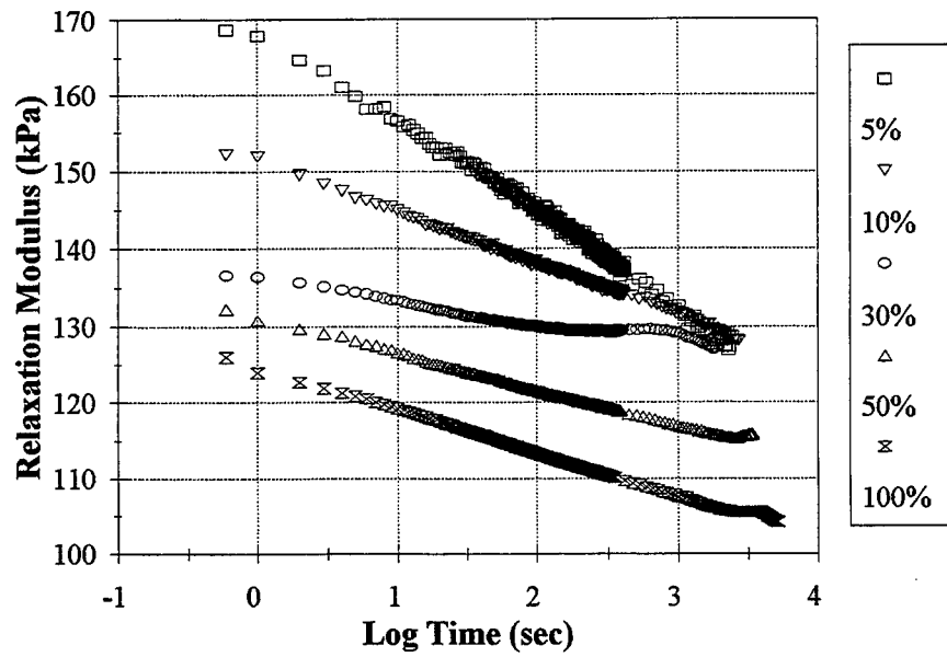
Figure 59. Relaxation Modulus of a 2000 Hours Artificially Weathered Crafc0 903 SL Specimen at 40 °C.
