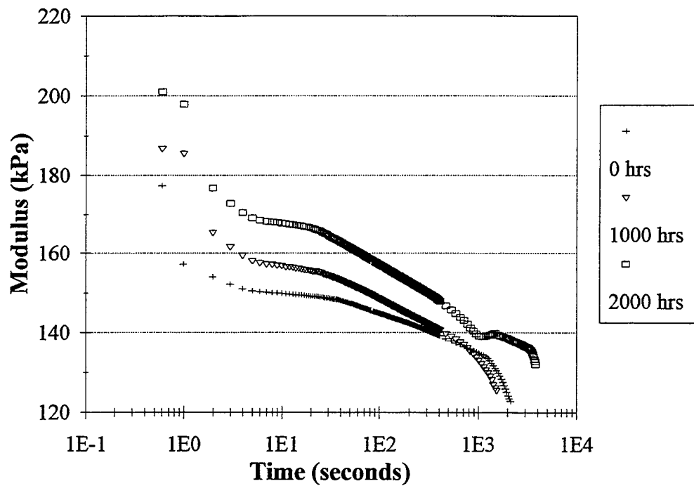
Figure 21. Relaxation Modulus for Seal V-812 at 15% Strain Level.
