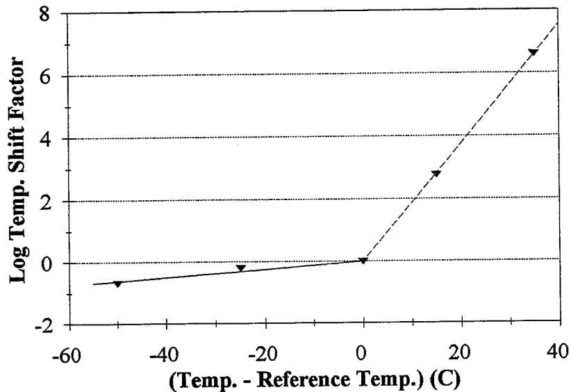
Figure 73. Time-Temperature Shift Factor Relationship of Crafc0 903 SL. (Reference temperature = 25^\circ\text{C} .)
