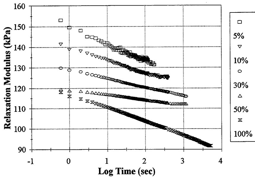
Figure 60. Relaxation Modulus of a Fresh Crafc0 903 SL Specimen at 60 °C.
