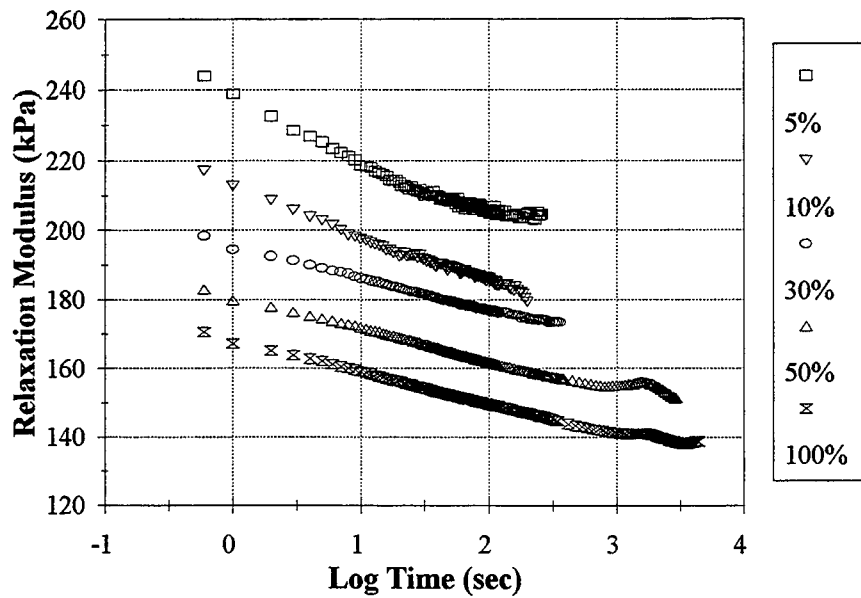
Figure 47. Relaxation Modulus of a 2000 Hours Artificially Weathered Crafc0 903 SL Specimen at -25 °C.
