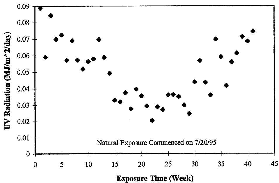
Figure 24. Average Daily Solar Radiation per Week at the Exposure Site.
