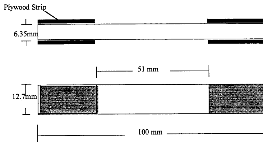
Figure 40. Relaxation Test Specimen with End Plates.
