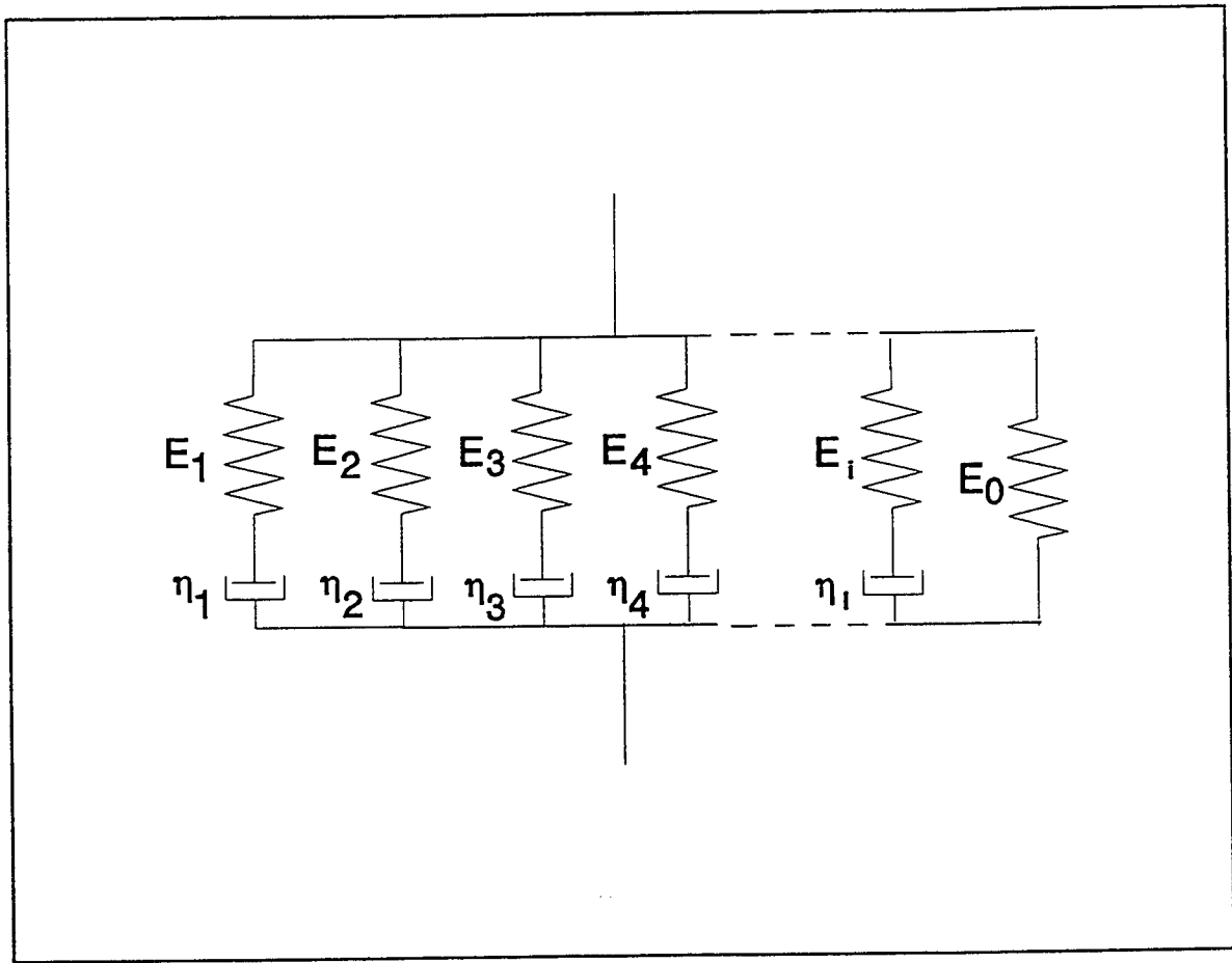
Figure 13. Generalized Maxwell Model.
