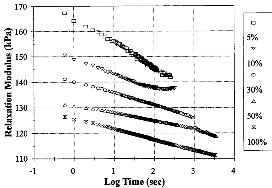
Figure 63. Relaxation Modulus of a 2000 Hours Artificially Weathered Crafc0 903 SL Specimen at 60 °C.
