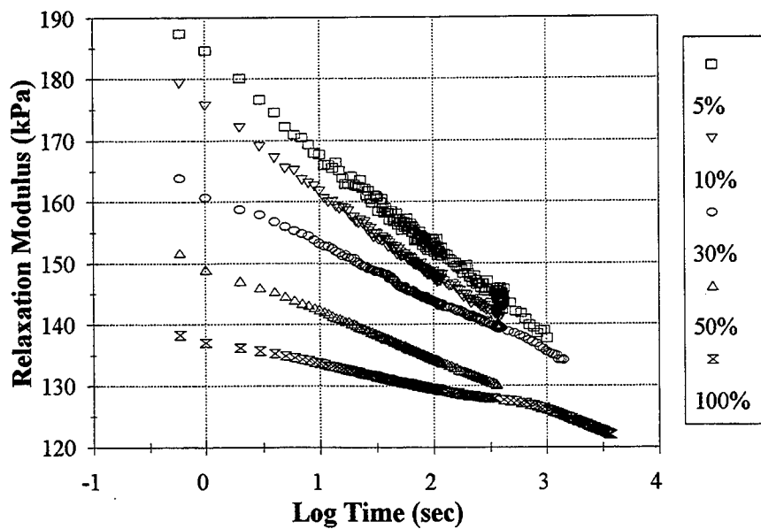
Figure 49. Relaxation Modulus of a 500 Hours Artificially Weathered Crafc0 903 SL Specimen at 0 °C.
