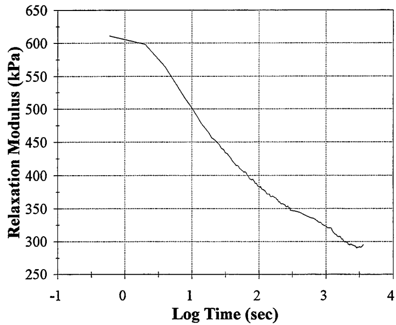
Figure 33. Relaxation Modulus of Type 2 Joint Sealants.
