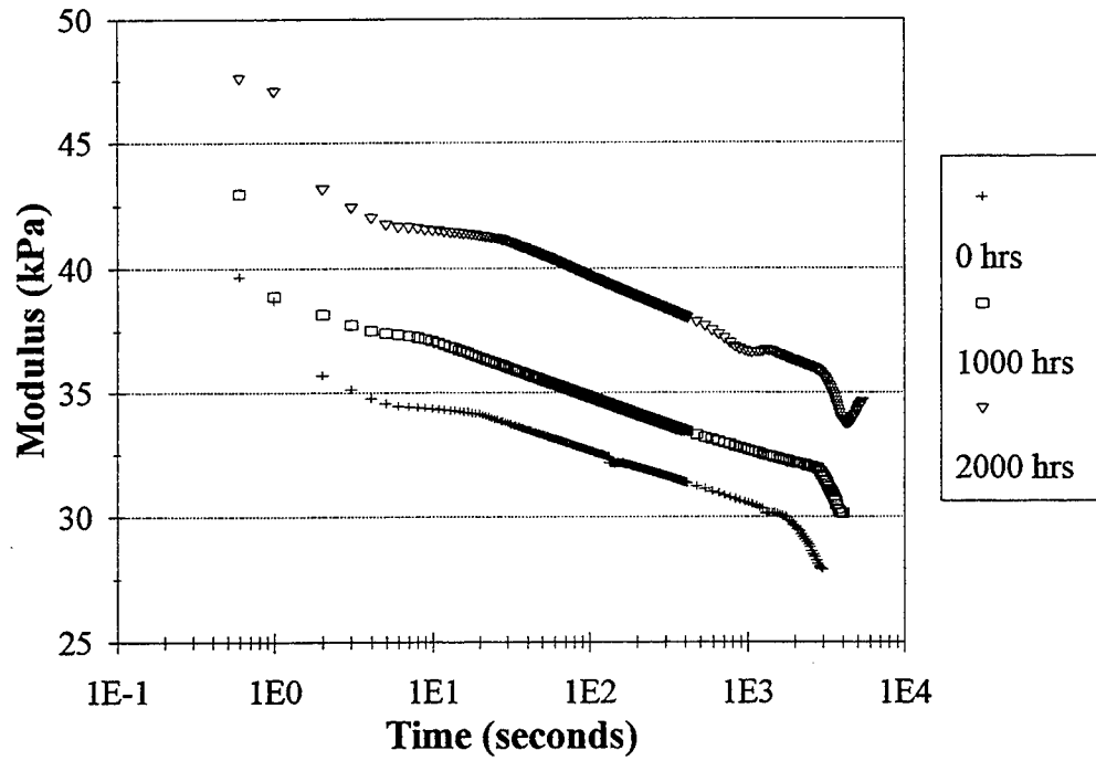
Figure 19. Relaxation Modulus for Seal V-687 at 15% Strain Level.
