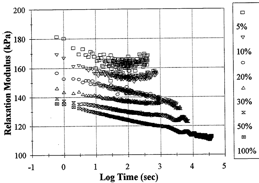
Figure 53. Relaxation Modulus of a 500 Hours Artificially Weathered Crafc0 903 SL Specimen at 25 °C.
