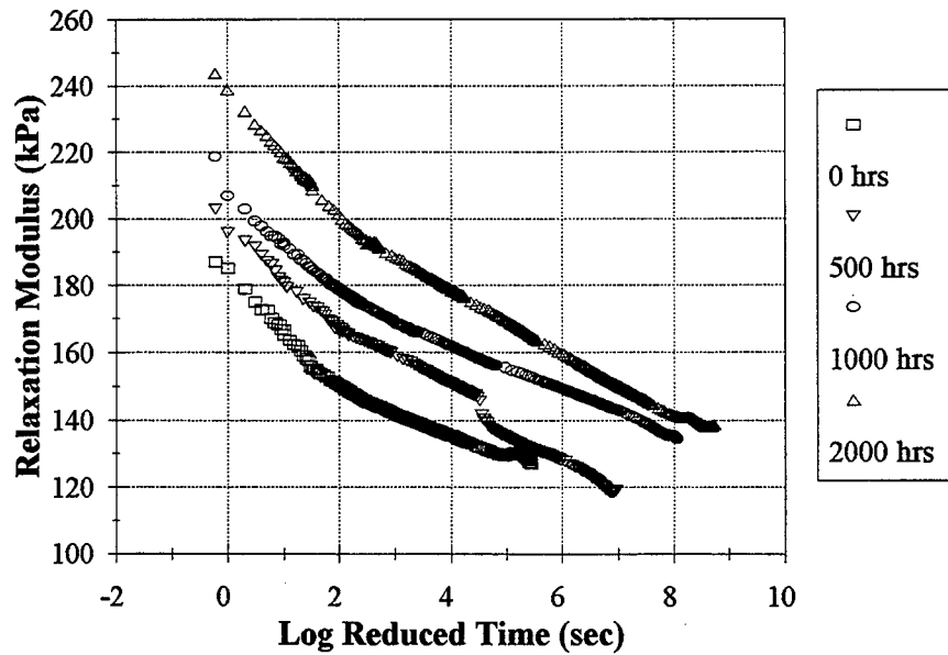
Figure 64. Time-Deformation Shift Factor Relationship for Crafc0 903 SL.
