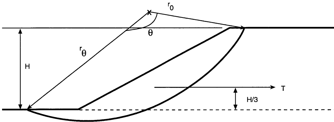
Figure 4.2 Log spiral shear surface and parameters used to determine the required reinforcement force for slopes on foundations with the same strength
