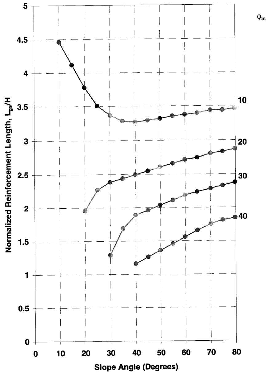
Figure 4.16 Minimum length of reinforcement for global stability of slopes on much stronger foundations – r_u = 0.5
