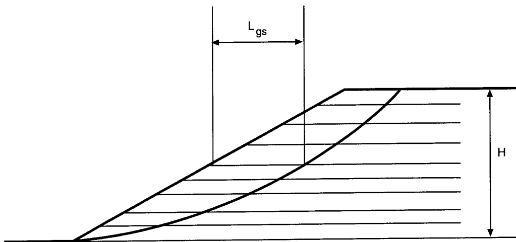
Figure 4.10 Scheme used to determine required reinforcement length for global stability with log spiral shear surfaces
