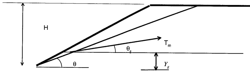
Figure 3.14 Planar shear surface model used in force equilibrium procedure by Leshchinsky and Reinschmidt to model translational failure
