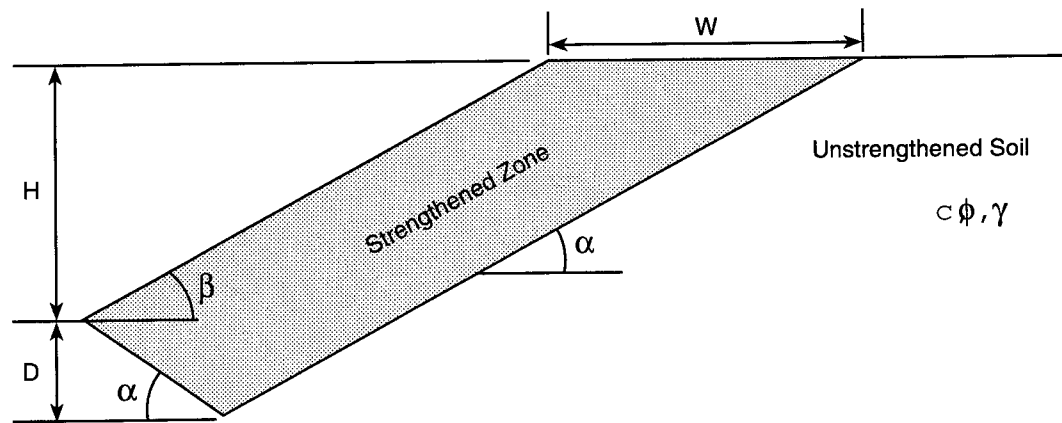
Figure 2.2 Slope parameters for strengthened earth slopes
