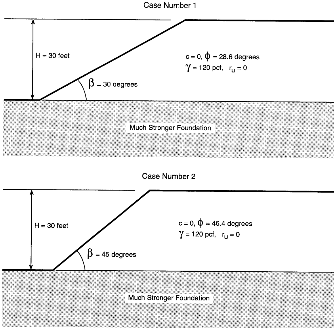
Figure 4.22 Examples used in comparison of new charts with existing methods
