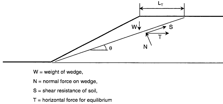
Figure 3.3 Sliding wedge force equilibrium model used by Schmertmann et al. for calculating required reinforcement length at top of slope
