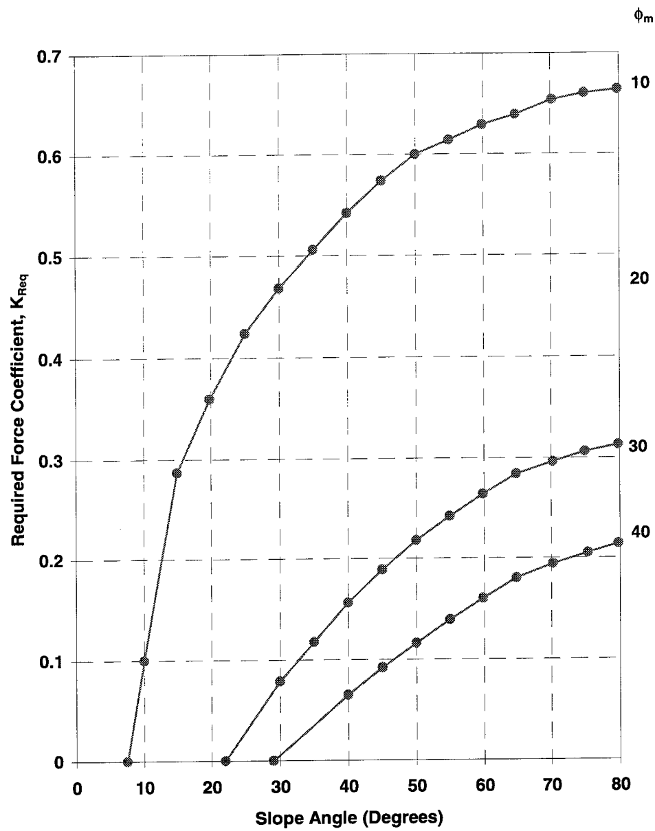
Figure 4.4 Chart for required reinforcement force coefficient ( K_{Req} ) for slopes on foundations with the same strength - r_u = 0.25
