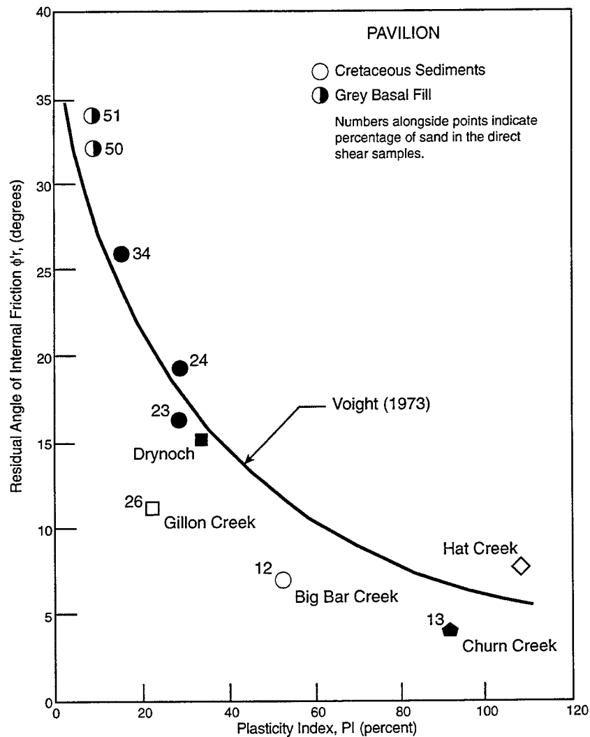
Figure 2.10 Relationship between residual friction angle and plasticity index (Bovis, 1985)
