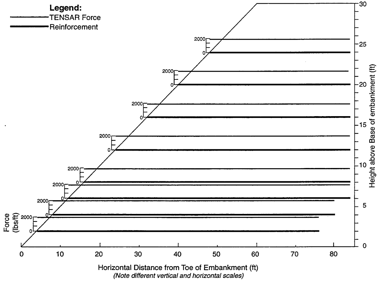
Figure 5.7 TENSAR recommended tensile forces for reinforcement
