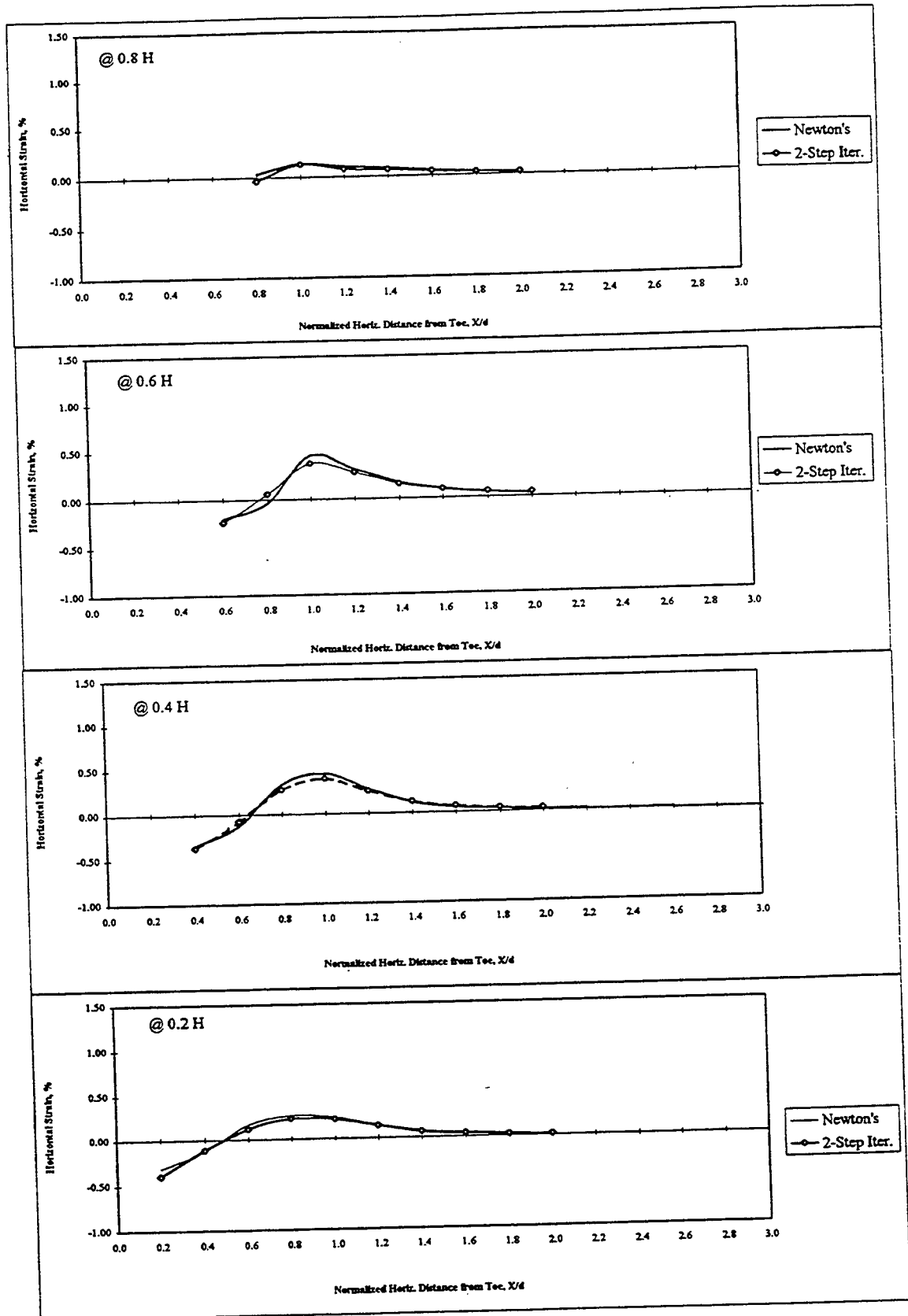
Figure A.26 Profiles of Horizontal Strains Showing Effects of Nonlinear Solution Scheme for 2:1 Slope and a Slope Height of 10 Feet.
