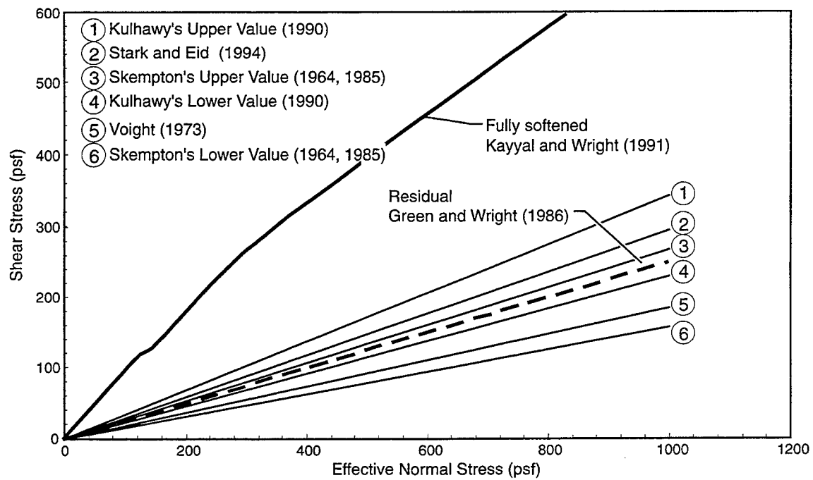
Figure 2.18a Fully softened and residual strength envelopes for Beaumont clay
