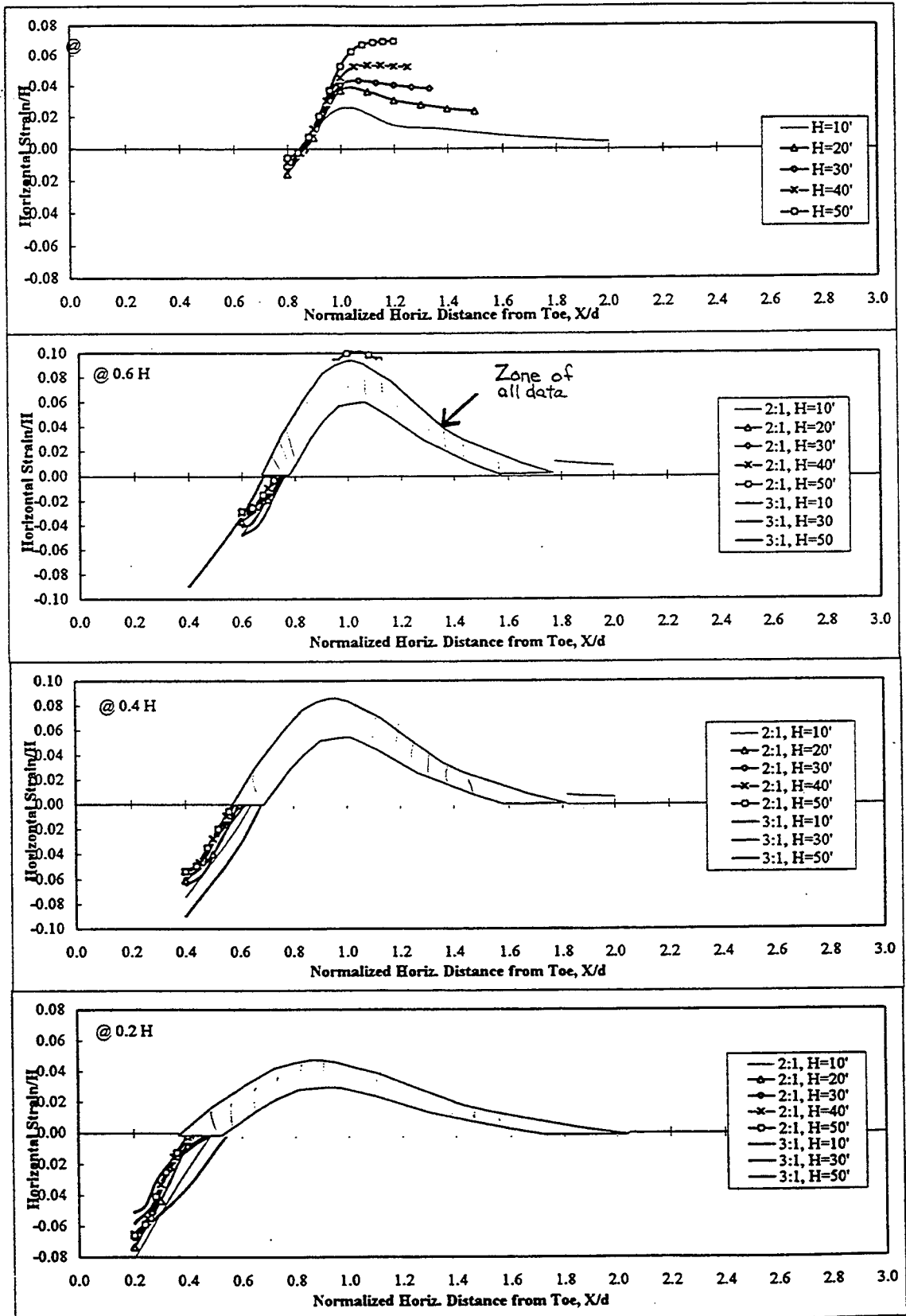
Figure A.13 Profiles of Normalized Horizontal Strains with Respect to Slope Height and Ratio
