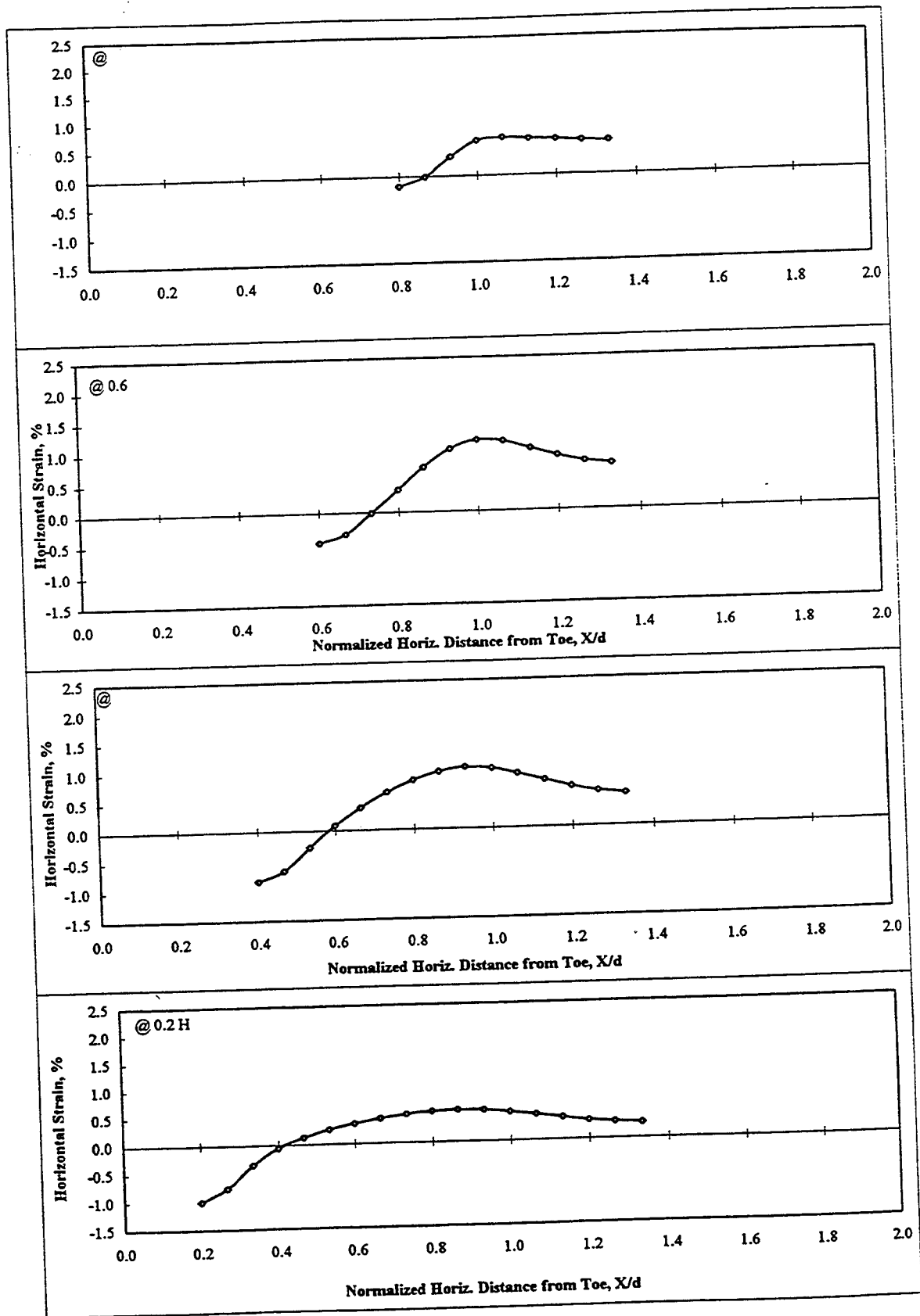
Figure A.2 Profiles of Horizontal Strains for Various Elevation Lines for 2:1 Slope and 30-foot Slope Height
