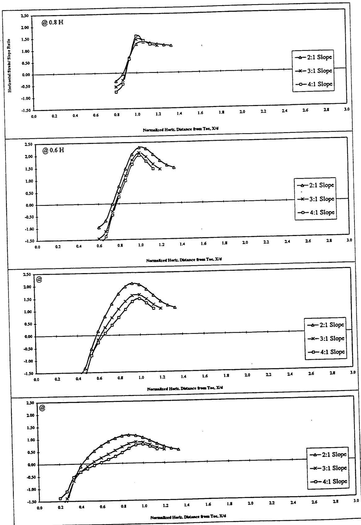
Figure A.12 Profiles of Normalized Horizontal Strains with Respect to Slope Ratio for 30-foot Height Slopes
