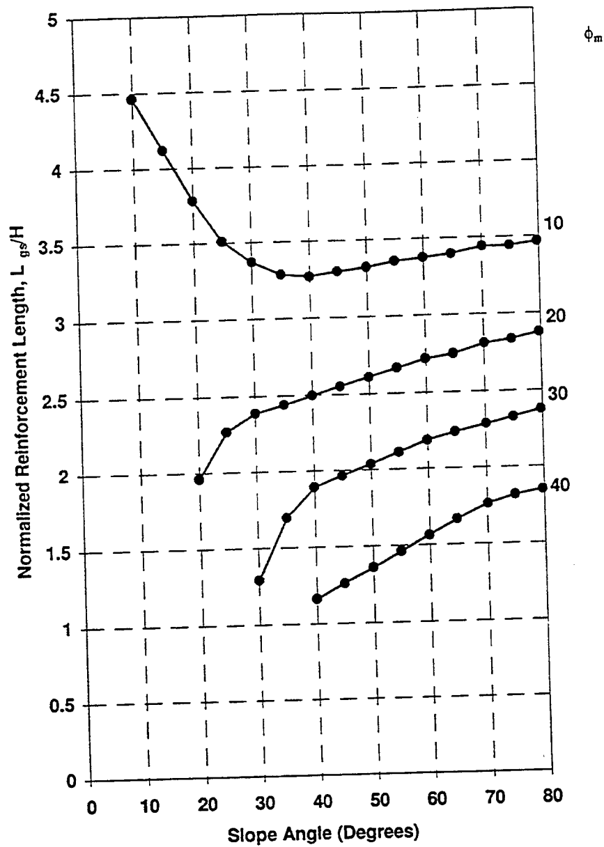
Figure B.2 Minimum Length of Reinforcement for Global Stability of Slopes on Much Stronger Foundations — r_u = 0.5
