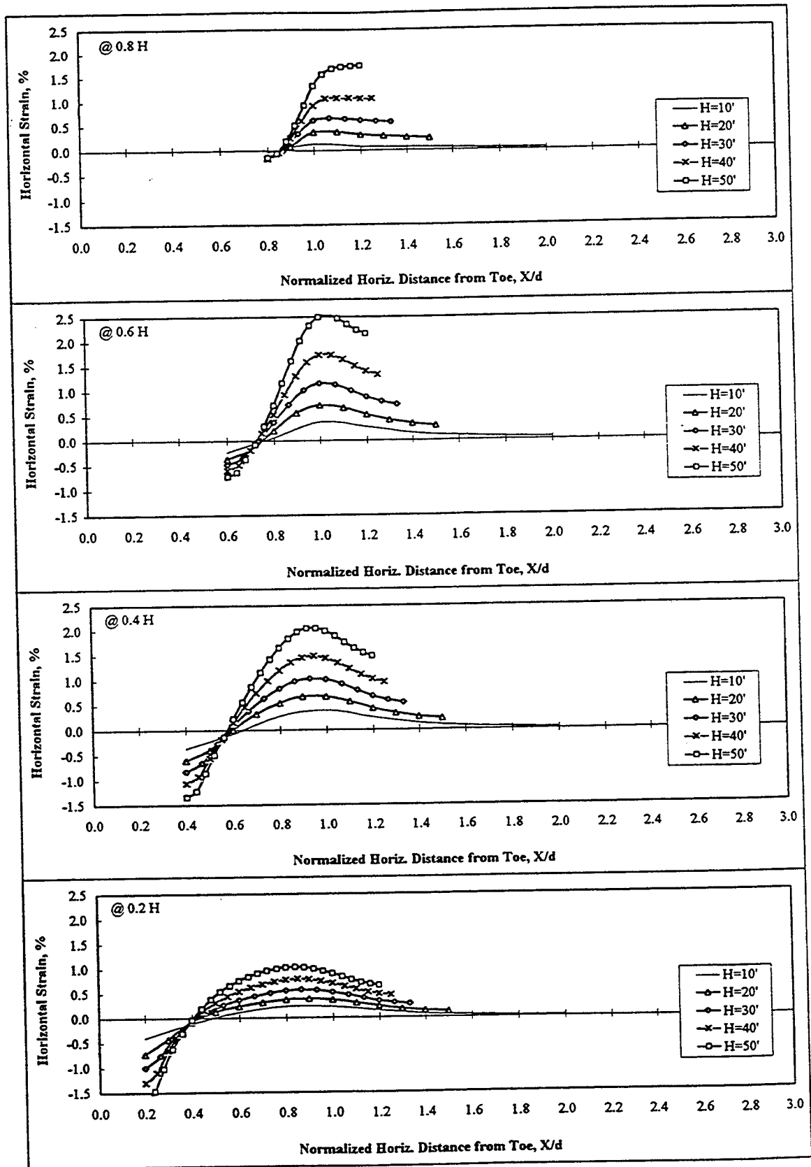
Figure A.3 Profiles of Horizontal Strains Along Various Elevation Lines for 2:1 Slope
