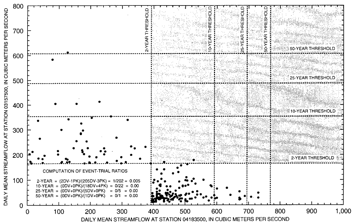
Figure 4a. Concurrent daily mean streamflows for stations 03157500 and 04183500.
