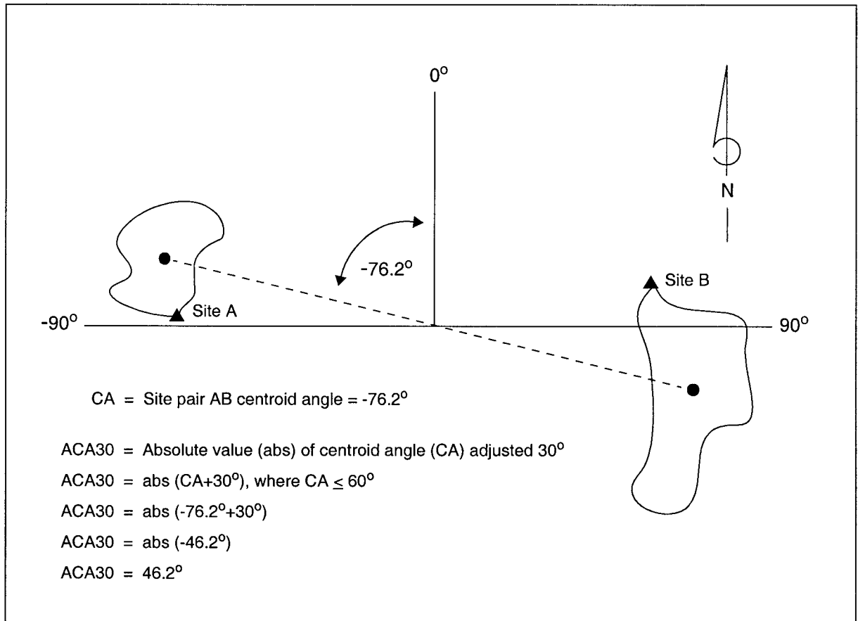
Figure 8. Diagram showing measurement of centroid angle (CA) and computation of absolute value of centroid angle adjusted 30 degrees (ACA30) for hypothetical site pair AB.
