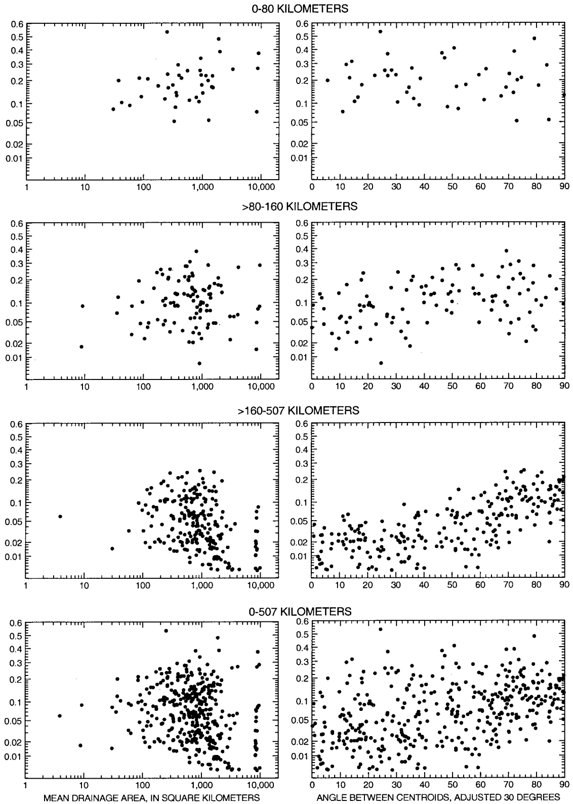
Figure 11. Event-trial ratios for the 2-year flood threshold plotted as a function of mean drainage area and adjusted centroid angle, for selected ranges of centroid distance among 30 sites in Ohio and border areas of adjacent states.
