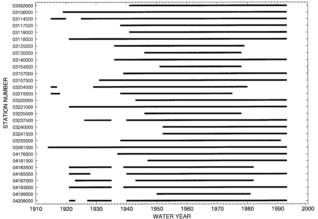
Figure 2. Individual and concurrent lengths of daily mean streamflow record for the 30 study sites in Ohio and border areas of adjacent states.
