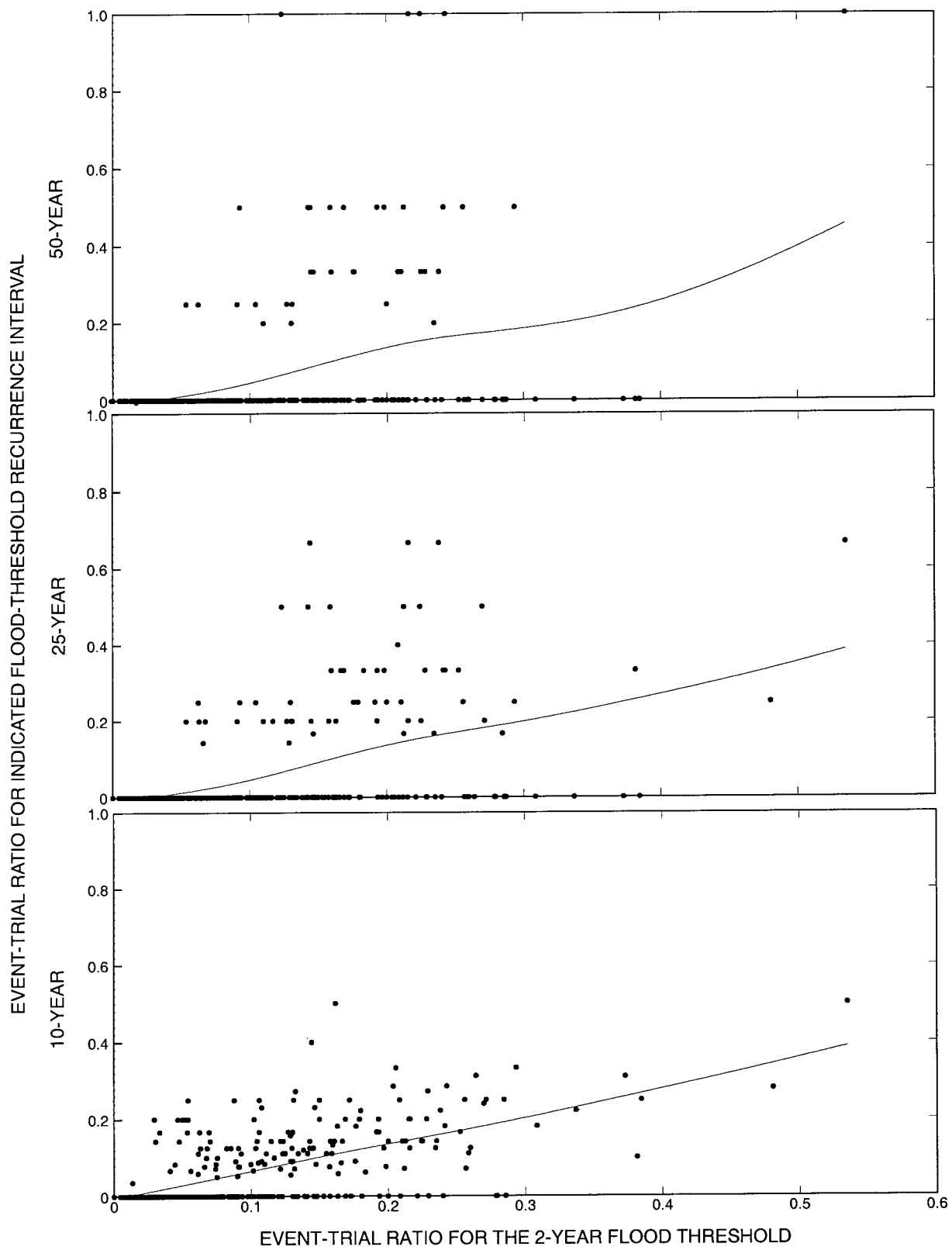
Figure 6. Relation between 2-year event-trial ratios and 10-, 25-, and 50-year event-trial ratios for the 30 study sites in Ohio and border areas of adjacent states.
