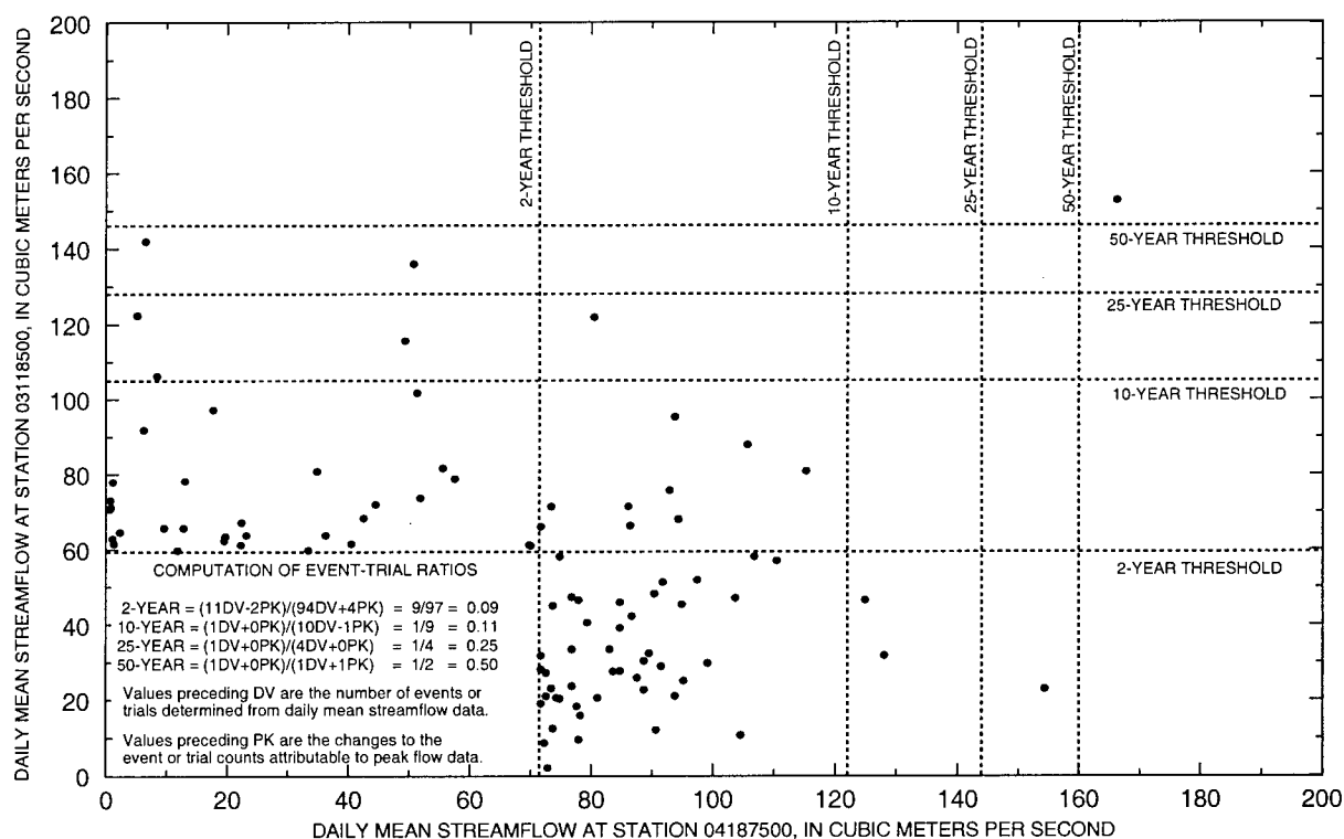
Figure 4b. Concurrent daily mean streamflows for stations 03118500 and 04187500.
