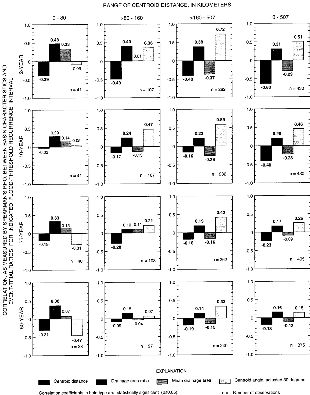
Figure 9. Correlation between event-trial ratios and selected basin characteristics grouped by centroid distance and flood-threshold recurrence interval.
