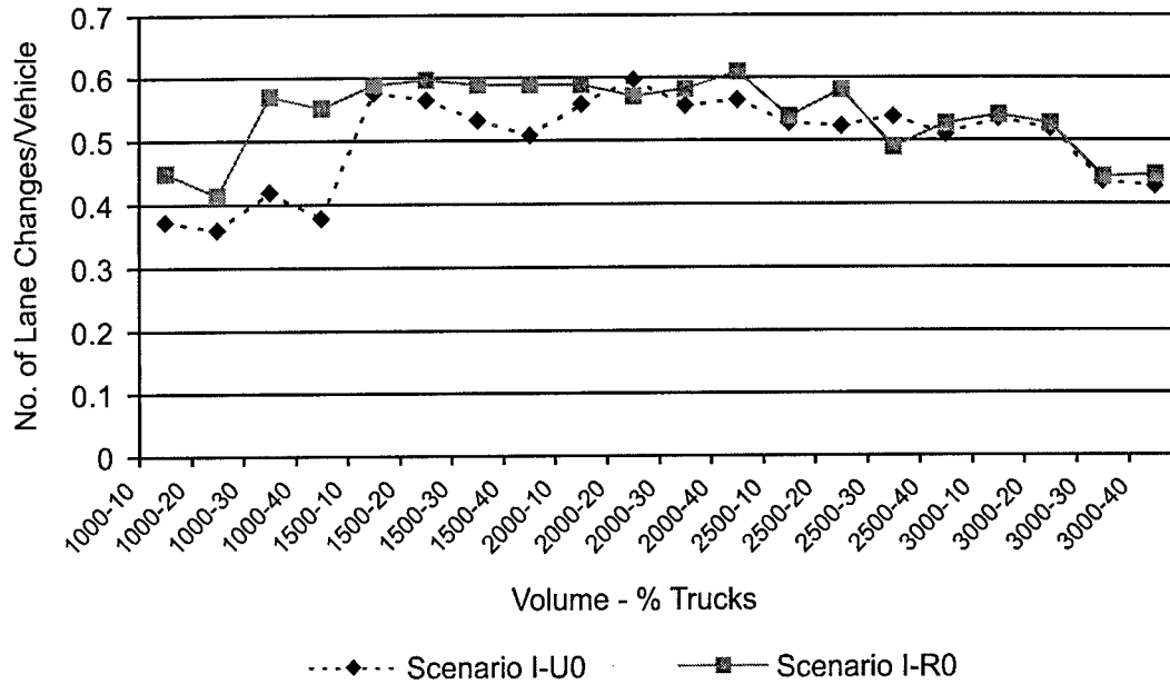
Figure 2. Scenario I-U0 vs. Scenario I-R0 for Lane Changes
