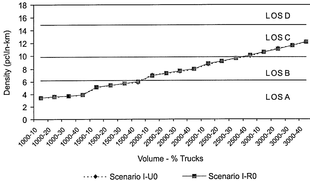
Figure 1. Scenario I-U0 vs. Scenario I-R0 for Density
