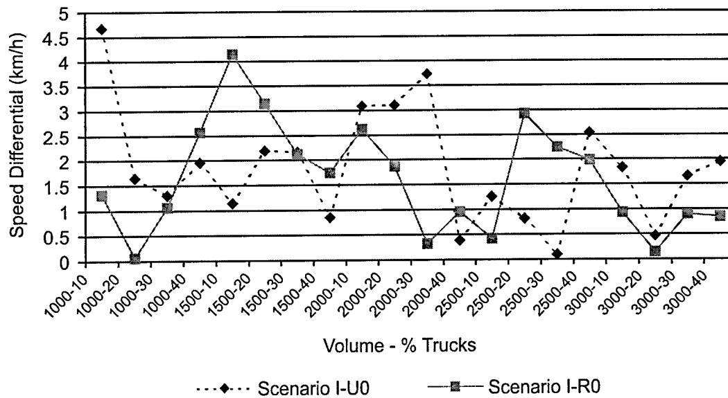
Figure 3. Scenario I-U0 vs. Scenario I-R0 for Speed Differential
