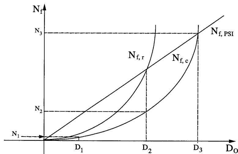
Figure 5.1: Conceptual diagram determined by rutting and cracking criteria and PSI criterion.
