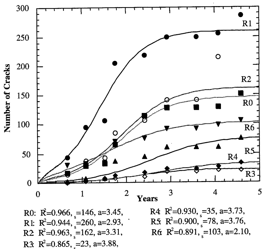
Figure 3.6: Evolution of cracks in overlays on rigid sections considering the initial rate of cracking.
