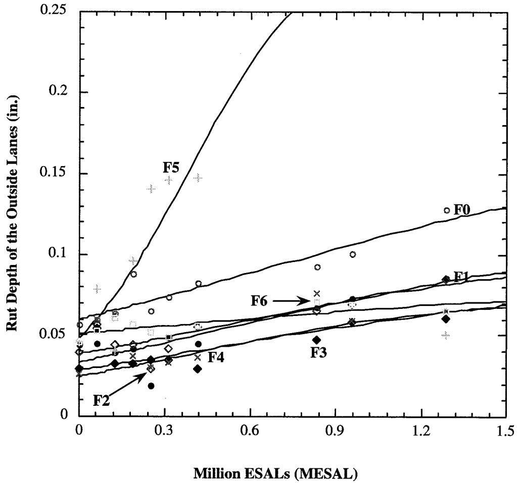
Figure 4.2: Rut depth of the outside lanes of flexible sections
