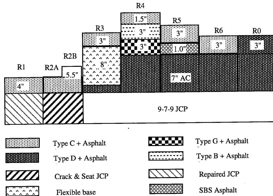
Figure 1.1: Overlay cross sections for rigid pavement (Note: 1 in.=25.4 mm).
