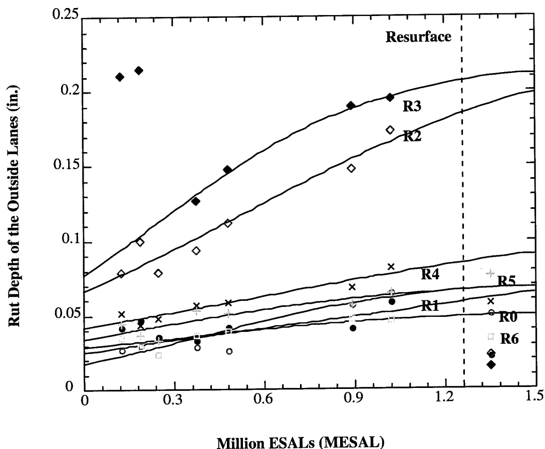
Figure 4.1: Rut depth of the outside lanes of rigid sections.
