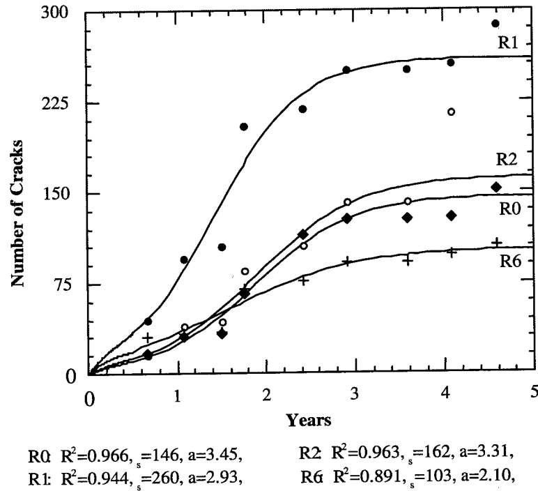
Figure 3.4: Evolution of cracks in overlays on R0, R1, R2, and R6 sections considering the initial rate of cracking.
