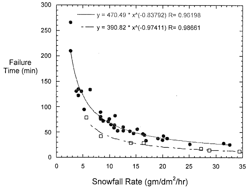
FIGURE 13. COMPARISON OF UNIVERSITY OF QUEBEC AT CHICOUTIMI (UQAC) OUTDOOR TESTS OF ULTRA+ NEAT (-0.5 TO -11.8°C) (SOLID DOTS) TO THE NCAR INDOOR TESTS AT -10°C (OPEN SQUARES)
