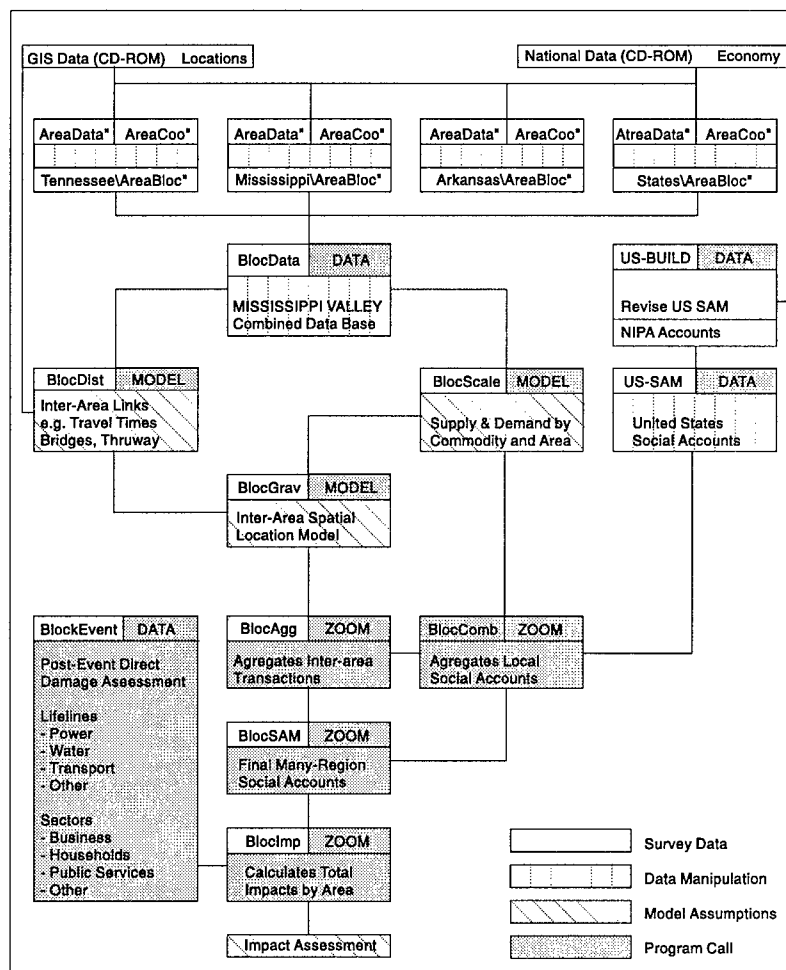
■ Figure 8.1 Flow Diagram for Mississippi Valley Model Programs
