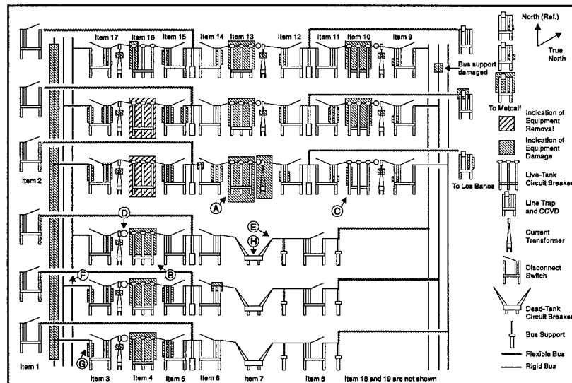
■ Figure 3.3 Damaged Equipment of Moss Landing 500kv Switchyard at the 1989 Loma Prieta Earthquake
