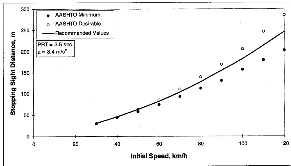
Figure 2-1. Comparison of 1994 AASHTO and Recommended Values for Stopping Sight Distance (3)
