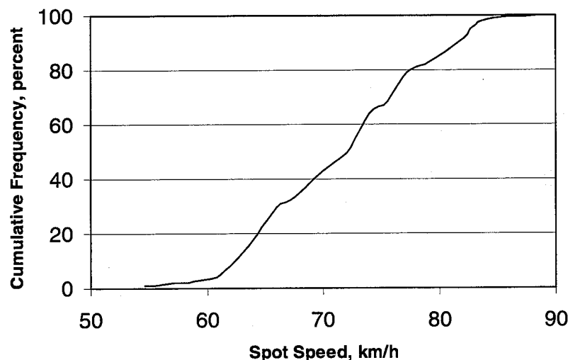
Figure 3-2. Spot Speed Study, Case Study A
