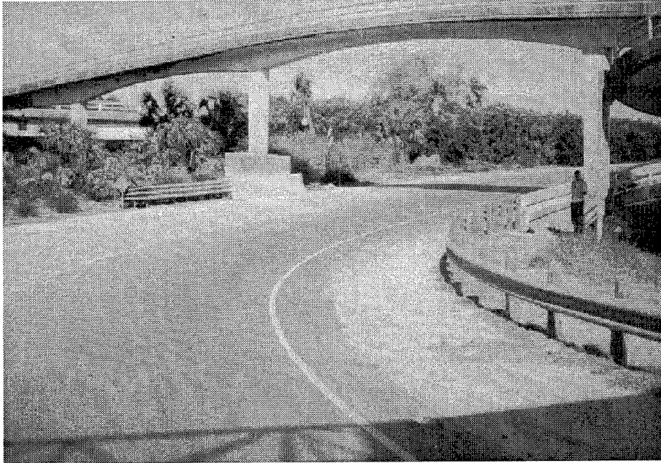
Figure 3-3. Case Study B, Horizontal Curvature
