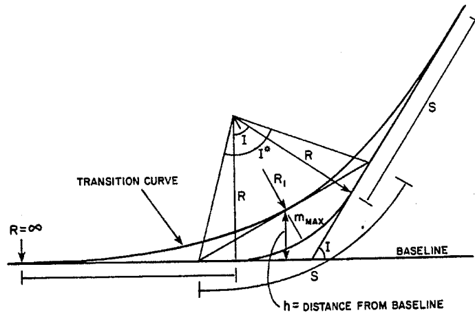
Figure 2-1. Transition Curve for Lateral Clearance (4)
