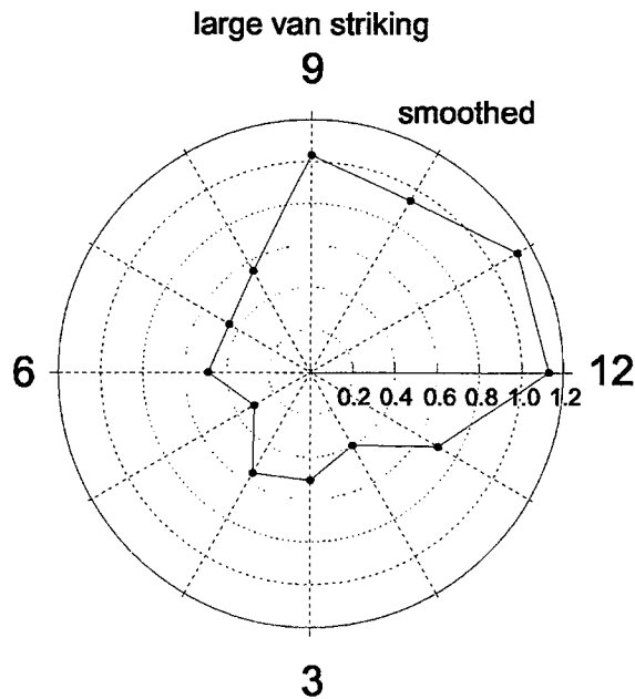
Figure 4.3-8. r(i) for the Drivers of Cars Being Struck by Large Vans. The Utility Vehicles Have Impact Points 11, 12, or 1. The Cars Have Impact Points Shown by the Clock Positions. Points Are Obtained by 3-point Weighted Moving Averaging.
