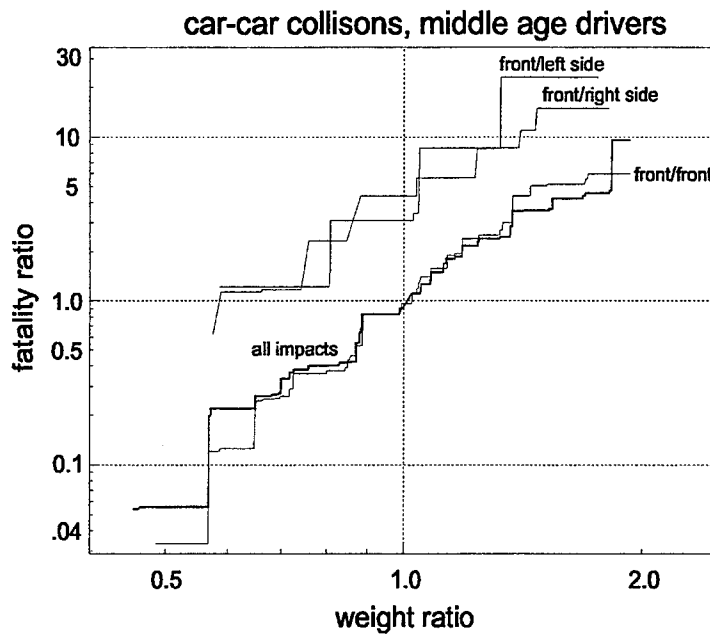
Figure 4.2-3. Ratio of Driver Fatalities in Collisions Between Two Cars, by Weight Ratio and Collision Configuration. Drivers 26 to 49 Years Old.
