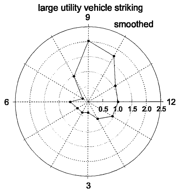
Figure 4.3-6. r(i) for the Drivers of Cars Being Struck by Large Utility Vehicles. The Utility Vehicles Have Impact Points 11, 12, or 1. The Cars Have Impact Points Shown by the Clock Positions. Points Are Obtained by 3-point Weighted Moving Averaging.
