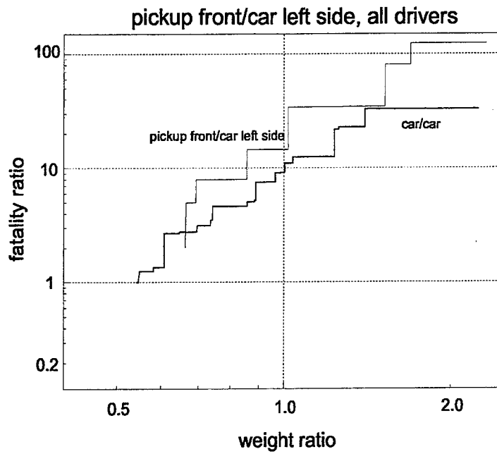
Figure 4.2-8. Ratio of Driver Fatalities in Front-left Side Collisions Between Pickup Trucks and Cars, and Collisions Between Two Cars, by Ratio of the Weights of the Pickup Truck and the Car.
