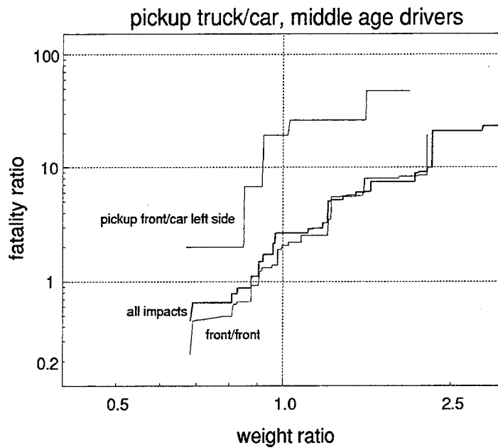
Figure 4.2-4. Ratio of Car Driver Fatalities to Pickup Truck Driver Fatalities in Collisions Between a Car and a Pickup Truck, by Ratio of the Weight of the Pickup Truck and the Car, and Collision Configuration.
