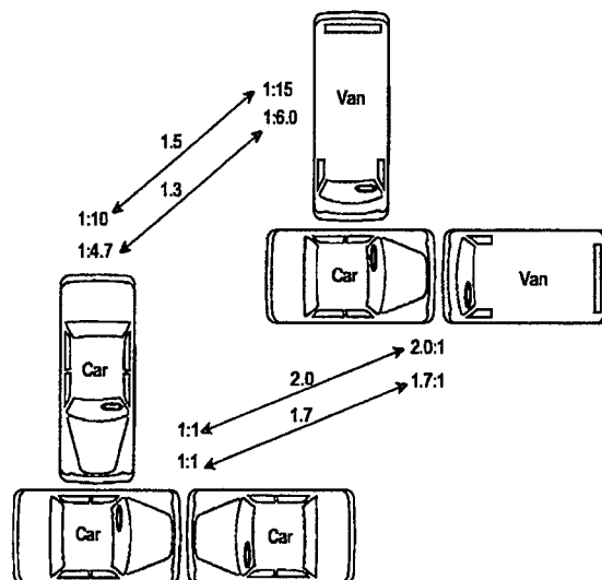
Figure 4.2-16. Comparing Collisions Between Vans and Cars of the Same Weight, with Collisions Between Cars of the Same Weights.
