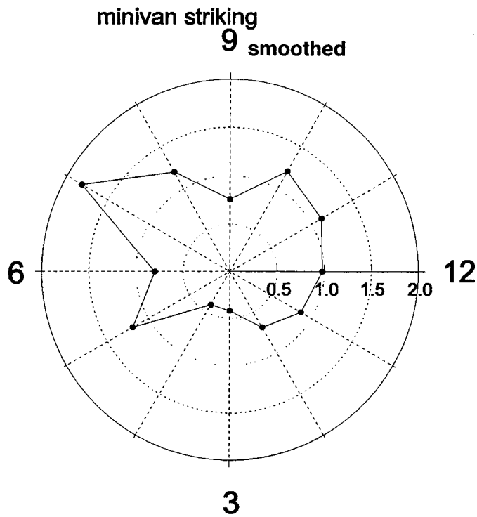
Figure 4.3-7. r(i) for the Drivers of Cars Being Struck by Minivans. The Utility Vehicles Have Impact Points 11, 12, or 1. The Cars Have Impact Points Shown by the Clock Positions. Points Are Obtained by 3-point Weighted Moving Averaging.
