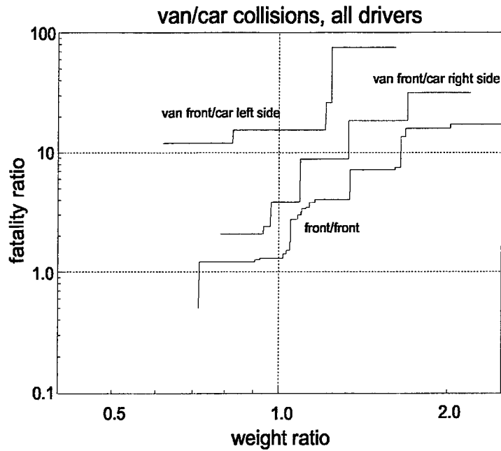
Figure 4.2-12. Ratio of Driver Fatalities in Collisions Between Vans and Car, by Vehicle Weight Ratio and Collision Configuration.
