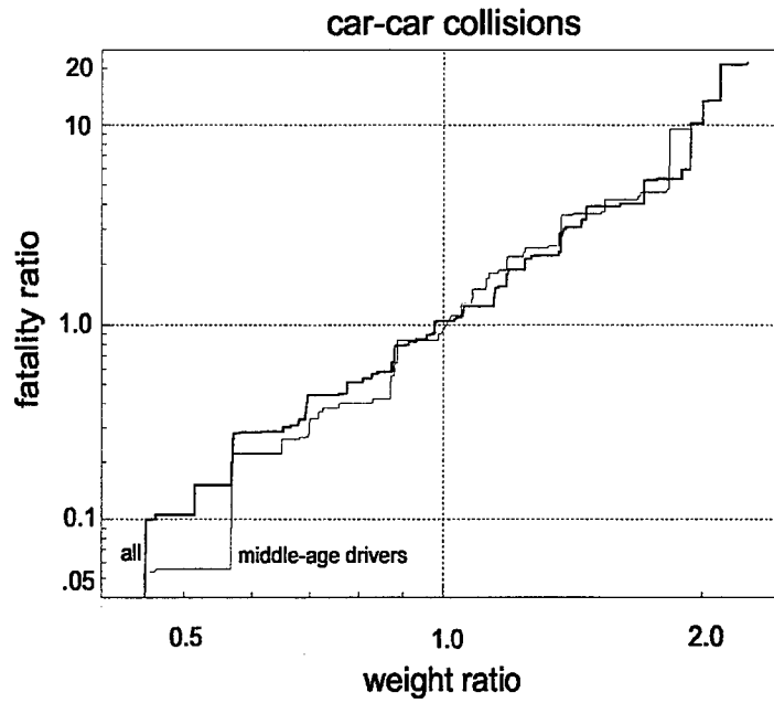
Figure 4.2-2. Ratio of Driver Fatalities in Collisions Between Two Cars, by Weight Ratio of the Cars, for All Drivers, and Drivers 26 to 49 Years Old. All Collision Configurations.
