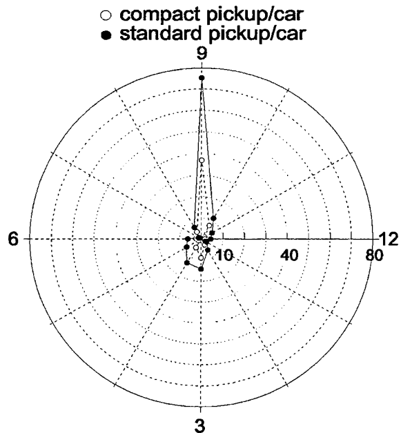
Figure 4.3-2a. Ratio of Driver Fatalities in Cars Struck to Those in Striking Pickup Trucks, for Compact and for Standard Pickup Trucks. The Striking Pickup Trucks Have Impact Points 11, 12, or 1, the Struck Cars Have Impact Points Shown by the Clock Positions.
