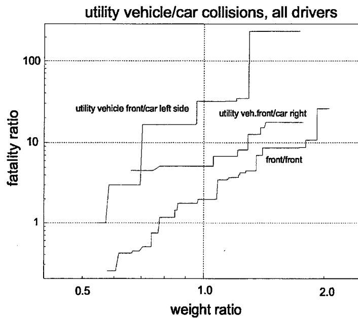
Figure 4.2-10. Ratio of Driver Fatalities in Collisions Between Utility Vehicle and Car, by Vehicle Weight Ratio and Collision Configuration.
