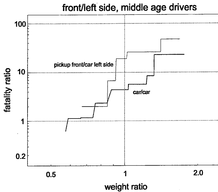
Figure 4.2-8. Ratio of Driver Fatalities in Front-left Side Collisions Between Pickup Trucks and Cars, and Collisions Between Two Cars, by Ratio of the Weights of the Pickup Truck and the Car.
