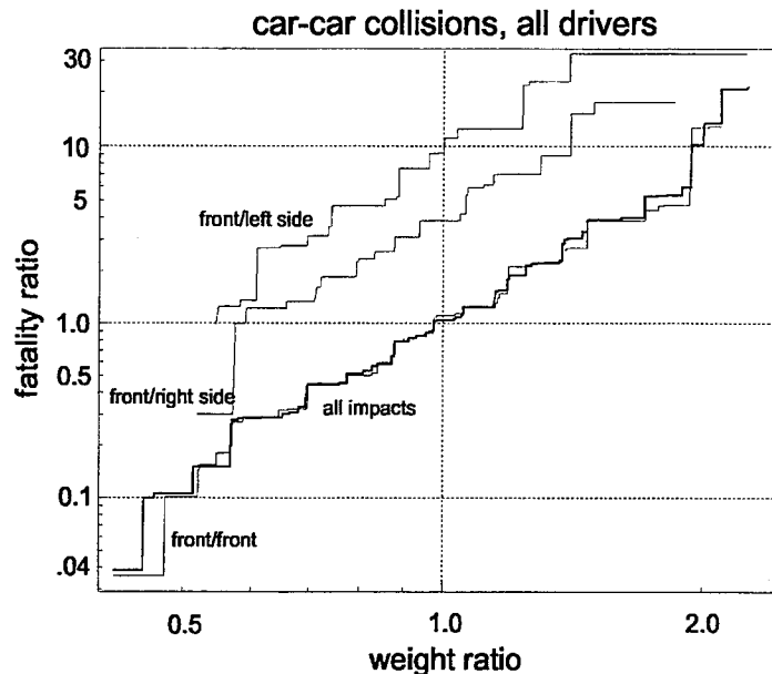
Figure 4.2-1. Ratio of Driver Fatalities in Collisions Between Two Cars, by Weight Ratio of the Cars, and Collision Configuration.
