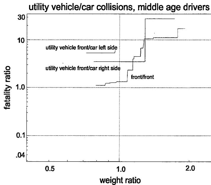
Figure 4.2-11. Ratio of Driver Fatalities in Collisions Between Utility Vehicle and Car, by Vehicle Weight Ratio and Collision Configuration, Middle Age Driver.
