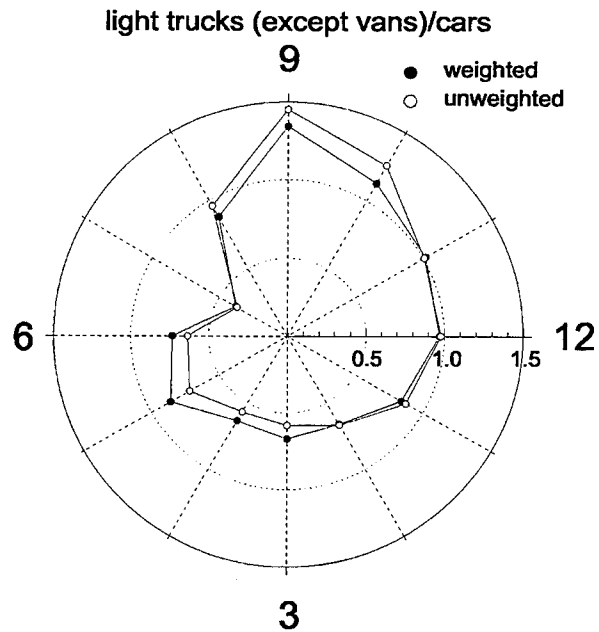
Figure 4.3-9. Averages of the r(i) Shown in Figures 4.3-3b, 4.3-4b, 4.3-5 and 4.3-6. Solid Dots Show Average Weighted with the Number of Collisions, Open Dots Show Averages with Equal Weights.
