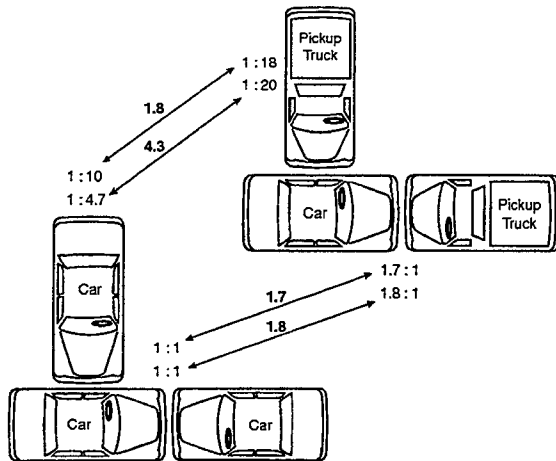
Figure 4.2-14. Comparing Collisions Between Pickup Trucks and Cars of the Same Weight, with Collisions Between Cars of the Same Weight.
