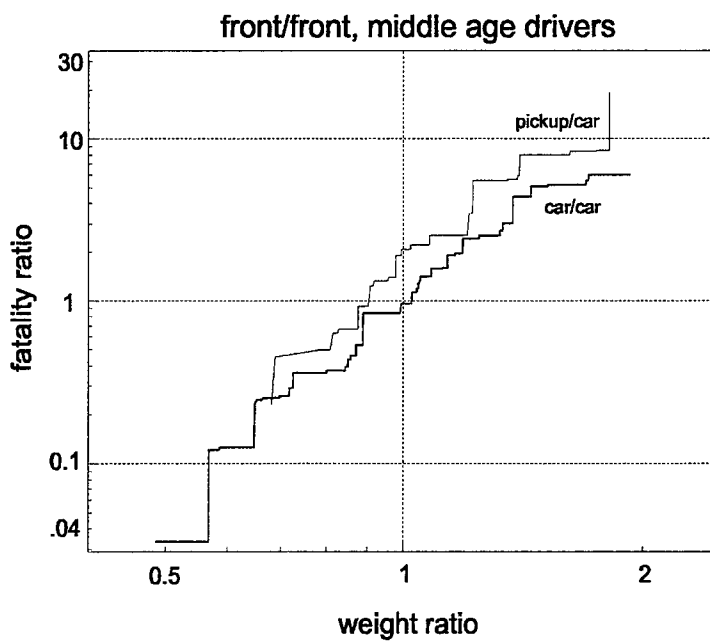
Figure 4.2-7. Ratio of Driver Fatalities in Front-front Collisions Between a Pickup Truck and a Car, and Collisions Between Two Cars, by Ratio of the Weights of the Vehicles. Drivers 26 to 49 Years Old.
