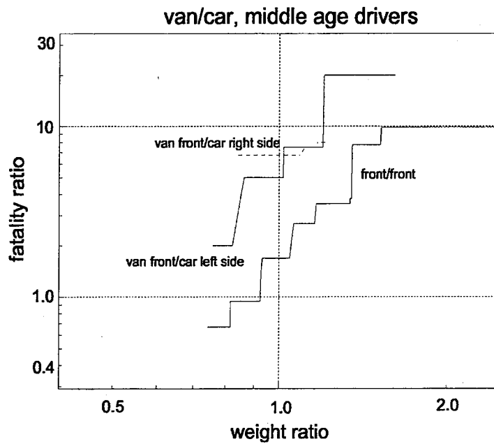
Figure 4.2-13. Ratio of Driver Fatalities in Collisions Between Vans and Cars, by Vehicle Weight Ratio and Collision Configuration, Middle Age Driver.
