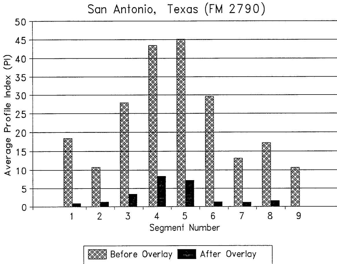
Figure 3. Measured Profile Indices on San Antonio Test Sections
