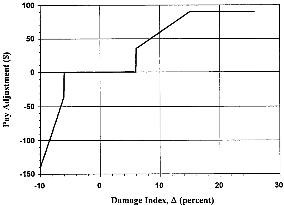
Figure 43. Pay Adjustment Schedule Based on a Tolerance Band of \pm 6 Percent on \Delta
