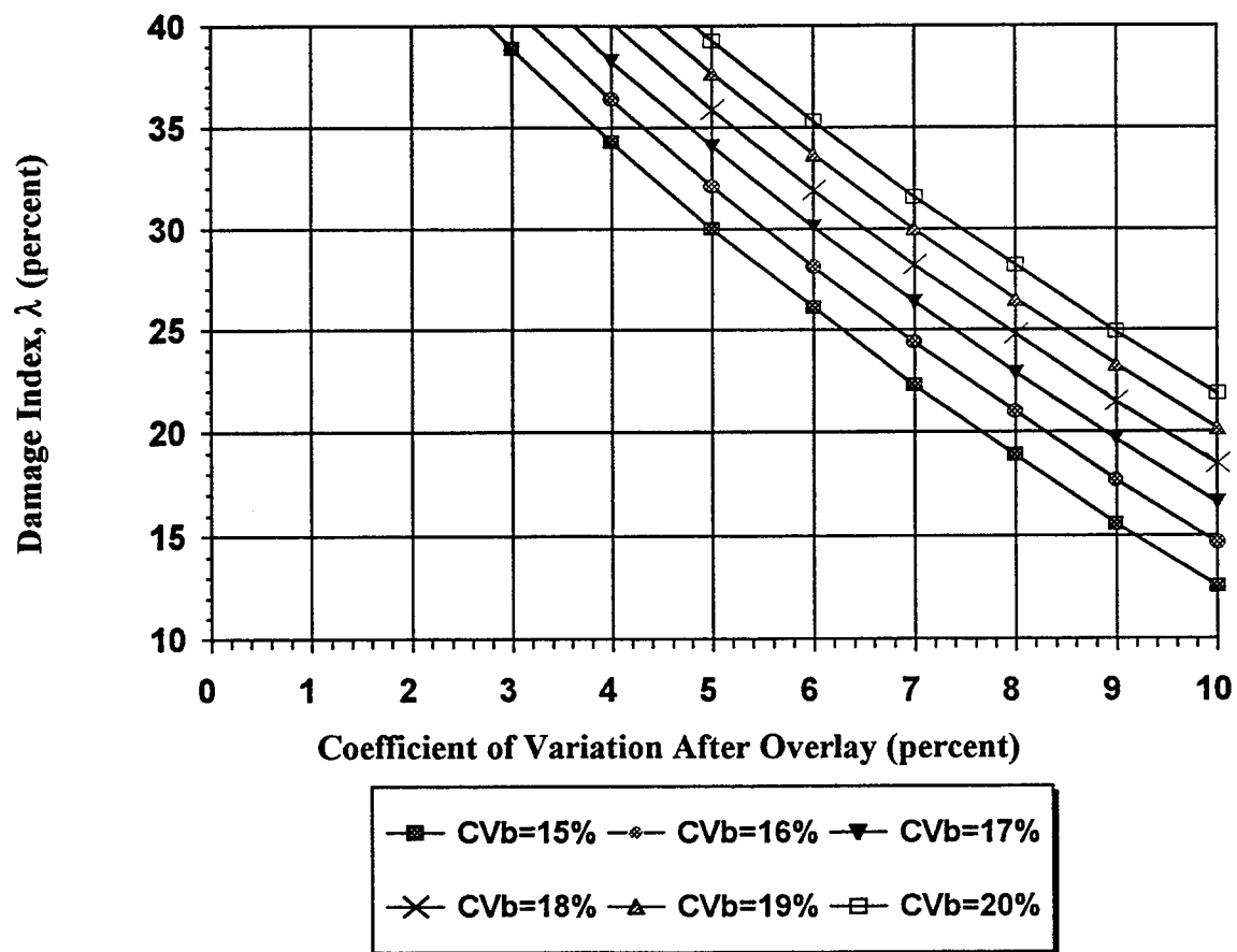
Figure 39. Chart to Evaluate Surface Smoothness Using Group A Test Methods for Coefficients of Variation Before the Overlay Between 15 and 20 Percent
