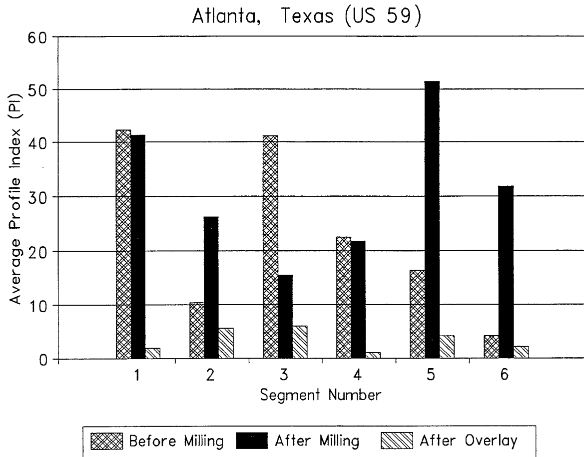
Figure 2. Measured Profile Indices on Atlanta Test Sections
