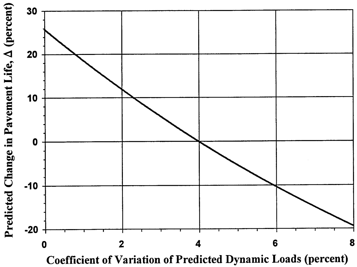
Figure 34. Relationship Between CV and Damage Index, \Delta
