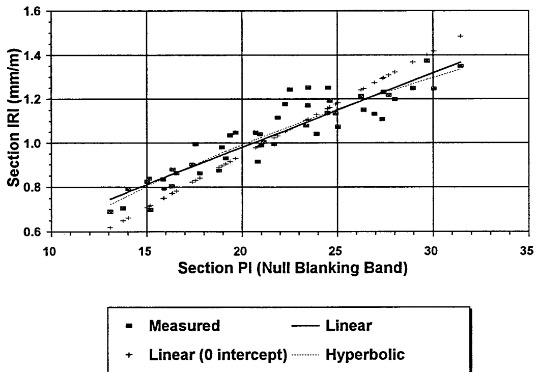
Figure 28. Comparison of Different Relationships Between IRI and PI_0
