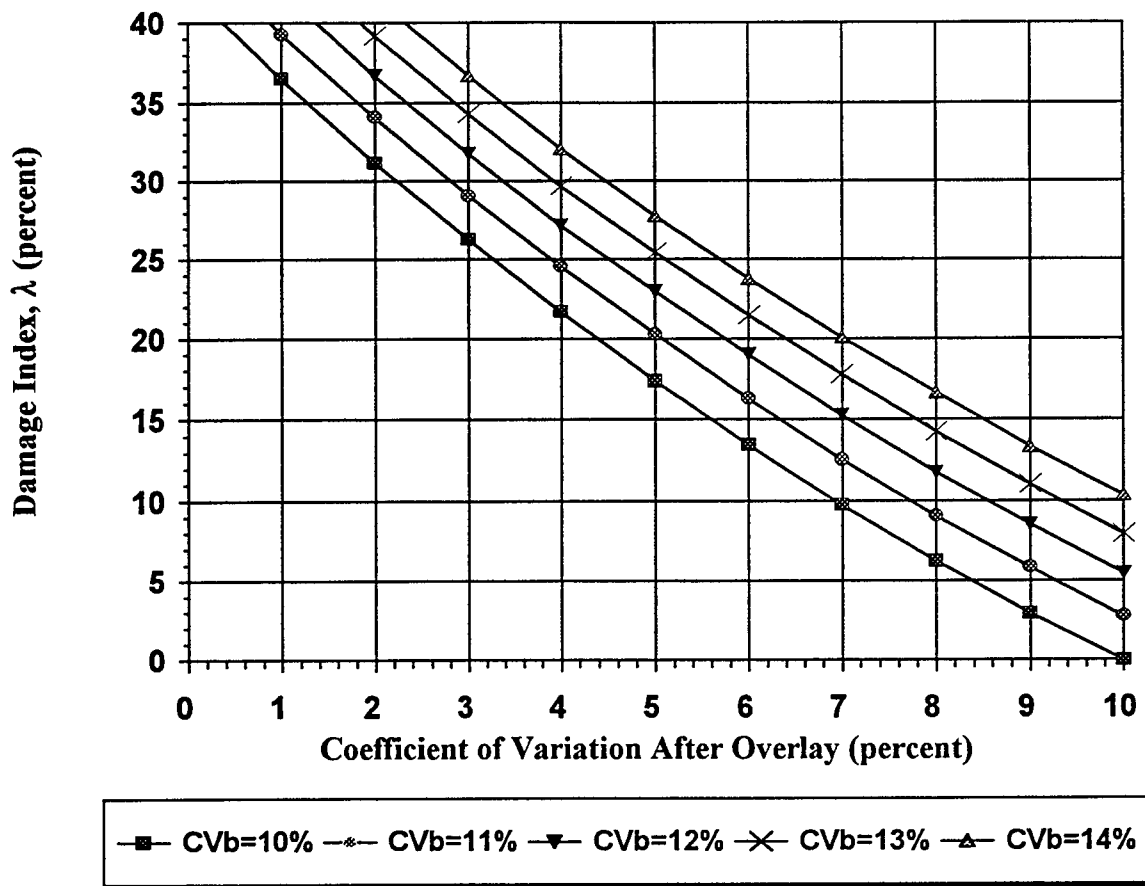
Figure 38. Chart to Evaluate Surface Smoothness Using Group A Test Methods for Coefficients of Variation Before the Overlay Between 10 and 14 Percent
