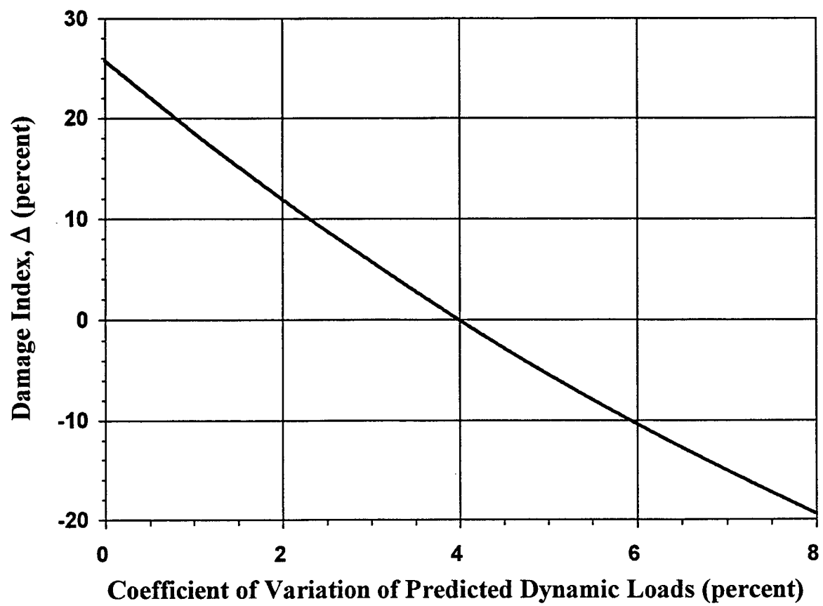
Figure 42. Relationship Between CV and Predicted Change in Pavement Life, \Delta
