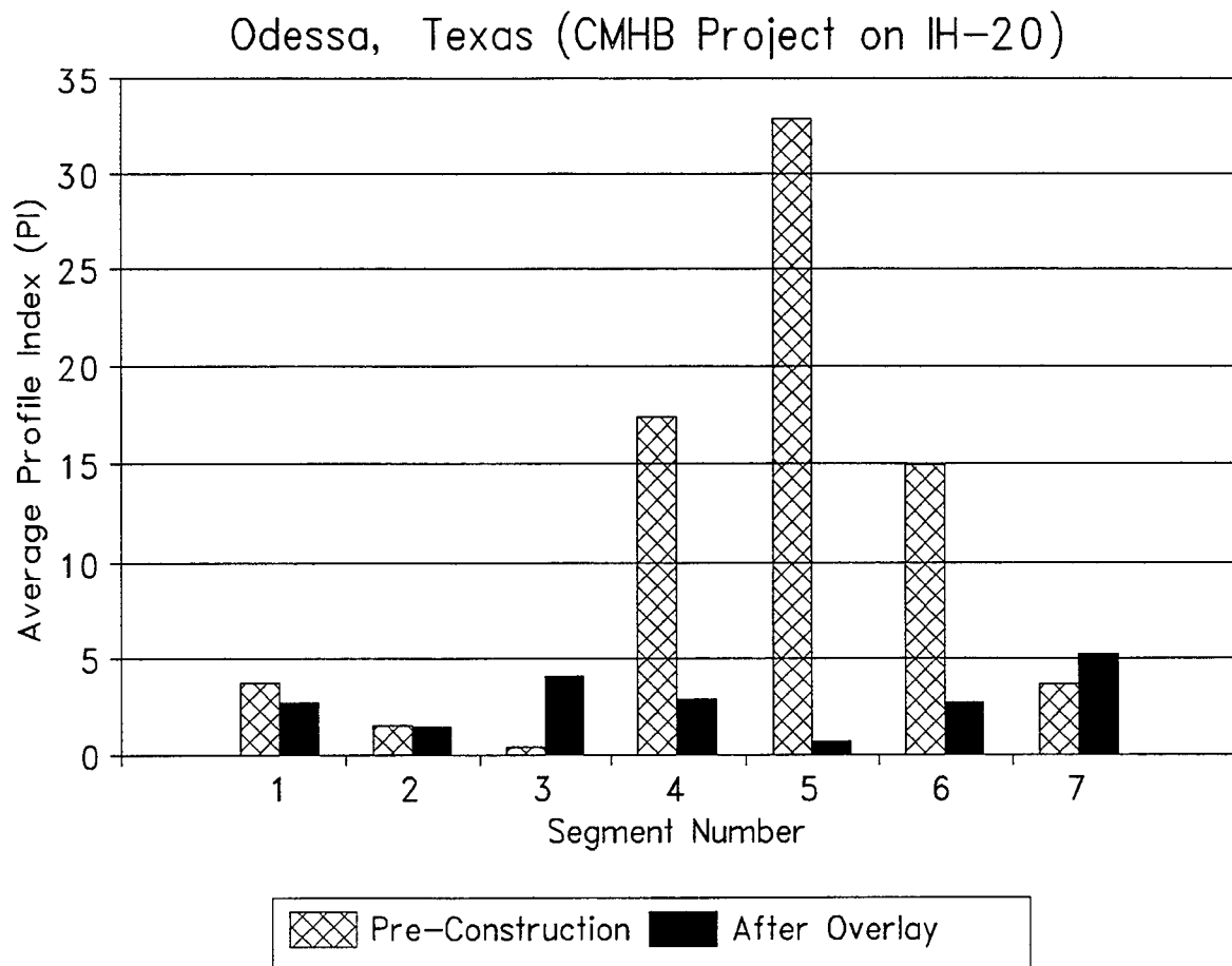
Figure 5. Measured Profile Indices on Odessa CMHB Test Sections
