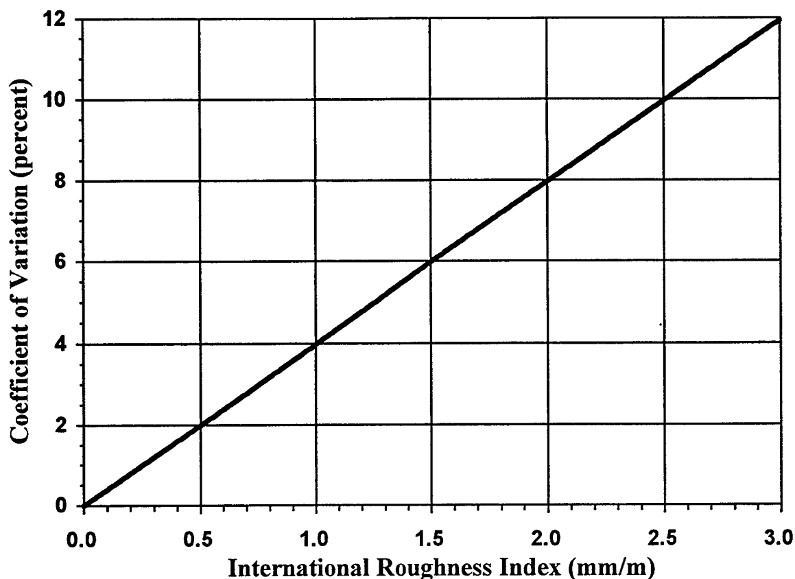
Figure 40. Chart to Estimate the Coefficient of Variation of Predicted Dynamic Loads Using IRI for a Vehicle Speed of 97 kph
