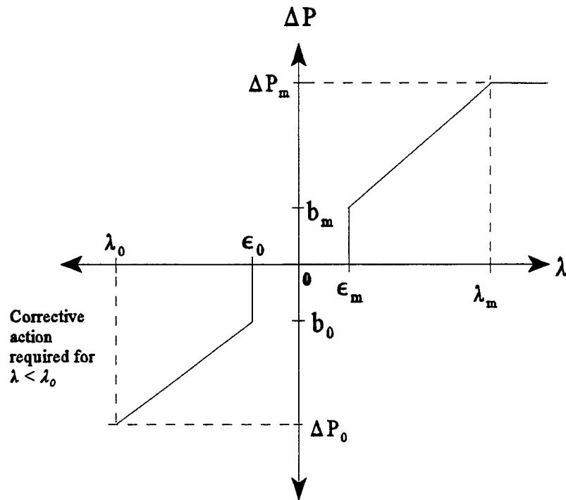
Figure 20. Illustration of Proposed Approach to Determine Pay Adjustments Based on \lambda
