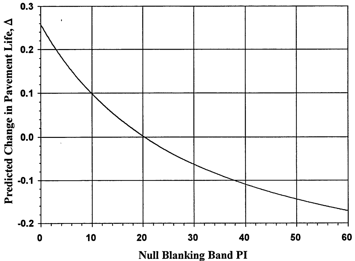
Figure 30. Predicted Change in Pavement Life Due to Departures from Target Smoothness of the Final Overlay (Paris n of 3.6 and 95 Percent Confidence Level Used)
