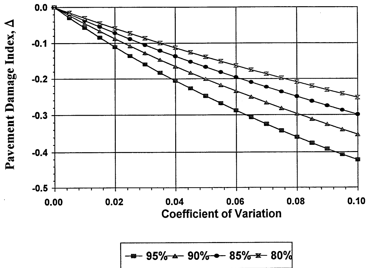
Figure 17. Values of \Delta for Different Levels of Dynamic Load Variability and Confidence Levels ( CV_0=0 and n=3.6 )
