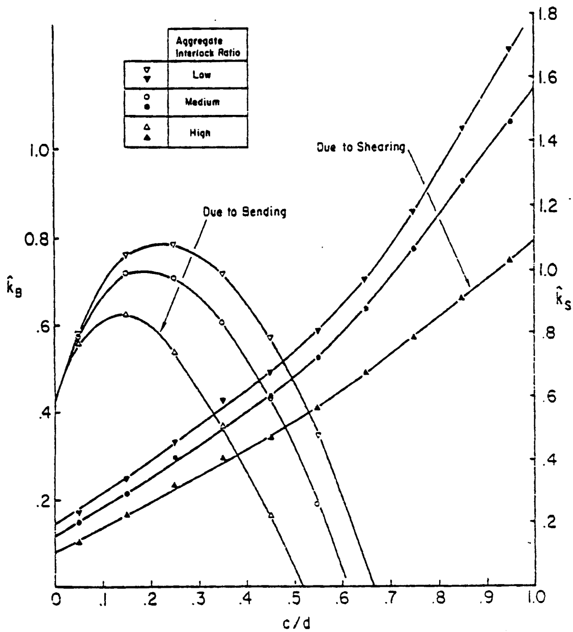
Figure A2. Non-dimensionalized Stress Intensity Factors Due to Bending and Shear (Jayawickrama, 1985)
