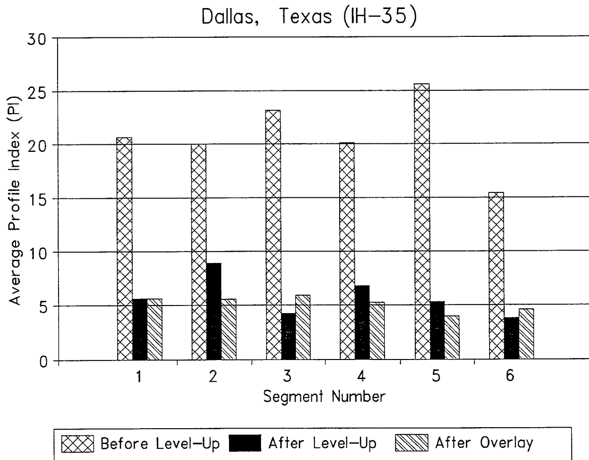
Figure 7. Measured Profile Indices on Dallas Test Sections
