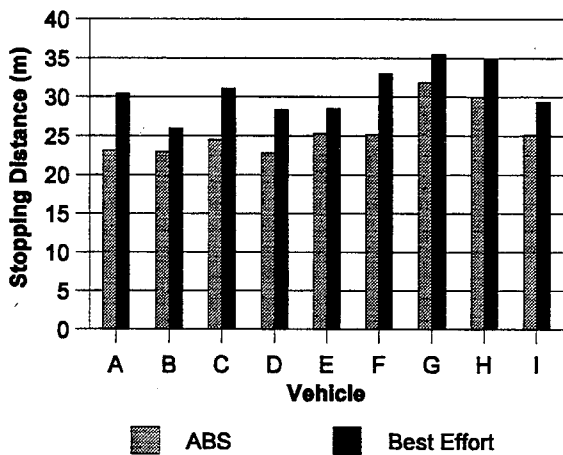
Figure A3. Straight line stopping distances observed on wet polished concrete. Test vehicles were lightly laden. Test speed was 64 km/h (40 mph).
