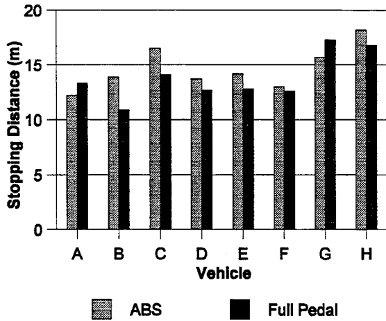
Figure A9. Straight line stopping distances observed on grass. Test vehicles were lightly laden. Vehicle “T” braking performance was not evaluated. Test speed was 40 km/h (25 mph).
