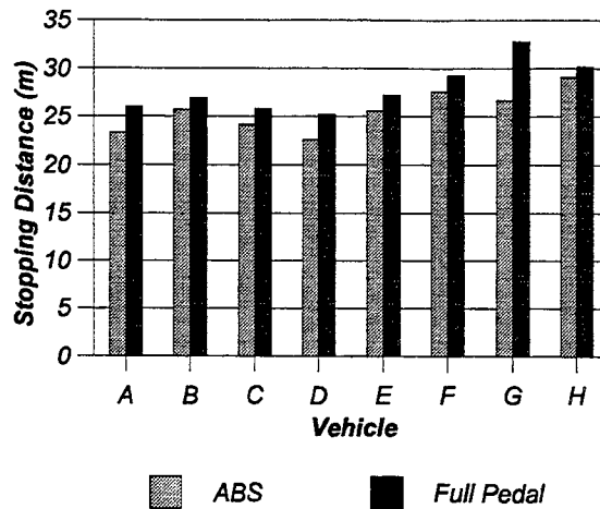
Figure 15. Straight line stopping distances observed on ABS Test Pad #3 (wet). Test vehicles were fully laden to their respective GVWRs. Vehicle “T” braking performance was not evaluated.
