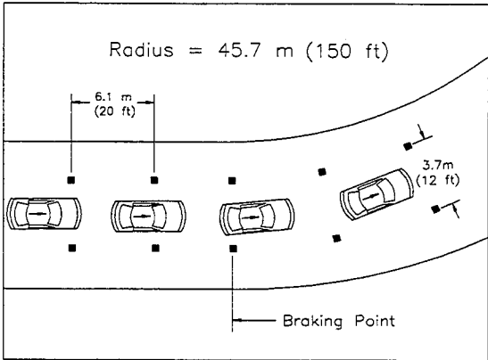
Figure 6. J-turn maneuver. Approach is tangent to a 45.7 m (150 ft) radius curve.
