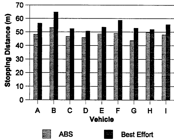
Figure A2. Straight line stopping distances observed on dry concrete. Test vehicles were fully laden to their respective GVWRs. Test speed was 97 km/h (60 mph).
