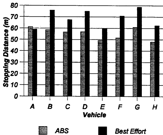
Figure A31. Stopping distances observed on the 152.4 m (500 ft) wet Jennite curve. Test vehicles were lightly laden. Test speed was 64 km/h (40 mph). Vehicle "T" braking performance was not evaluated.
