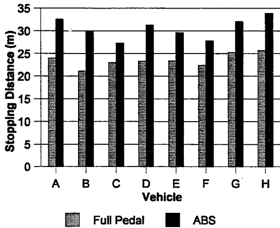
Figure A11. Straight line stopping distances observed on loose gravel. Test vehicles were lightly laden. Test speed was 56 km/h (35 mph). Vehicle “T” braking performance was not evaluated.
