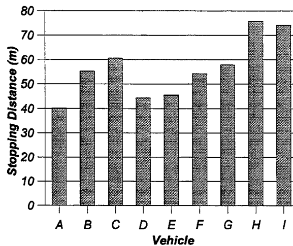
Figure 20. Wet asphalt to wet asphalt/wet epoxy split-mu single lane change stopping distances. Test vehicles were fully laden to their respective GVWRs. Note: the epoxy surface was reconditioned prior to the brake performance evaluation of vehicles "H" and "T".
