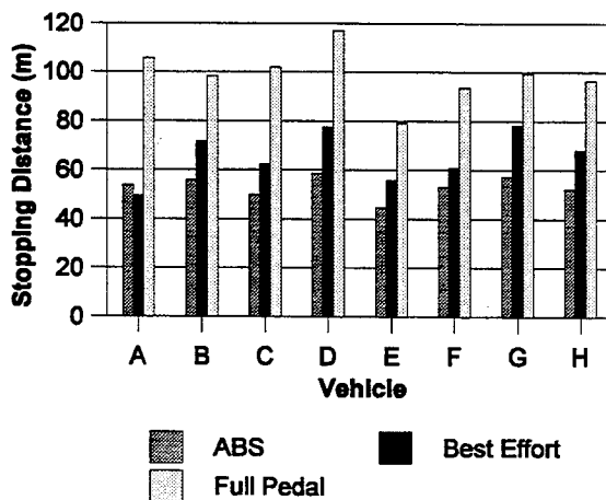
Figure A7. Straight line stopping distances observed on wet Jennite. Test vehicles were lightly laden. Test speed was 64 km/h (40 mph). Vehicle "T" braking performance was not evaluated.
