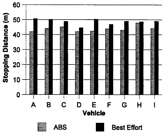
Figure A1. Straight line stopping distances observed on dry concrete. Test vehicles were lightly laden. Test speed was 97 km/h (60 mph).
