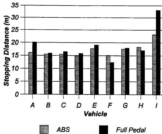
Figure 12. Straight line stopping distances observed on grass. Test vehicles were fully laden to their respective GVWRs. Note: the grass was very wet when the braking performance of vehicle “T” was evaluated.
