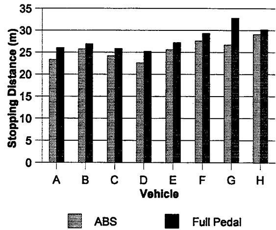
Figure A26. Straight line stopping distances observed on ABS Test Pad #3 (wet). Test vehicles were fully laden to their respective GVWRs. Test speed was 64 km/h (40 mph). Vehicle “T” braking performance was not evaluated.
