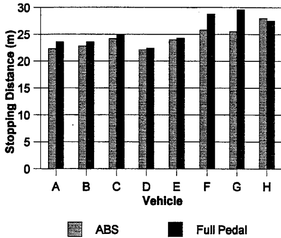
Figure A25. Straight line stopping distances observed on ABS Test Pad #3 (wet). Test vehicles were lightly. Test speed was 64 km/h (40 mph). Vehicle “T” braking performance was not evaluated.
