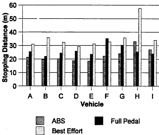
Figure A27. Straight line stopping distances observed on the wet asphalt/wet epoxy split-mu surface. Test vehicles were lightly laden. Test speed was 48 km/h (30 mph). Note: the epoxy surface was reconditioned prior to the brake performance evaluation of vehicles “H” and “T”.
