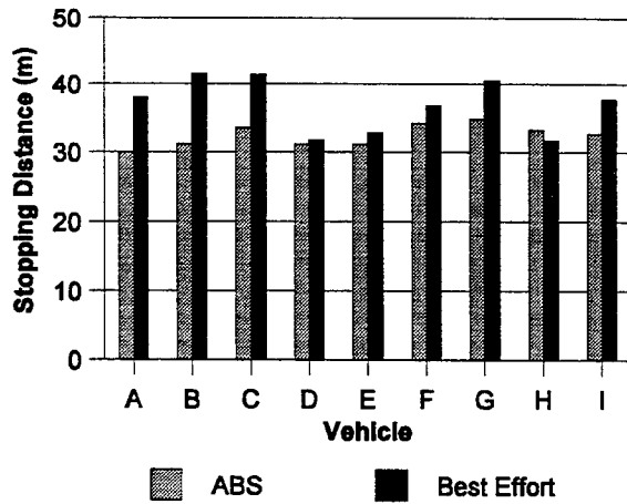
Figure A5. Straight line stopping distances observed on wet asphalt. Test vehicles were lightly laden. Test speed was 80 km/h (50 mph).
