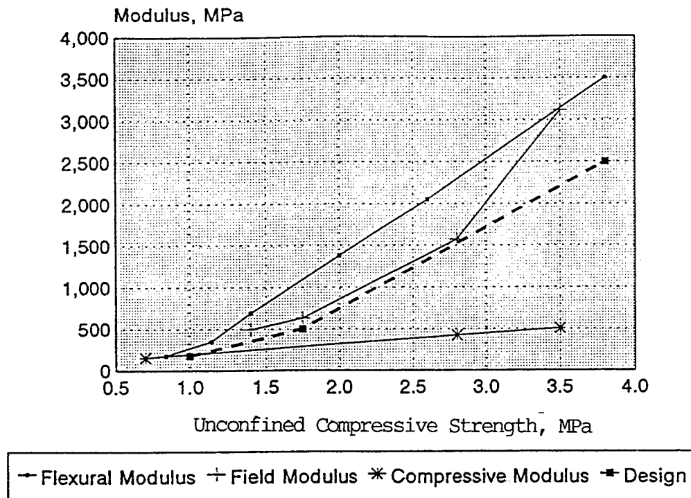
Figure 2. Relationships Between Unconfined Compressive Strength and Moduli of Lime-Stabilized Soils.
