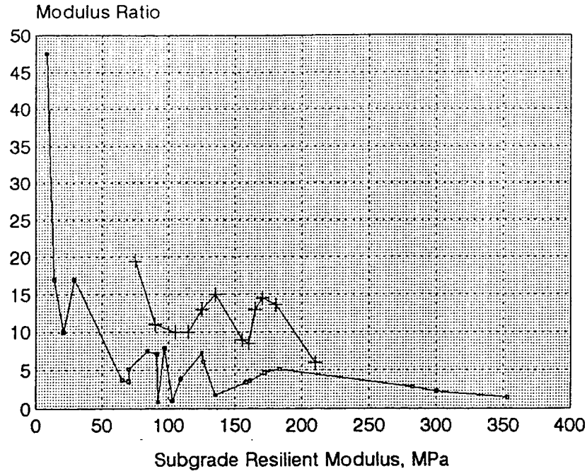
Figure 4. Relationship Between In Situ Modulus of the Natural Subgrade Soil as Determined by FWD Measurements and the Moduli Ratio (Lime-Stabilized Layer to Natural Subgrade Layer) as Determined by FWD Measurements.
