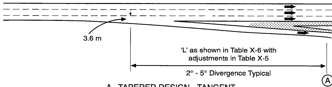
- A - TAPERED DESIGN - TANGENT
