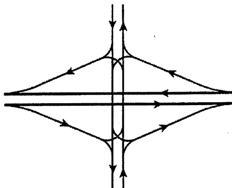
Conventional Diamond
