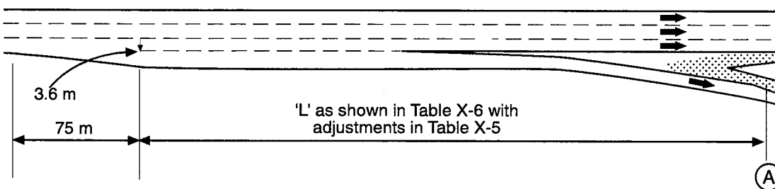
- C - PARALLEL DESIGN
