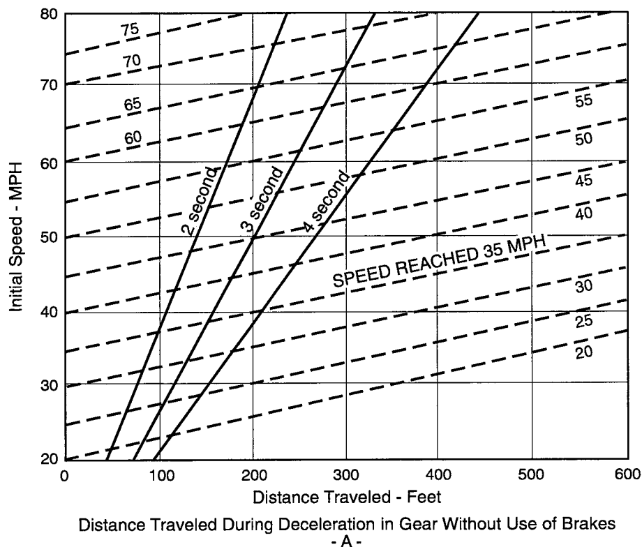
Figure 1.20. AASHO 1965, distance traveled during deceleration
